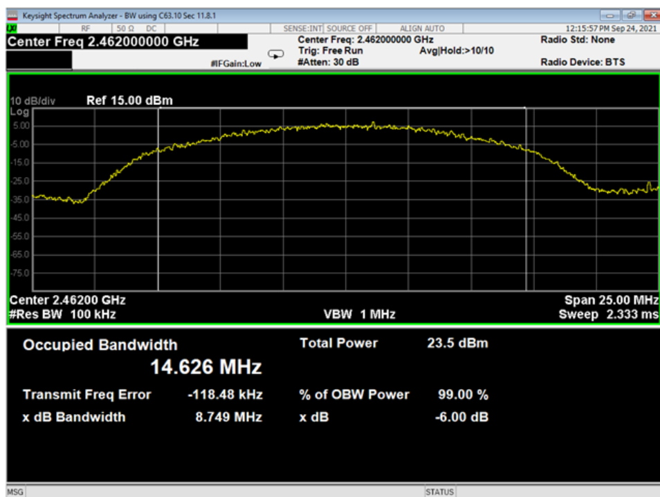
06 OBW-6dB, High, Wifi B
