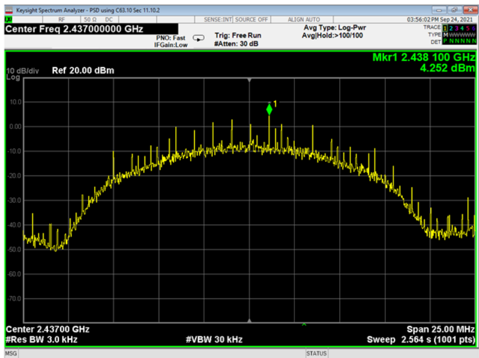
08 PSD, Mid, Wifi B
