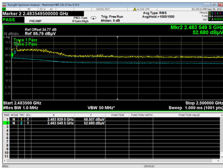
38 Higher Band Edge, Restricted, Wifi N
