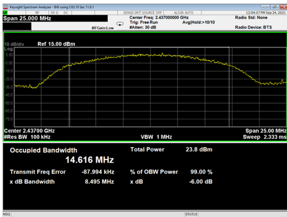
05 OBW-6dB, Mid, Wifi B
