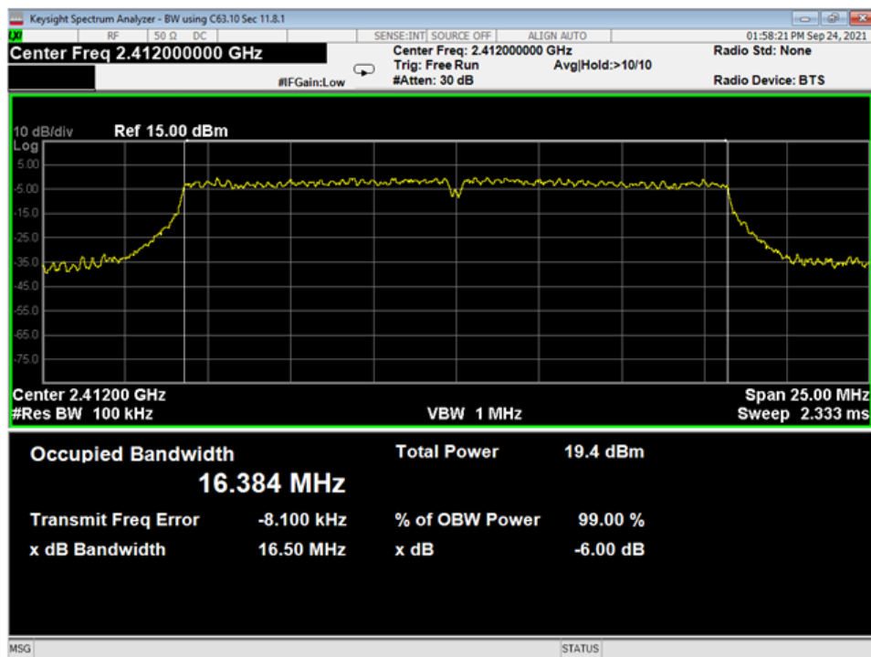
17 OBW-6dB, Low, Wifi G
