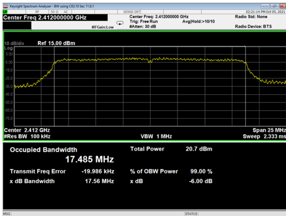
30 OBW-6dB, Low, Wifi N
