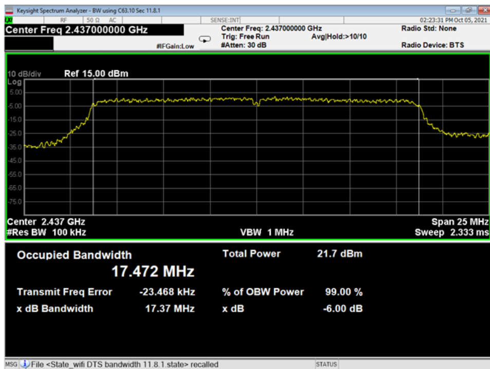
31 OBW-6dB, Mid, Wifi N
