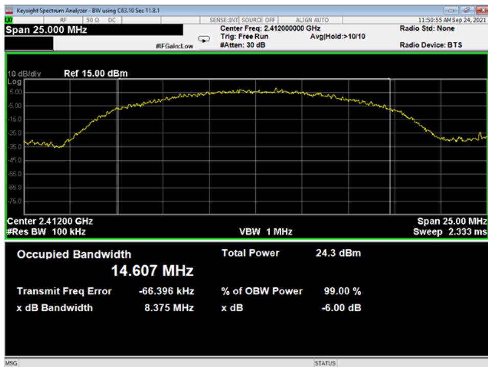
04 OBW-6dB, Low, Wifi B
