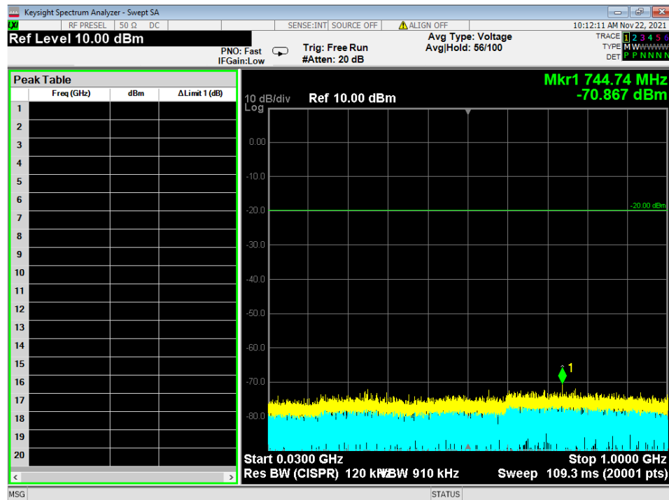
Figure 11 - Radiated Emissions Plot, WIFI 802.11g, 30M – 1G
