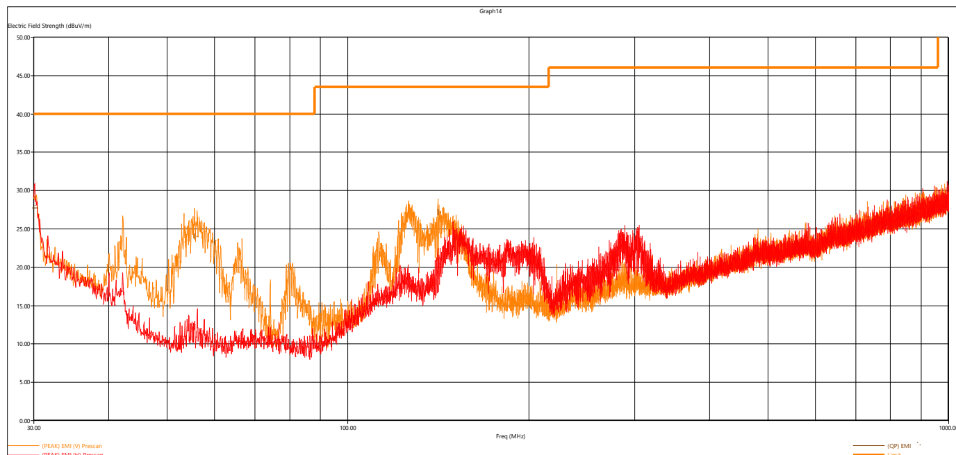
Figure 6 - Radiated Emissions Plot, 802.11g
