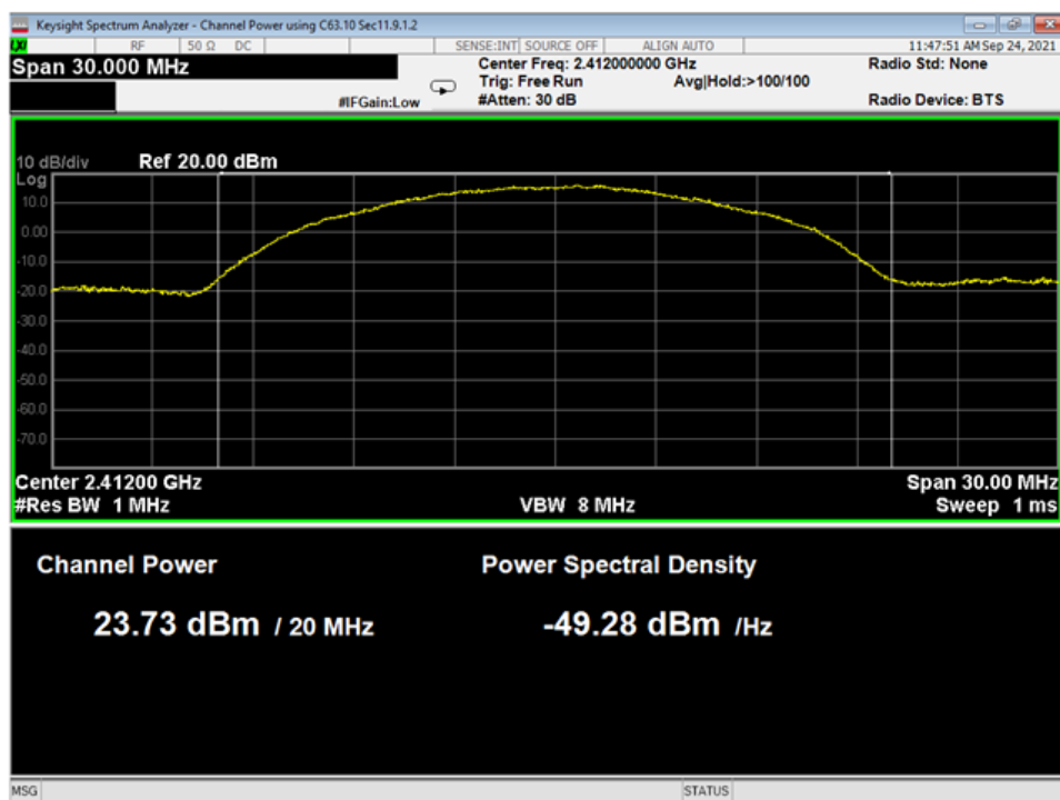
01 Pwr, Low, Wifi B
