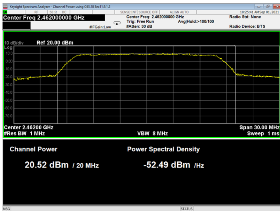
16 Pwr, High, Wifi G
