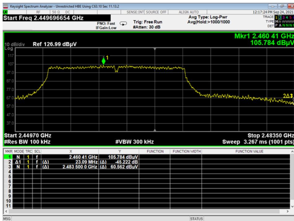
24 HBE, Unrestricted, Wifi G
