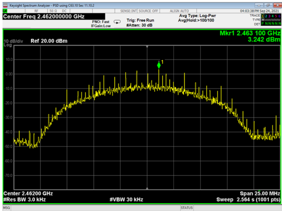
09 PSD, High, Wifi B
