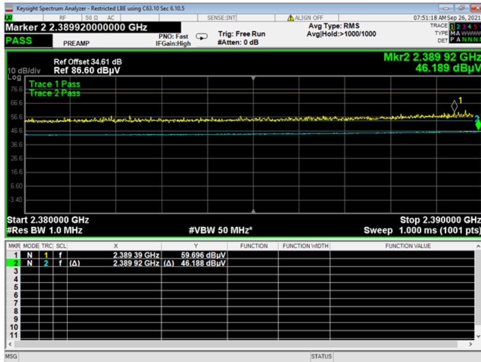
25 LBE Restricted Wifi G
