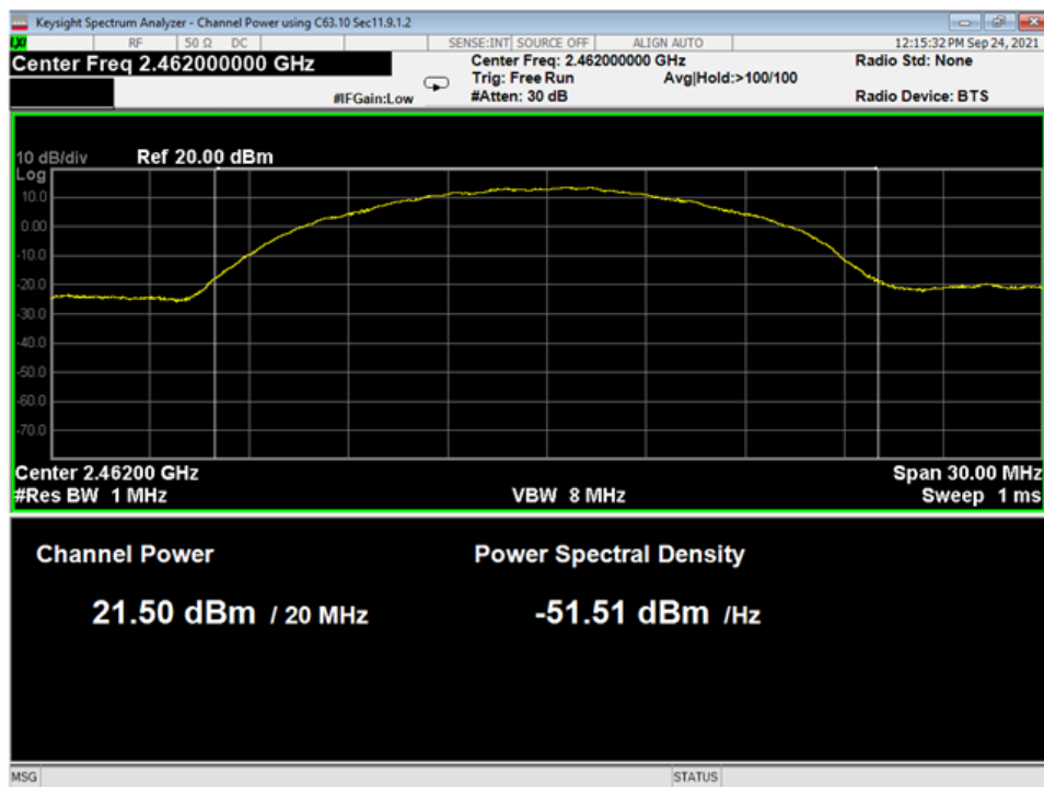
03 Pwr,High, Wifi B
