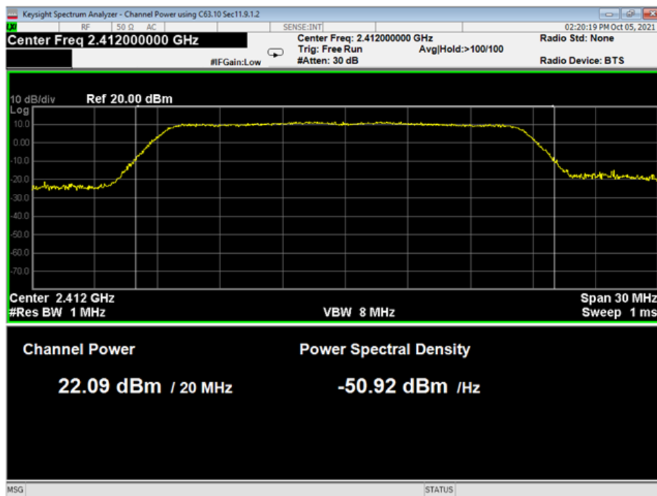
27 Power, Low, Wifi N
