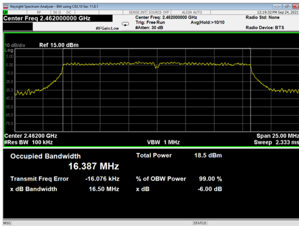
19 OBW-6dB, High, Wifi G
