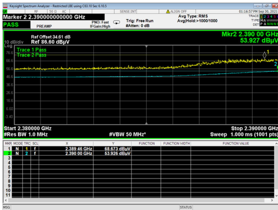
39 Lower Band Edge, Restricted, Wifi N
