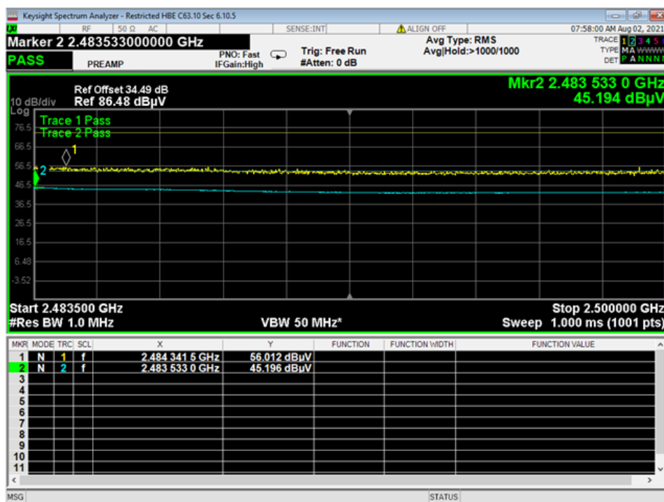
12 HBE Restricted Wifi B, 11Mbps
