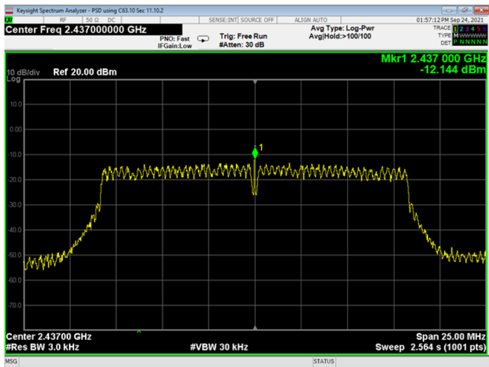
21 PSD, Mid, Wifi G
