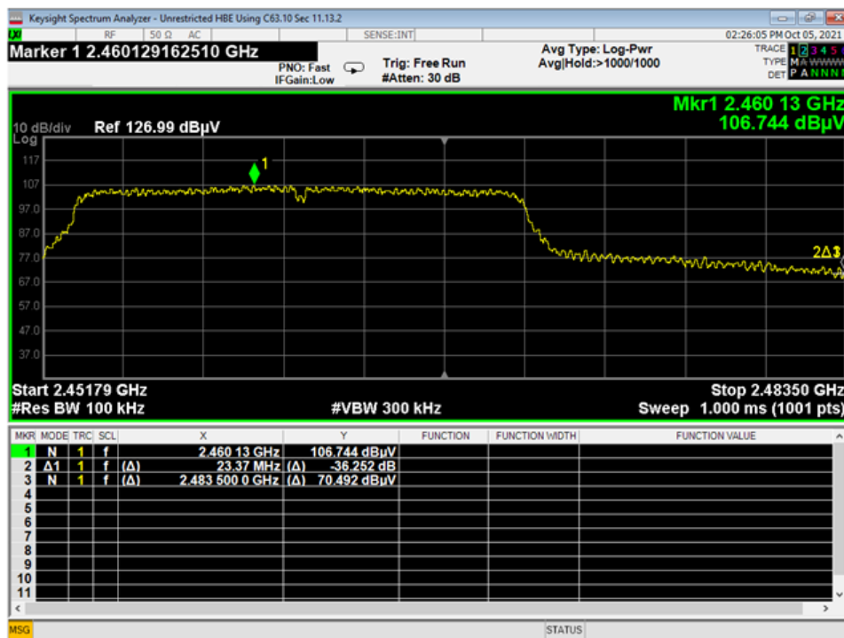
37 Higher Band Edge, Unrestricted, Wifi N
