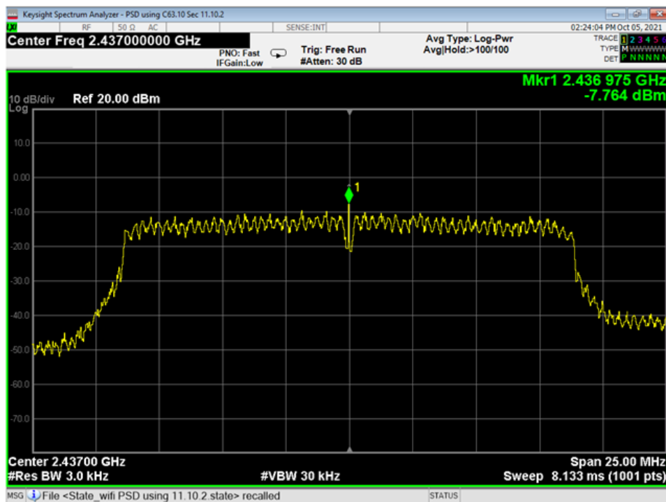
34 PSD, Mid, Wifi N
