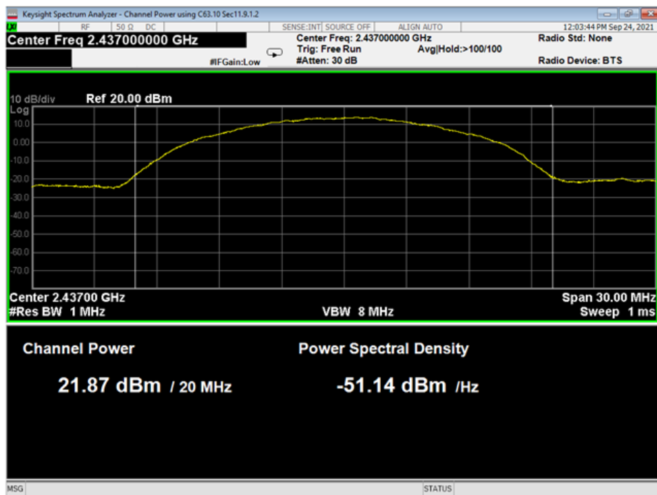
02 Pwr, Mid, Wifi B
