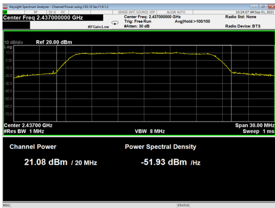
15 Pwr, Mid, Wifi G
