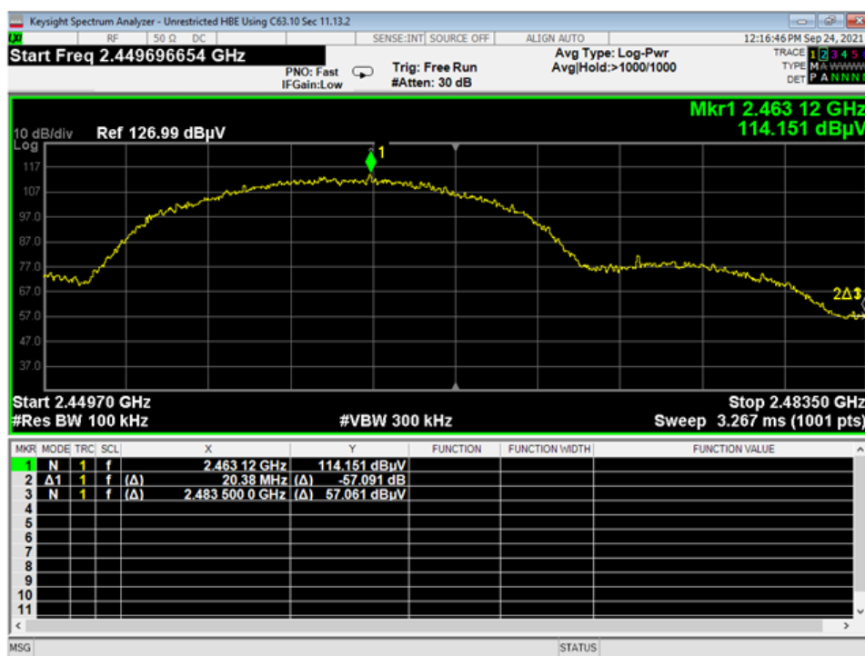
11 HBE, Unrestricted, Wifi B
