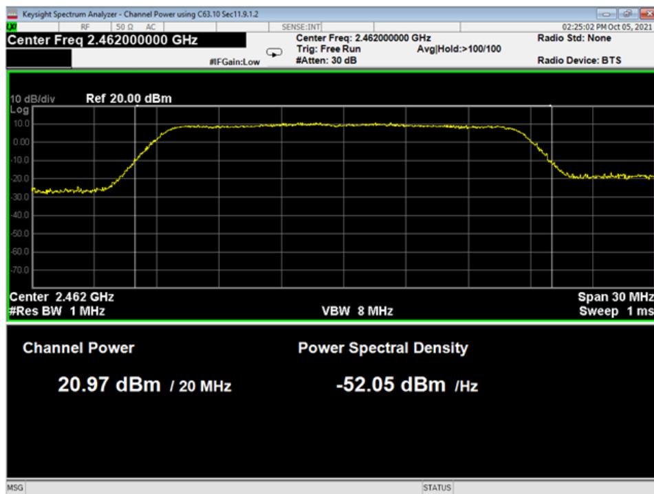
29 Power, High, Wifi N
