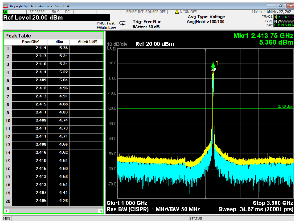
Figure 15 - Radiated Emissions Plot, WIFI 802.11n, 1G - 3.6G
