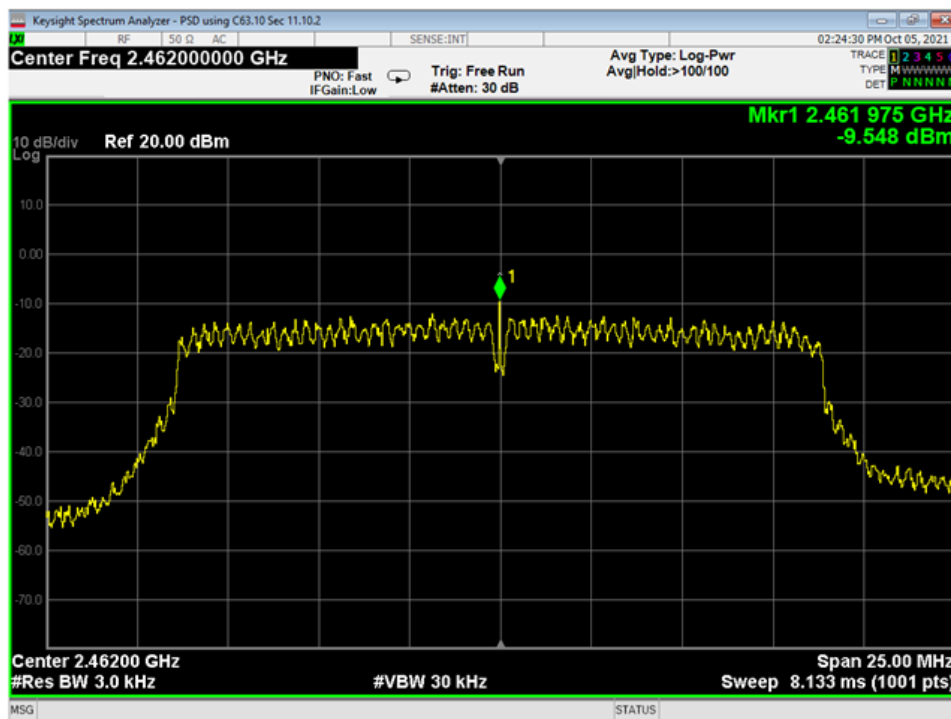
35 PSD, High, Wifi N
