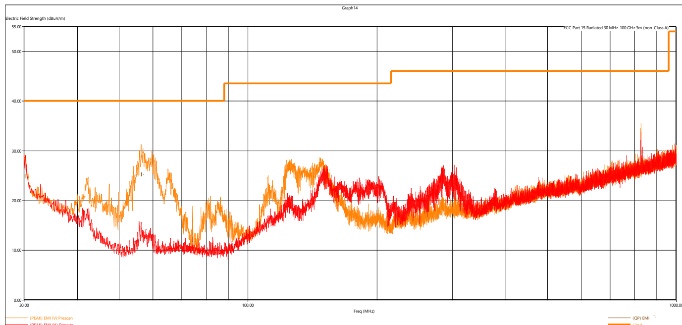
Figure 5 - Radiated Emissions Plot, 802.11b
