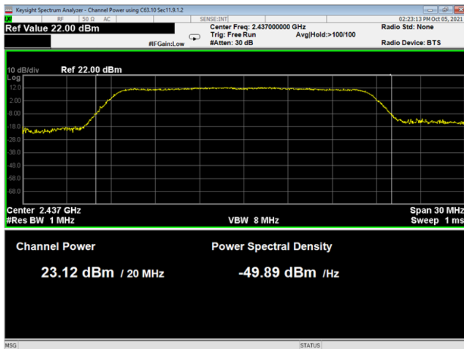
28 Power, Mid, Wifi N
