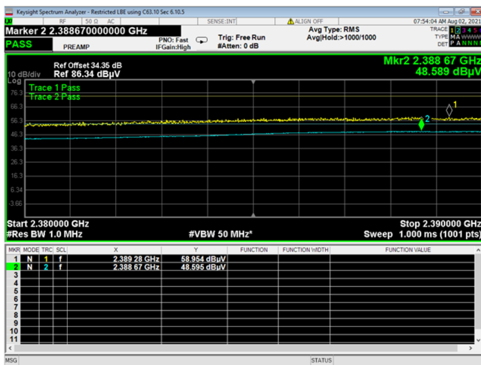
13 LBE Restricted Wifi B, 11MBps
