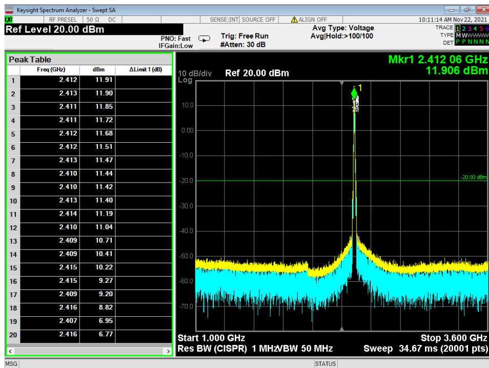
Figure 9 - Radiated Emissions Plot, WIFI 802.11b, 1G – 3.6G
