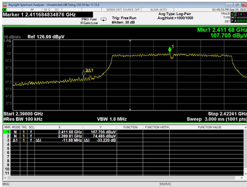
23 LBE, Unrestricted, Wifi G
