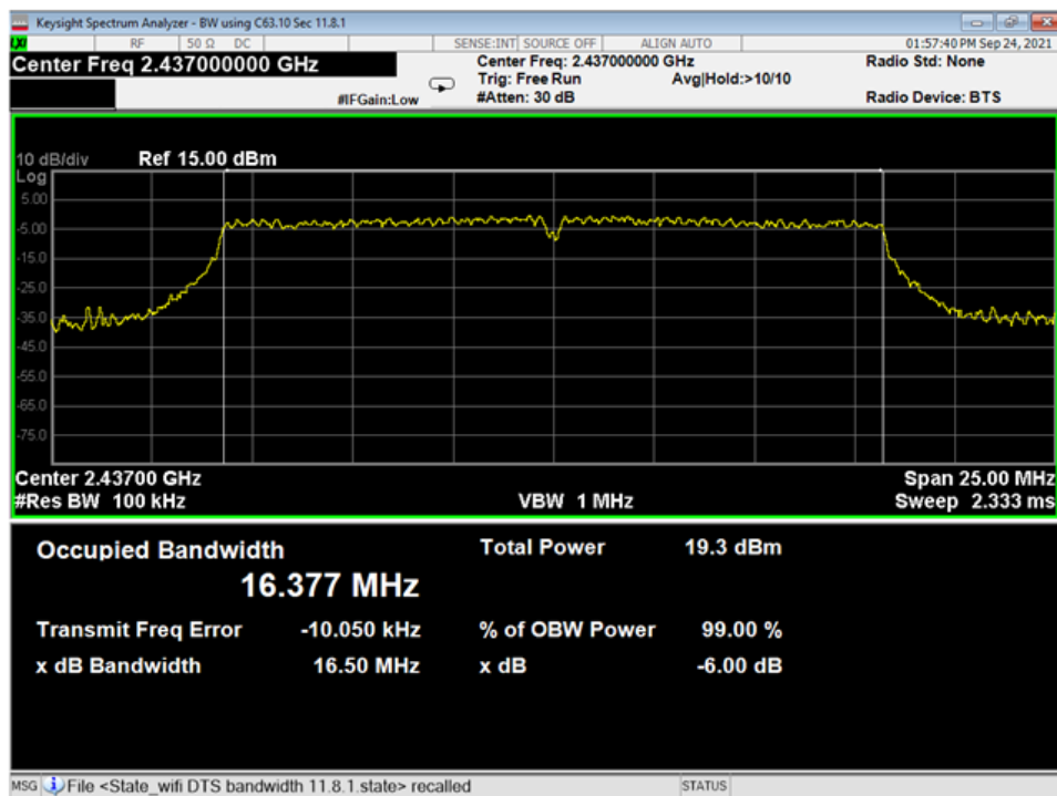
18 OBW-6dB, Mid, Wifi G
