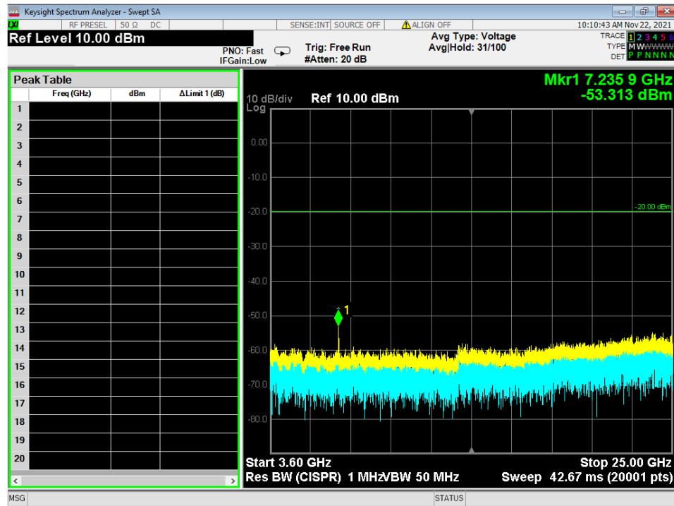
Figure 10 - Radiated Emissions Plot, WIFI 802.11b, 3.6G – 25G
