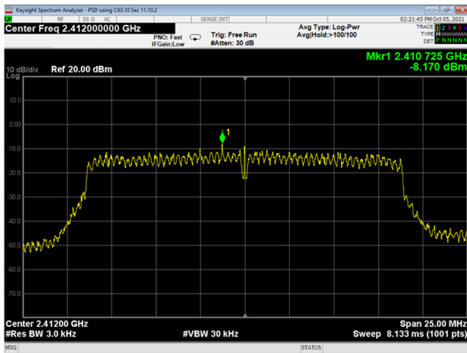
33 PSD, Low, Wifi N
