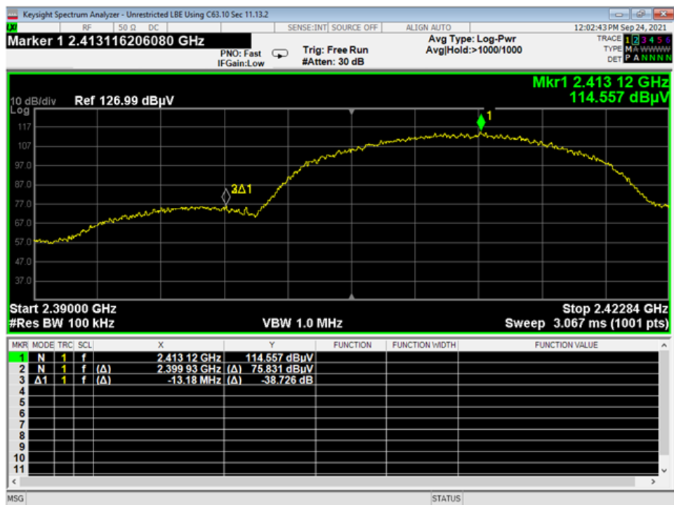
10 LBE, Unrestricted, Wifi B
