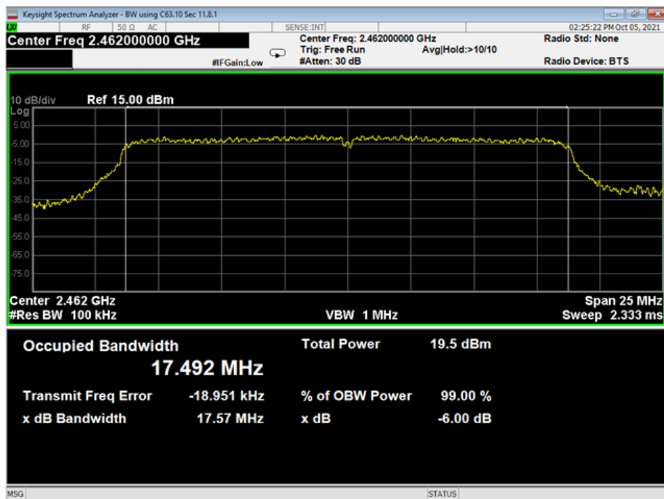
32 OBW-6dB, High, Wifi N
