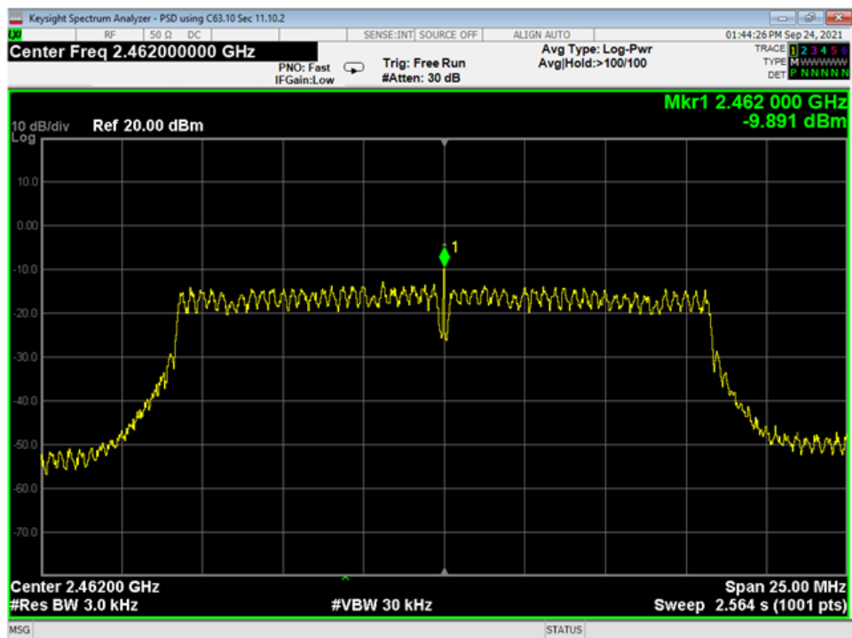
22 PSD, High, Wifi G
