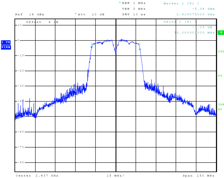
Figure 21 Plot of Transmitter 6-dB Occupied Bandwidth (802.11 n40-mode)
