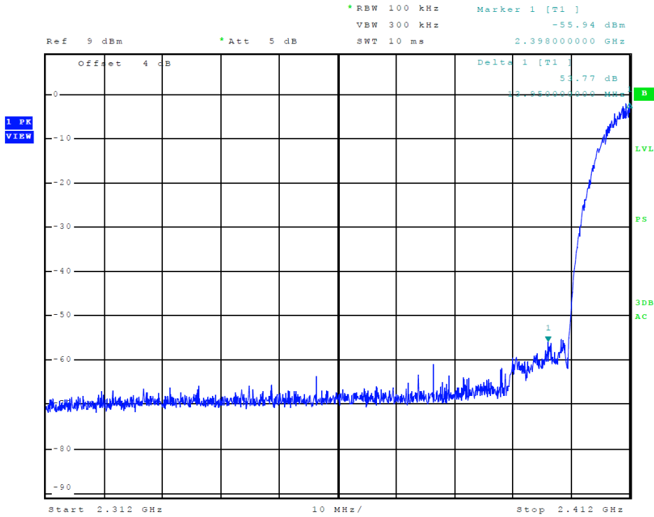
Figure 7 Plot of Lower Band Edge (802.11 b-mode)
