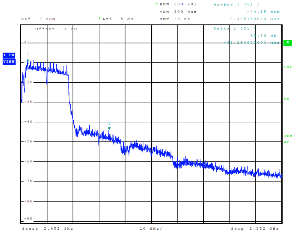
Figure 14 Plot of Upper Band Edge (802.11 n40-mode)
