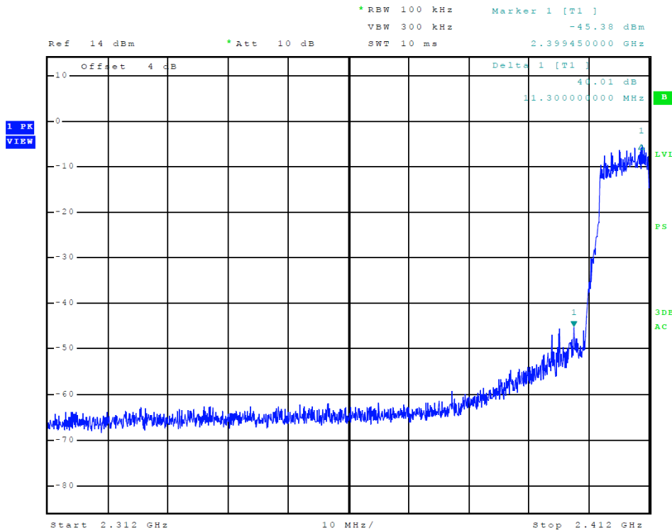
Figure 8 Plot of Lower Band Edge (802.11 g-mode)
