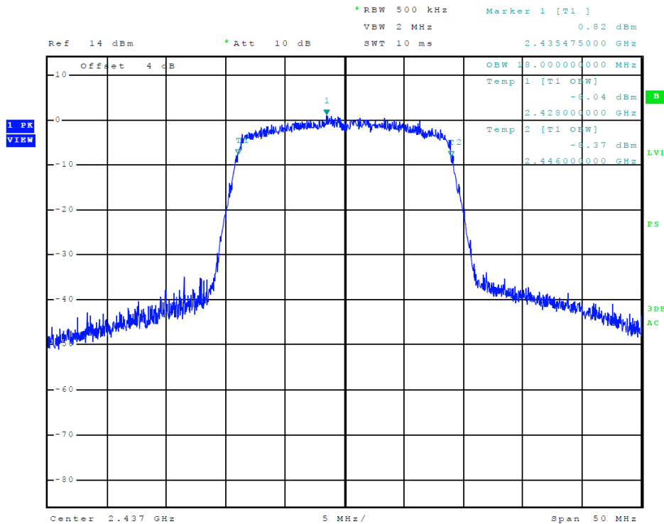
Figure 20 Plot of Transmitter 99% Occupied Bandwidth (802.11 n-mode)
