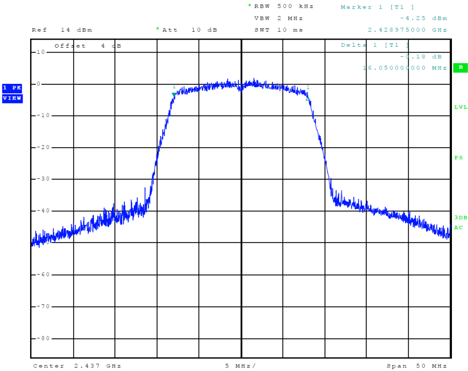
Figure 17 Plot of Transmitter 6-dB Occupied Bandwidth (802.11 g-mode)
