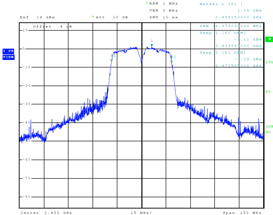
Figure 22 Plot of Transmitter 99% Occupied Bandwidth (802.11 n40-mode)
