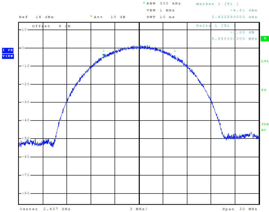
Figure 15 Plot of Transmitter 6-dB Occupied Bandwidth (802.11 b-mode)
