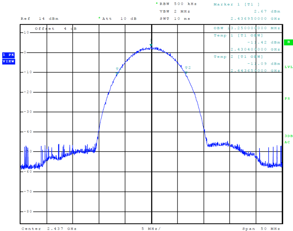
Figure 16 Plot of Transmitter 99% Occupied Bandwidth (802.11 b-mode)
