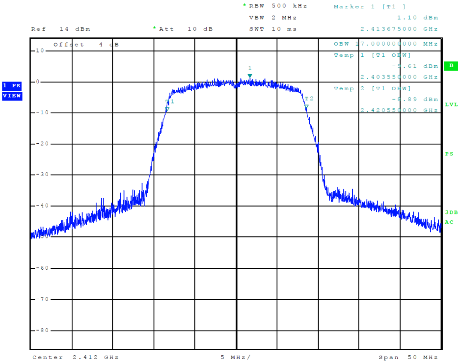
Figure 18 Plot of Transmitter 99% Occupied Bandwidth (802.11 g-mode)
