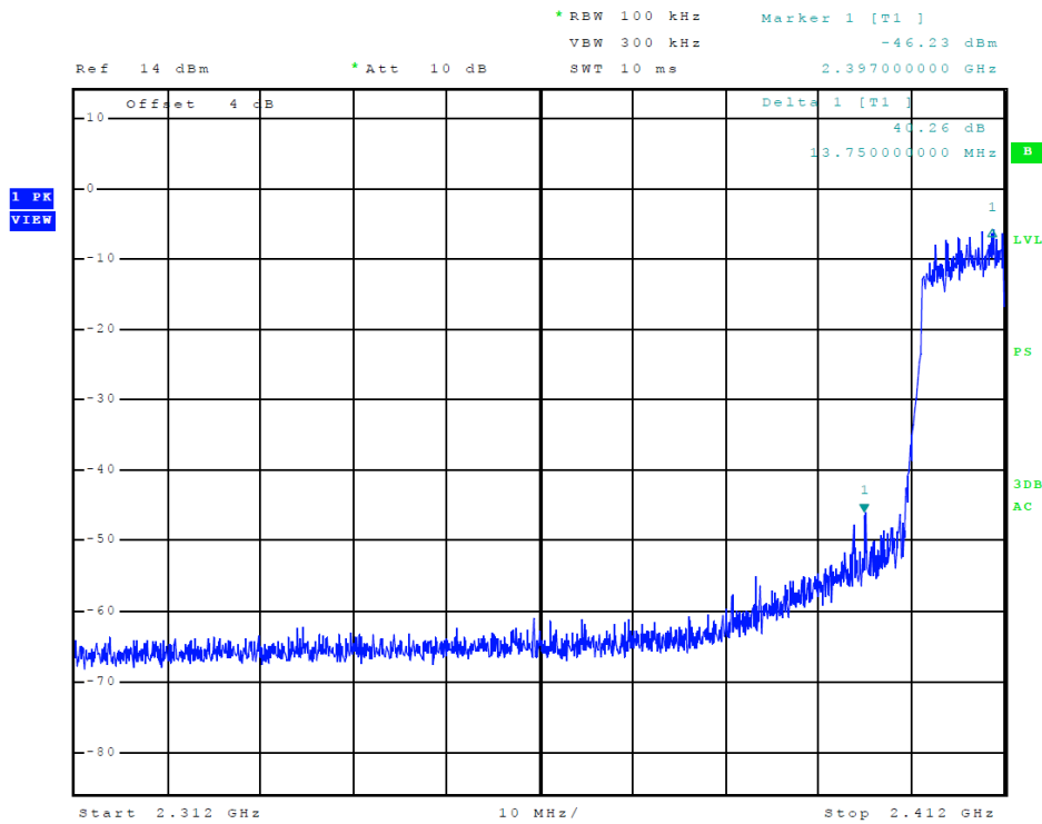
Figure 9 Plot of Lower Band Edge (802.11 n-mode)
