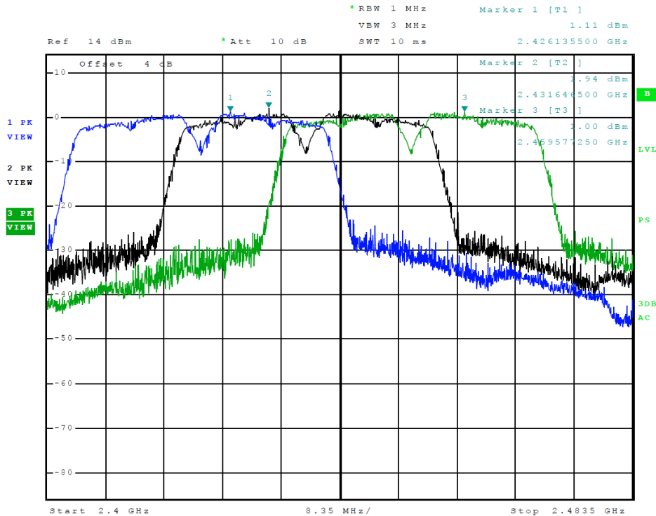
Figure 6 Plot of Transmitter Emissions in Operational Frequency (802.11 n40-Mode)
