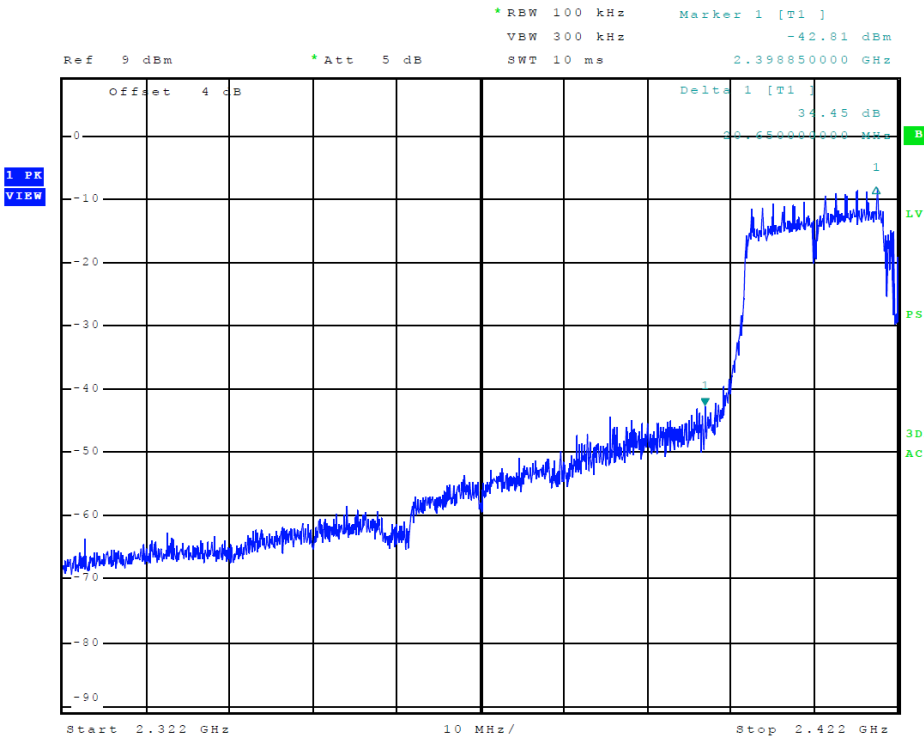
Figure 10 Plot of Lower Band Edge (802.11 n40-mode)
