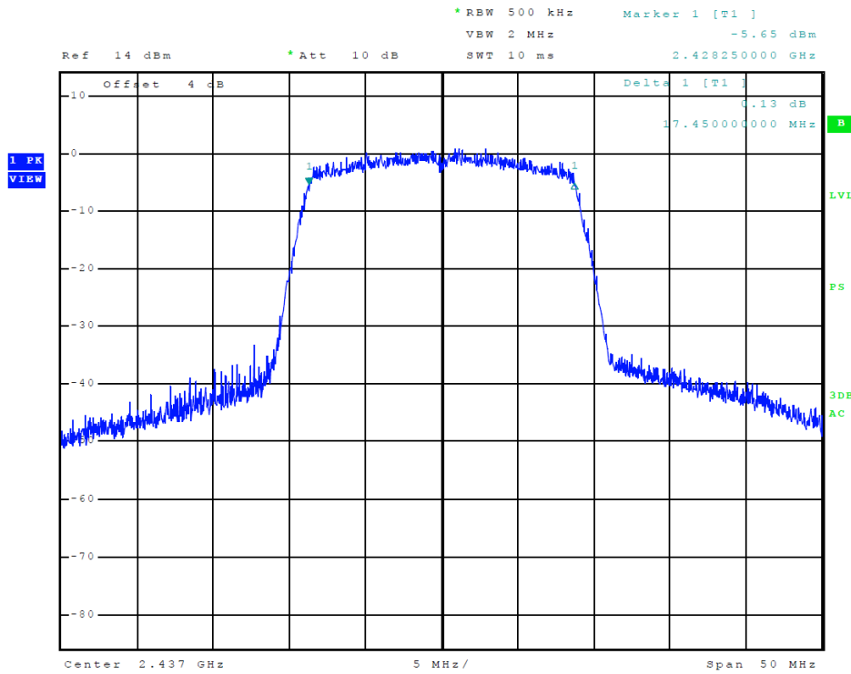
Figure 19 Plot of Transmitter 6-dB Occupied Bandwidth (802.11 n-mode)
