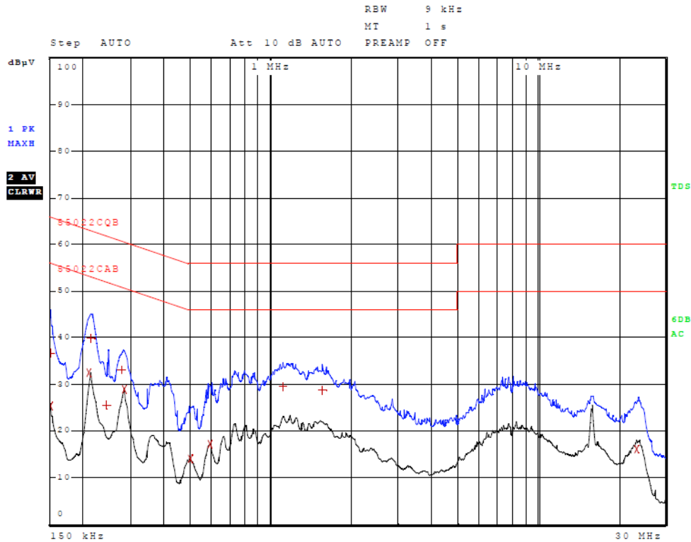
Figure 2 AC Line Conducted emissions of EUT line 2 (EUT AC Adapter 326-00086-01)
