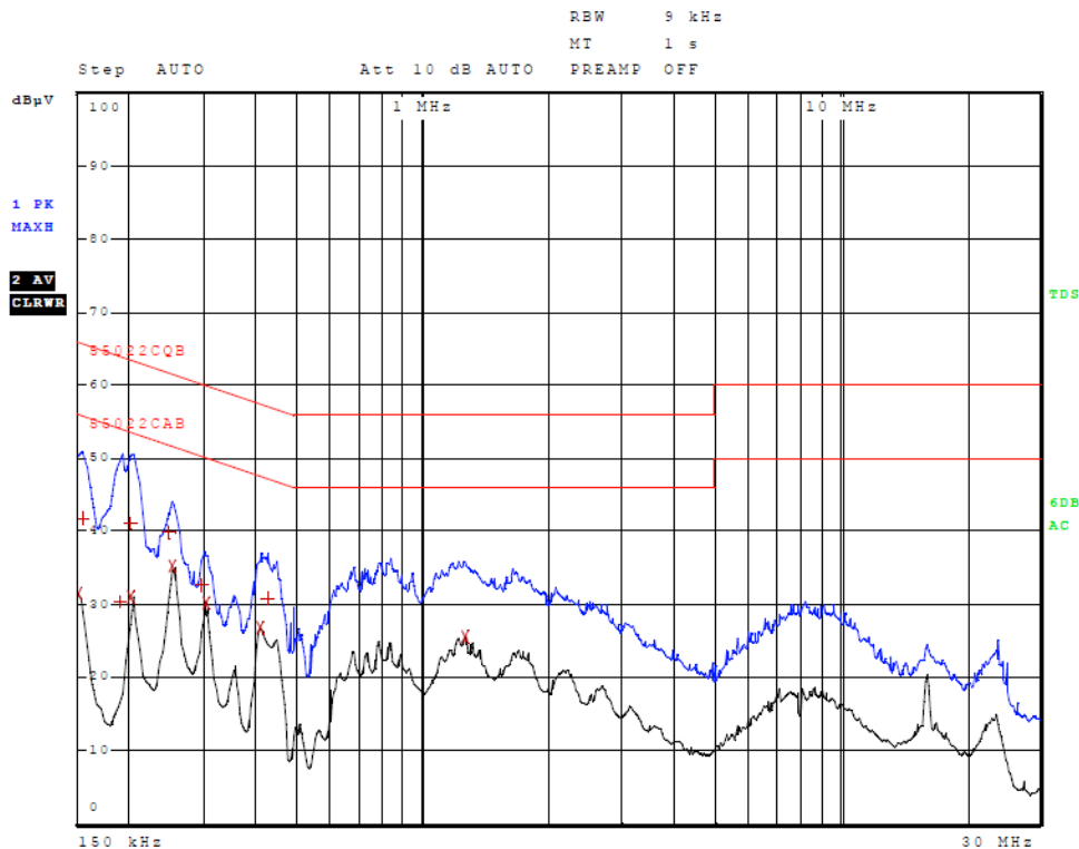
Figure 2 AC Line Conducted emissions of EUT line 2 (EUT AC Adapter 326-00072-xx)
