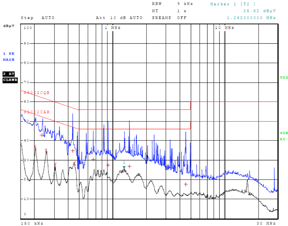
Figure 1 AC Line Conducted emissions of EUT line 1 (EUT AC Adapter 326-00072-xx)
