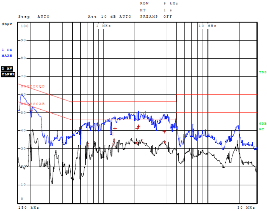
Figure 3 AC Line Conducted emissions of EUT line 1 (EUT CPU)
