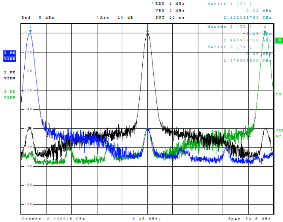
Figure 5 Plot of Transmitter Emissions (In 2402-2480 MHz)
