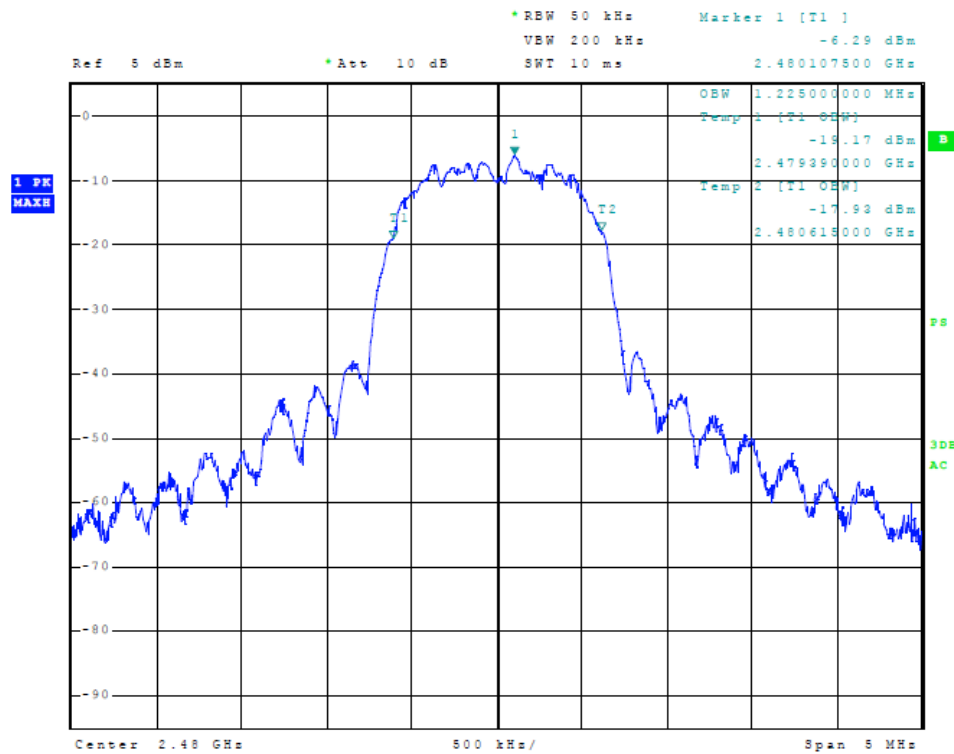
Figure 6 Plot of Transmitter Emissions (2402-2480 MHz, 99% Occupied Bandwidth)
