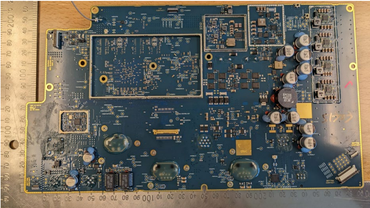
PCBA: (Front)
