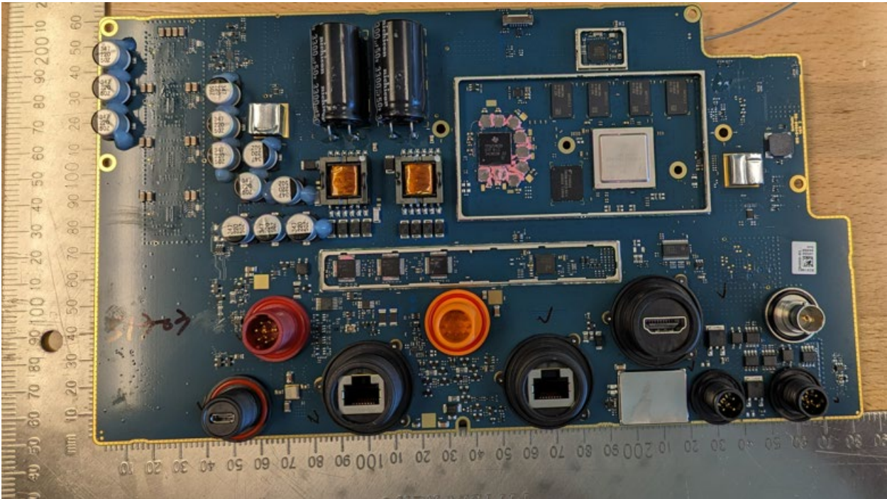
PCBA: (Back)
