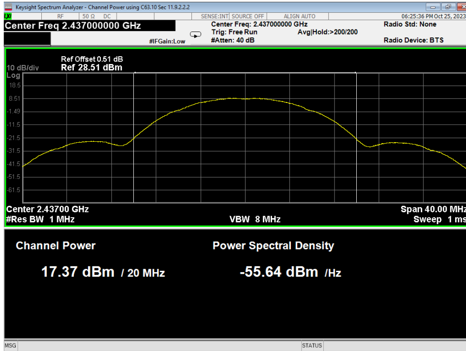
Figure 3 – Conducted Average Power Measurement, 802.11b
