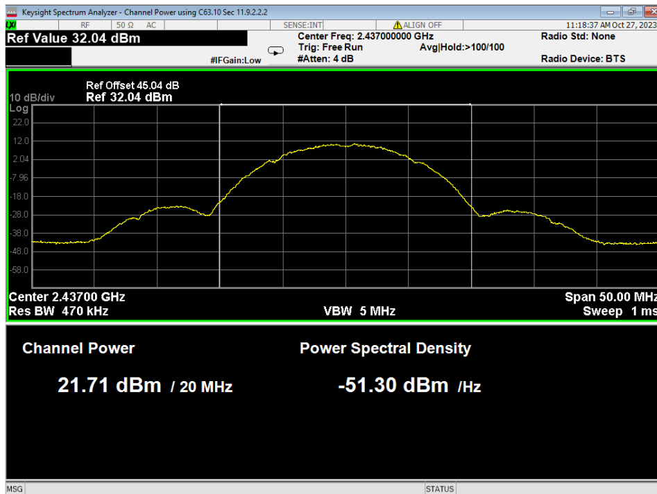
Figure 4 – Radiated Average Power Measurement, 802.11b Measurement corrections/EIRP conversions are included in reference offset.
