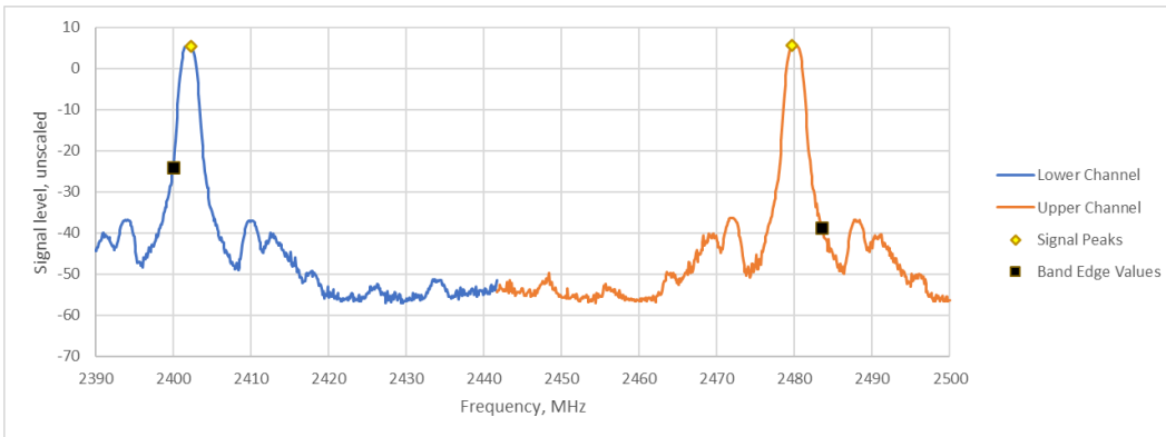
Figure TR16.2: Spectral data for BLE 1Mbps at -10 °C
