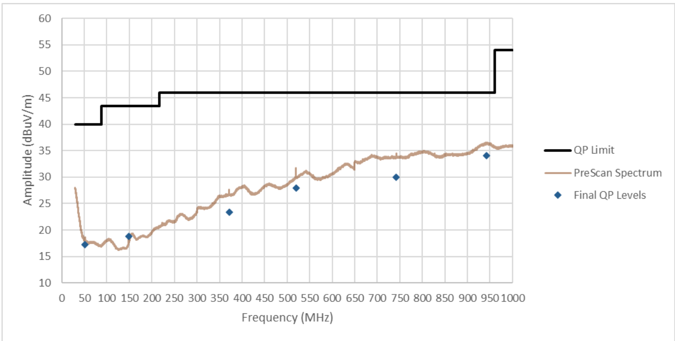
Figure RE07.1: Spectral data (Low Channel)
