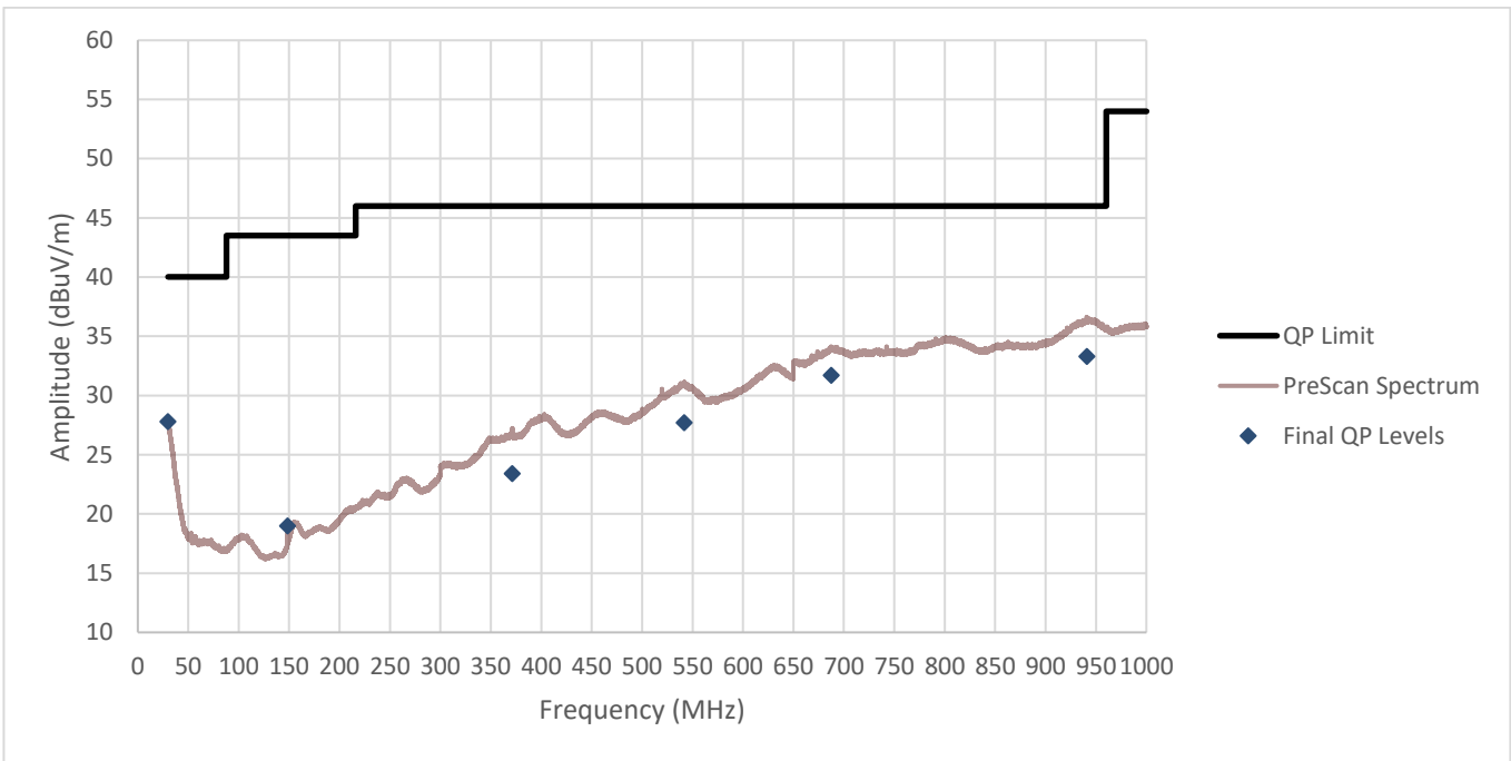
Figure RE07.3: Spectral data (High Channel)
