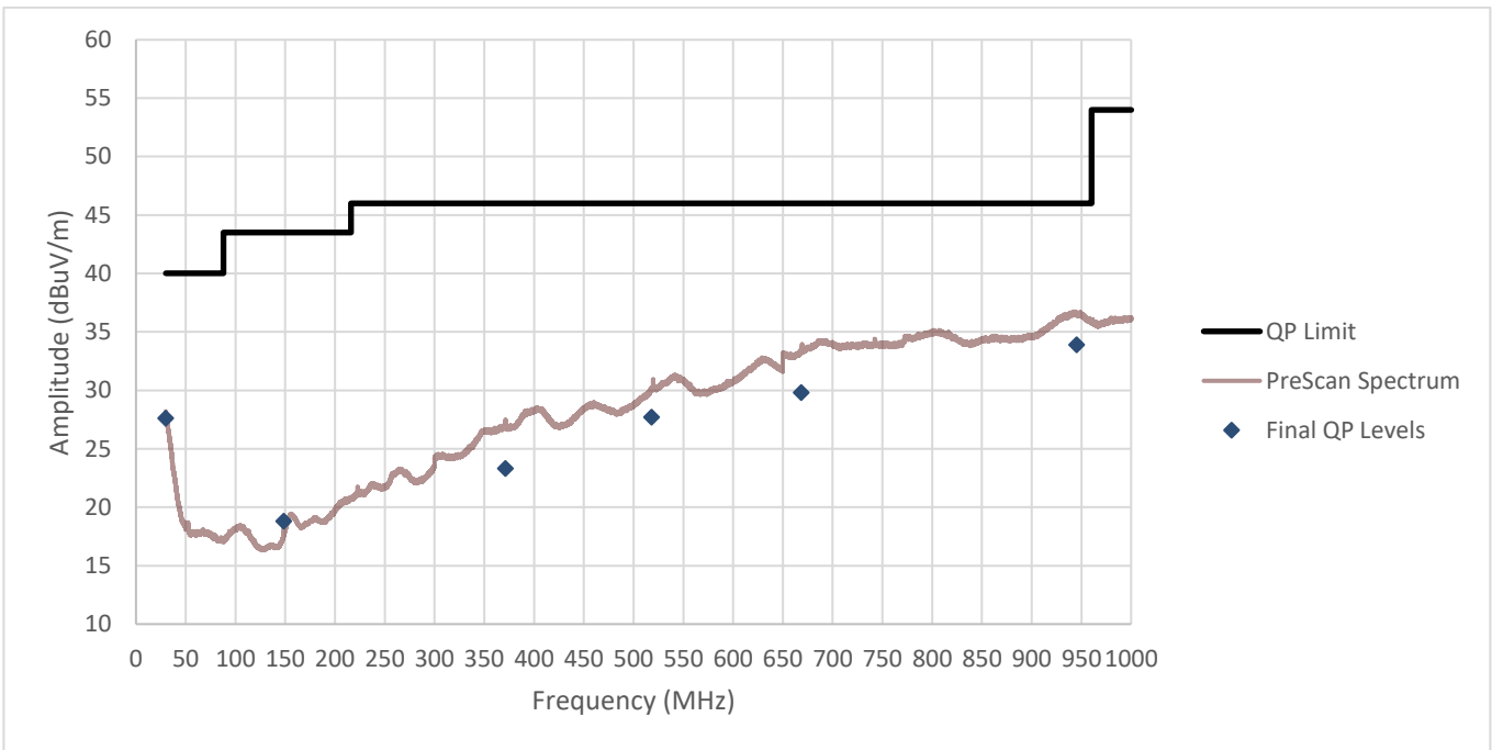
Figure RE07.2: Spectral data (Mid Channel)
