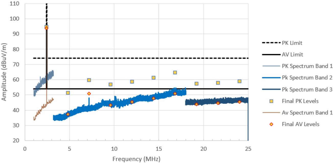
Figure RE08.1: Spectral data for the 2402 MHz transmission frequency
