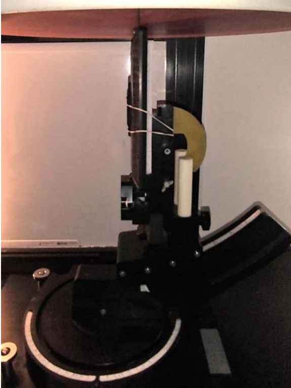
Figure C.3 – Setup Photos, Right Edge Touch - ELI Phantom
