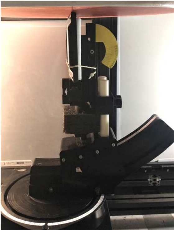
Figure C.4 – Setup Photos, Bottom - Touch – ELI Phantom
