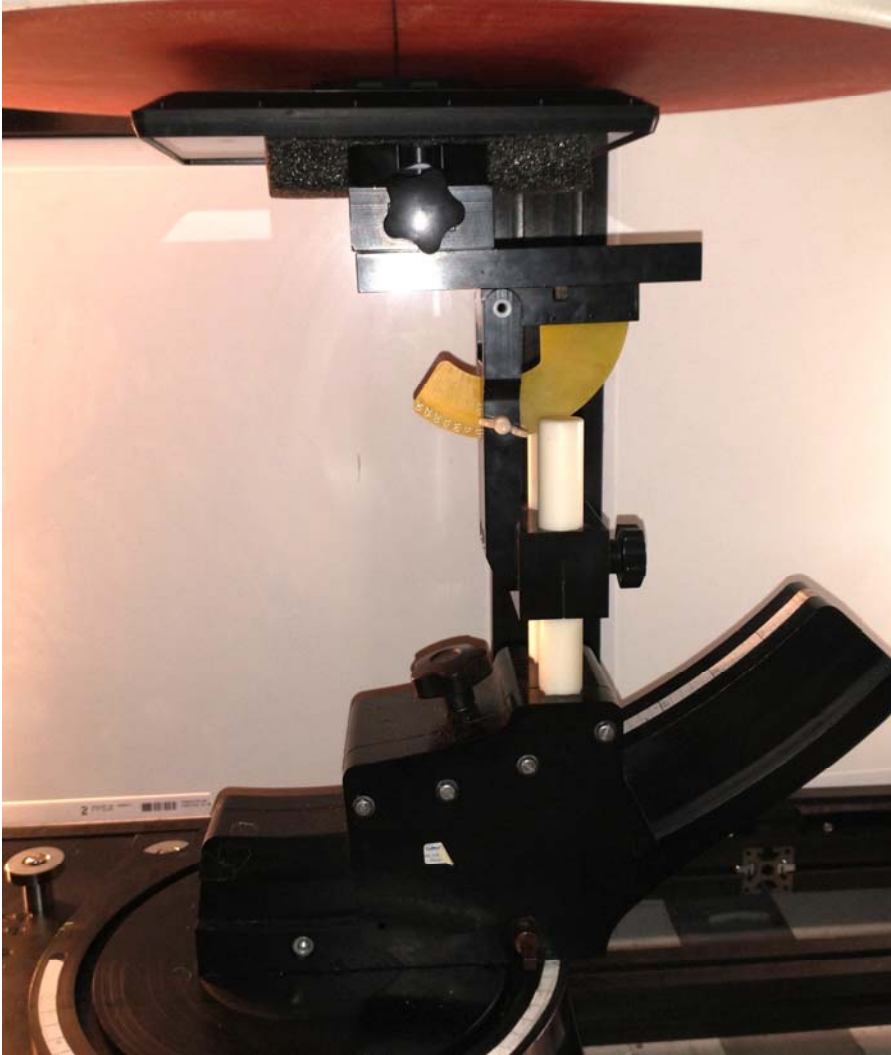
Figure C.1 – Setup Photos, Back Side Touch – ELI Phantom
