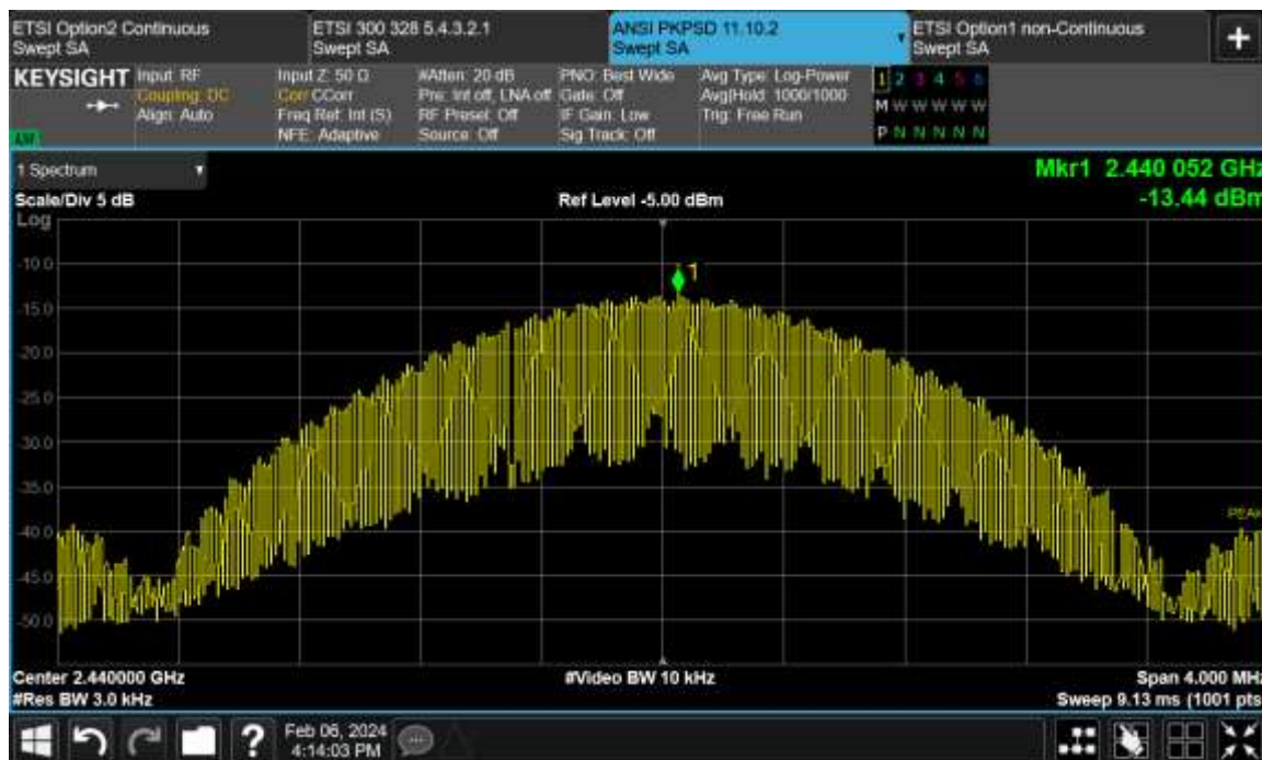
Figure TR20.2: Test data for BLE 2 Mbps, 2440 MHz
