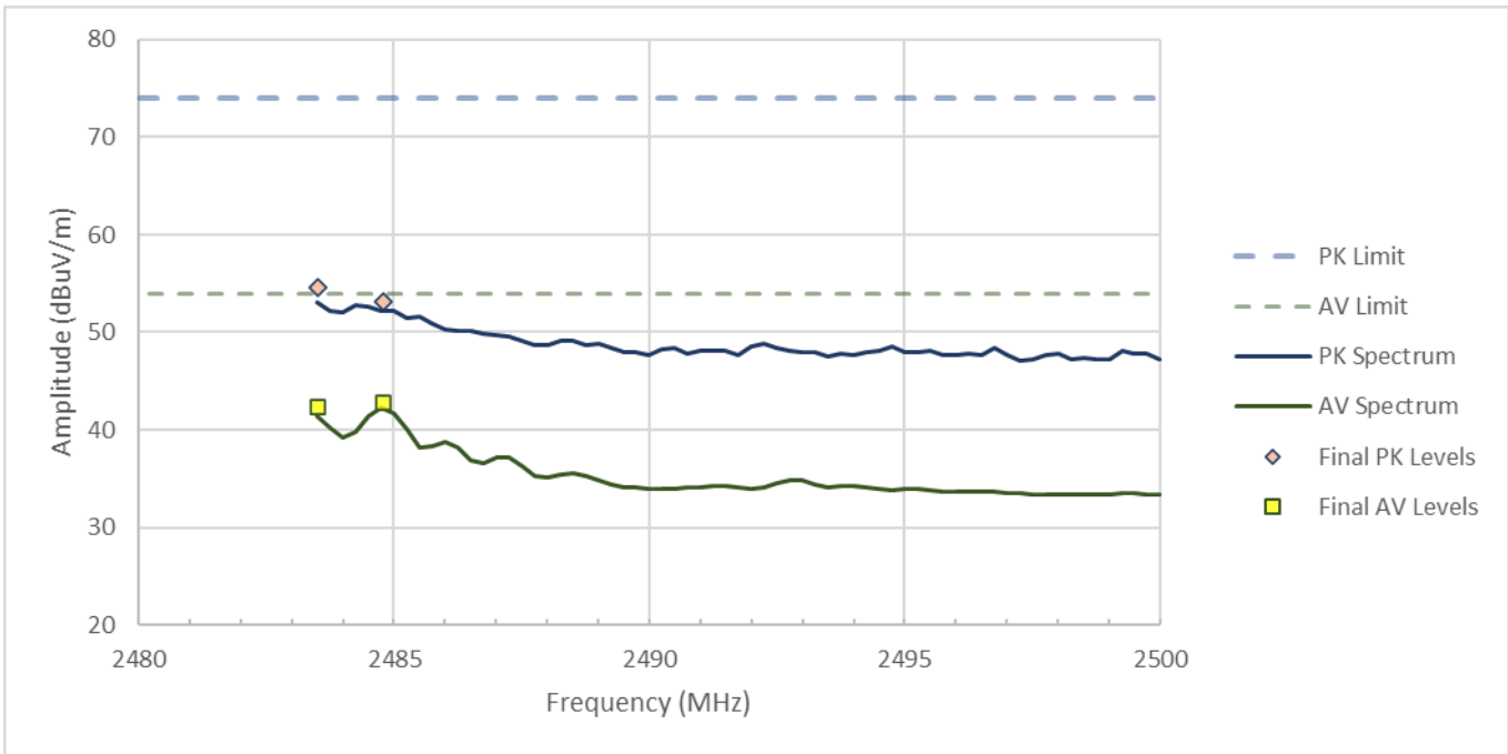
Figure RE02.2: FCC restricted band spectral data from 2483.5 to 2500 MHz (Y orientation) BLE 2 Mbps.
