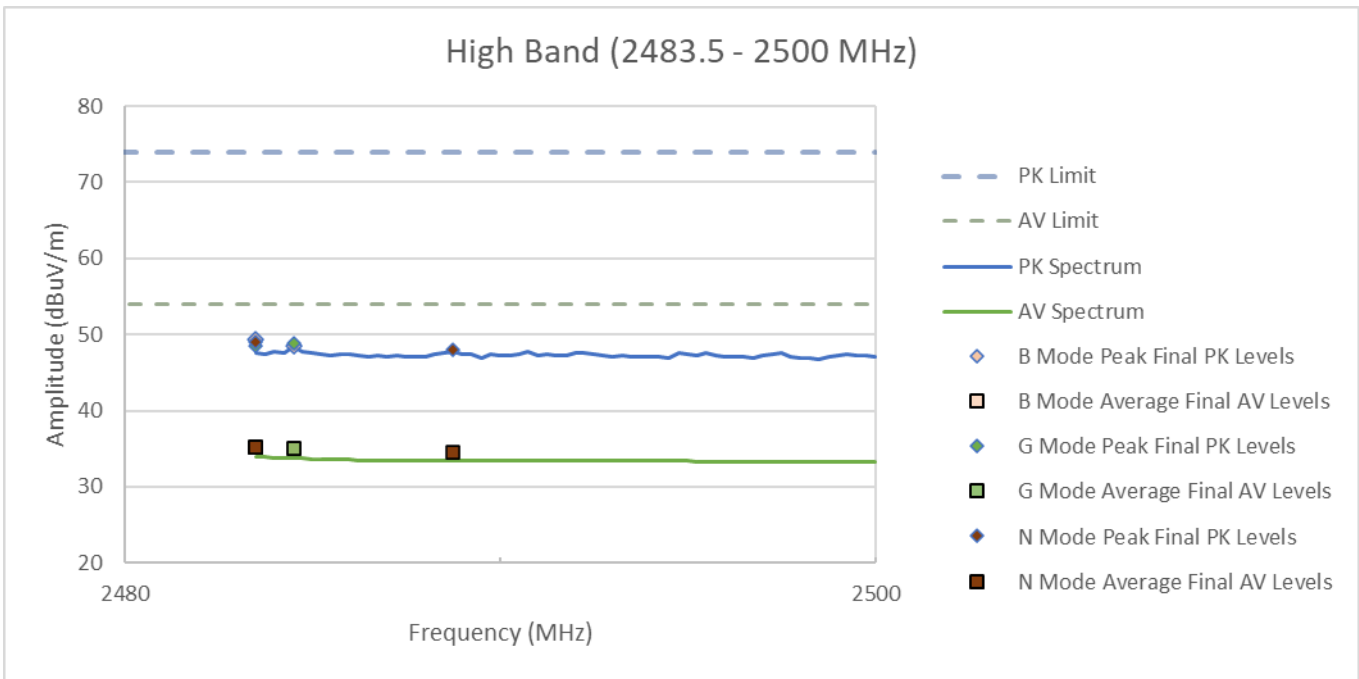
Figure RE04.2: FCC restricted band spectral data from 2483.5 to 2500 MHz (EUT transmitting on channel 11)
