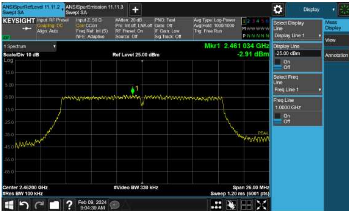
Figure TR28.8: Reference level measurement for IEEE 802.11 G 24 Mbps on Ch.11
