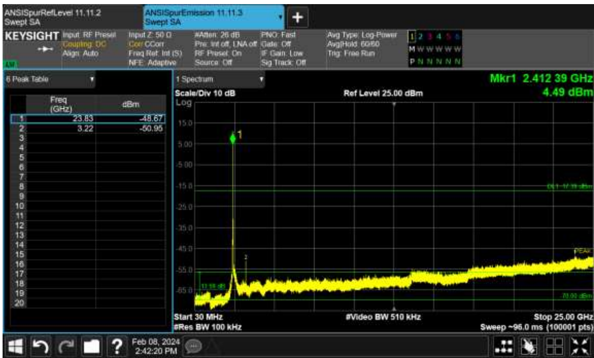
Figure TR28.7: Spectral data for IEEE 802.11 B 1 Mbps on Ch.1
