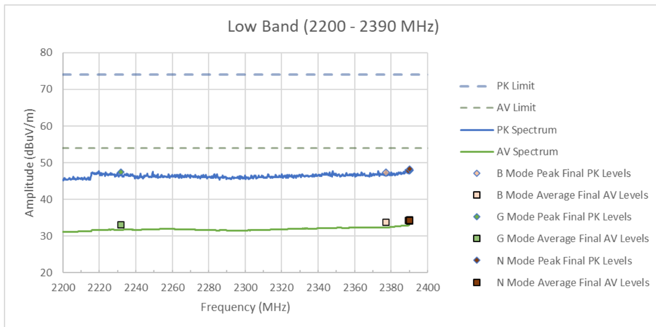
Figure RE04.1: FCC restricted band spectral data from 2200 to 2390 MHz (EUT transmitting on channel 1)
