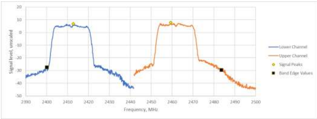
Figure TR44.3: Spectral data for IEEE 802.11 n MCS5 at 20 °C and 4.25 Vdc which represents Ch1 and Ch11.
