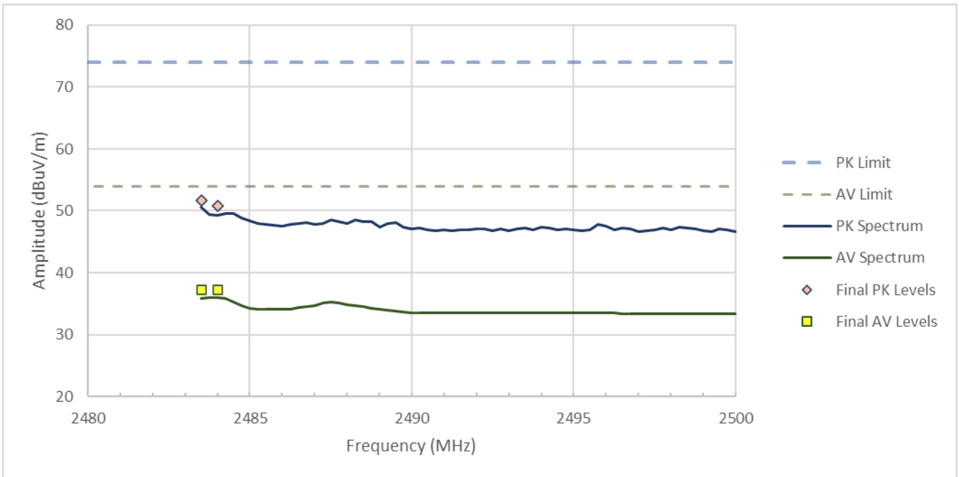
Figure RE03.2: FCC restricted band spectral data from 2483.5 to 2500 MHz (Y orientation)
