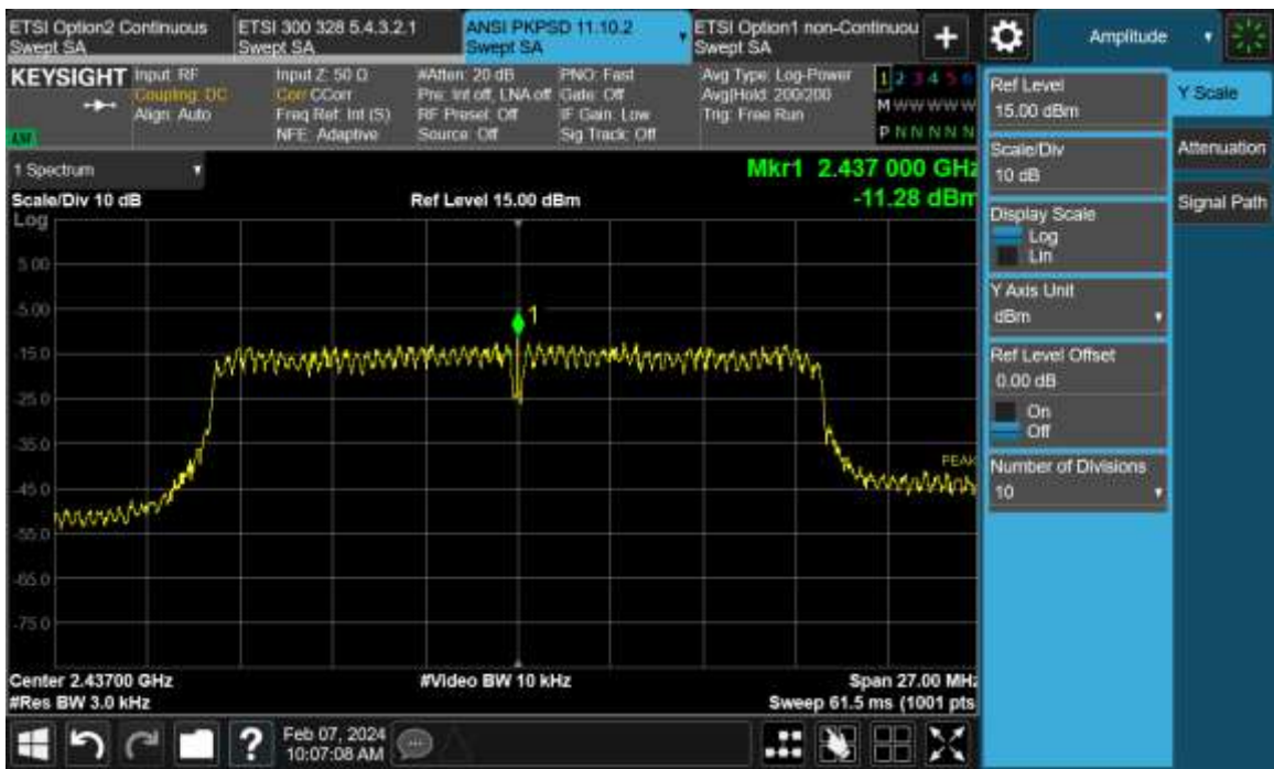
Figure TR20.6: Test data for WiFi mode N MCS1, Ch6
