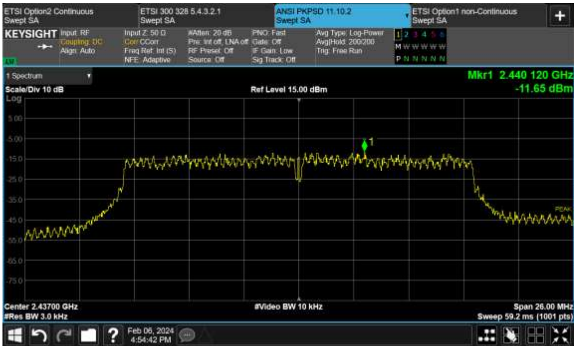
Figure TR20.5: Test data for WiFi mode G24 Mbps, Ch6
