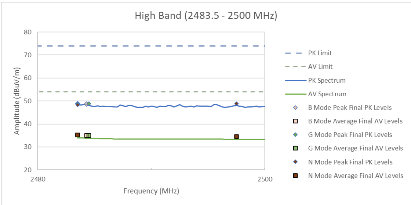
Figure RE04.3: FCC restricted band spectral data from 2483.5 to 2500 MHz (EUT transmitting on channel 12)
