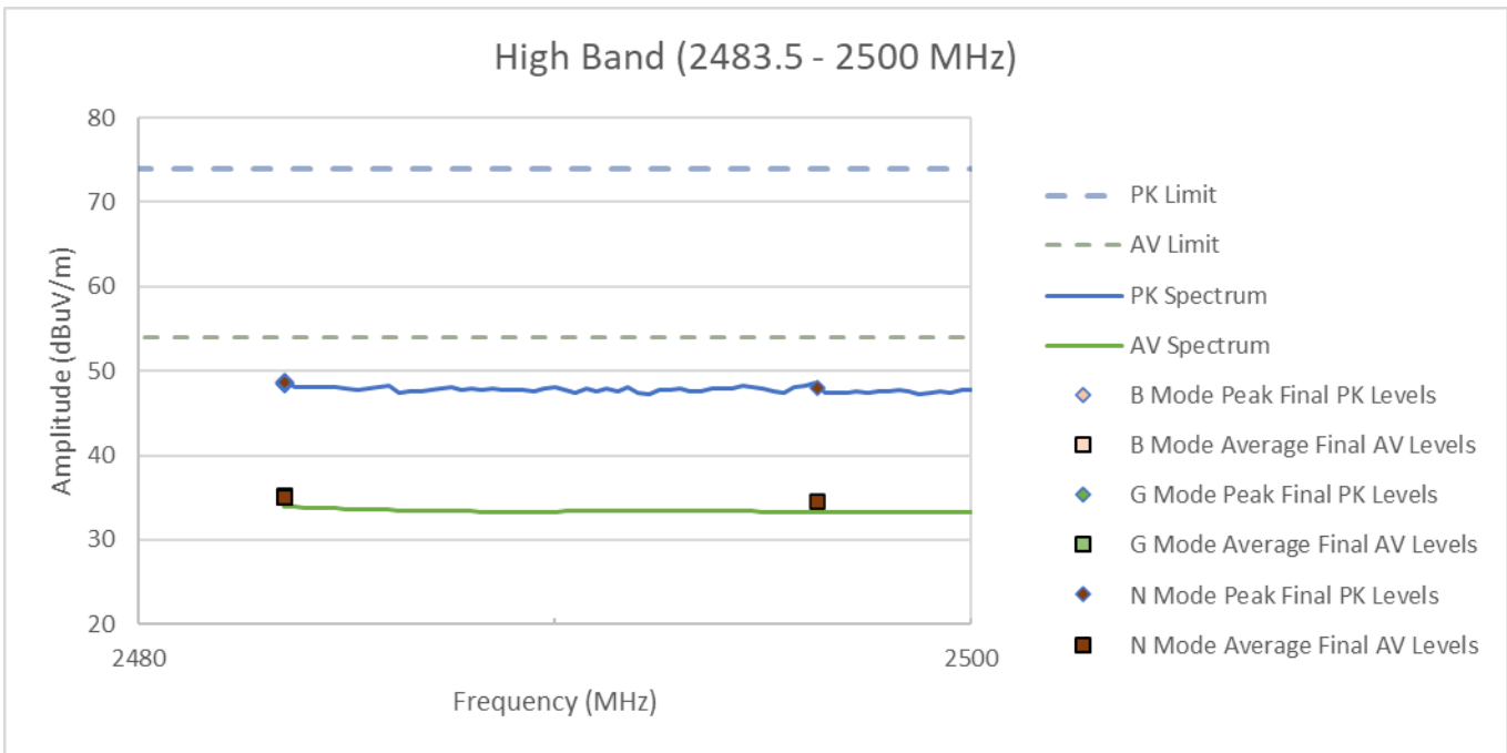
Figure RE04.4: FCC restricted band spectral data from 2483.5 to 2500 MHz (EUT transmitting on channel 13)
