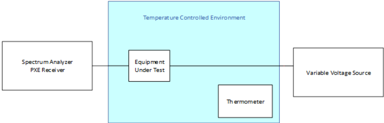
Figure TR44.5: Schematic drawing of the test equipment setup
