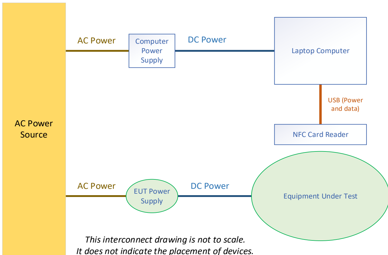
Figure 4: Block diagram of equipment arrangement A9
