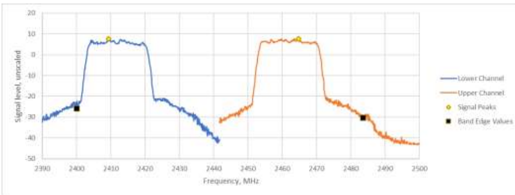
Figure TR44.1: Spectral data for IEEE 802.11 n MCS5 at -10 °C which represents Ch1 and Ch11.
