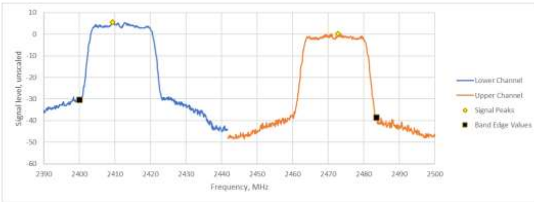
Figure TR44.2: Spectral data for IEEE 802.11 n MCS5 at -10 °C which represents Ch1 and Ch13.
