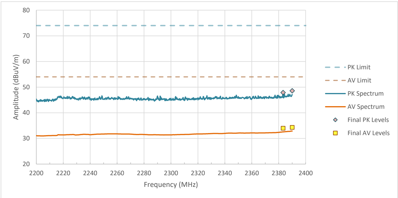
Figure RE02.1: FCC restricted band spectral data from 2200 to 2390 MHz (Y orientation) BLE 2 Mbps.
