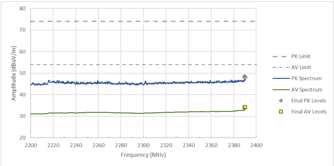
Figure RE03.1: FCC restricted band spectral data from 2200 to 2390 MHz (Y orientation)
