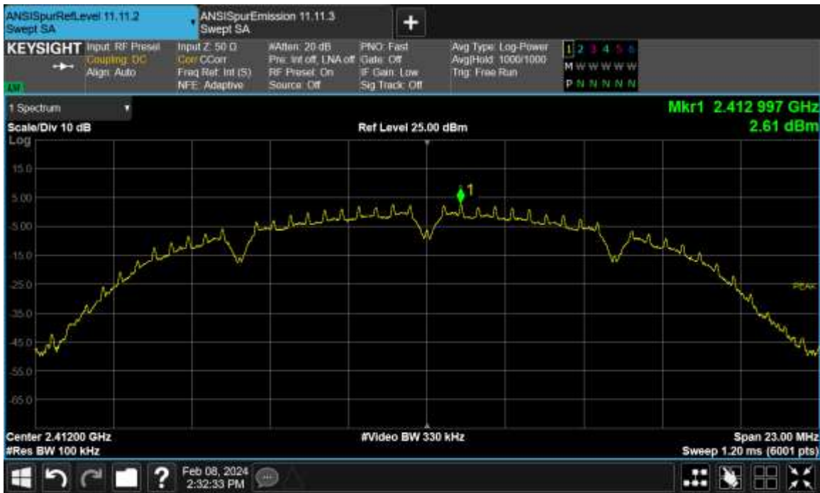
Figure TR28.6: Reference level measurement for IEEE 802.11 B 1 Mbps on Ch.1
