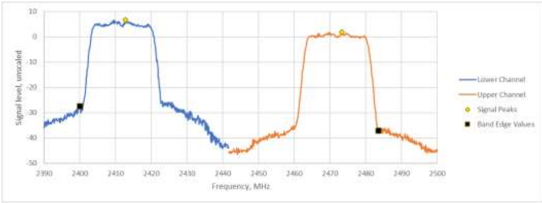
Figure TR44.4: Spectral data for IEEE 802.11 n MCS5 at 20 °C and 4.25 Vdc which represents Ch1 and Ch13.
