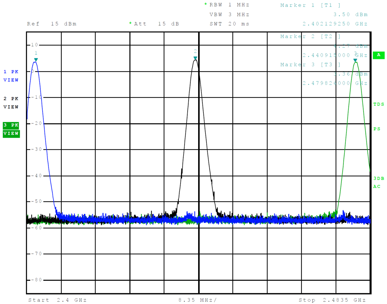
Figure 5 Plot of Transmitter Emissions Operation in 2402-2480 MHz Mode 2 BT 2EDR
