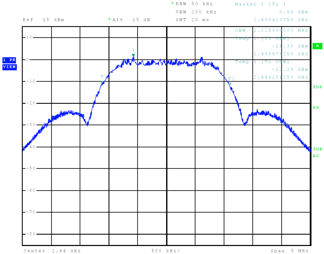
Figure 28 Plot of 99% Occupied Bandwidth Mode 4 BT BLE
