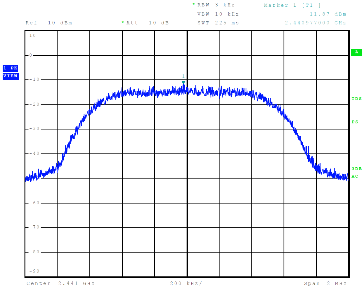
Figure 35 Plot of Transmitter Power Spectral Density Mode 2 BT 2EDR
