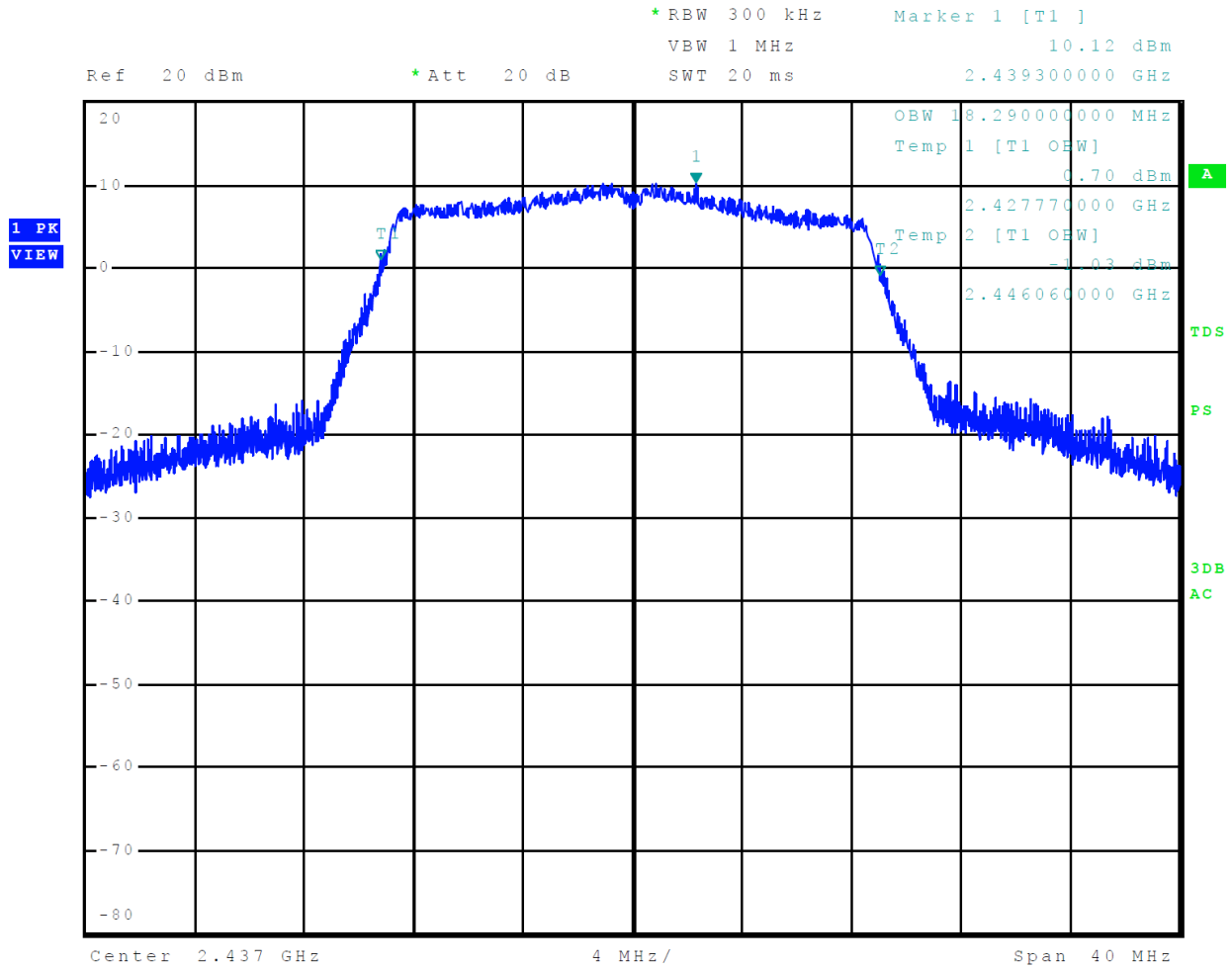
Figure 34 Plot of 99% Occupied Bandwidth Mode 7 802.11n
