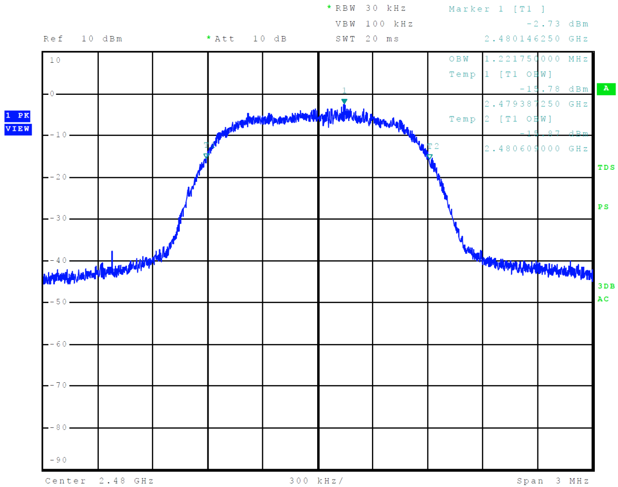
Figure 24 Plot of 99% Occupied Bandwidth Mode 2 BT 2EDR
