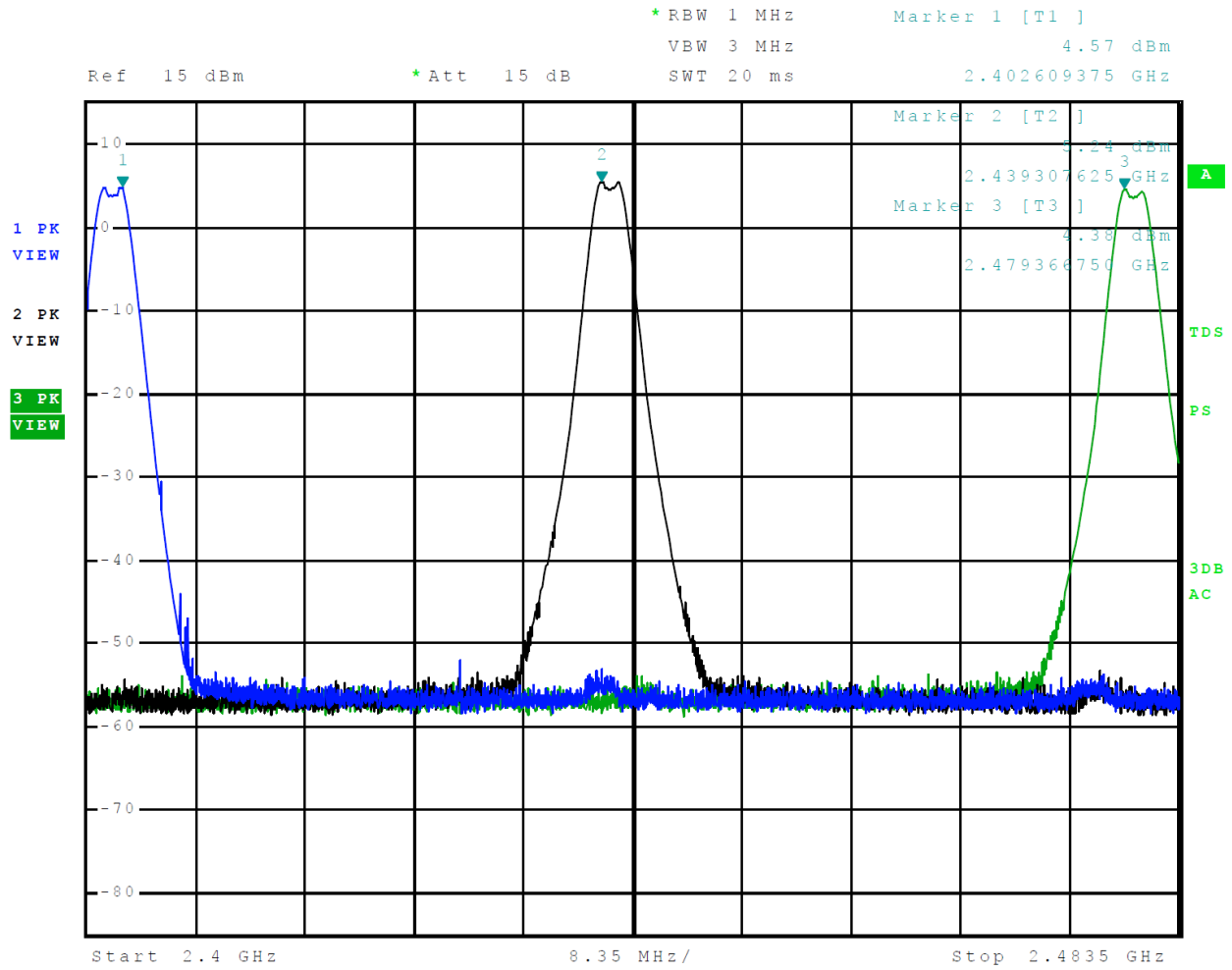
Figure 7 Plot of Transmitter Emissions Operation in 2402-2480 MHz Mode 4 BT BLE
