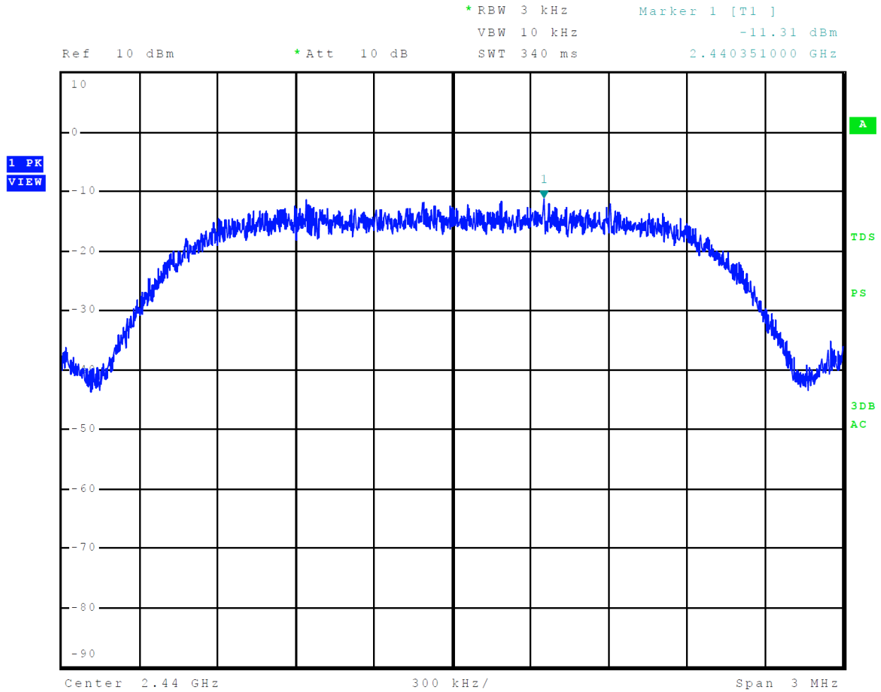
Figure 37 Plot of Transmitter Power Spectral Density Mode 4 BT BLE
