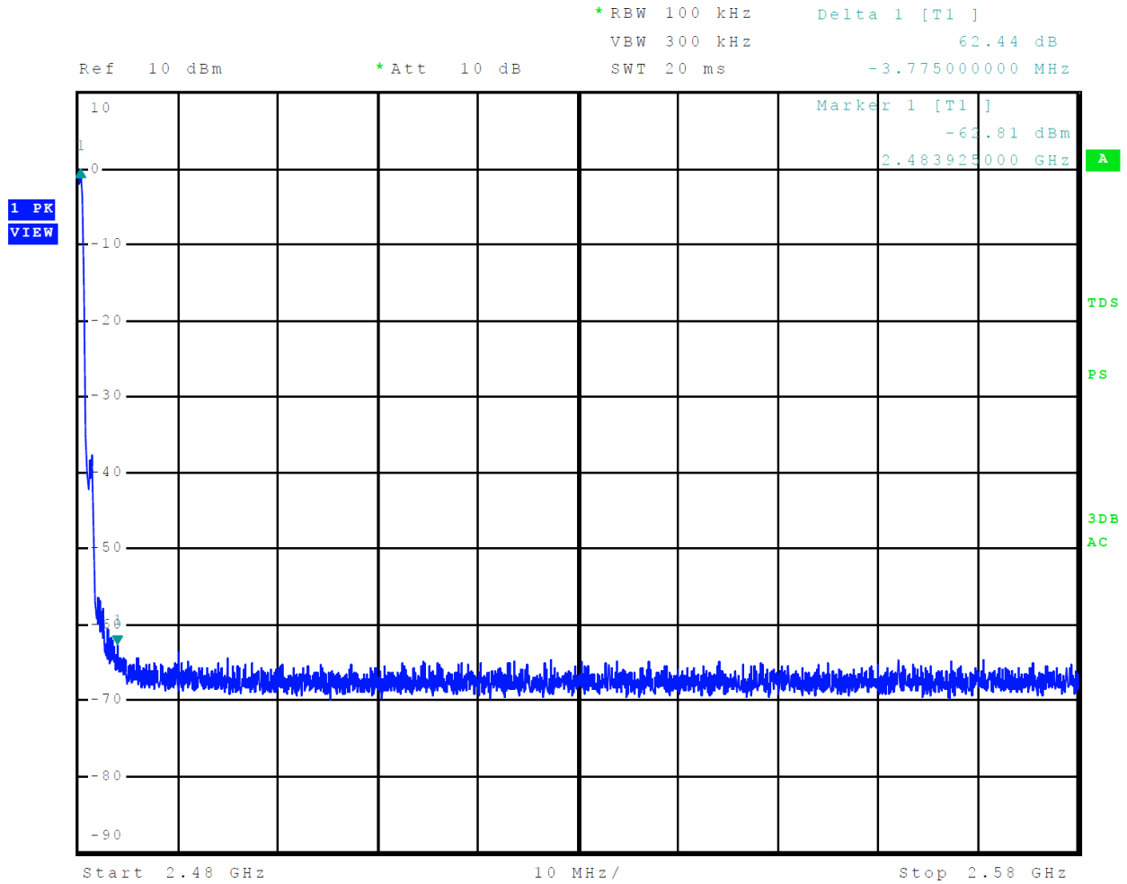
Figure 17 Plot of Transmitter Emissions High Band Edge Mode 2 BT 2EDR
