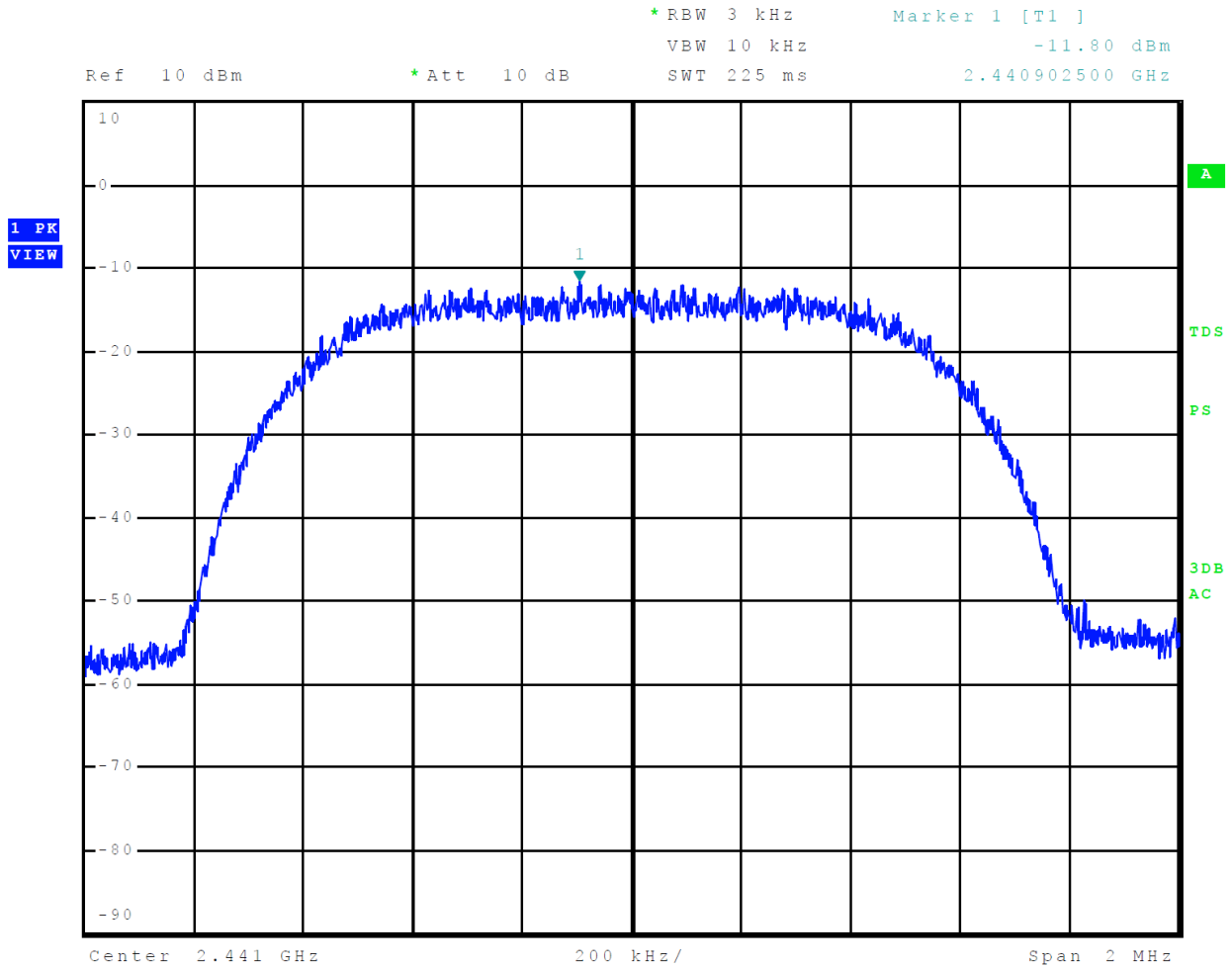
Figure 36 Plot of Transmitter Power Spectral Density Mode 3 BT 3EDR
