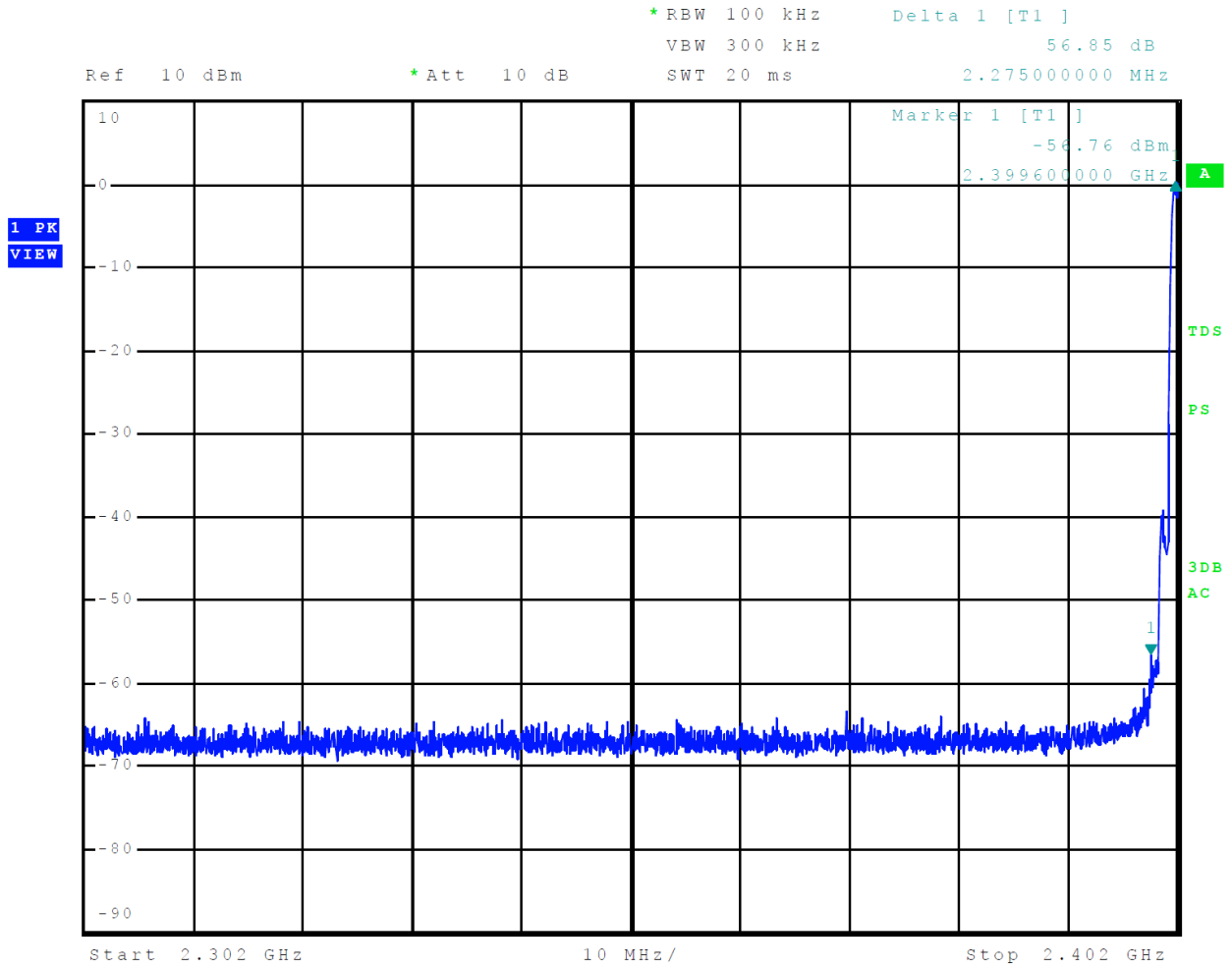
Figure 12 Plot of Transmitter Emissions Low Band Edge Mode 3 BT 3EDR
