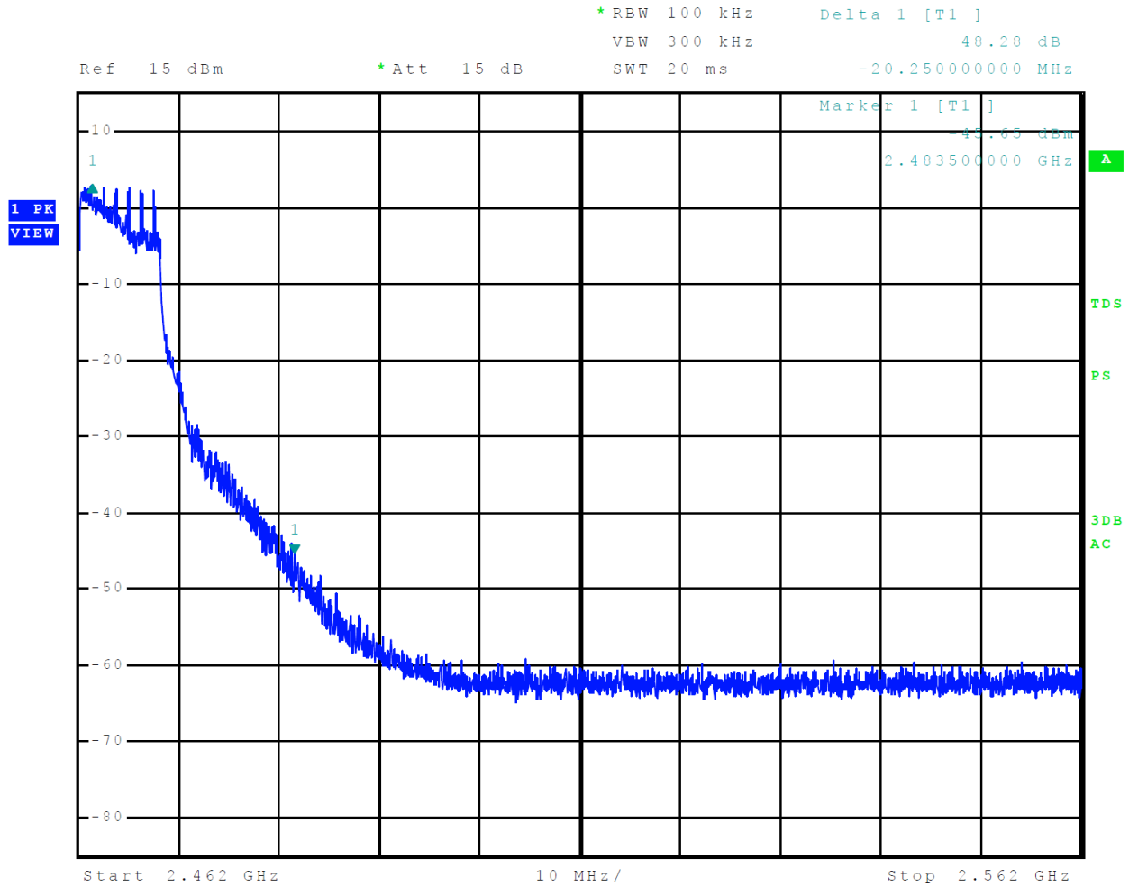
Figure 21 Plot of Transmitter Emissions High Band Edge Mode 6 802.11g
