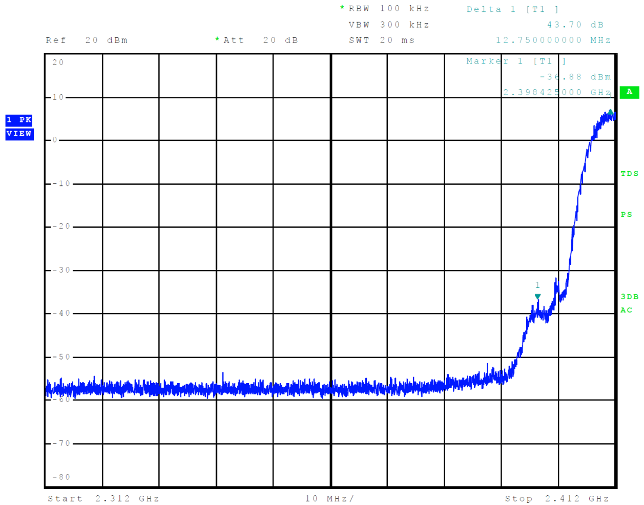
Figure 14 Plot of Transmitter Emissions Low Band Edge Mode 5 802.11b
