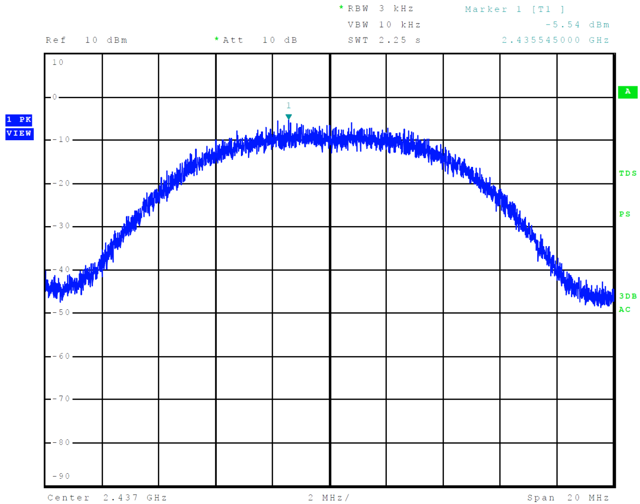
Figure 38 Plot of Transmitter Power Spectral Density Mode 5 802.11b
