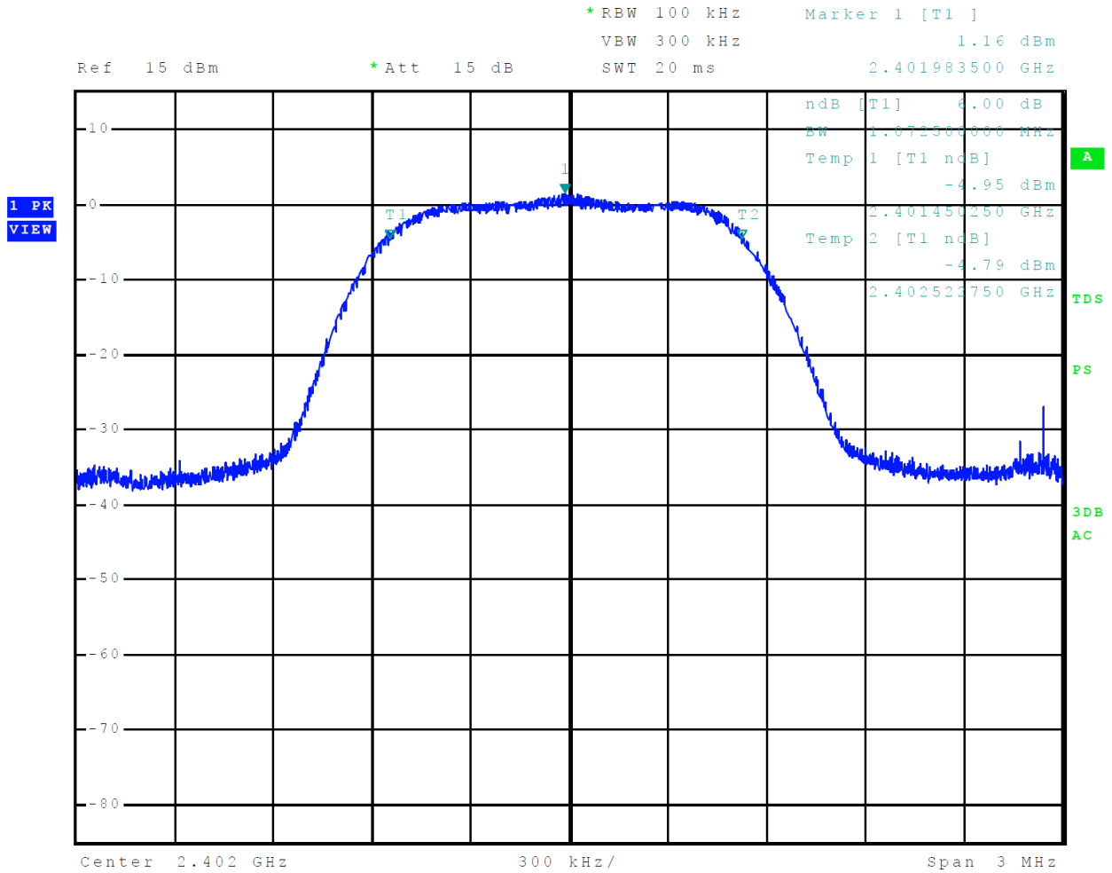
Figure 25 Plot of 6-dB Occupied Bandwidth Mode 3 BT 3EDR
