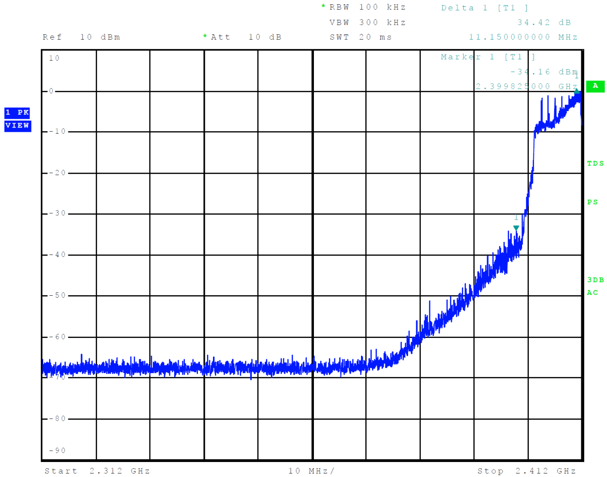
Figure 16 Plot of Transmitter Emissions Low Band Edge Mode 7 802.11n
