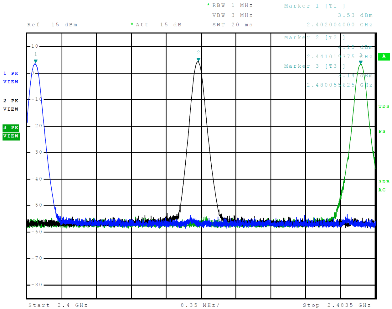
Figure 6 Plot of Transmitter Emissions Operation in 2402-2480 MHz Mode 3 BT 3EDR
