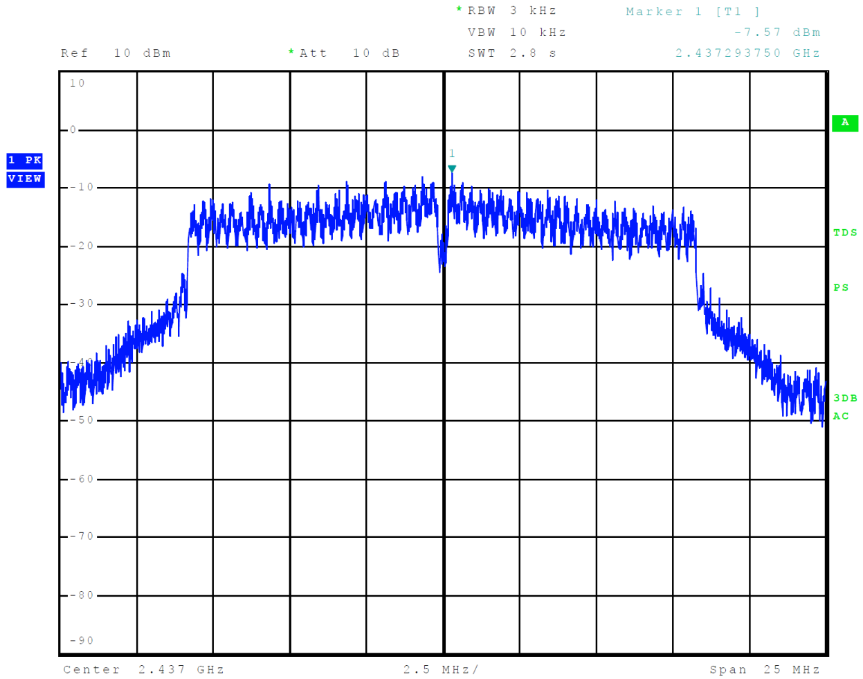
Figure 39 Plot of Transmitter Power Spectral Density Mode 6 802.11g
