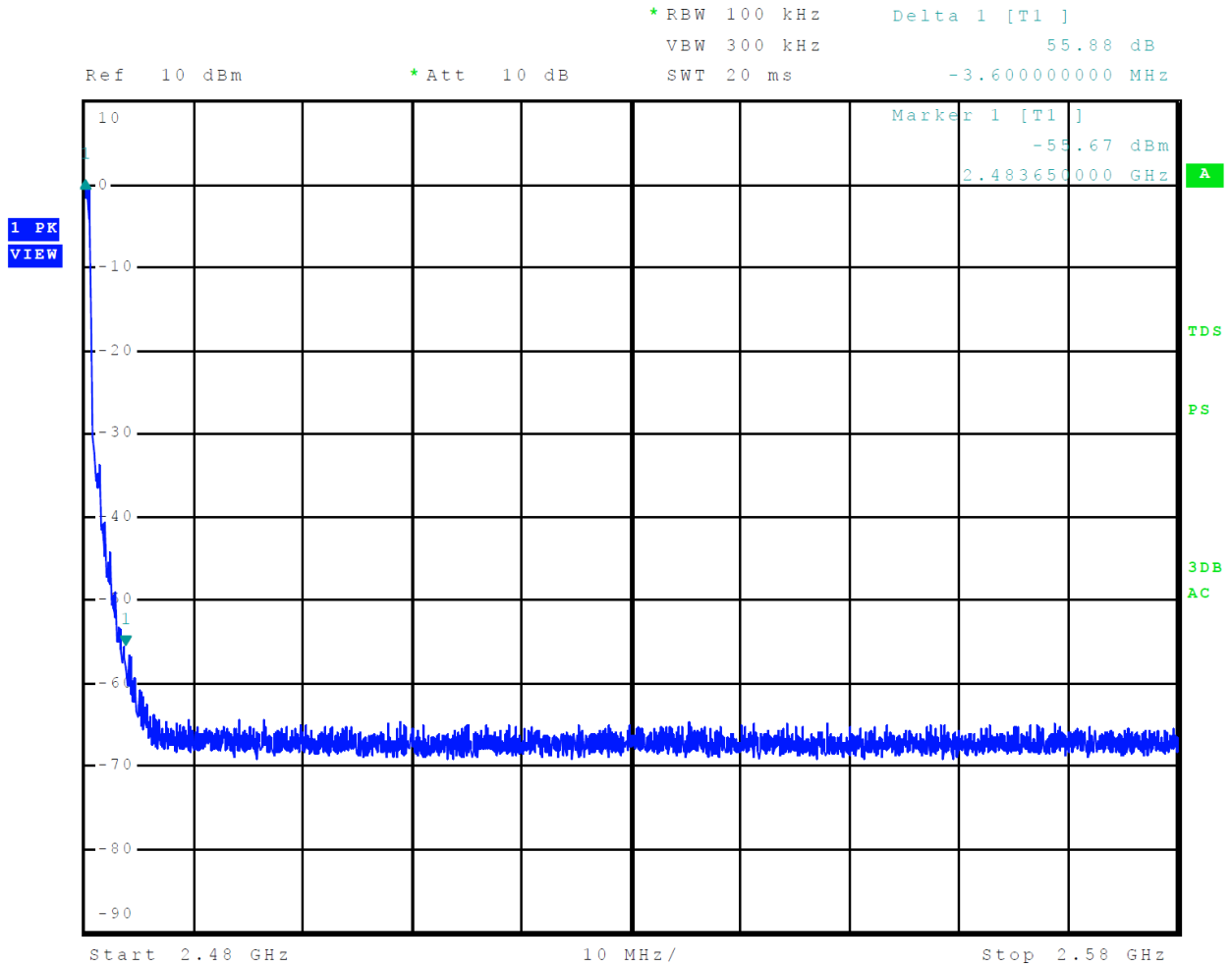
Figure 18 Plot of Transmitter Emissions High Band Edge Mode 3 BR 3EDR
