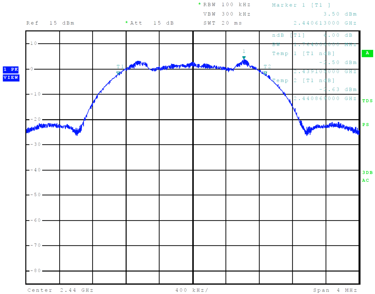
Figure 27 Plot of 6-dB Occupied Bandwidth Mode 4 BT BLE
