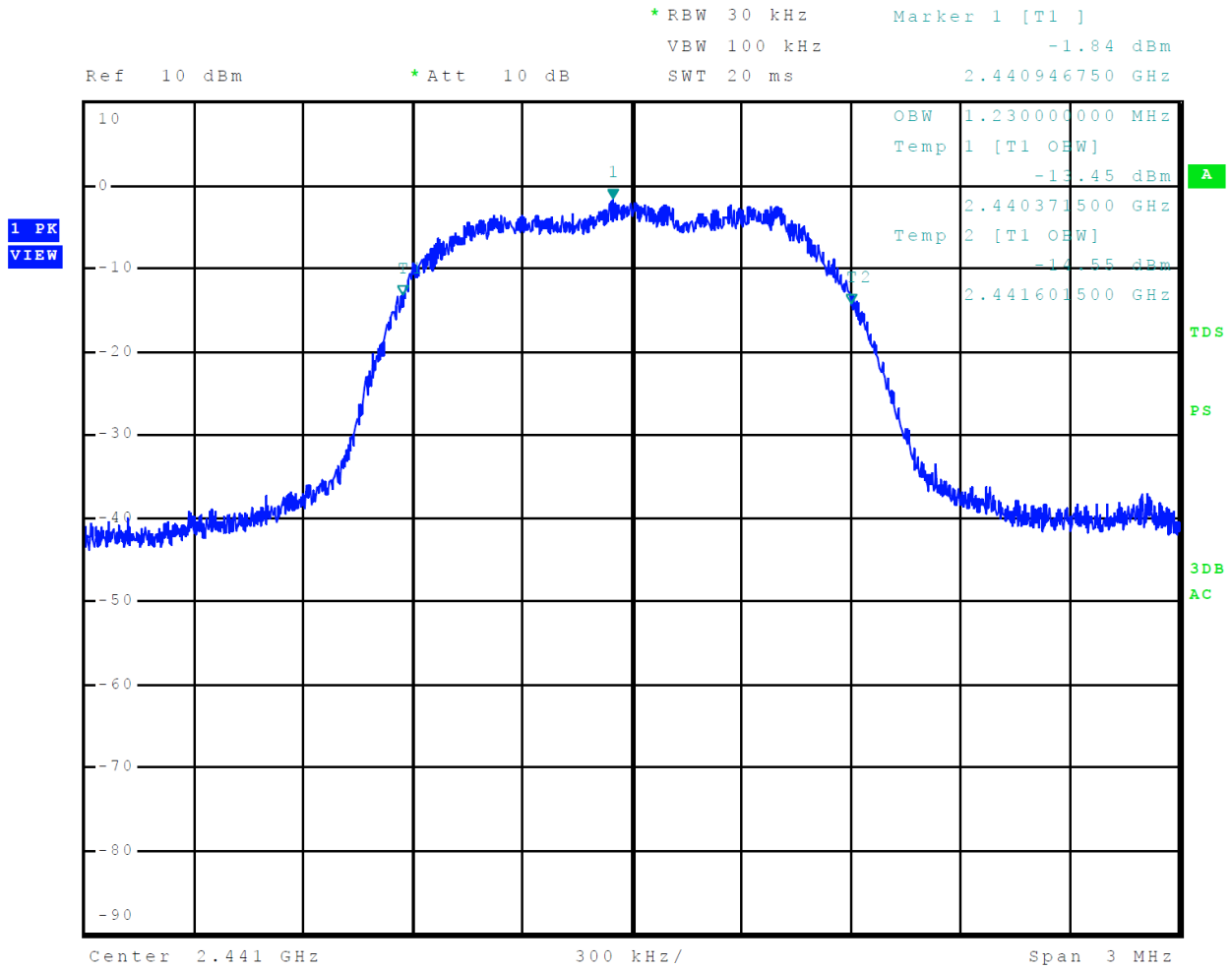
Figure 26 Plot of 99% Occupied Bandwidth Mode 3 BT 3EDR
