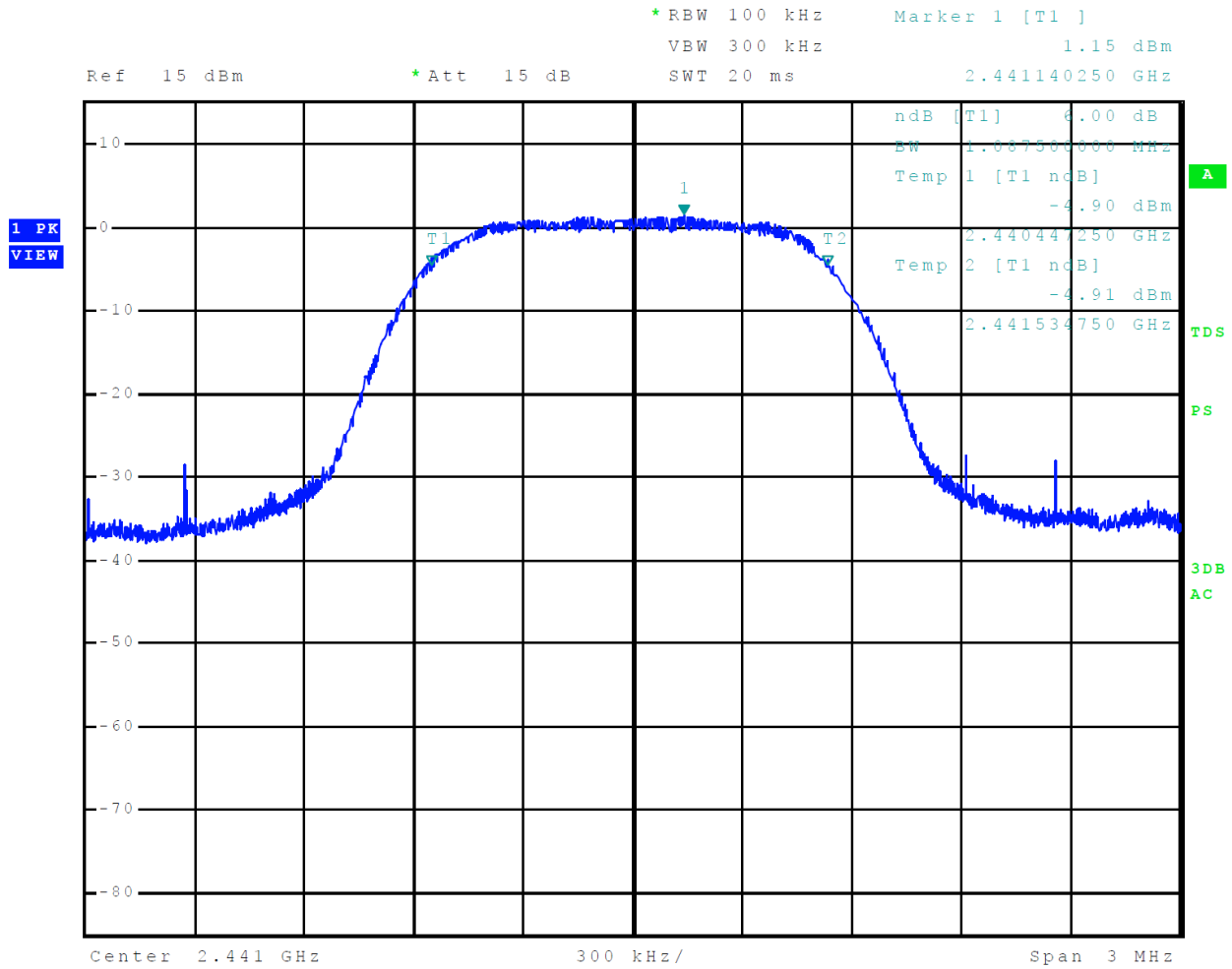
Figure 23 Plot of 6-dB Occupied Bandwidth Mode 2 BT 2EDR
