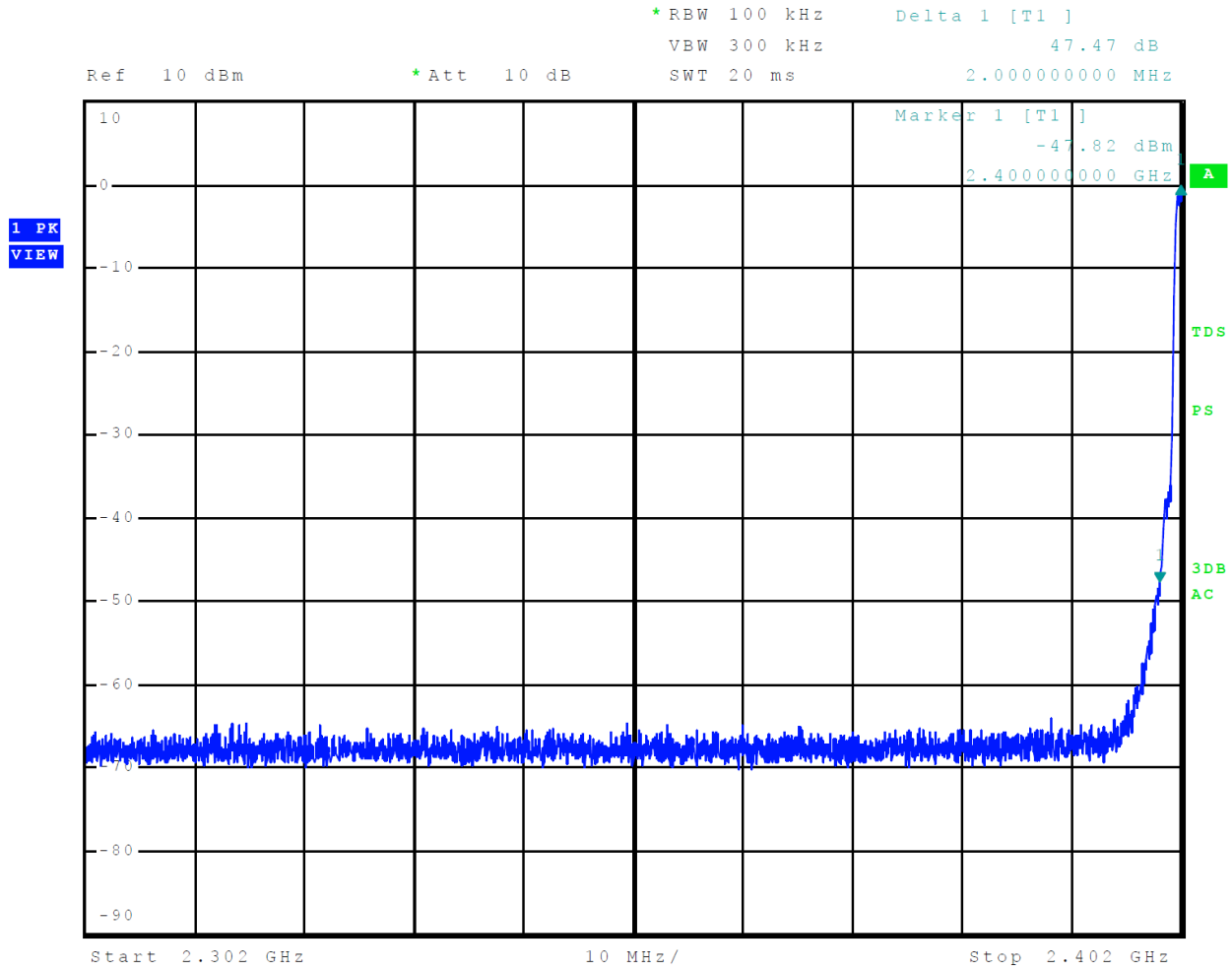
Figure 11 Plot of Transmitter Emissions Low Band Edge Mode 2 BT 2EDR
