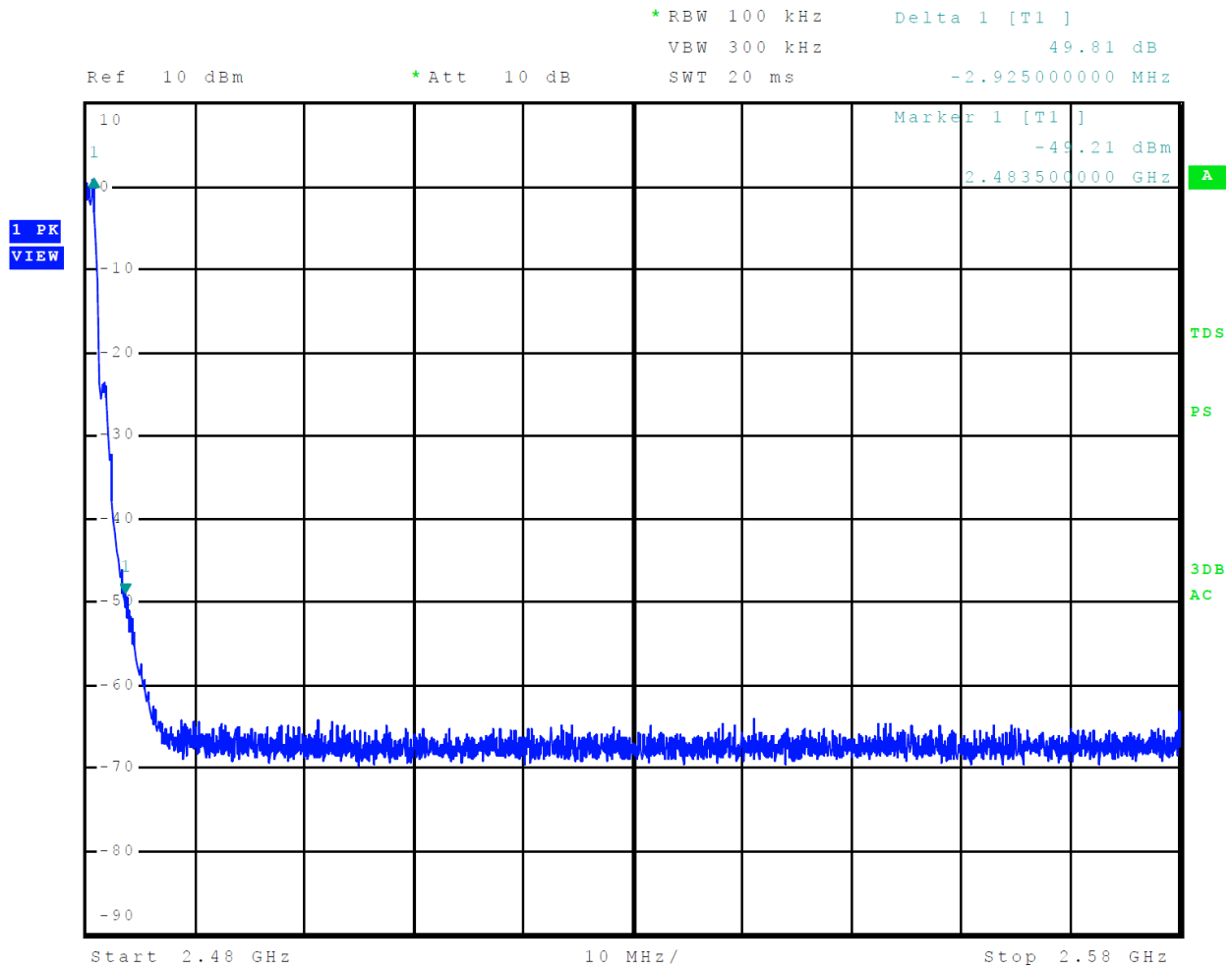
Figure 19 Plot of Transmitter Emissions High Band Edge Mode 4 BT BLE
