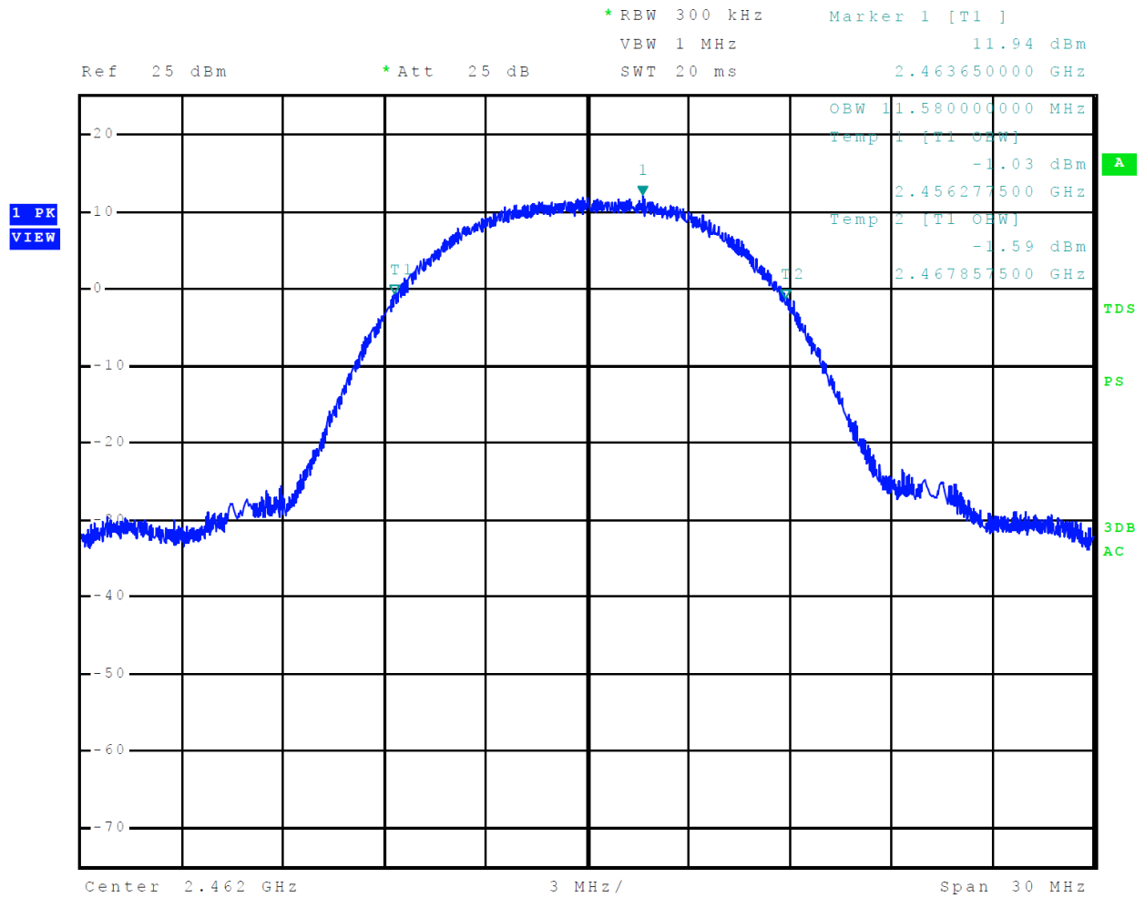
Figure 30 Plot of 99% Occupied Bandwidth Mode 5 802.11b
