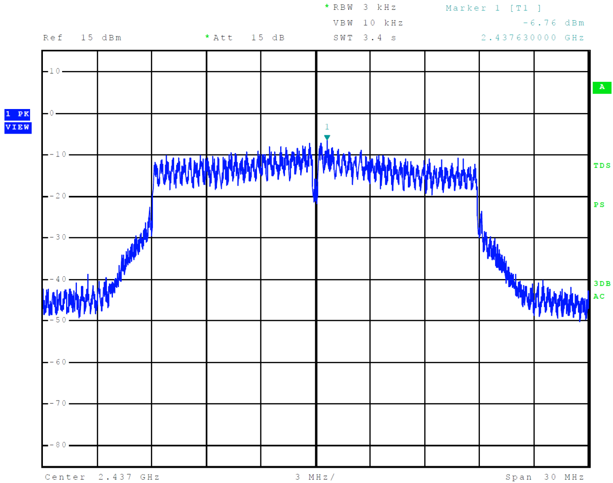
Figure 40 Plot of Transmitter Power Spectral Density Mode 7 802.11n
