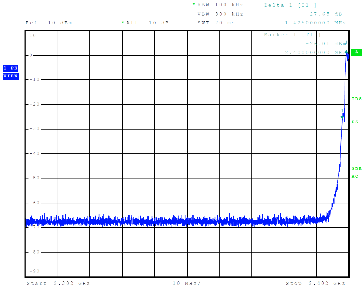
Figure 13 Plot of Transmitter Emissions Low Band Edge Mode 4 BT BLE
