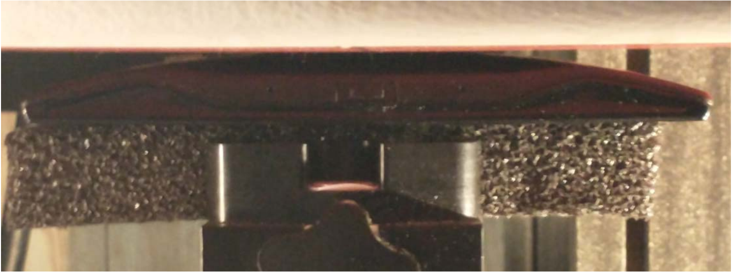
Figure C.2 – Setup Photo, Back Touch –Close
