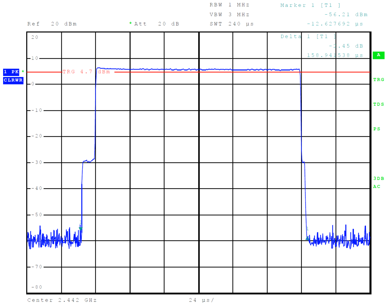
Figure 13 Plot of Dwell time On Channel Mode 1 BT BR
