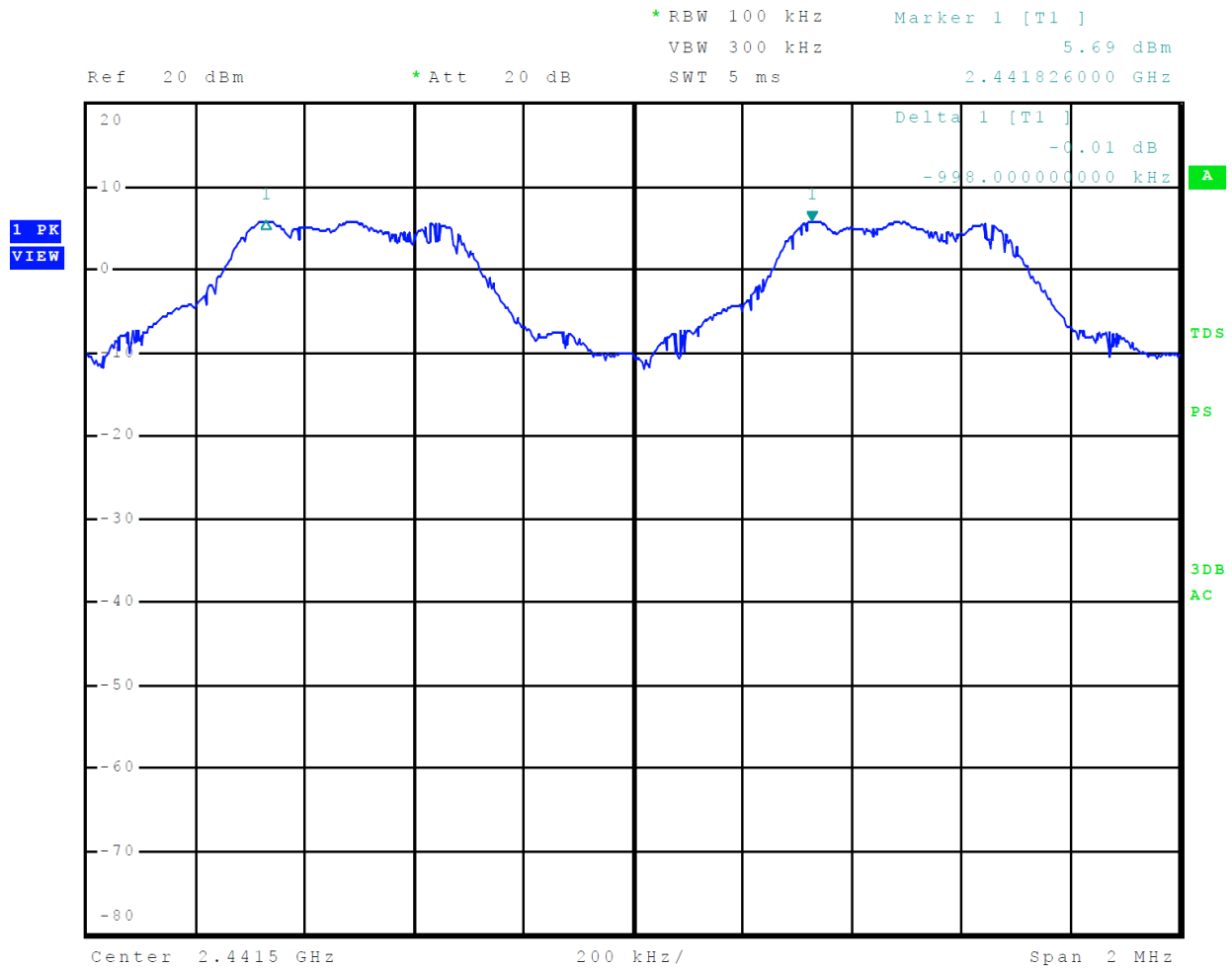
Figure 12 Plot of Channel Separation Mode 1 BT BR
