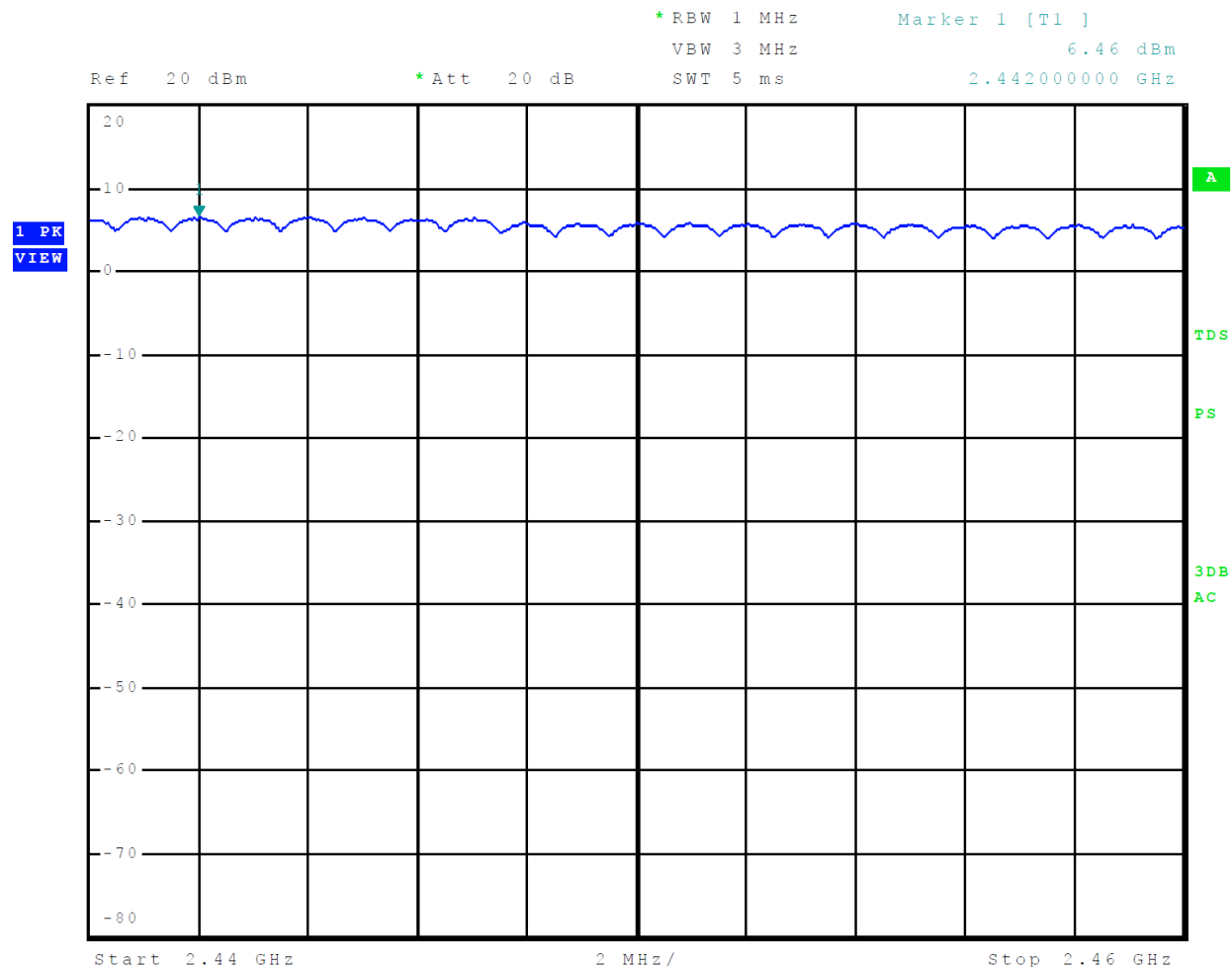
Figure 10 Plot of Number of Hopping Channels Mode 1 BT BR
