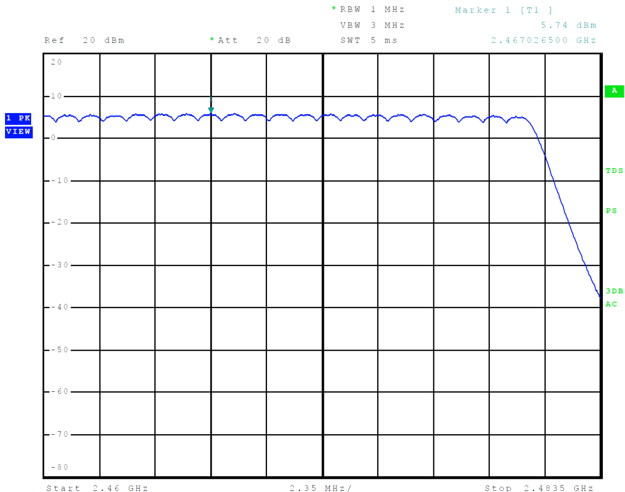
Figure 11 Plot of Number of Hopping Channels Mode 1 BT BR
