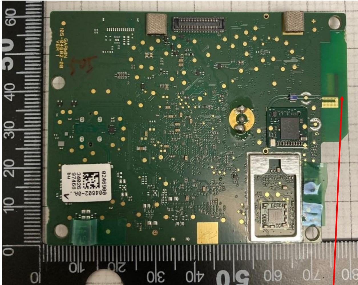
Planar Inverted F Antenna (PIFA)
