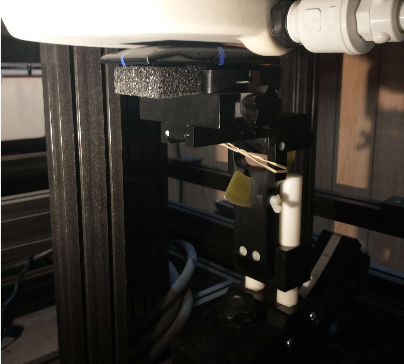
Figure C.5 – Setup Photo, Back Touch -Far – Twin Sam
