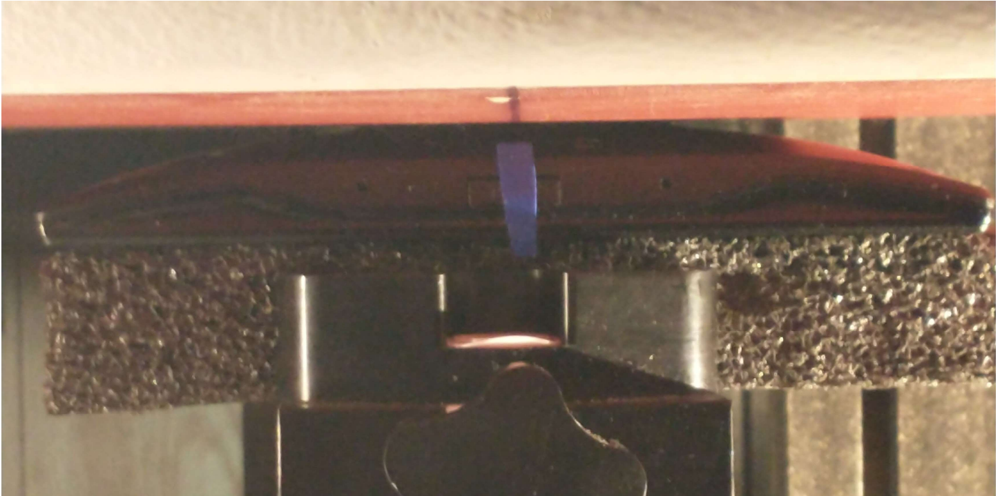
Figure C.2 – Setup Photo, Back Touch –Close - ELI
