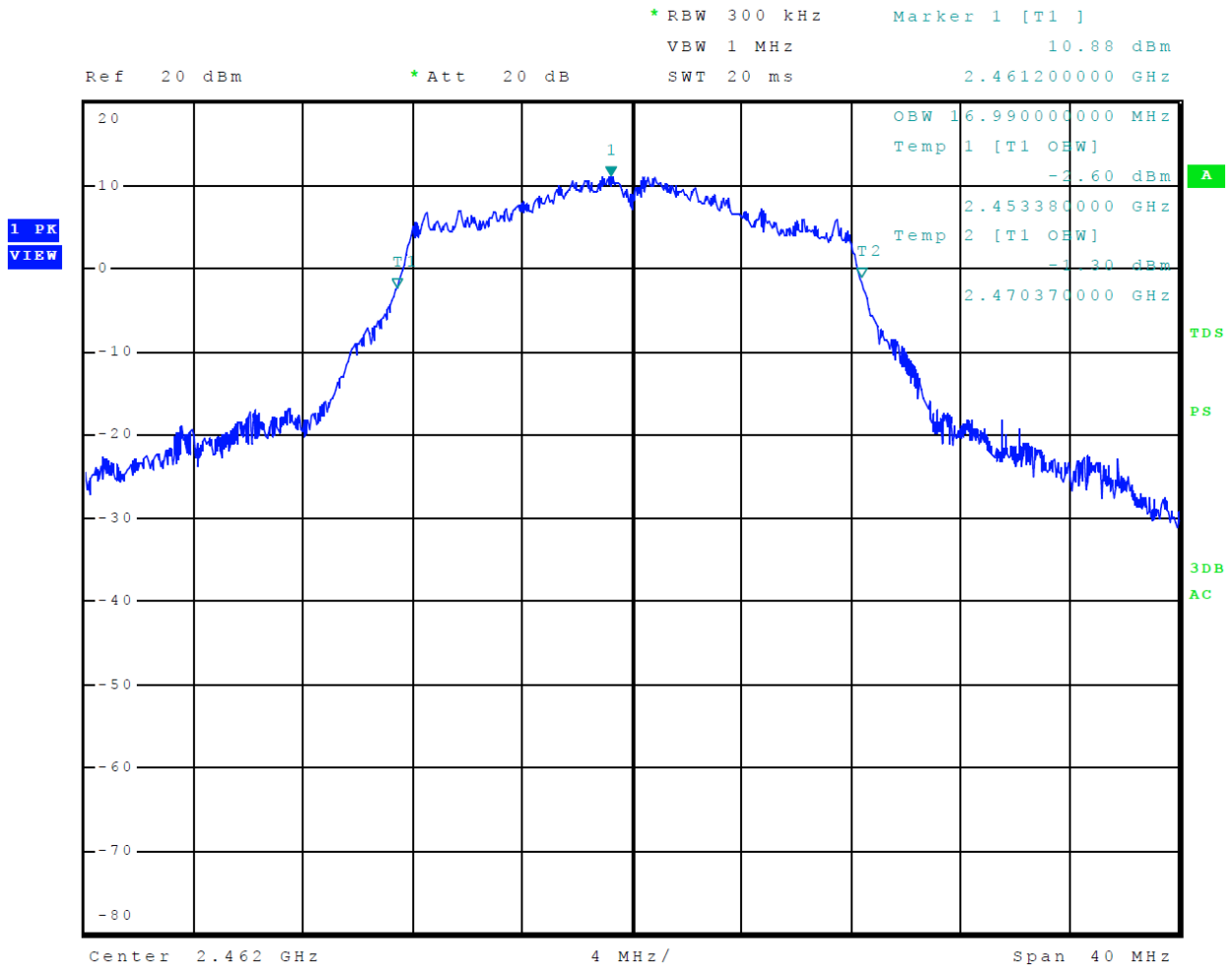
Figure 32 Plot of 99% Occupied Bandwidth Mode 6 802.11g
