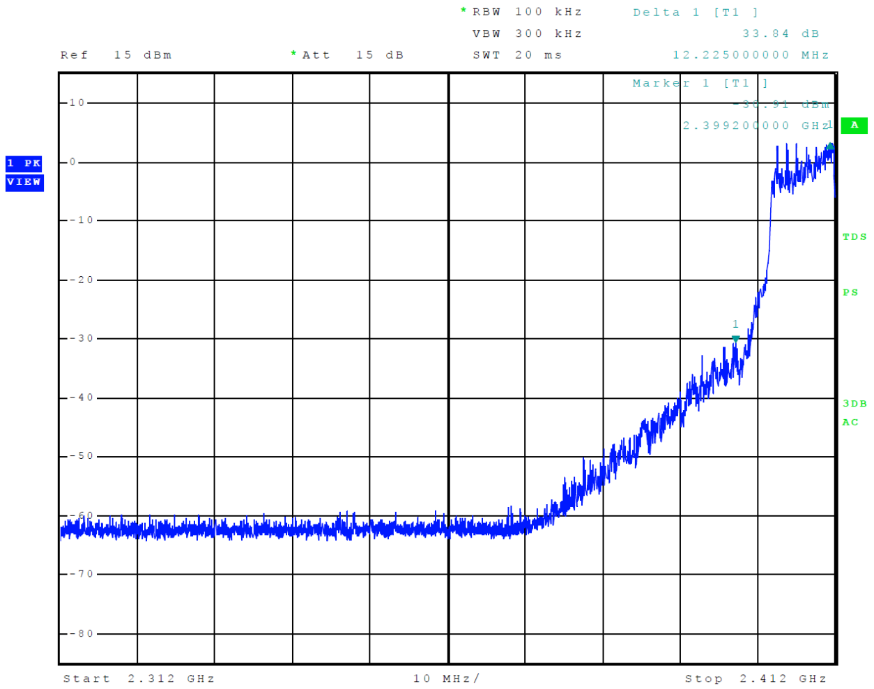
Figure 15 Plot of Transmitter Emissions Low Band Edge Mode 6 802.11g
