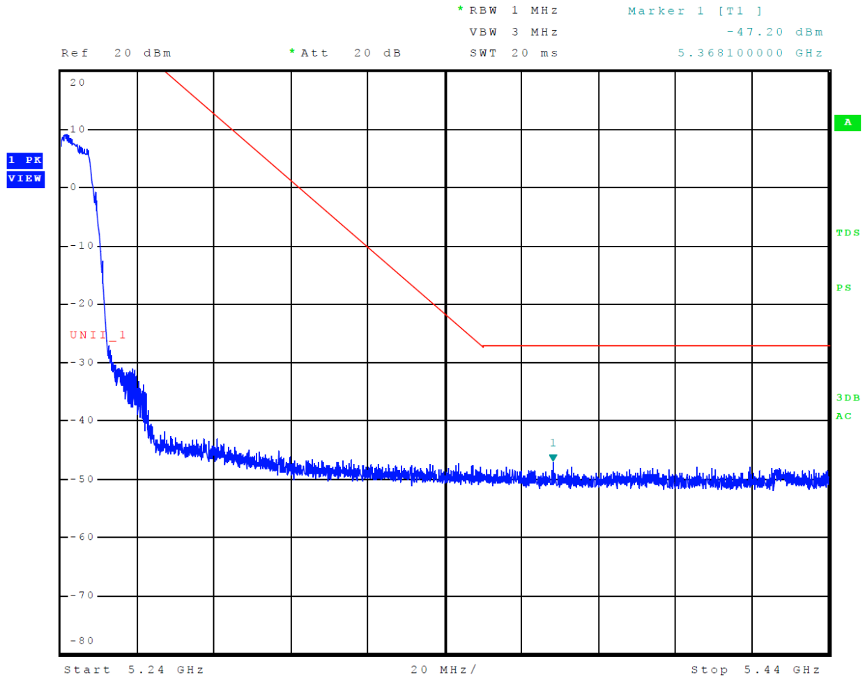
Figure 13 Plot of Upper Band Edge Across 5150-5250 MHz Mode 8 U-NII-1 (802.11a)
