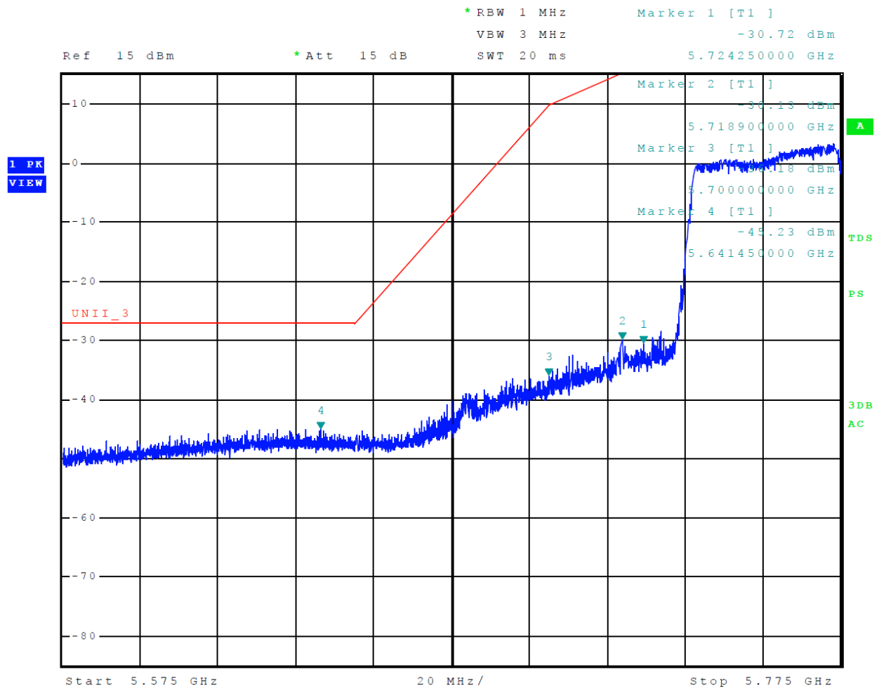
Figure 32 Plot of Lower Band Edge Across 5725-5850 MHz Mode 15 U-NII-3 (802.11ac80)
