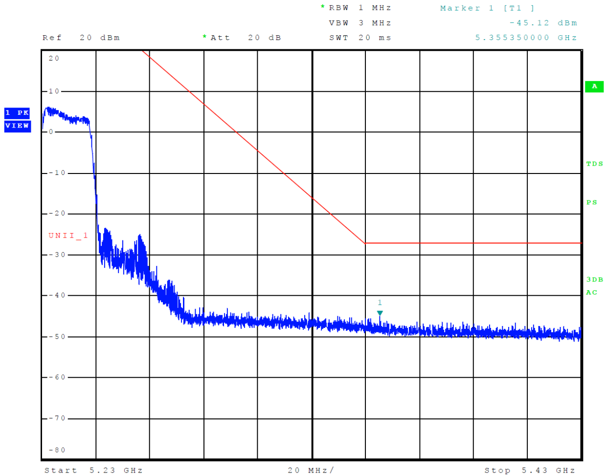
Figure 15 Plot of Upper Band Edge Across 5150-5250 MHz Mode 10 U-NII-1 (802.11n40)
