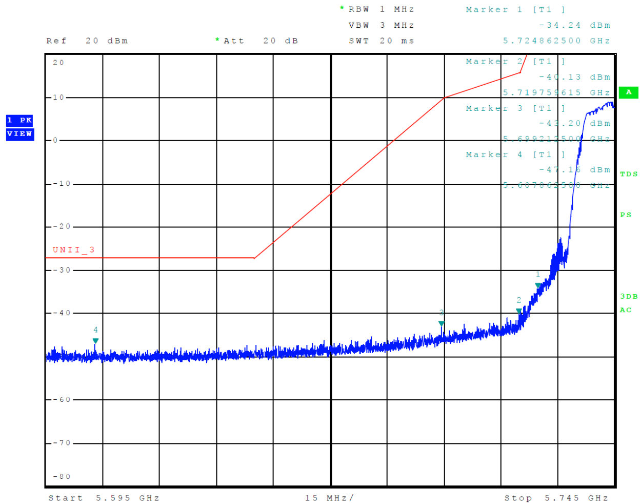
Figure 29 Plot of Lower Band Edge Across 5725-5850 MHz Mode 12 U-NII-3 (802.11a)
