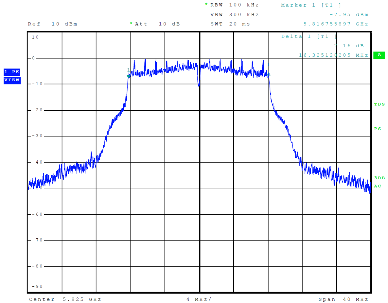
Figure 41 Plot of 6-dB Occupied Bandwidth 5725-5850 MHz Mode 12 U-NII-3 (802.11a)
