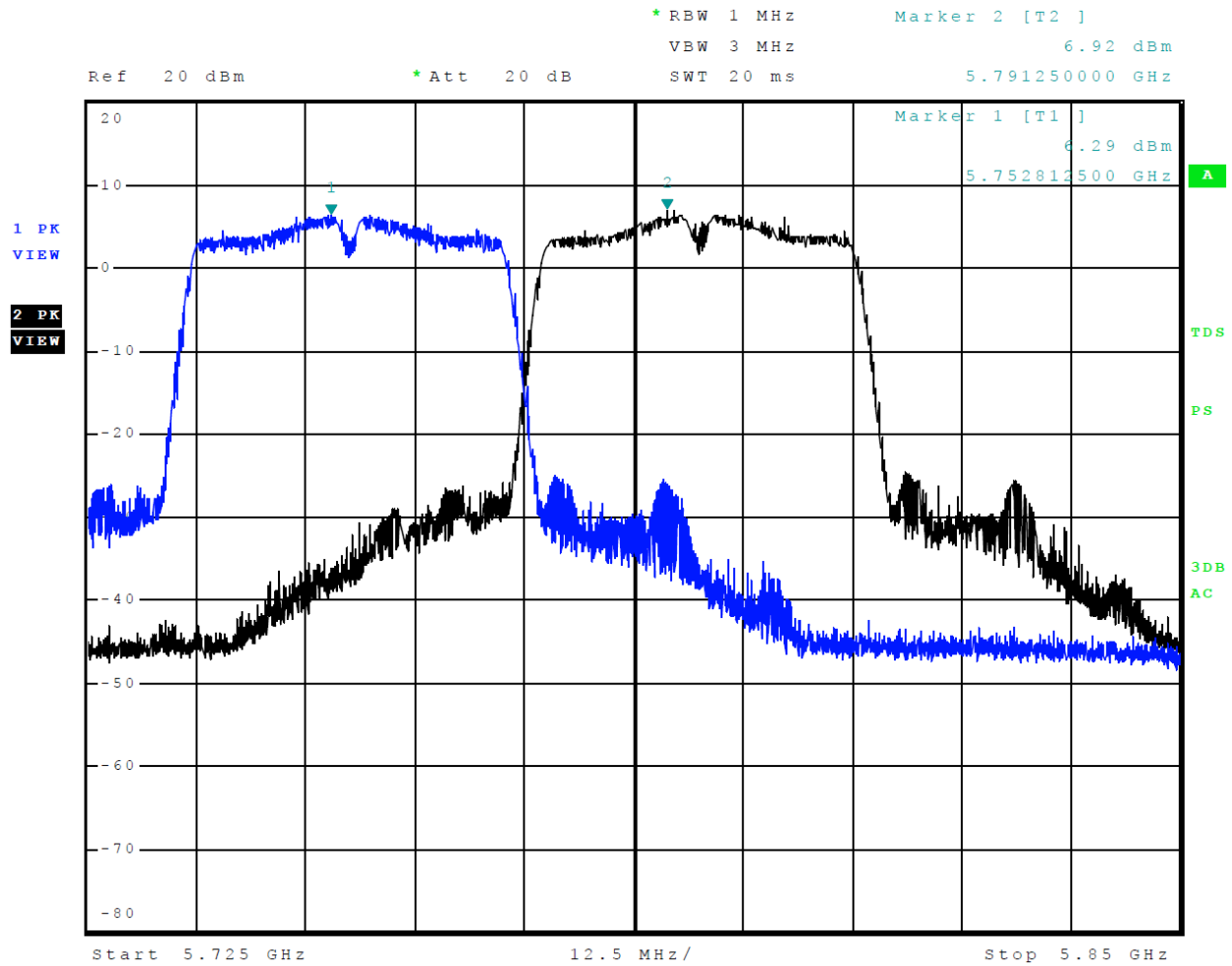
Figure 27 Plot of Transmitter Emissions Across 5725-5850 MHz Mode 14 U-NII-3 (802.11n40)
