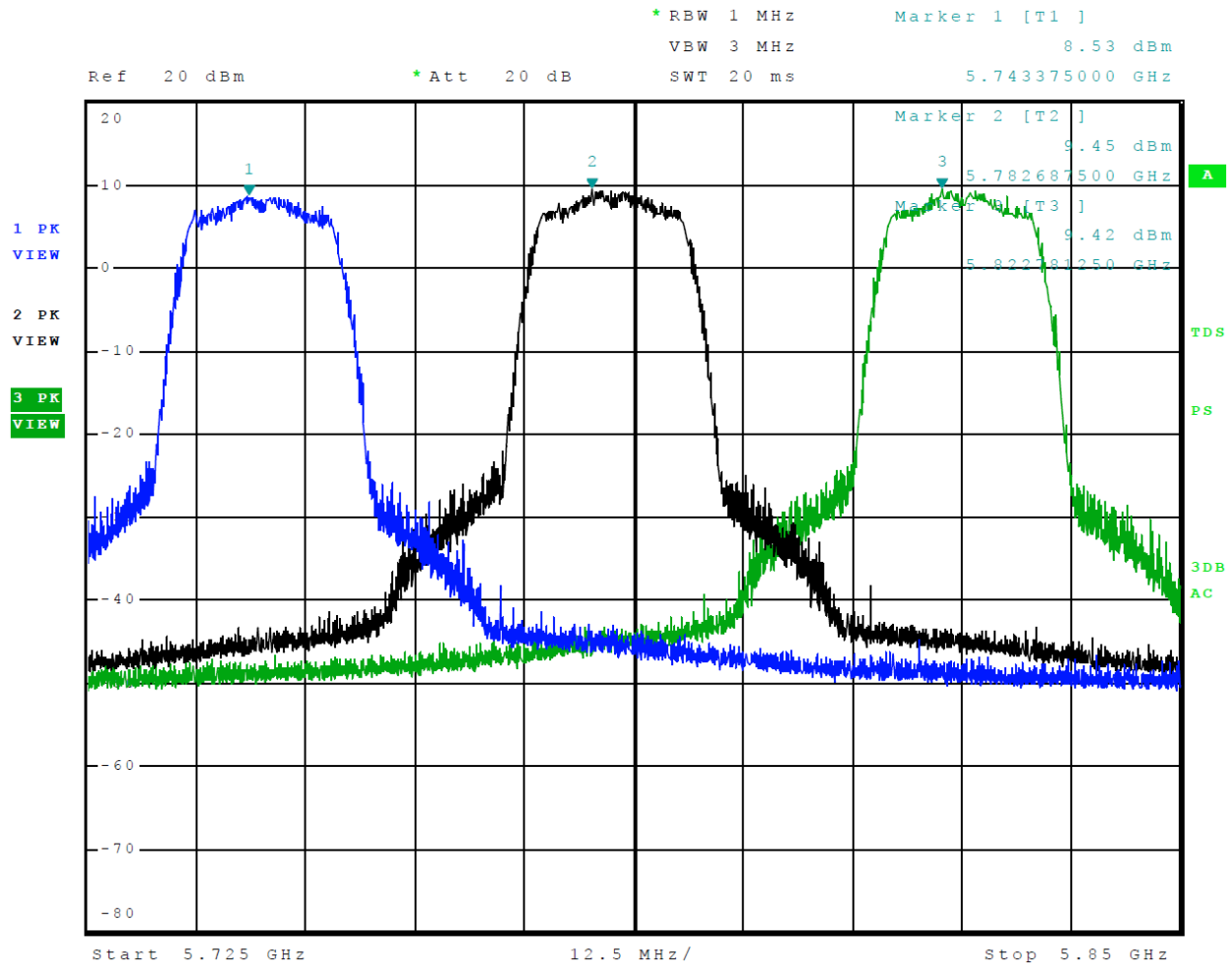
Figure 26 Plot of Transmitter Emissions Across 5725-5850 MHz Mode 13 U-NII-3 (802.11n)
