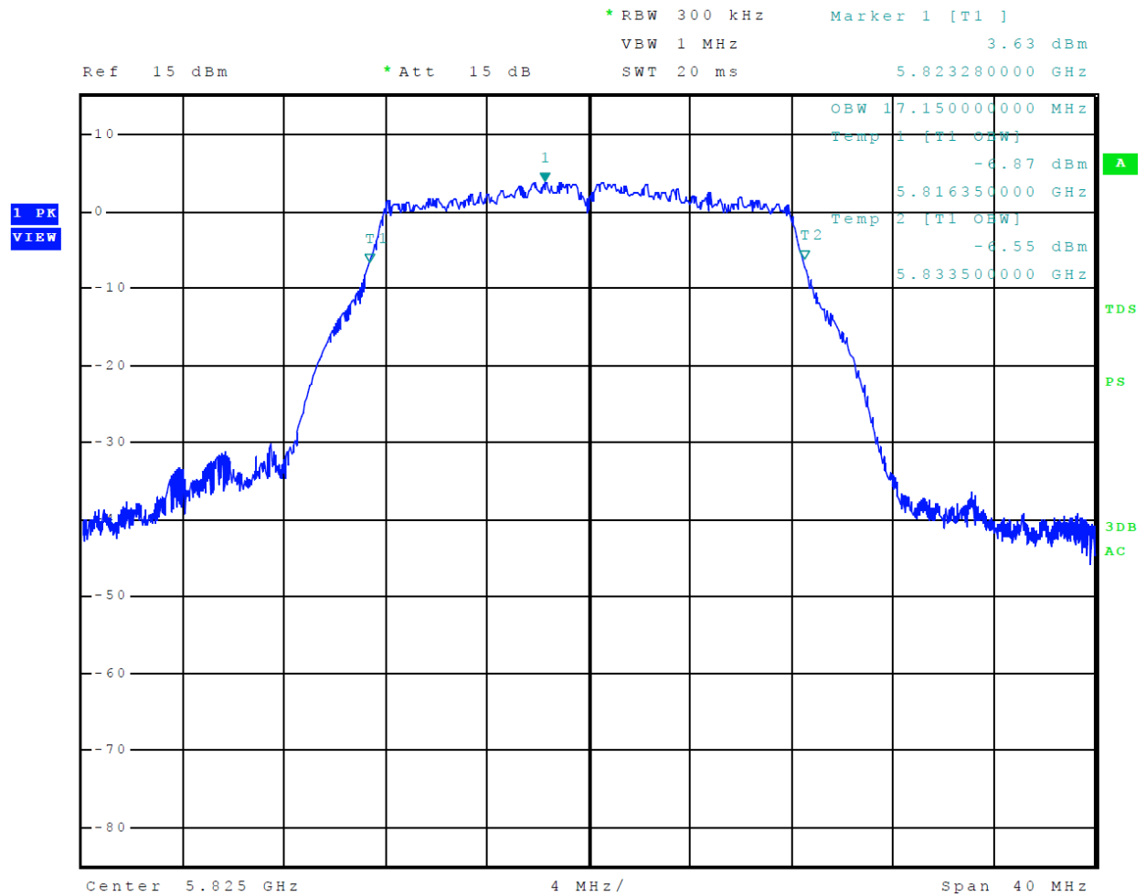
Figure 37 Plot of 99% Occupied Bandwidth 5725-5850 MHz Mode 12 U-NII-3 (802.11a)
