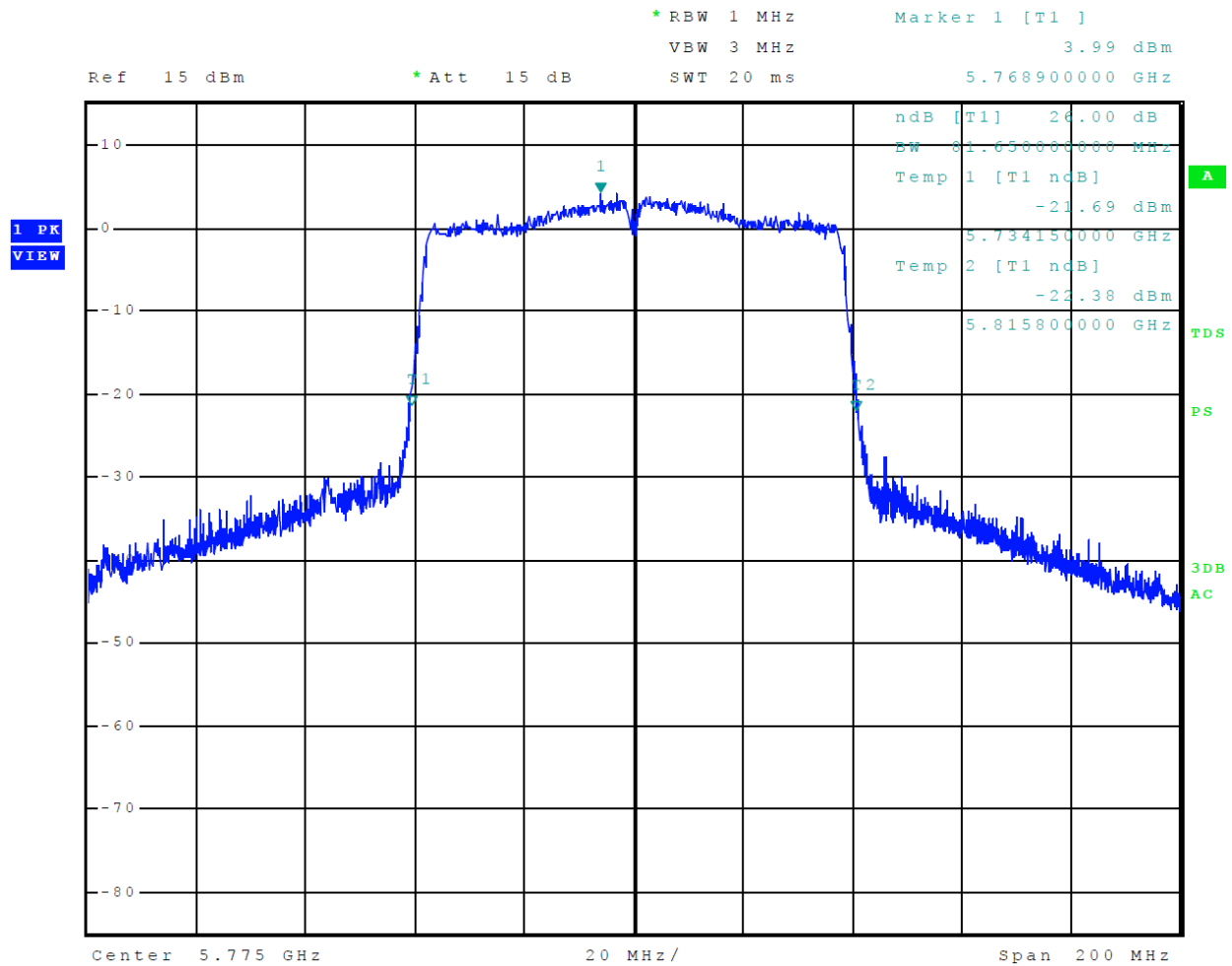
Figure 48 Plot of 26-dB Occupied Bandwidth 5725-5850 MHz Mode 15 U-NII-3 (802.11ac80)
