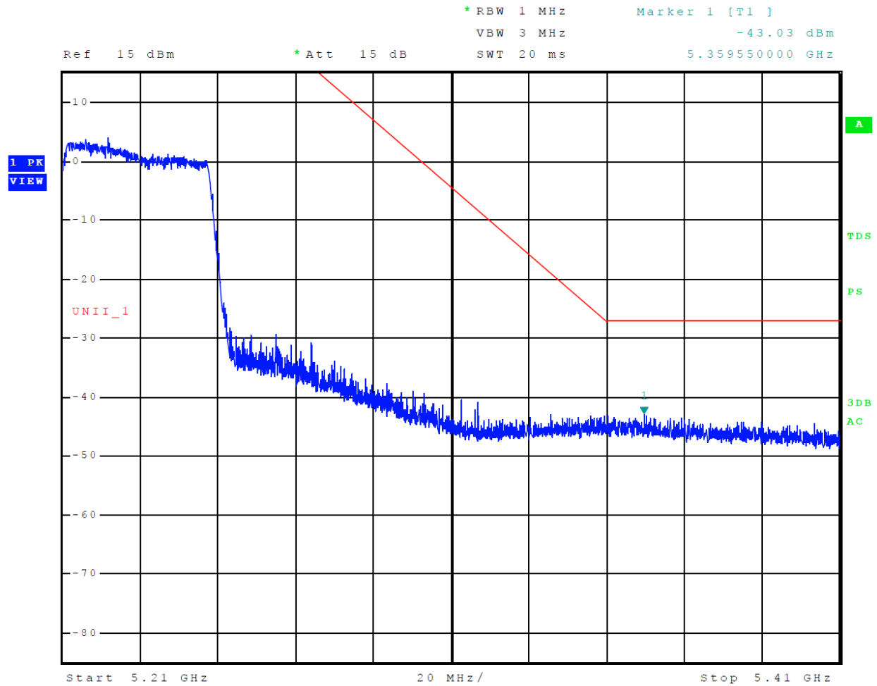
Figure 16 Plot of Upper Band Edge Across 5150-5250 MHz Mode 11 U-NII-1 (802.11ac80)
