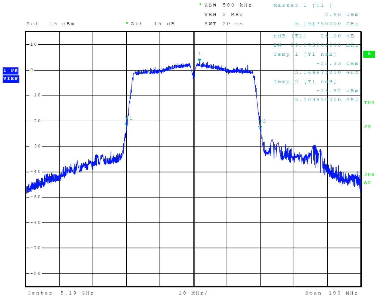
Figure 19 Plot of 26-dB Occupied Bandwidth 5150-5250 MHz Mode 10 U-NII-1 (802.11n40)
