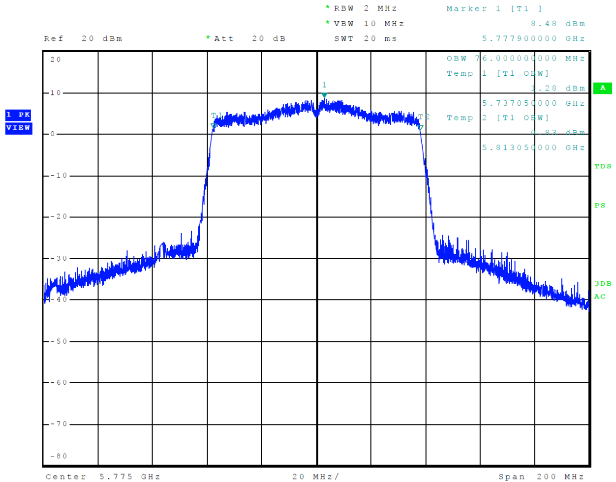
Figure 40 Plot of 99% Occupied Bandwidth 5725-5850 MHz Mode 15 U-NII-3 (802.11ac80)
