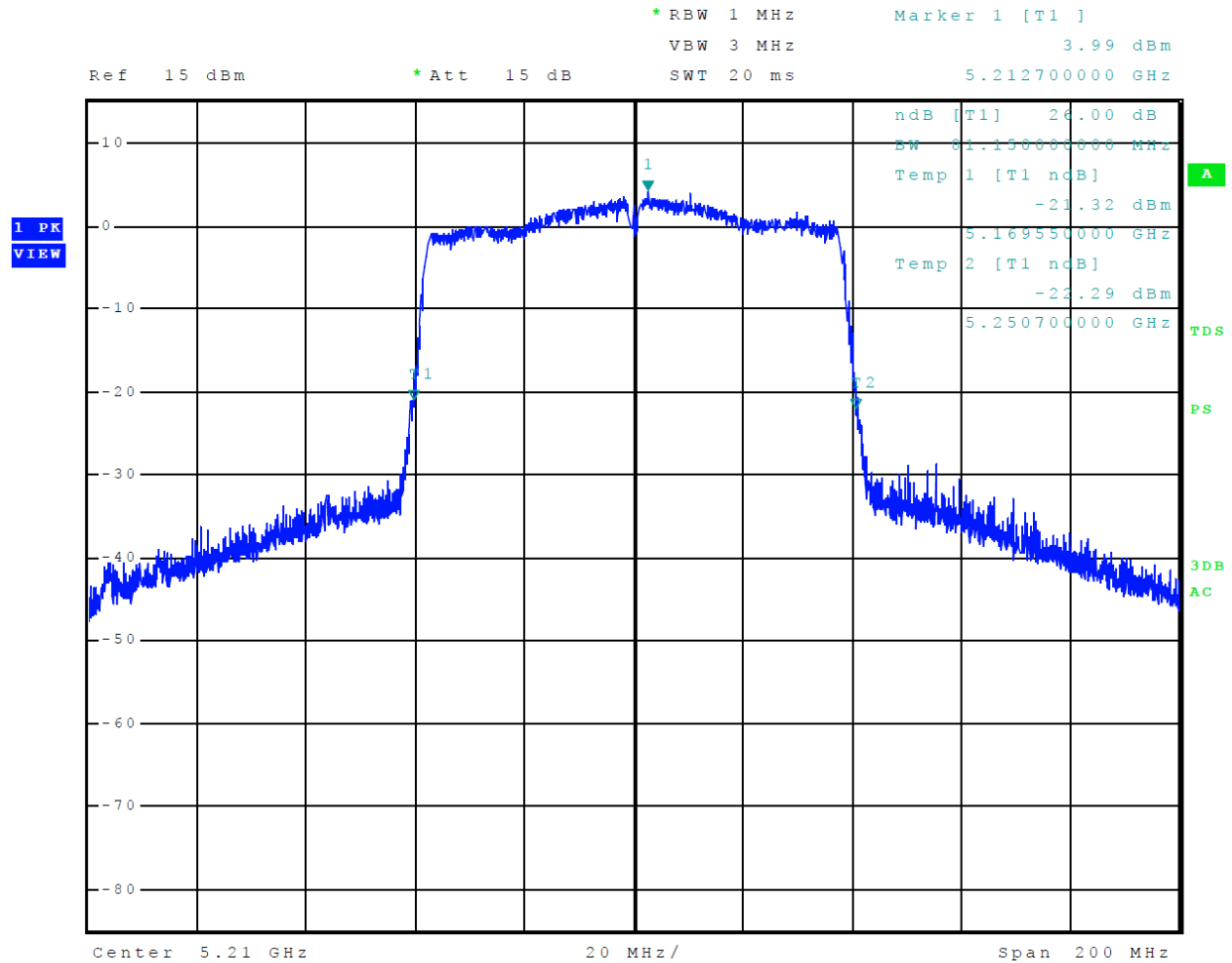
Figure 20 Plot of 26-dB Occupied Bandwidth 5150-5250 MHz Mode 11 U-NII-1 (802.11ac80)
