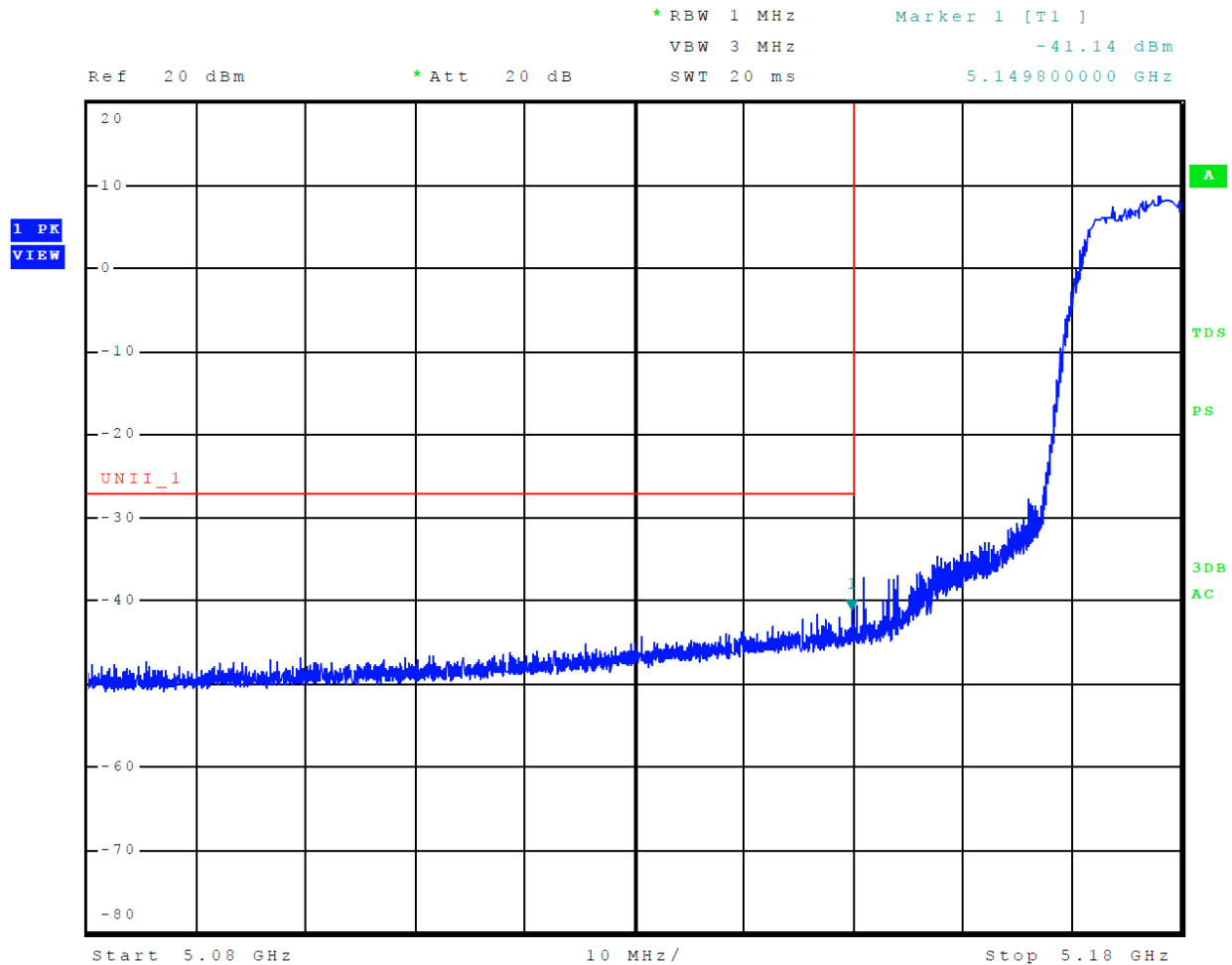
Figure 10 Plot of Lower Band Edge Across 5150-5250 MHz Mode 9 U-NII-1 (802.11n)
