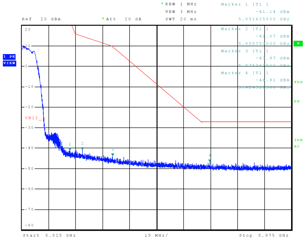
Figure 33 Plot of Upper Band Edge Across 5725-5850 MHz Mode 12 U-NII-3 (802.11a)
