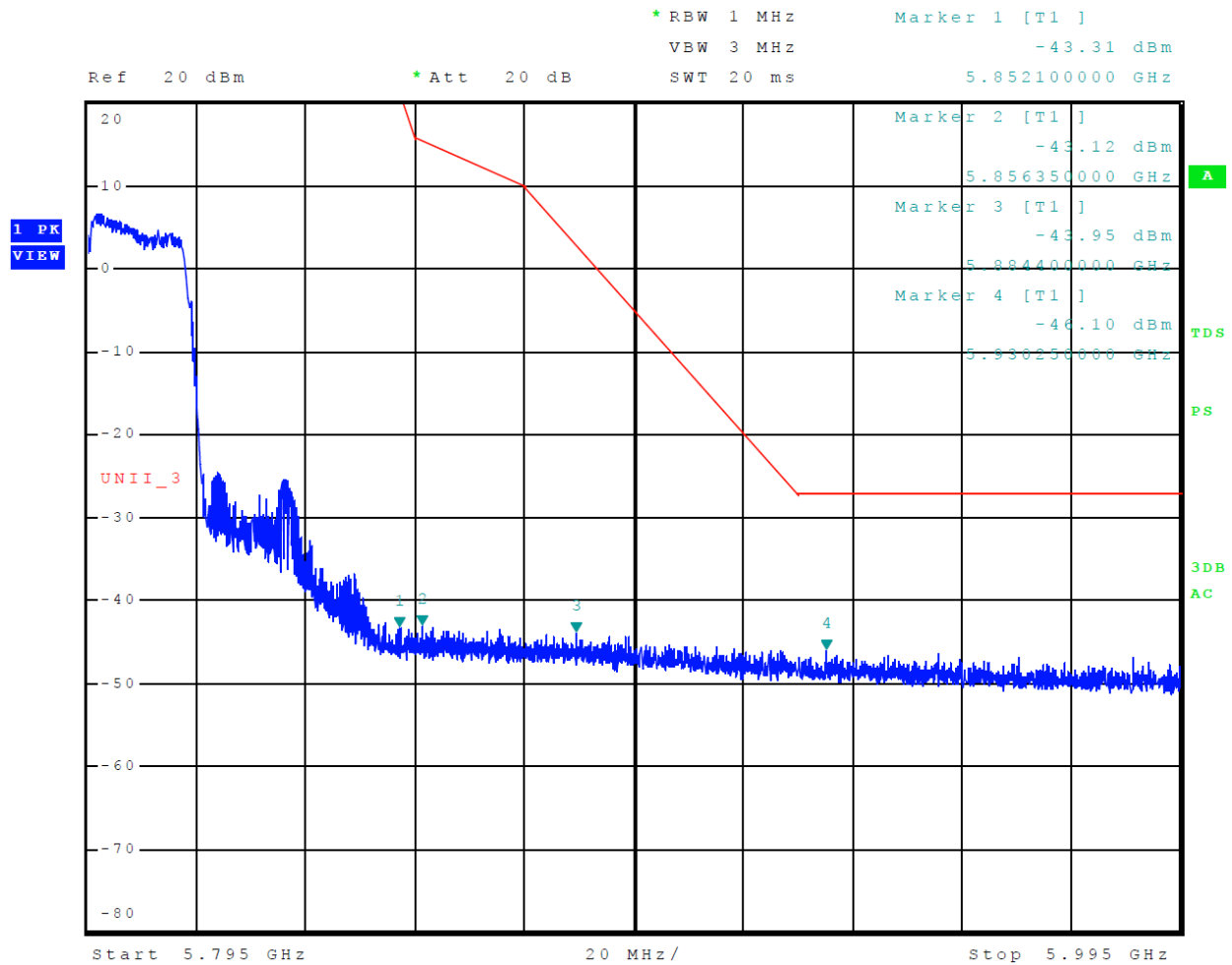
Figure 35 Plot of Upper Band Edge Across 5725-5850 MHz Mode 14 U-NII-3 (802.11n40)
