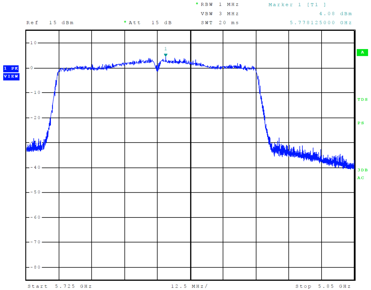
Figure 28 Plot of Transmitter Emissions Across 5725-5850 MHz Mode 15 U-NII-3 (802.11ac80)
