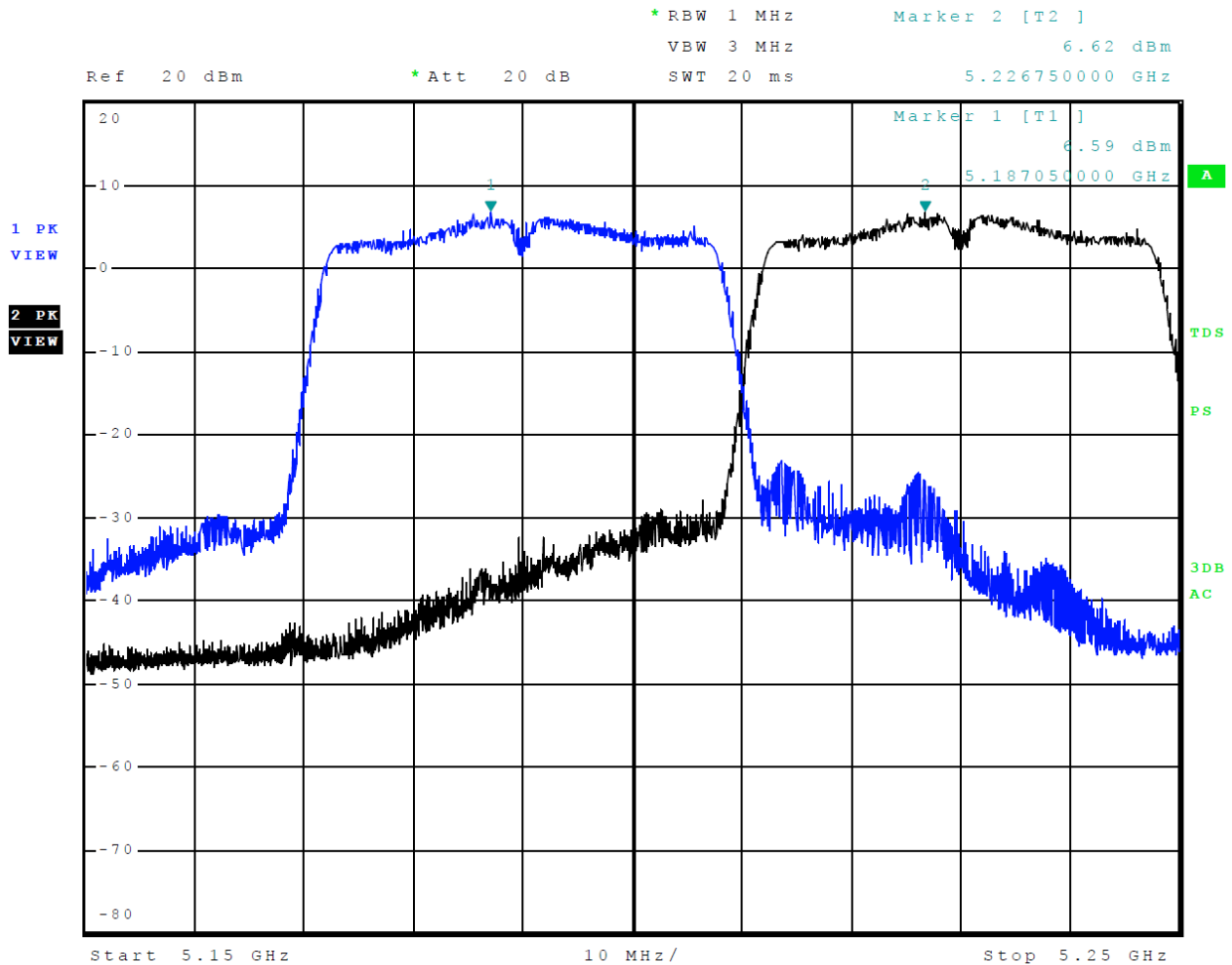
Figure 7 Plot of Transmitter Emissions Across 5150-5250 MHz Mode 10 U-NII-1 (802.11n40)
