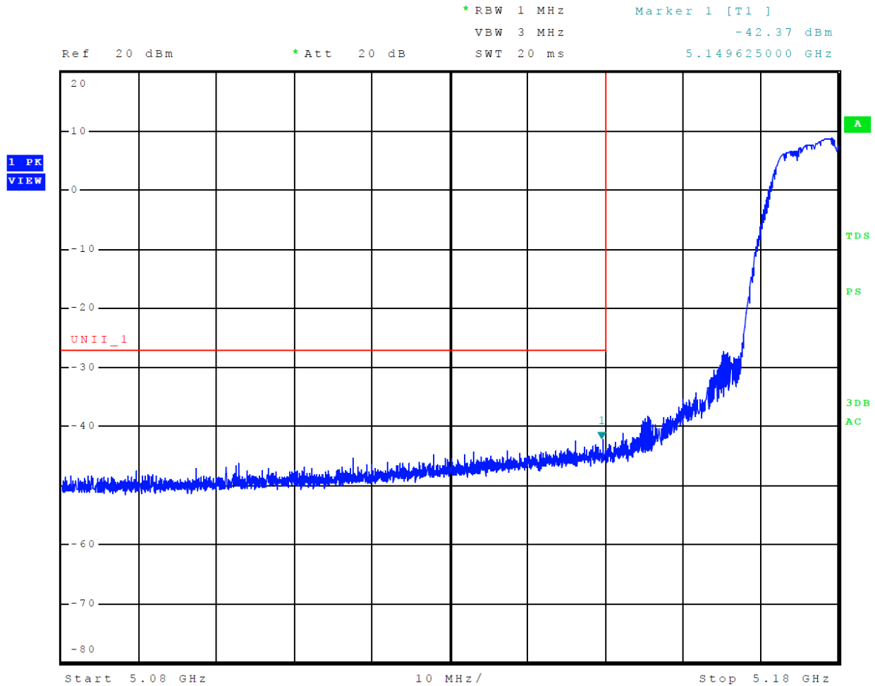
Figure 9 Plot of Lower Band Edge Across 5150-5250 MHz Mode 8 U-NII-1 (802.11a)
