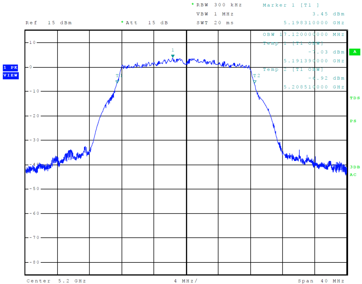
Figure 21 Plot of 99% Occupied Bandwidth 5150-5250 MHz Mode 8 U-NII-1 (802.11a)
