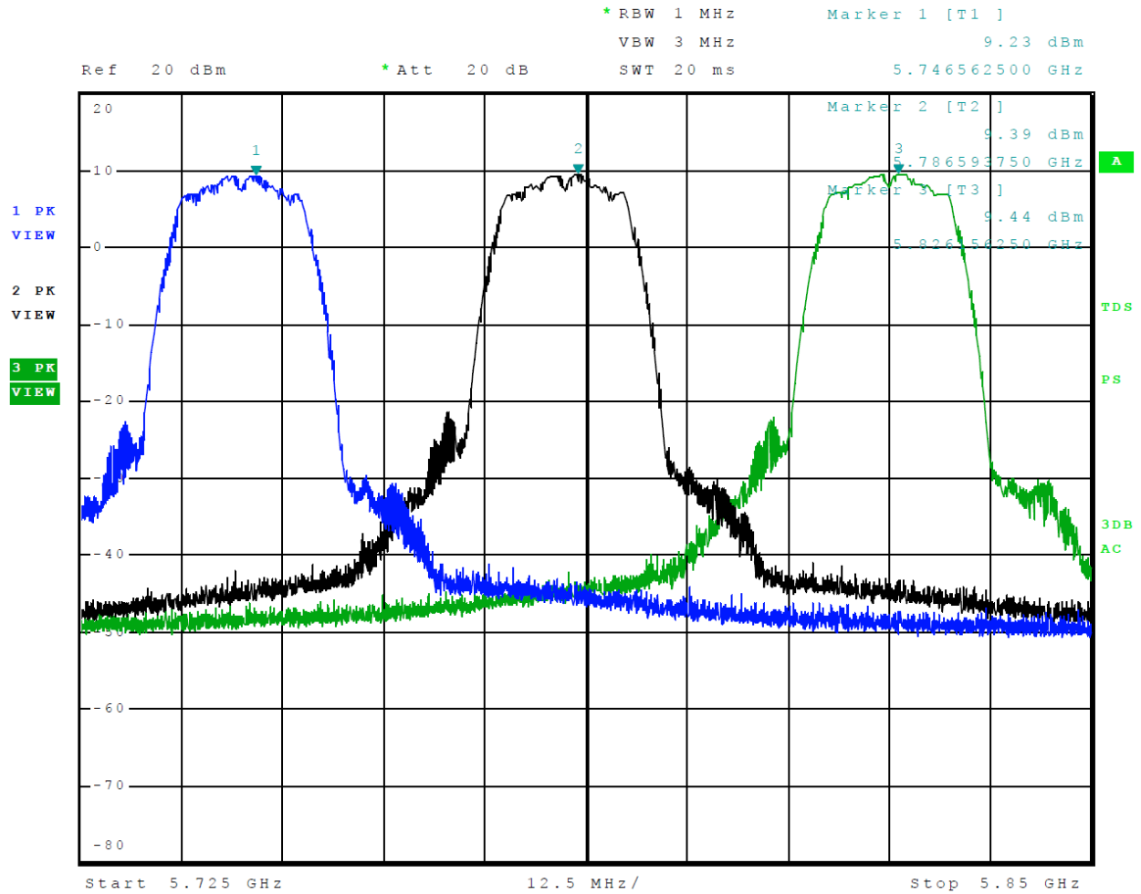
Figure 25 Plot of Transmitter Emissions Across 5725-5850 MHz Mode 12 U-NII-3 (802.11a)
