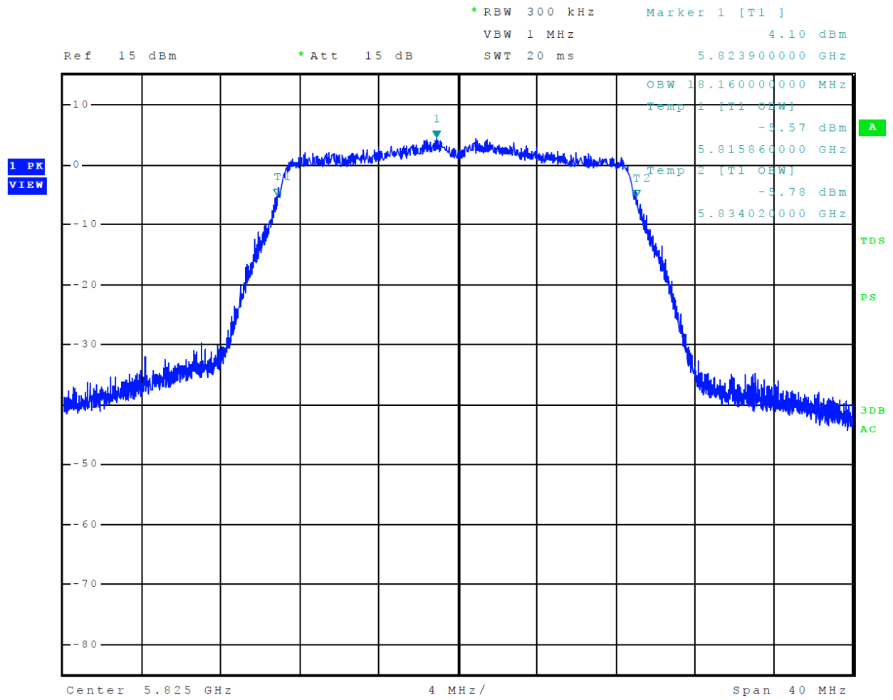
Figure 38 Plot of 99% Occupied Bandwidth 5725-5850 MHz Mode 13 U-NII-3 (802.11n)
