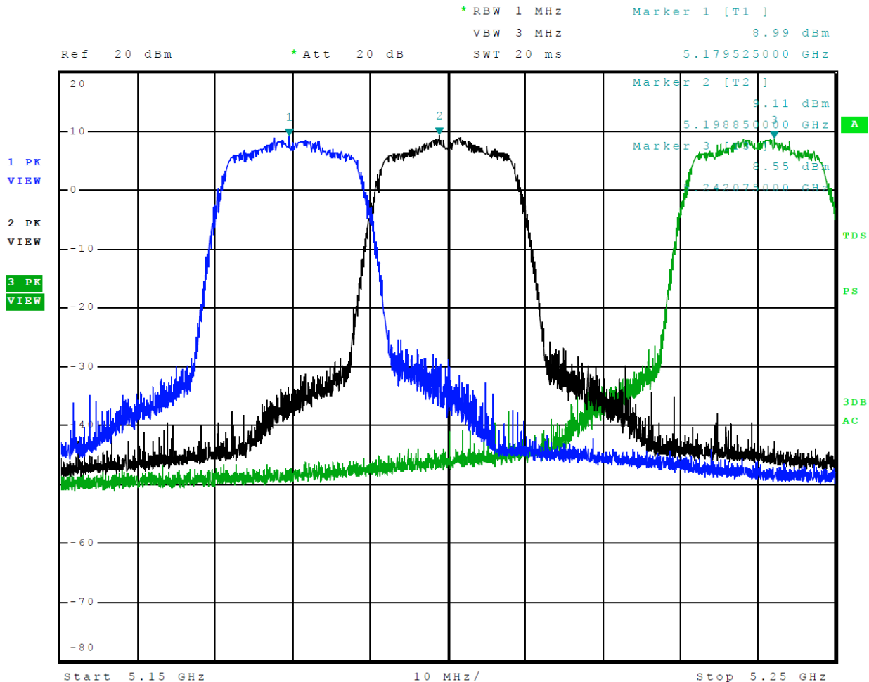
Figure 6 Plot of Transmitter Emissions Across 5150-5250 MHz Mode 9 U-NII-1 (802.11n)
