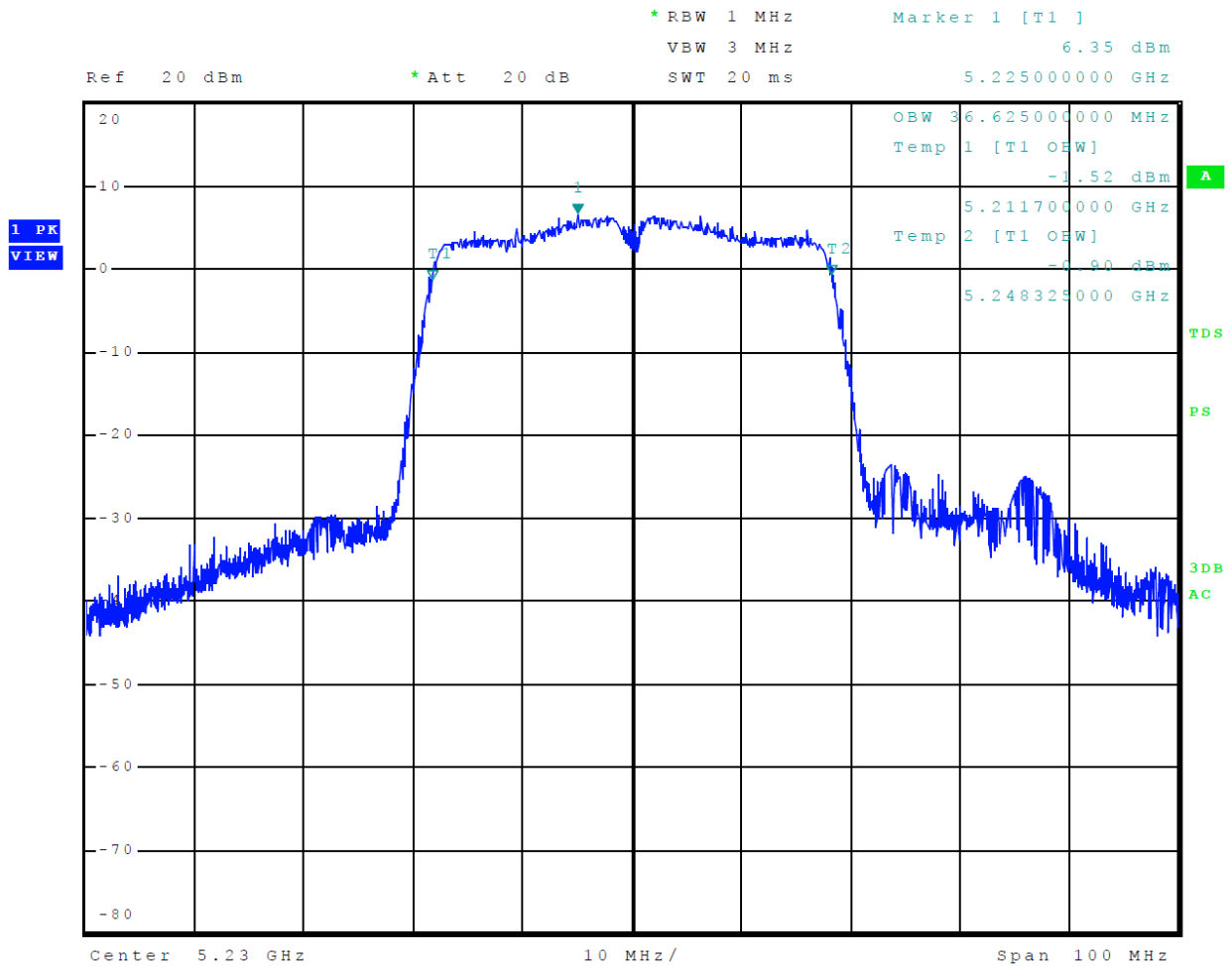
Figure 23 Plot of 99% Occupied Bandwidth 5150-5250 MHz Mode 10 U-NII-1 (802.11n40)
