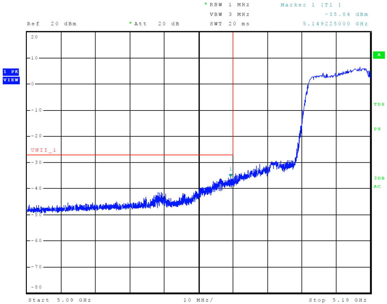
Figure 11 Plot of Lower Band Edge Across 5150-5250 MHz Mode 10 (802.11n40)
