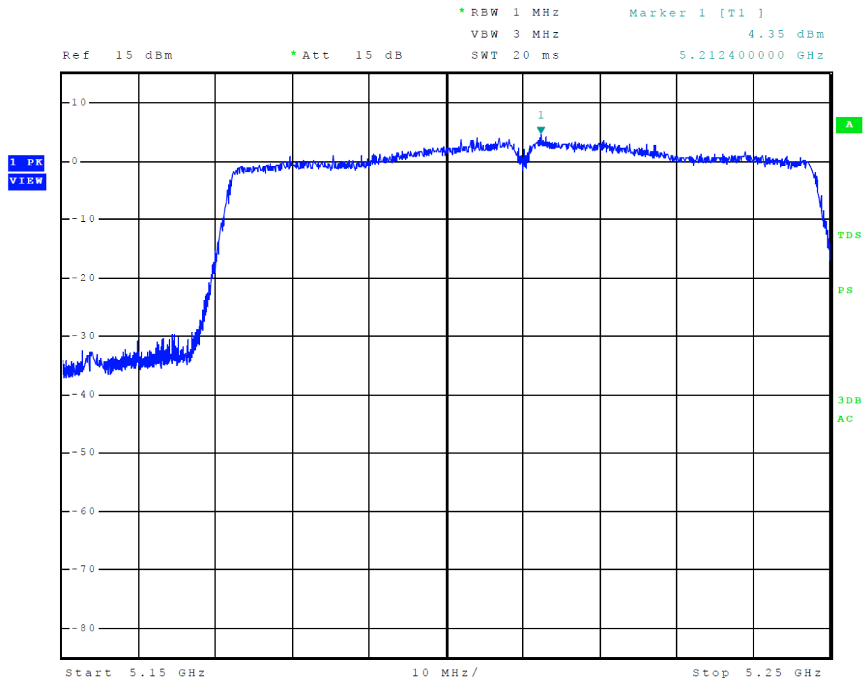
Figure 8 Plot of Transmitter Emissions Across 5150-5250 MHz Mode 11 U-NII-1 (802.11ac80)
