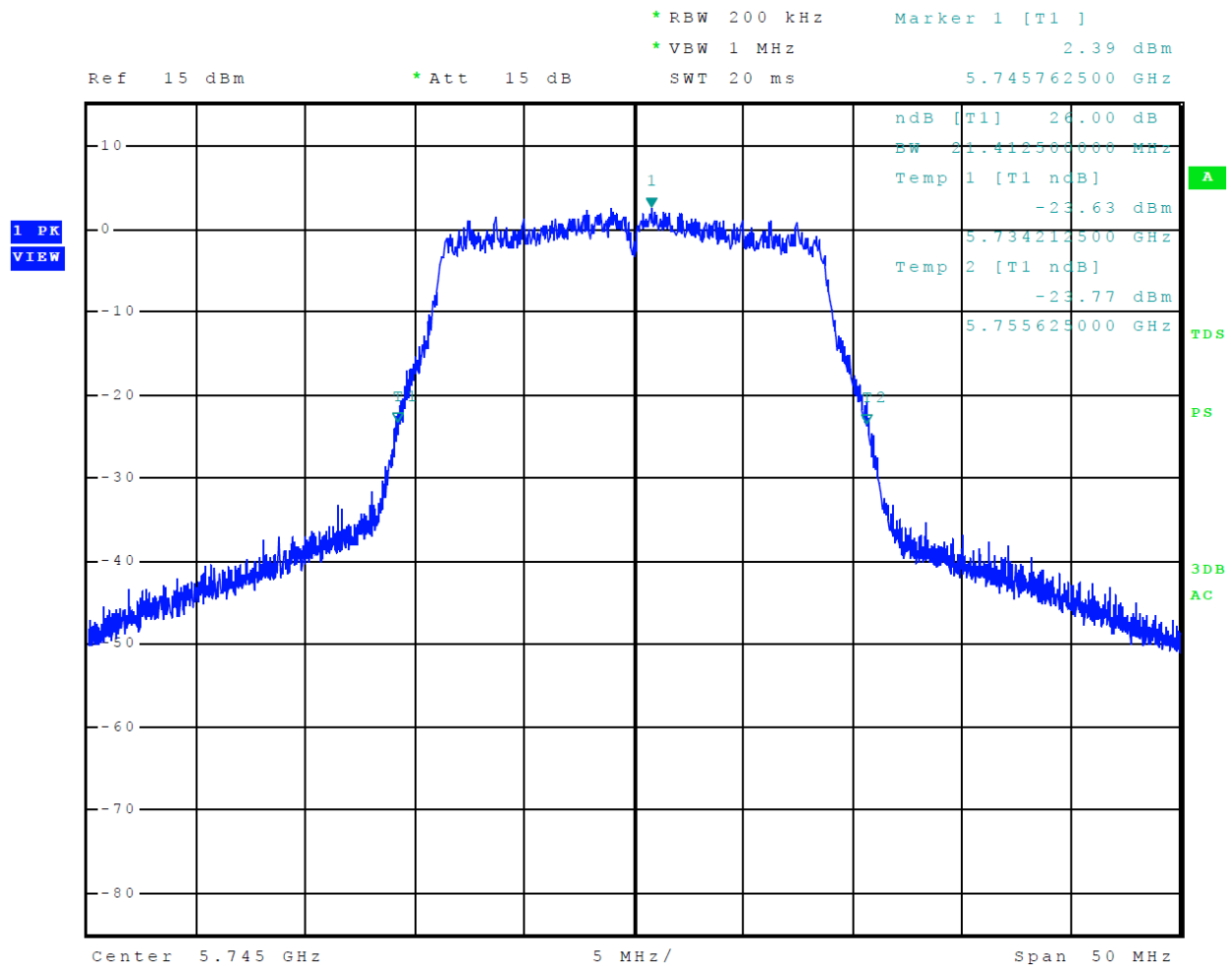
Figure 46 Plot of 26-dB Occupied Bandwidth 5725-5850 MHz Mode 13 U-NII-3 (802.11n)
