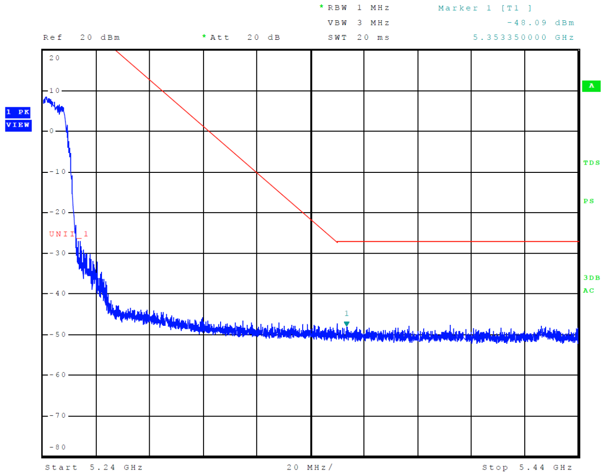
Figure 14 Plot of Upper Band Edge Across 5150-5250 MHz Mode 9 U-NII-1 (802.11n)
