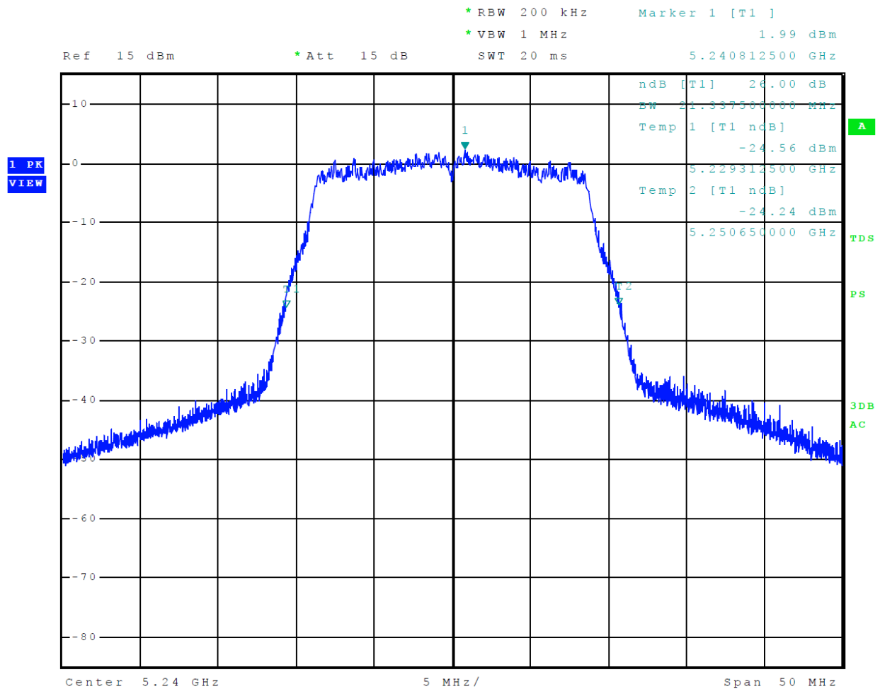
Figure 18 Plot of 26-dB Occupied Bandwidth 5150-5250 MHz Mode 9 U-NII-1 (802.11n)
