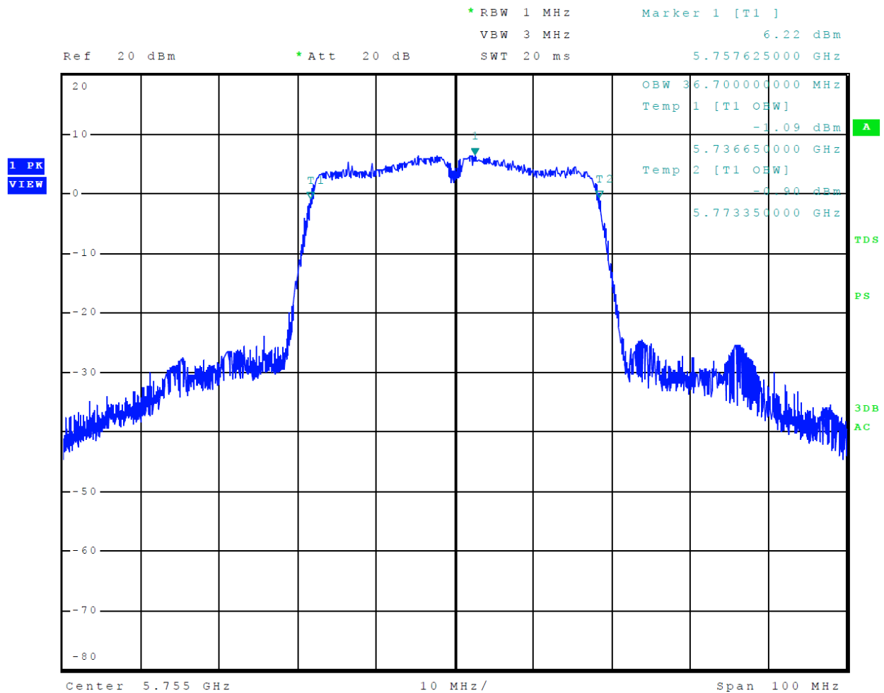
Figure 39 Plot of 99% Occupied Bandwidth 5725-5850 MHz Mode 14 U-NII-3 (802.11n40)
