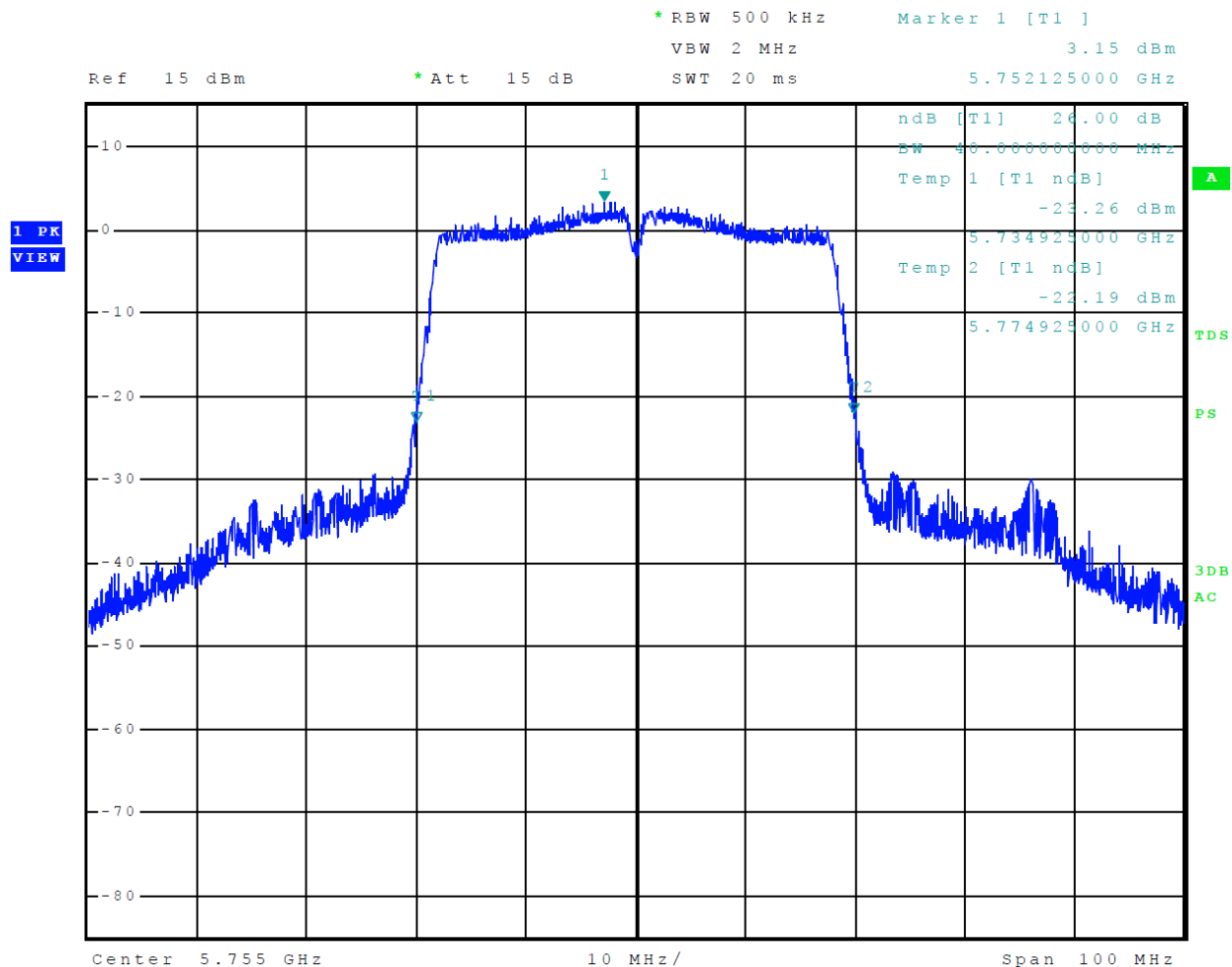
Figure 47 Plot of 26-dB Occupied Bandwidth 5725-5850 MHz Mode 14 U-NII-3 (802.11n40)
