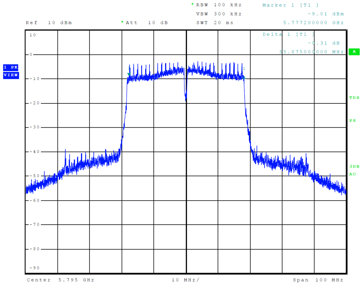
Figure 43 Plot of 6-dB Occupied Bandwidth 5725-5850 MHz Mode 14 U-NII-3 (802.11n40)
