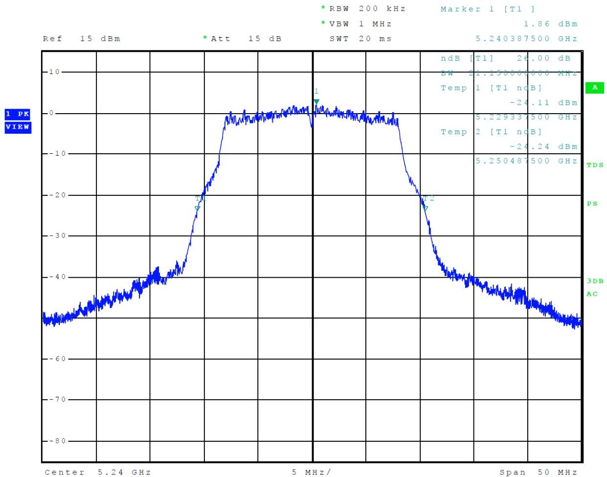
Figure 17 Plot of 26-dB Occupied Bandwidth 5150-5250 MHz Mode 8 U-NII-1 (802.11a)
