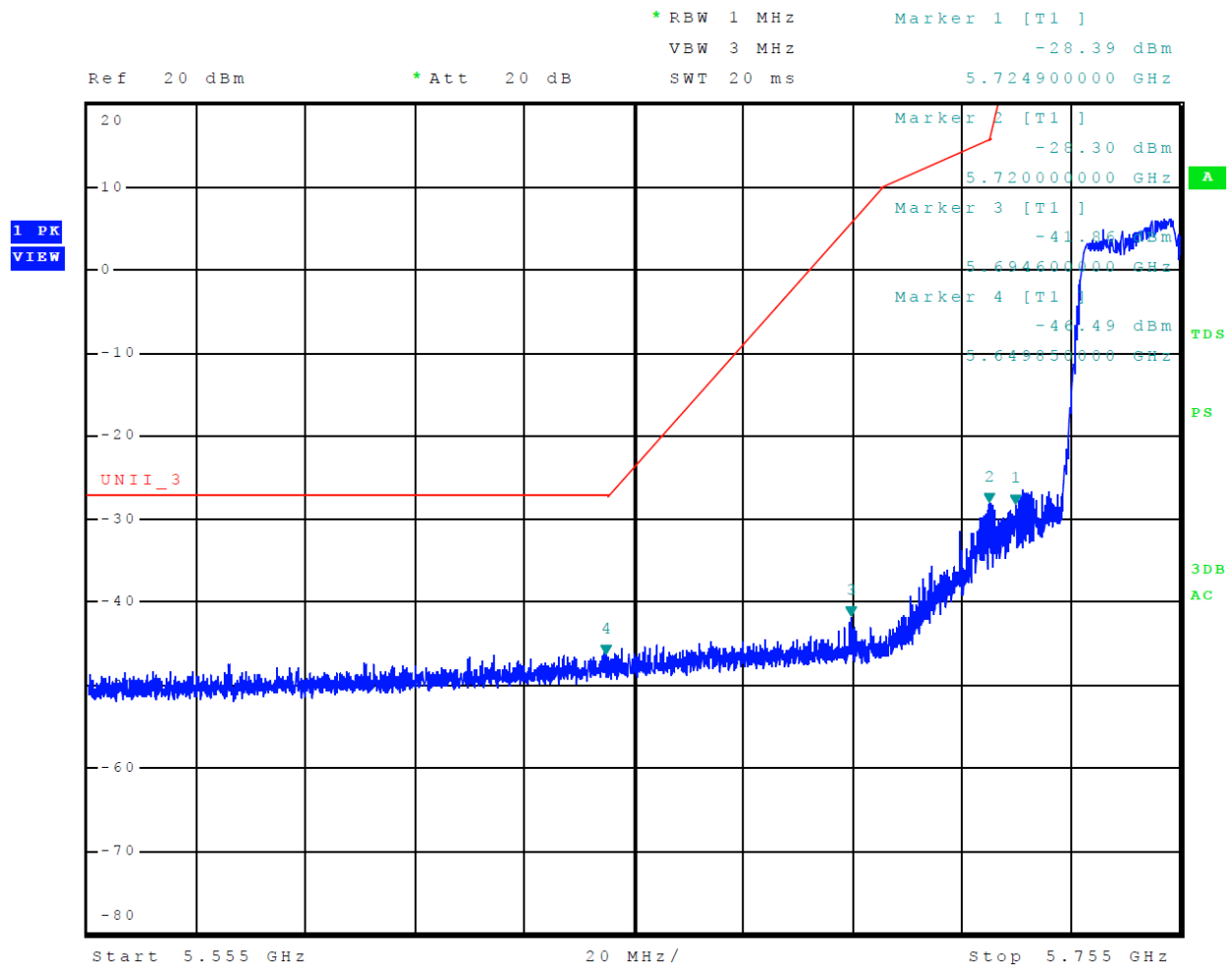
Figure 31 Plot of Lower Band Edge Across 5725-5850 MHz Mode 14 U-NII-3 (802.11n40)
