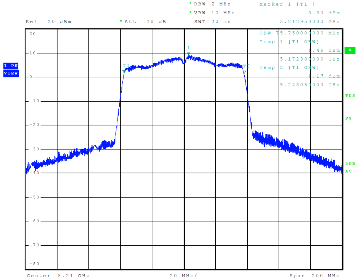
Figure 24 Plot of 99% Occupied Bandwidth 5150-5250 MHz Mode 11 U-NII-1 (802.11ac80)
