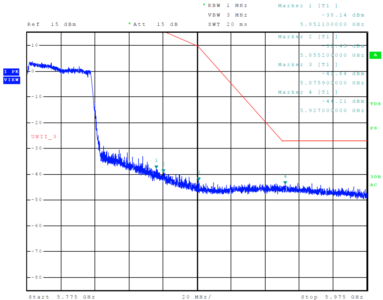
Figure 36 Plot of Upper Band Edge Across 5725-5850 MHz Mode 15 U-NII-3 (802.11ac80)
