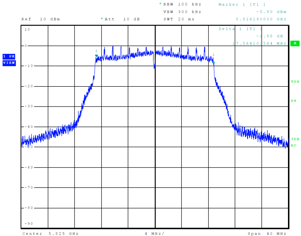
Figure 42 Plot of 6-dB Occupied Bandwidth 5725-5850 MHz Mode 13 U-NII-3 (802.11n)
