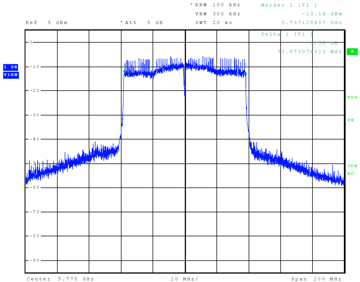
Figure 44 Plot of 6-dB Occupied Bandwidth 5725-5850 MHz Mode 15 U-NII-3 (802.11ac80)
