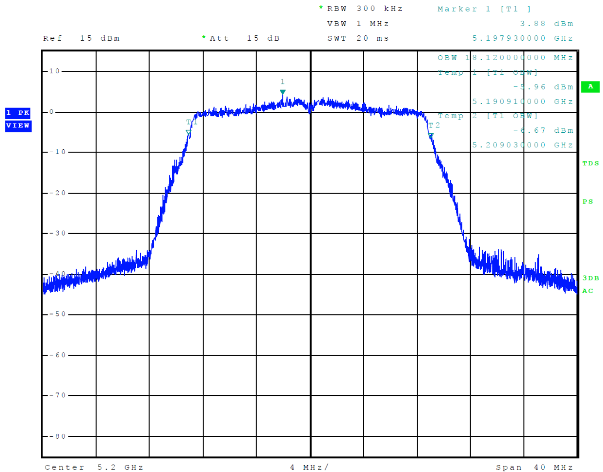
Figure 22 Plot of 99% Occupied Bandwidth 5150-5250 MHz Mode 9 U-NII-1 (802.11n)
