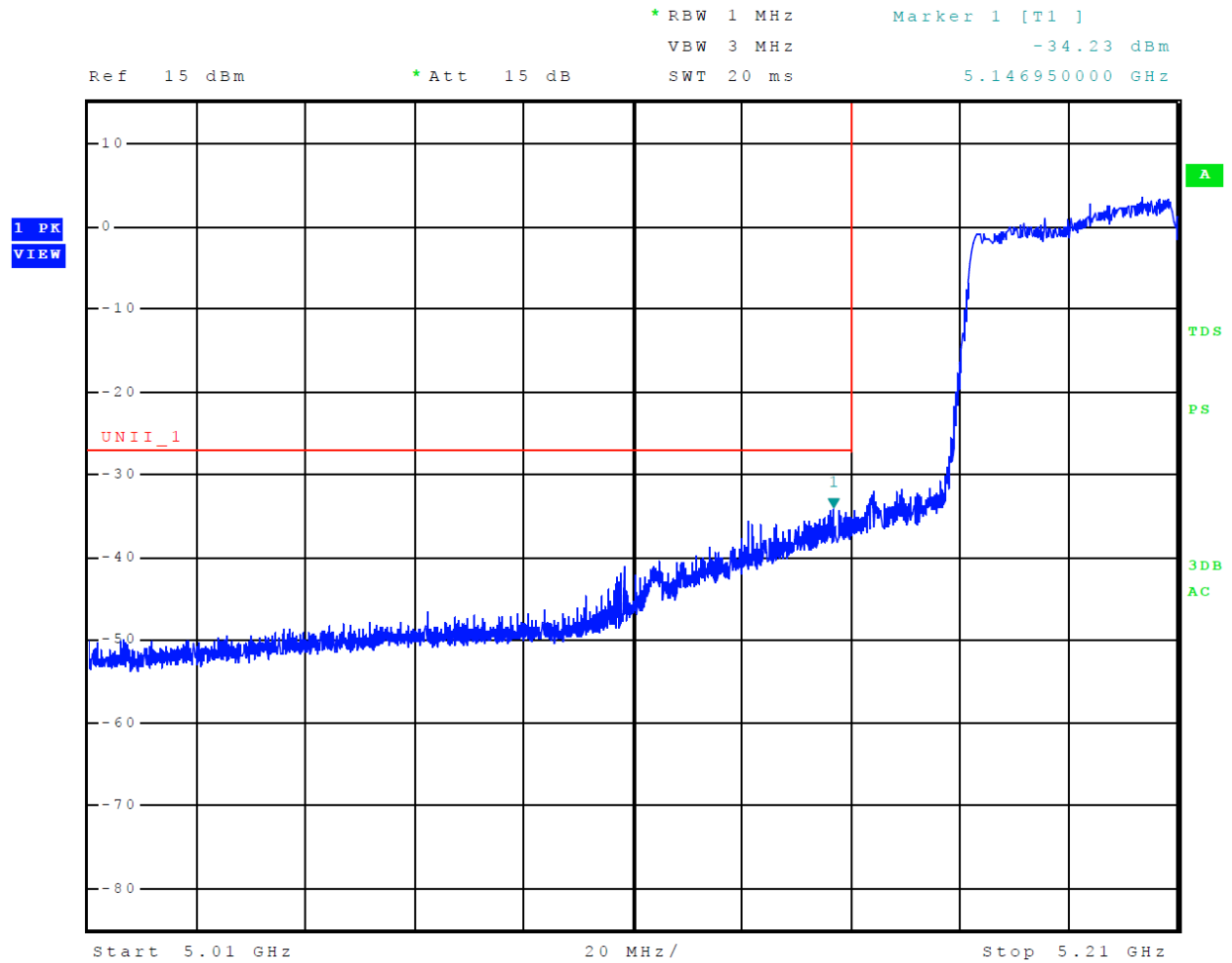
Figure 12 Plot of Lower Band Edge Across 5150-5250 MHz Mode 11 (802.11ac80)
