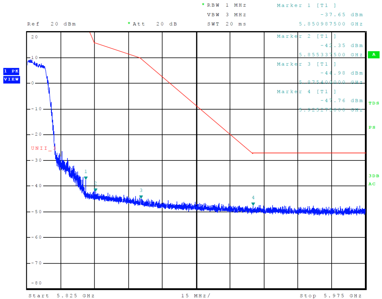
Figure 34 Plot of Upper Band Edge Across 5725-5850 MHz Mode 13 U-NII-3 (802.11n)
