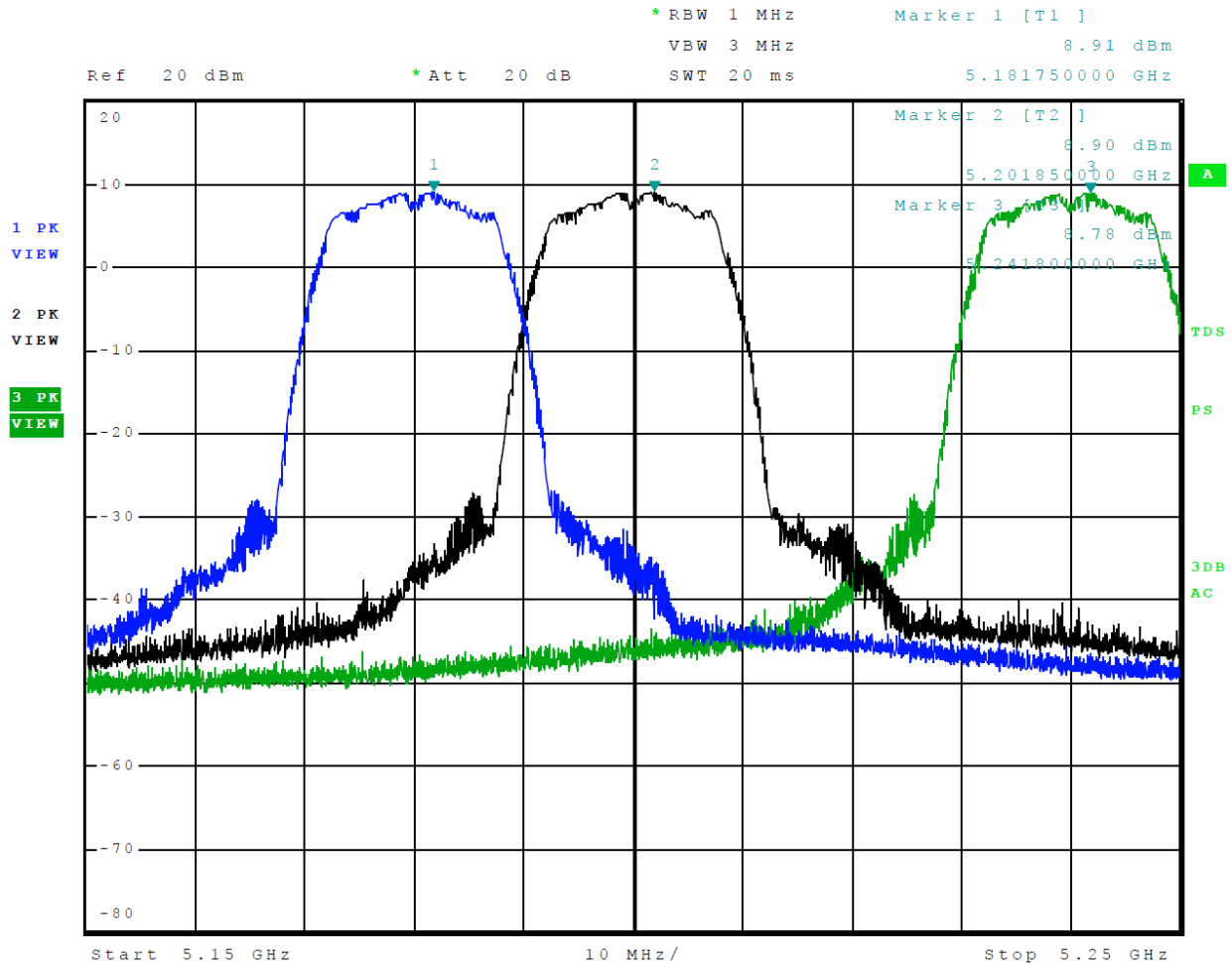
Figure 5 Plot of Transmitter Emissions Across 5150-5250 MHz Mode 8 U-NII-1 (802.11a)
