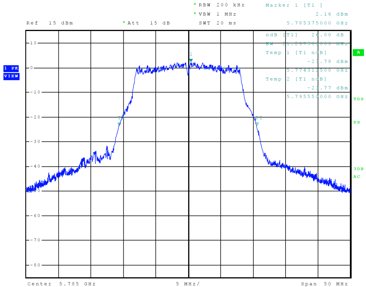
Figure 45 Plot of 26-dB Occupied Bandwidth 5725-5850 MHz Mode 12 U-NII-3 (802.11a)
