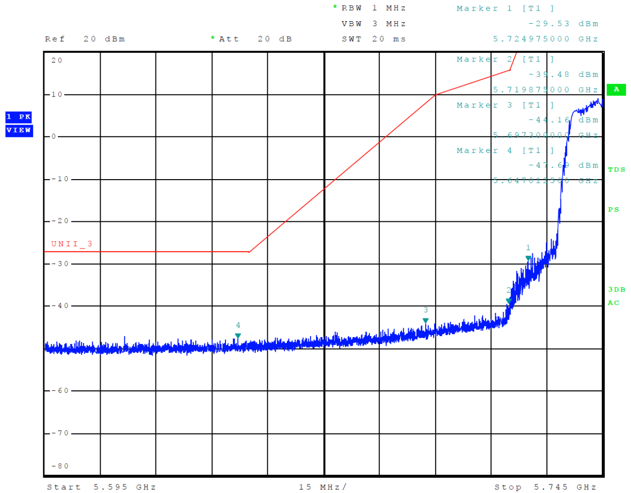
Figure 30 Plot of Lower Band Edge Across 5725-5850 MHz Mode 13 U-NII-3 (802.11n)
