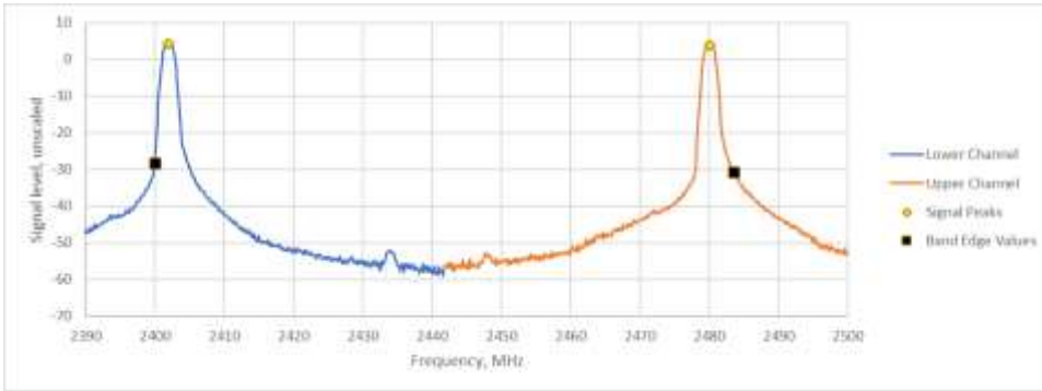
Figure TR16.3: Spectral data for BLE 1 Mbps at 20°C and 4.5 Vdc
