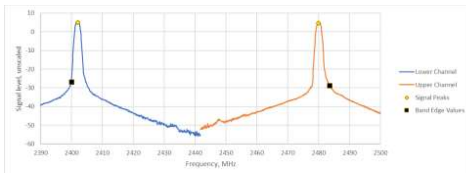
Figure TR16.1: Spectral data for BLE 1Mbps at -20°C
