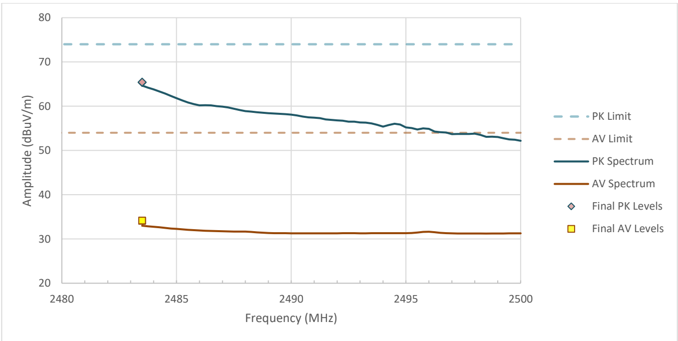
Figure RE01.2: Spectral data
