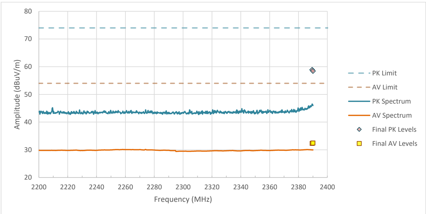
Figure RE01.1: Spectral data
