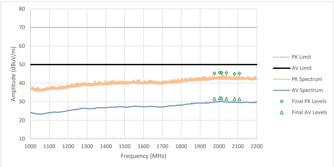
Figure RE05.1: Spectral data
