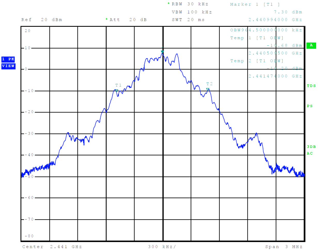
Figure 7 Plot of Transmitter Emissions 99% Occupied Bandwidth Mode 2, BT BR
