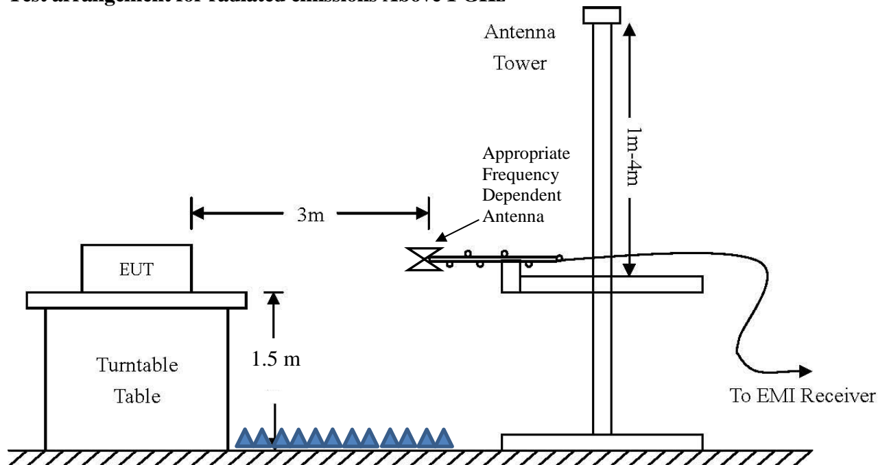
Test arrangement for radiated emissions Above 1 GHz
