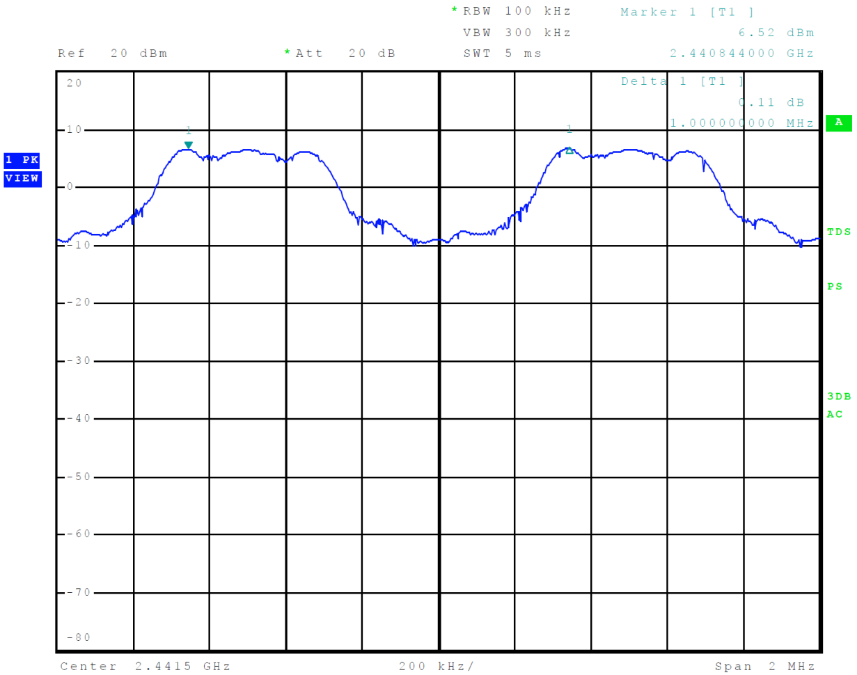
Figure 12 Plot of Channel Separation Mode 2, BT BR
