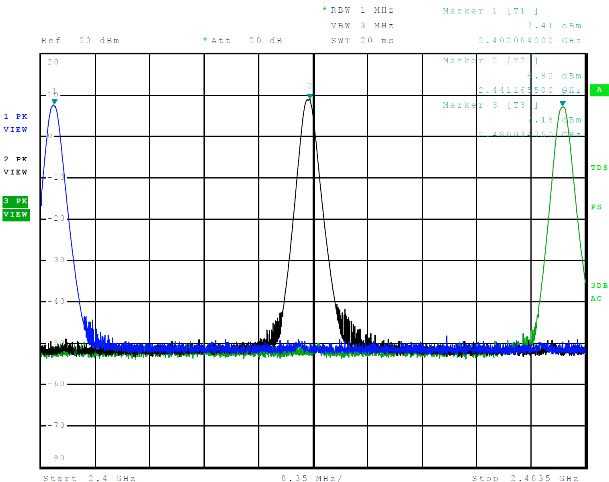
Figure 5 Plot of Transmitter Emissions Operation in 2402-2480 MHz Mode 2, BT BR
