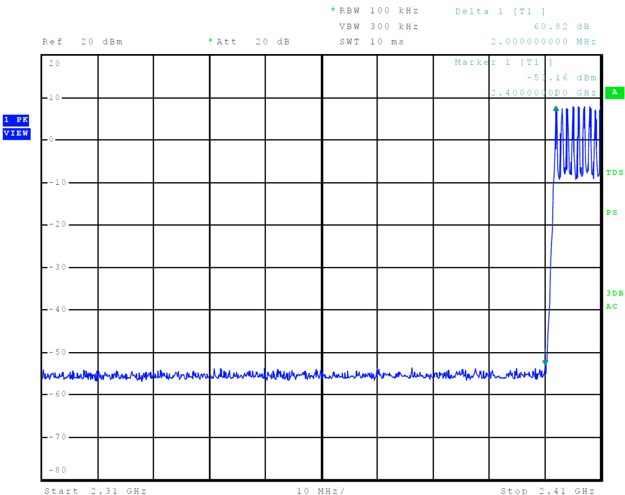
Figure 15 Plot of Transmitter Emissions Low Band Edge Mode 2, BT BR
