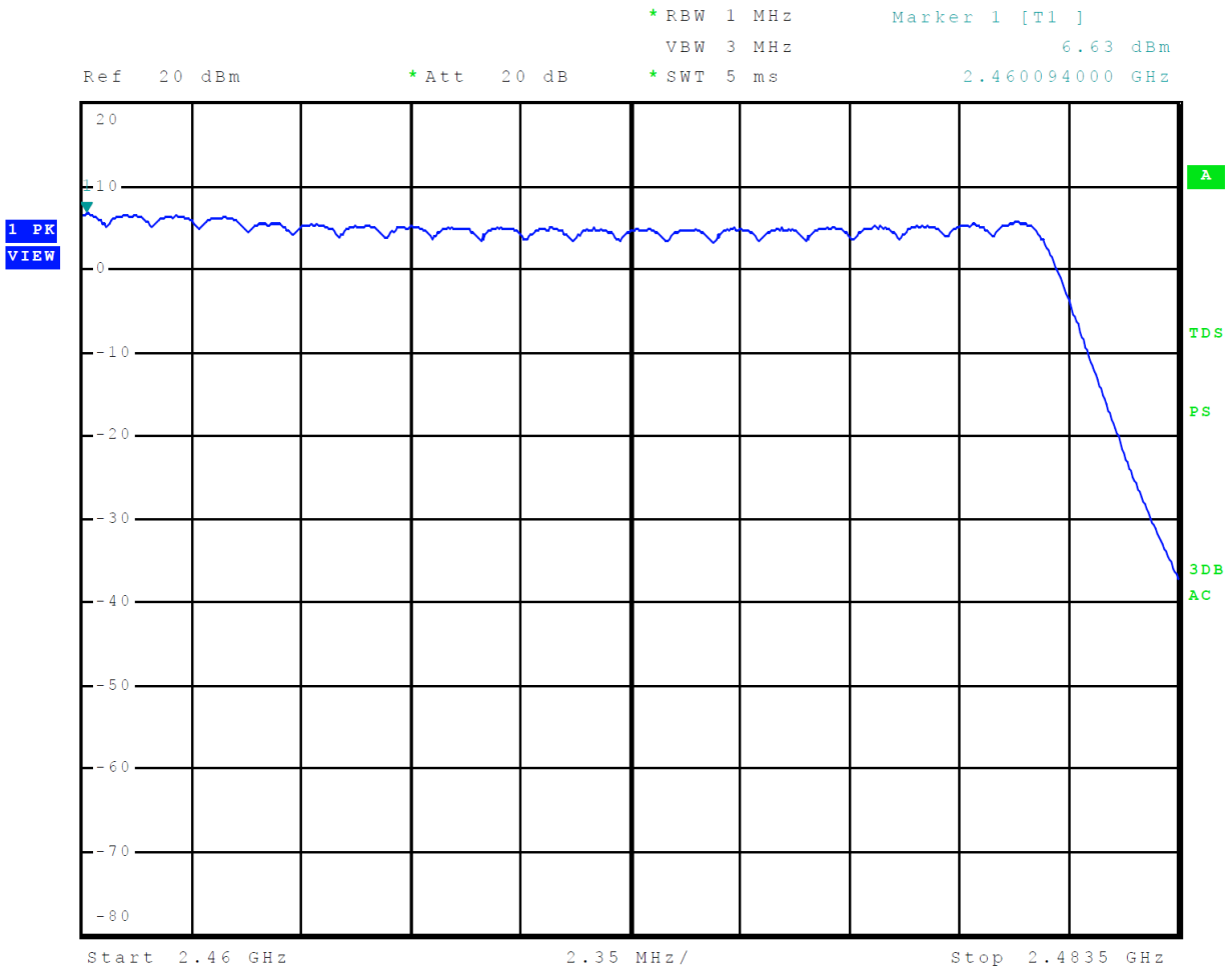
Figure 11 Plot of Number of Hopping Channels Mode 2, BT BR
