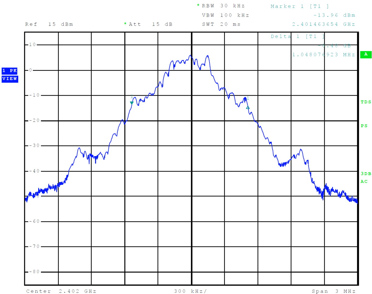
Figure 6 Plot of Transmitter Emissions 20-dB Occupied Bandwidth Mode 2, BT BR
