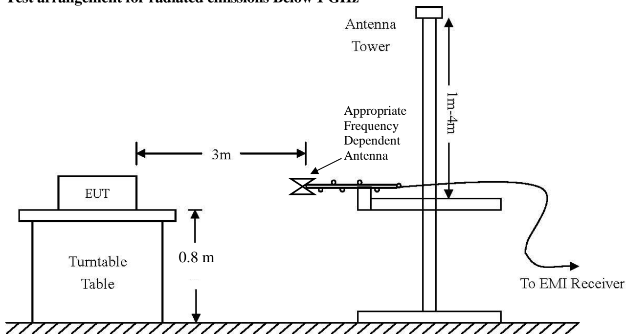
Diagram 3 Test arrangement for radiated emissions tested on Open Area Test Site (OATS) Test arrangement for radiated emissions Below 1 GHz
