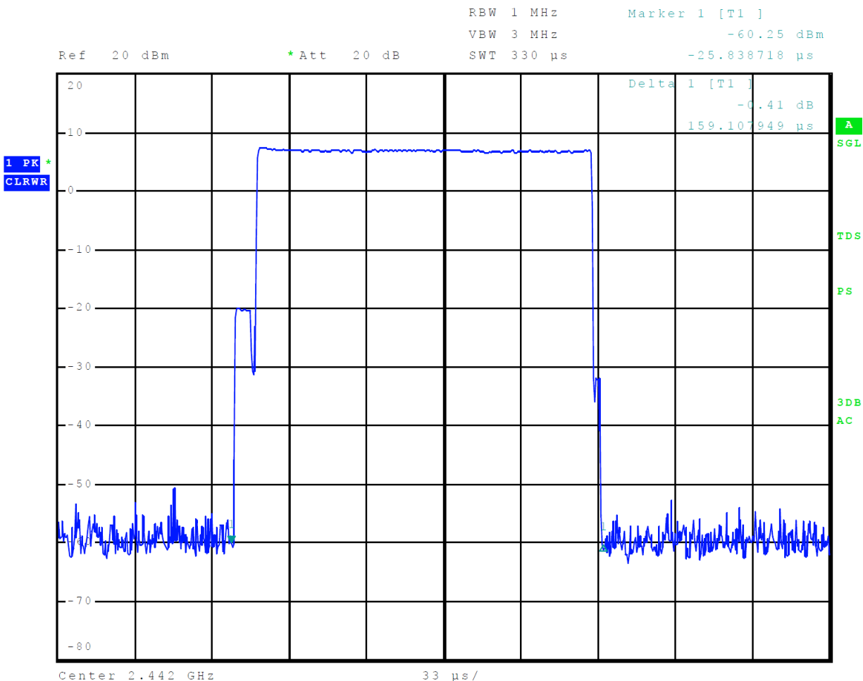
Figure 13 Plot of Dwell time On Channel Mode 2, BT BR
