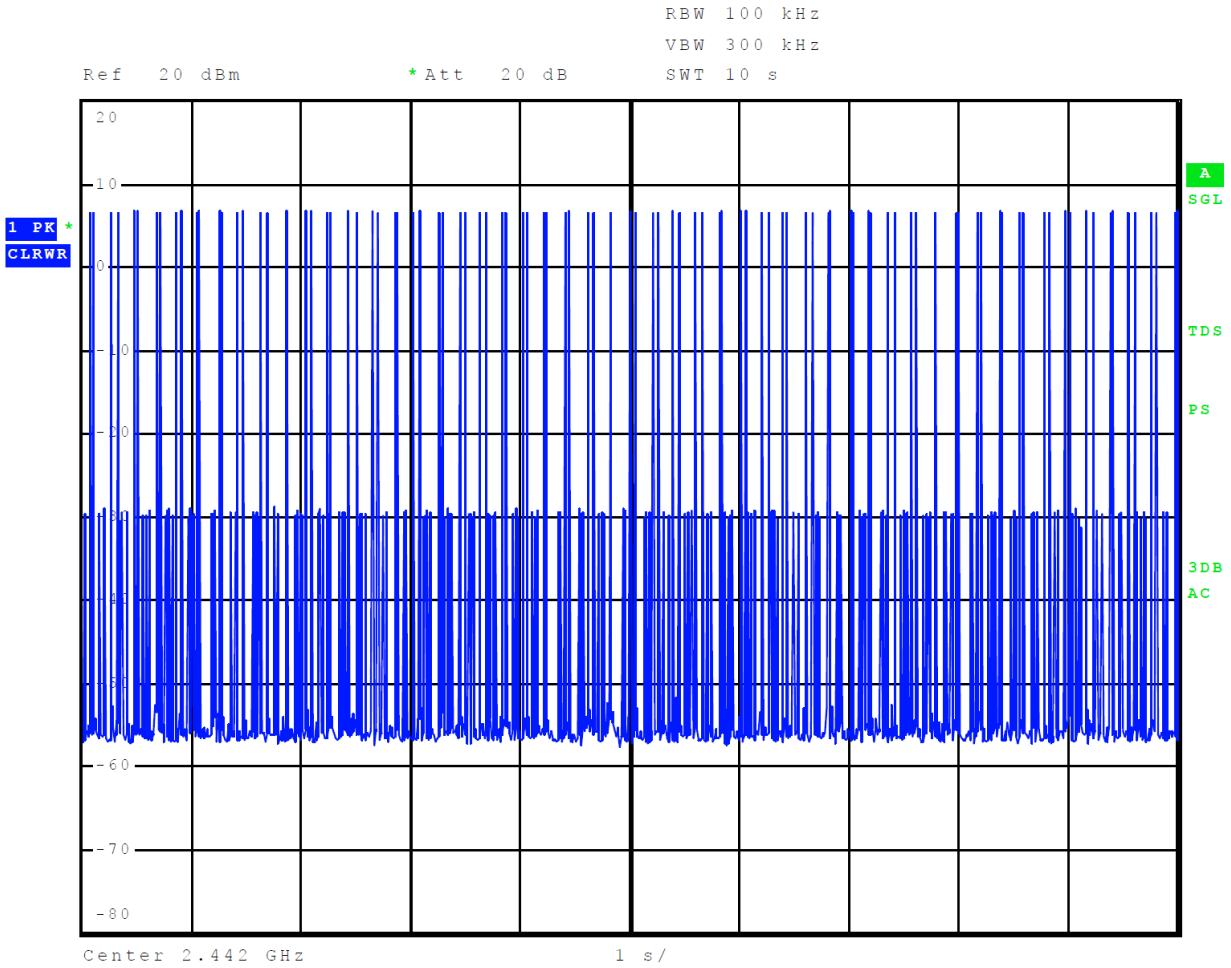
Figure 14 Plot of Number of Times on Channel over 10 Second Period Mode 2, BT BR
