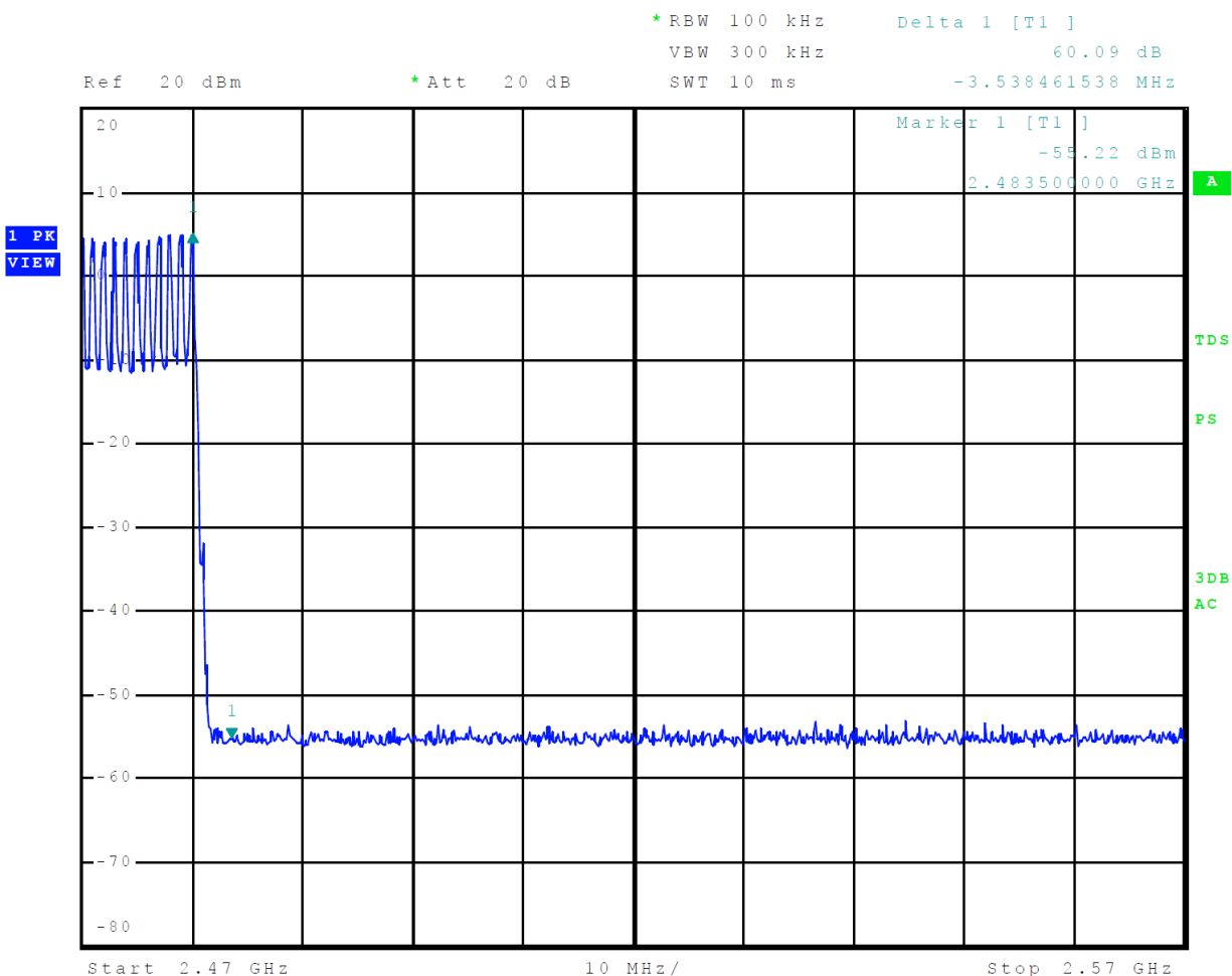
Figure 16 Plot of Transmitter Emissions High Band Edge Mode 2, BT BR
