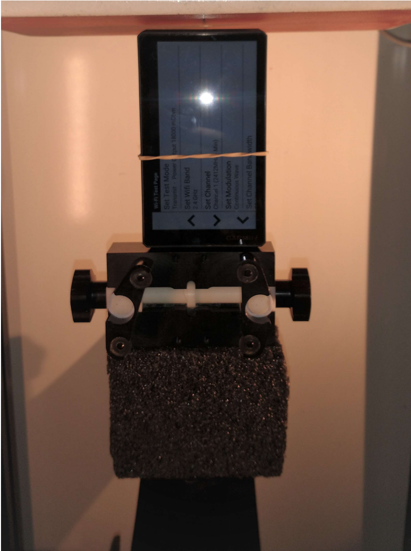
Figure C.5 – Setup Photo, Left Edge 5mm - MFP Phantom – Body SAR
