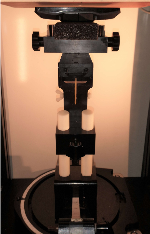
Figure C.2 – Setup Photo, Front Side 5mm – MFP Phantom – Body SAR
