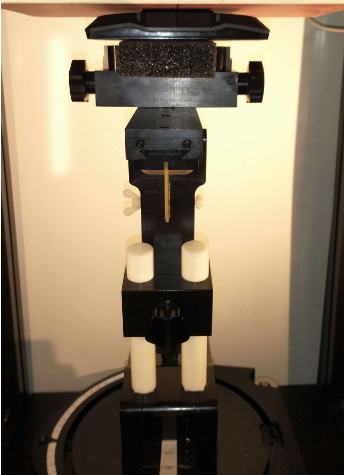
Figure C.3 – Setup Photo, Back Side -Touch – MFP Phantom – Extremity SAR
