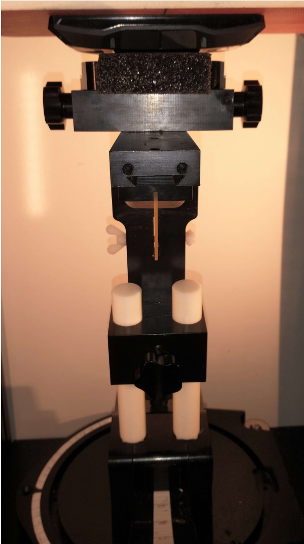
Figure C.4 – Setup Photo, Front Side -Touch – MFP Phantom – Extremity SAR
