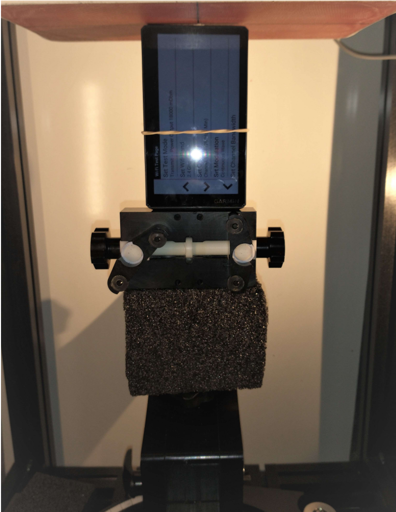
Figure C.6 – Setup Photo, Left Edge - Touch – MFP Phantom – Extremity SAR
