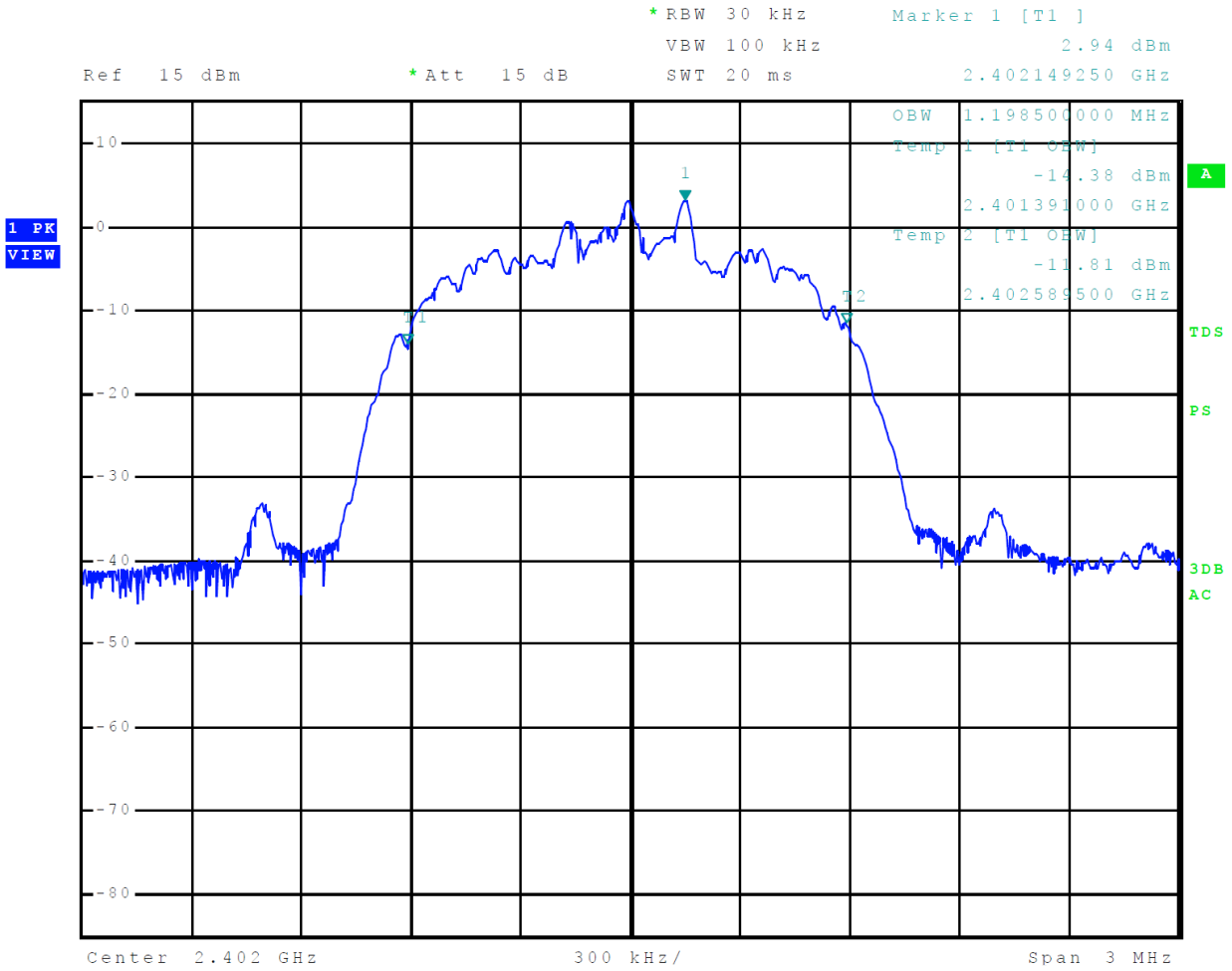
Figure 26 Plot of Transmitter 99% Occupied Bandwidth Mode 4, BT 3EDR (8DPSK)
