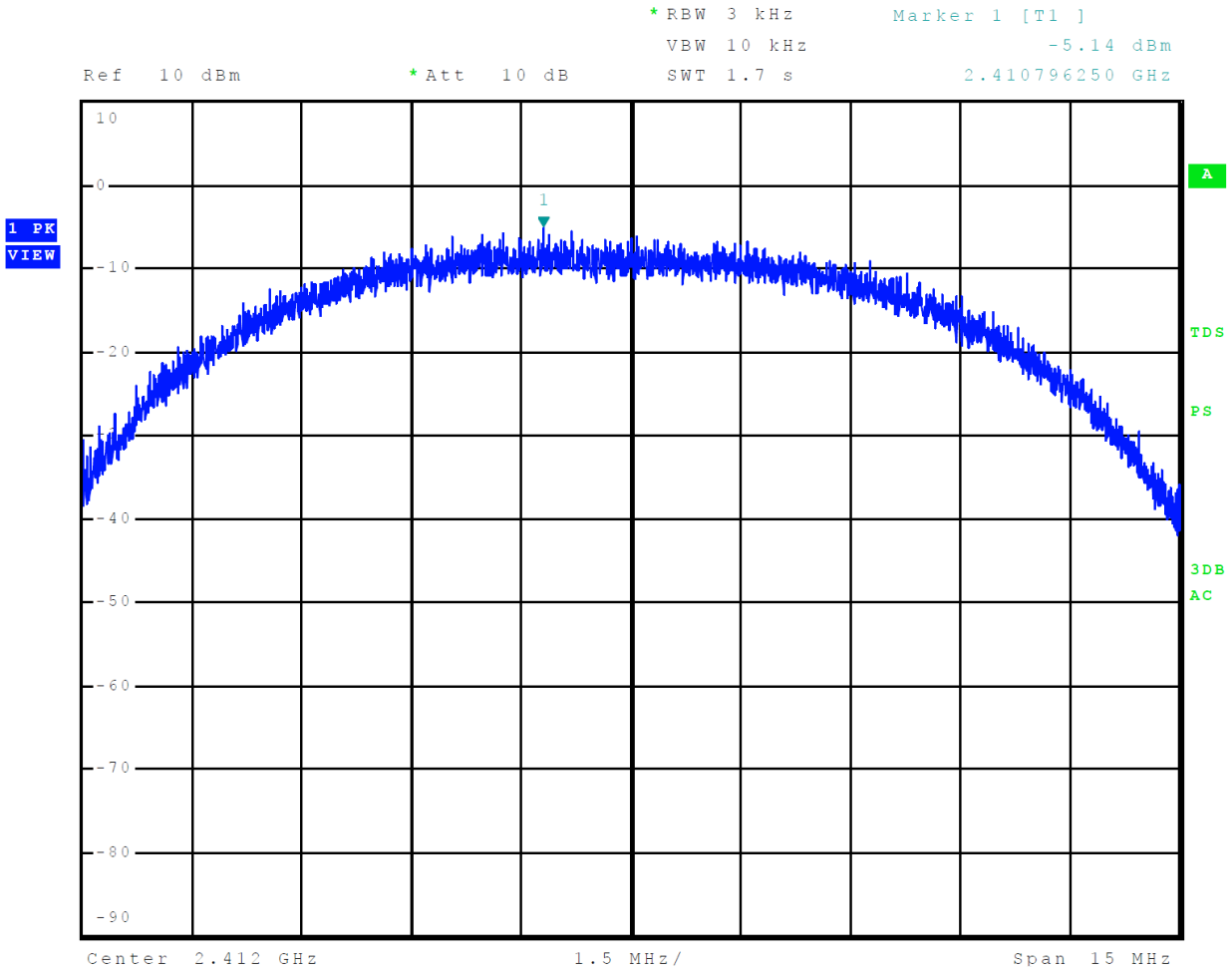
Figure 38 Plot of Transmitter Power Spectral Density Mode 6, 802.11b (DSSS/CCK)
