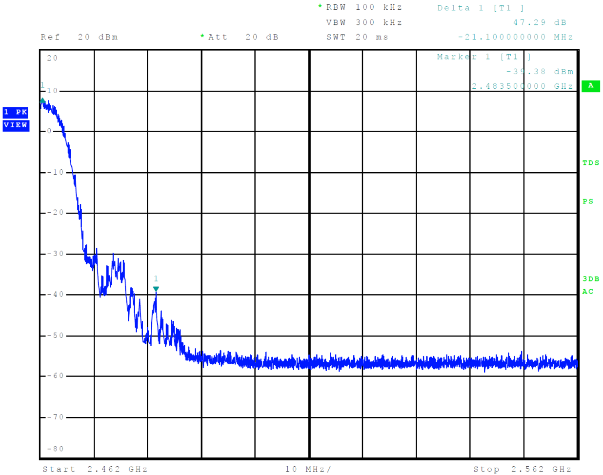
Figure 20 Plot of Transmitter Emissions High Band Edge Mode 6, 802.11b (DSSS/CCK)
