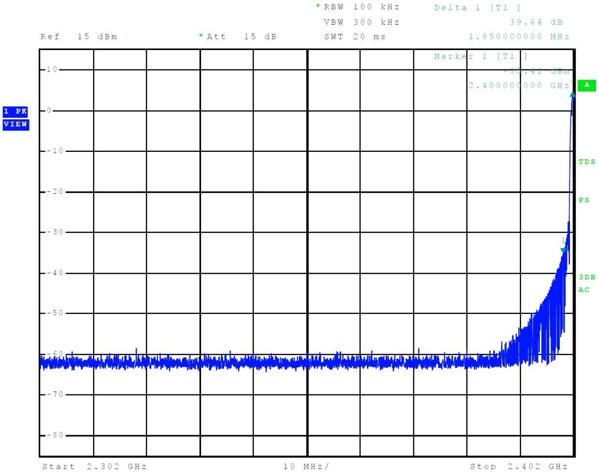
Figure 12 Plot of Transmitter Emissions Low Band Edge Mode 4, BT 3EDR (8DPSK)
