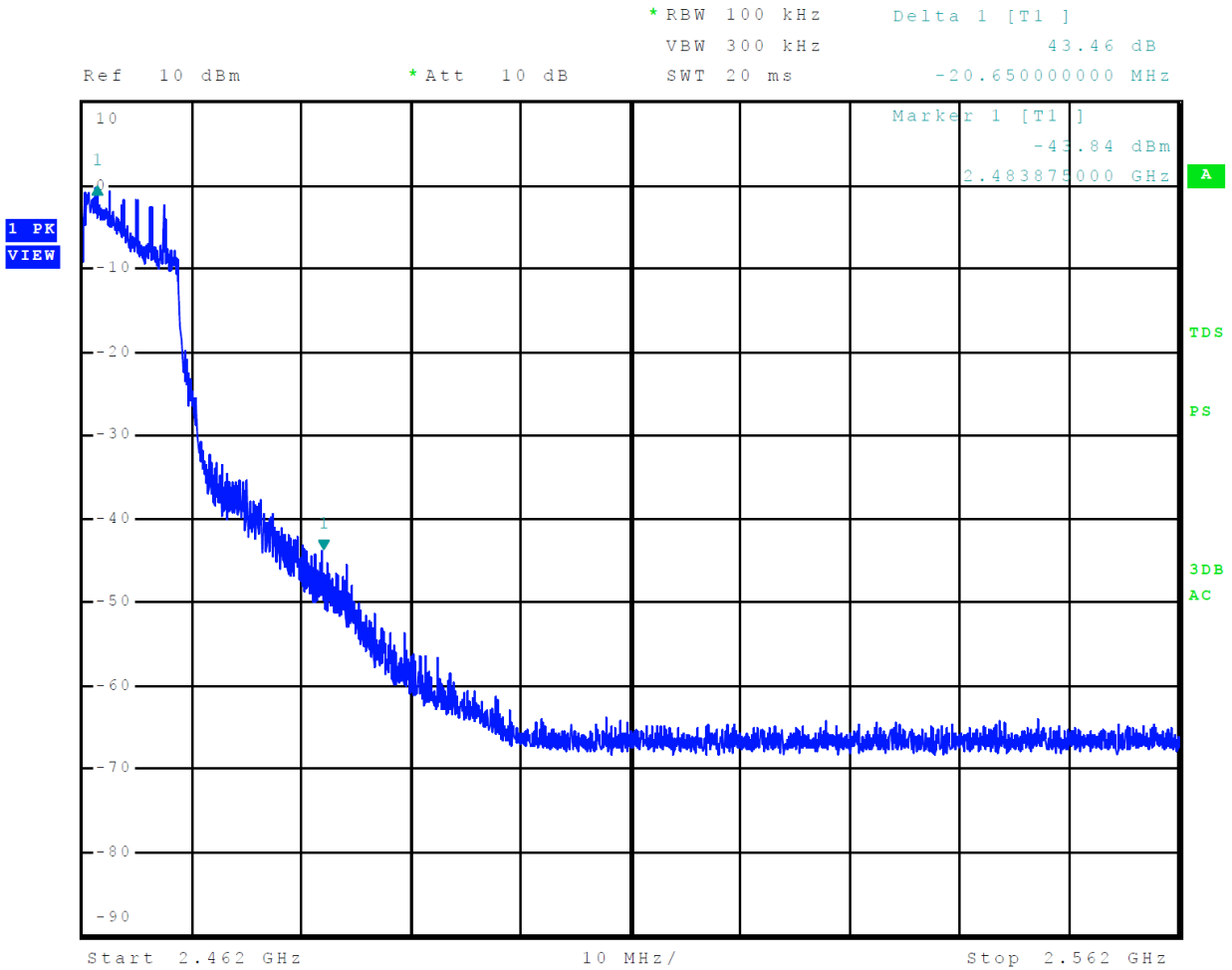
Figure 22 Plot of Transmitter Emissions High Band Edge Mode 8, 802.11n (MSC)
