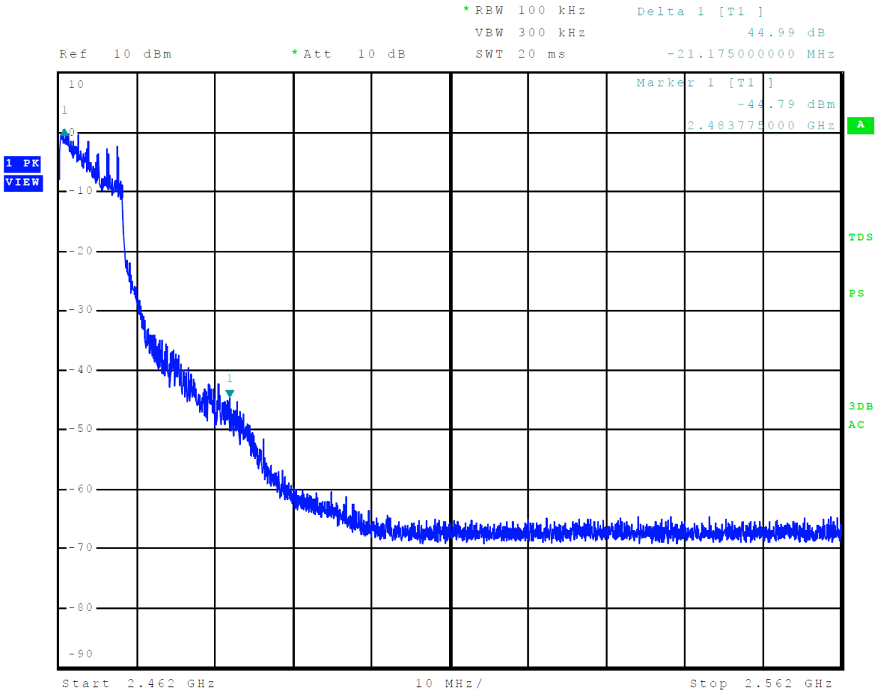
Figure 21 Plot of Transmitter Emissions High Band Edge Mode 7, 802.11g (OFDM)
