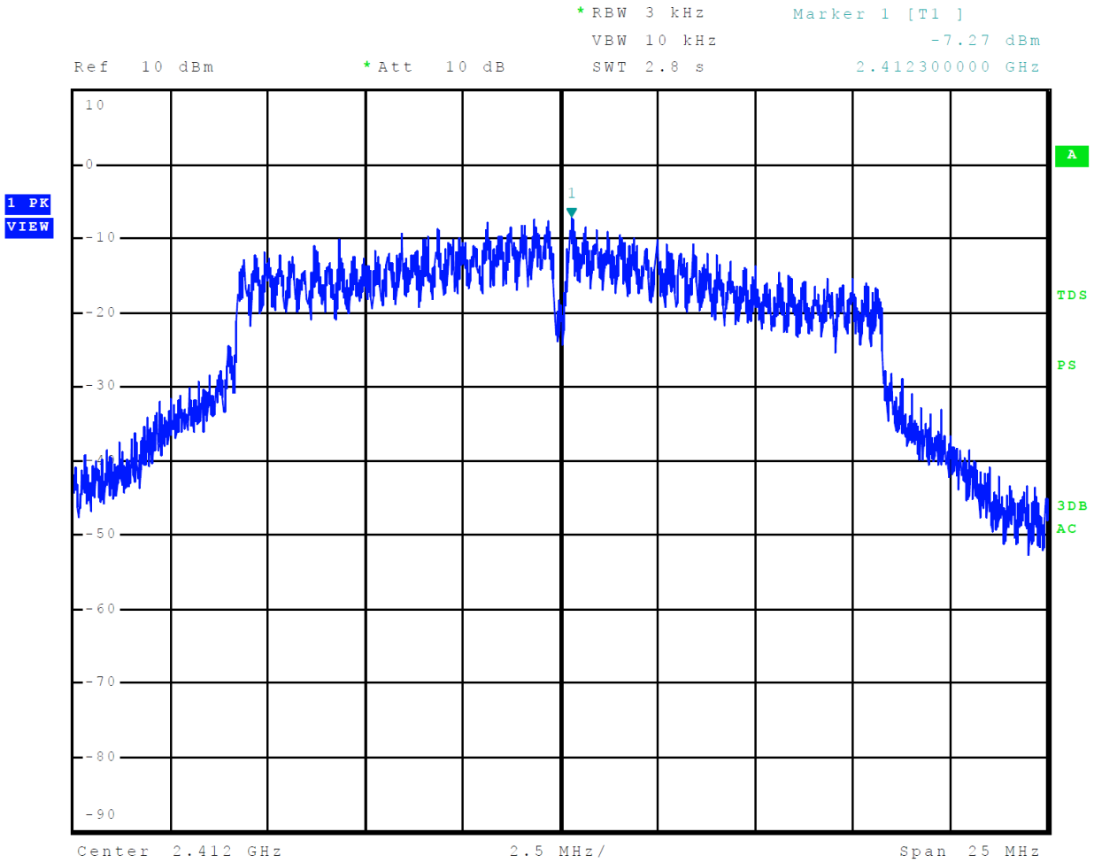
Figure 31 Plot of 6-dB Occupied Bandwidth Mode 7, 802.11g (OFDM)
