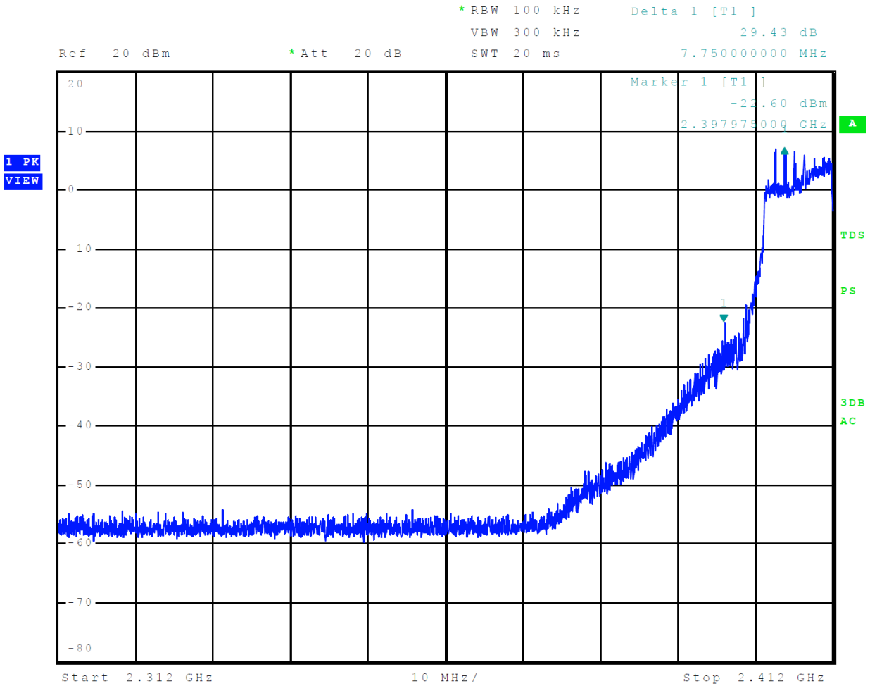
Figure 16 Plot of Transmitter Emissions Low Band Edge Mode 8, 802.11n (MSC)
