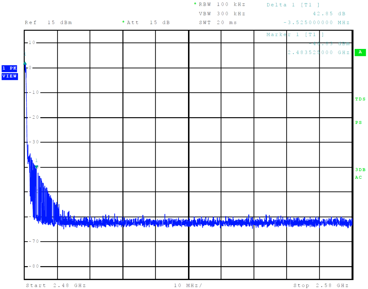
Figure 17 Plot of Transmitter Emissions High Band Edge Mode 3, BT 2EDR ( \pi/4 -DQPSK)
