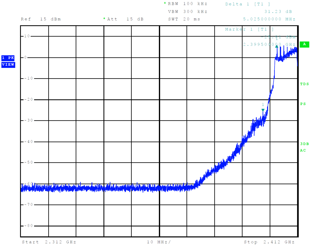
Figure 15 Plot of Transmitter Emissions Low Band Edge Mode 7, 802.11g (OFDM)
