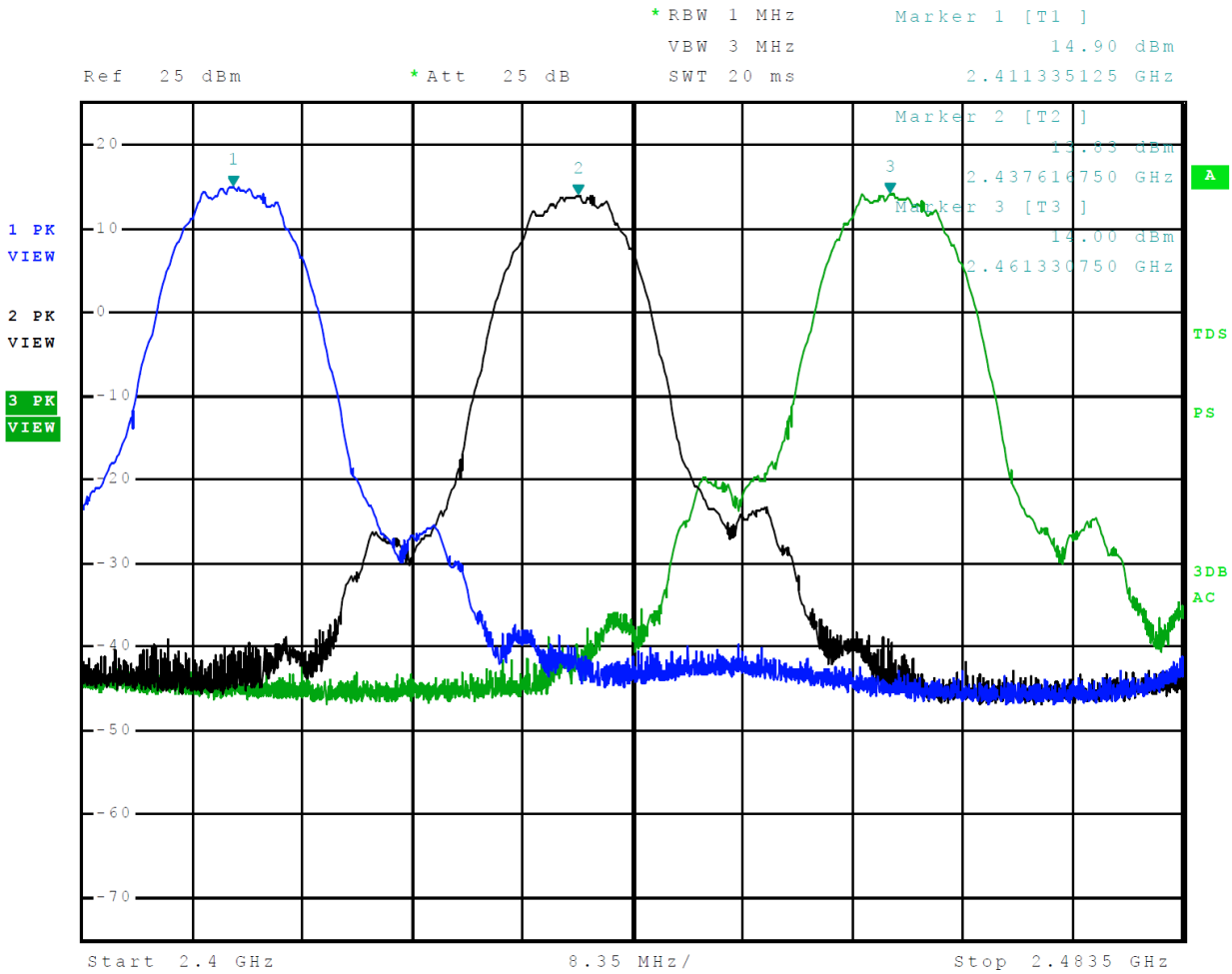
Figure 8 Plot of Transmitter Operation in 2412-2462 MHz Mode 6, 802.11b (DSSS/CCK)
