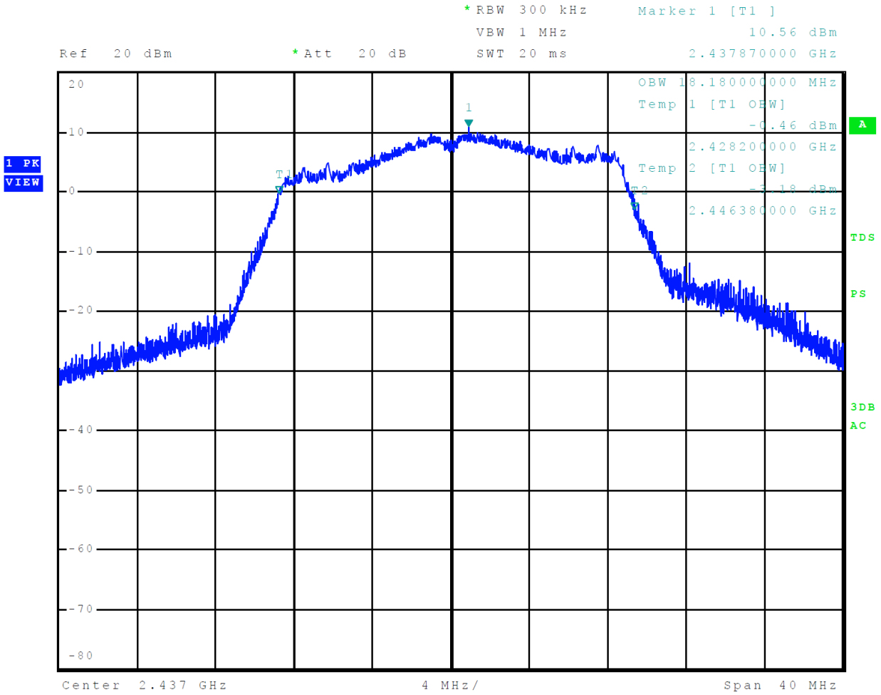
Figure 34 Plot of 99% Occupied Bandwidth Mode 8, 802.11n (MSC)
