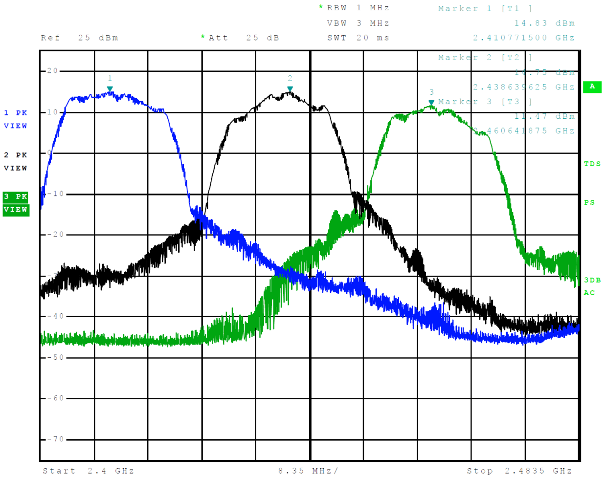
Figure 9 Plot of Transmitter Operation in 2412-2462 MHz Mode 7, 802.11g (OFDM)
