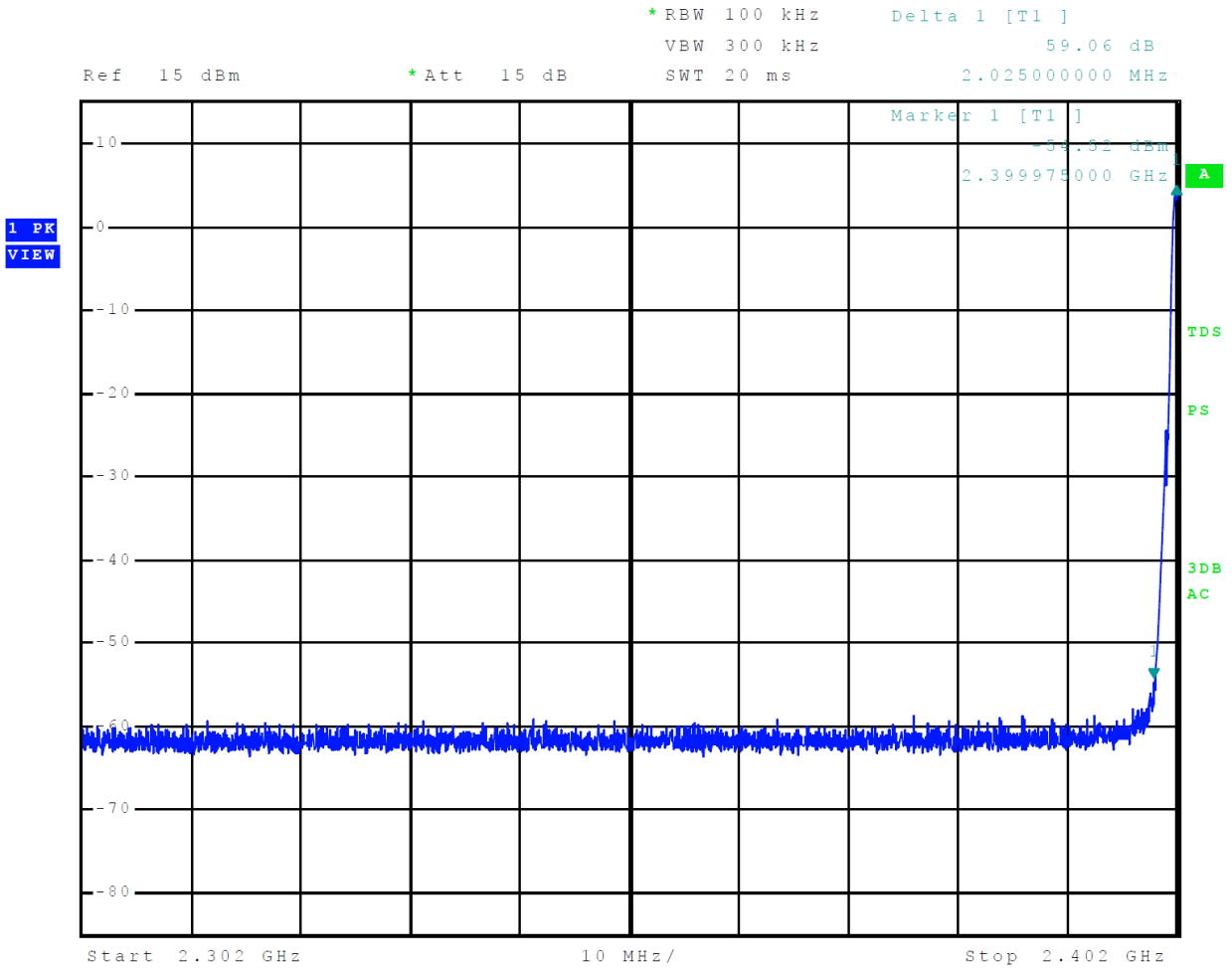
Figure 13 Plot of Transmitter Emissions Low Band Edge Mode 5, BT BLE (GMSK)
