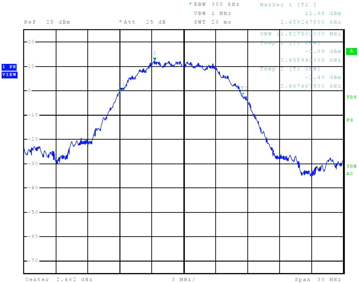
Figure 30 Plot of 99% Occupied Bandwidth Mode 6, 802.11b (DSSS/CCK)
