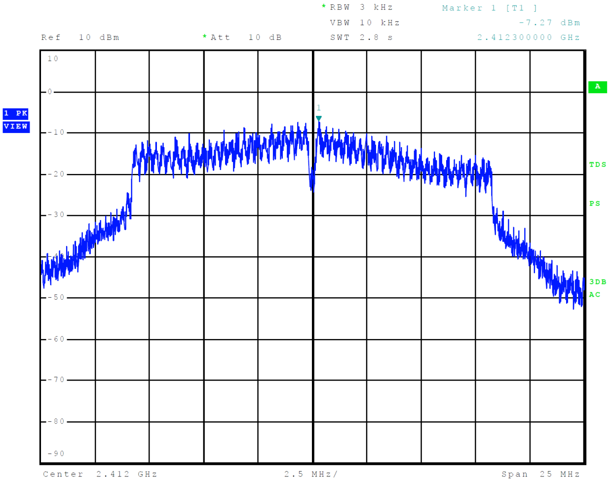
Figure 39 Plot of Transmitter Power Spectral Density Mode 7, 802.11g (OFDM)
