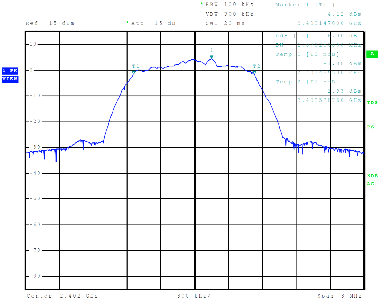
Figure 23 Plot of 6-dB Occupied Bandwidth Mode 3, BT 2EDR ( \pi/4 -DQPSK)
