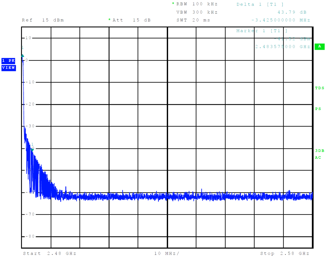
Figure 18 Plot of Transmitter Emissions High Band Edge Mode 4, BT 3EDR (8DPSK)
