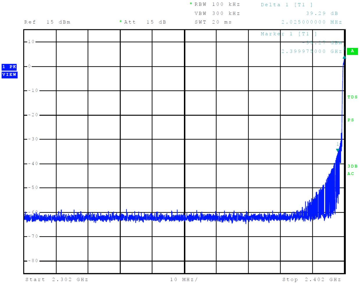
Figure 11 Plot of Transmitter Emissions Low Band Edge Mode 3, BT 2EDR ( \pi/4 -DQPSK)
