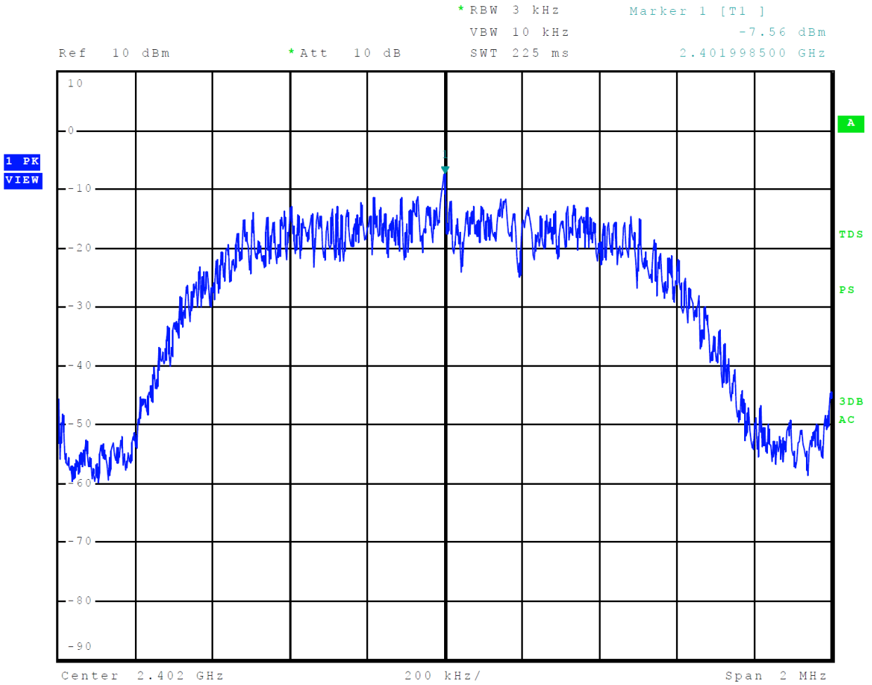
Figure 36 Plot of Transmitter Power Spectral Density Mode 4, BT 3EDR (8DPSK)
