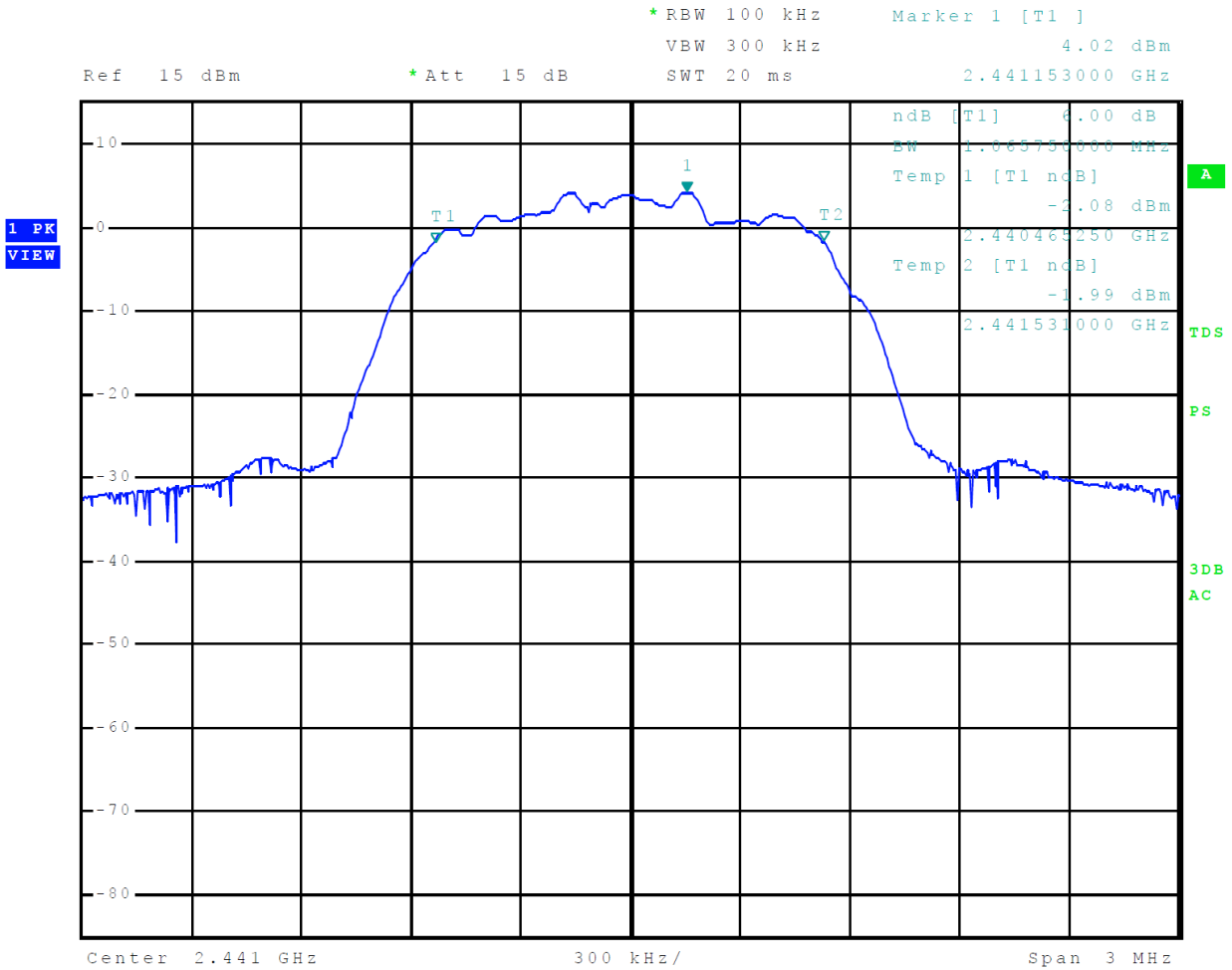
Figure 25 Plot of 6-dB Occupied Bandwidth Mode 4, BT 3EDR (8DPSK)
