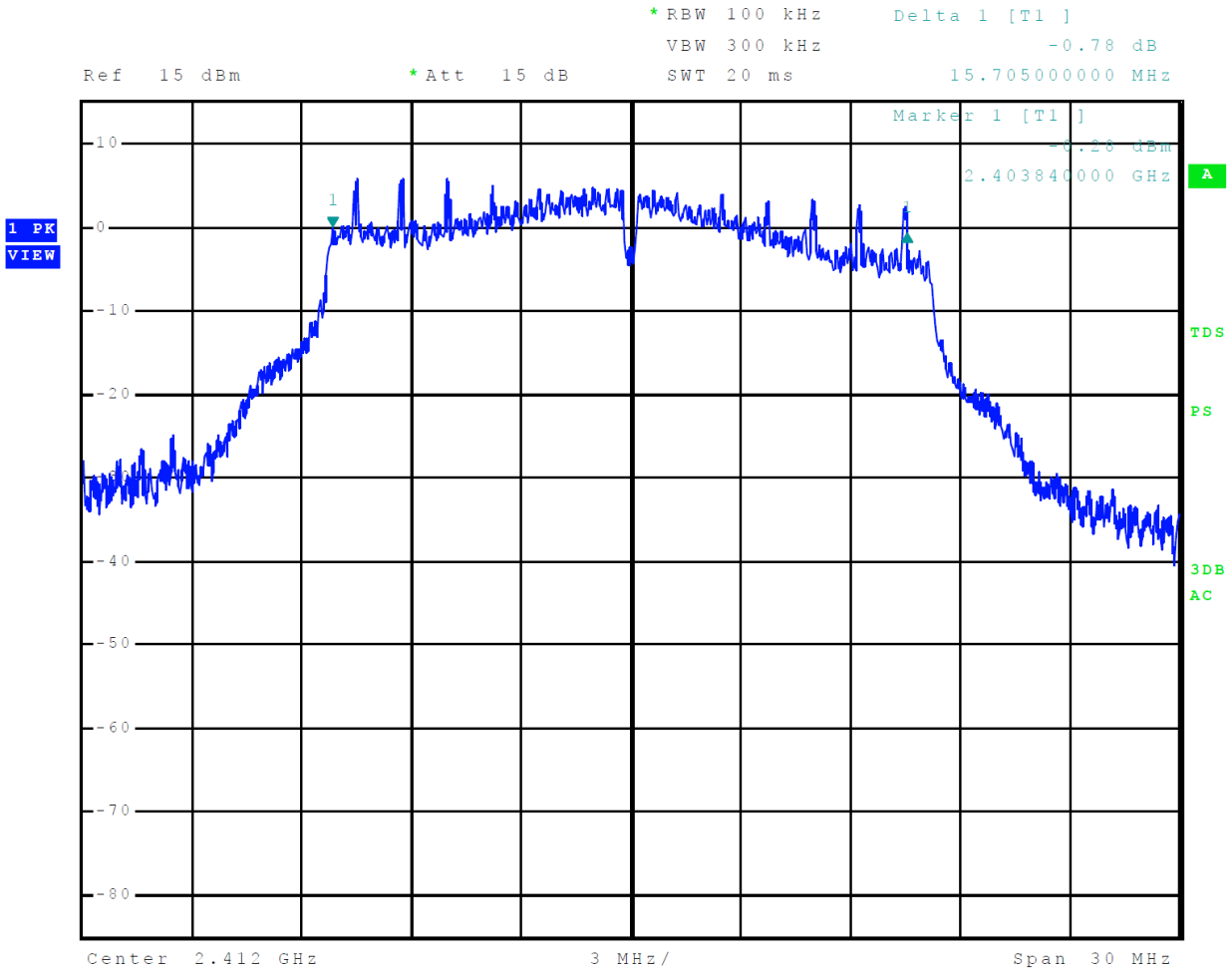
Figure 32 Plot of 99% Occupied Bandwidth Mode 7, 802.11g (OFDM)
