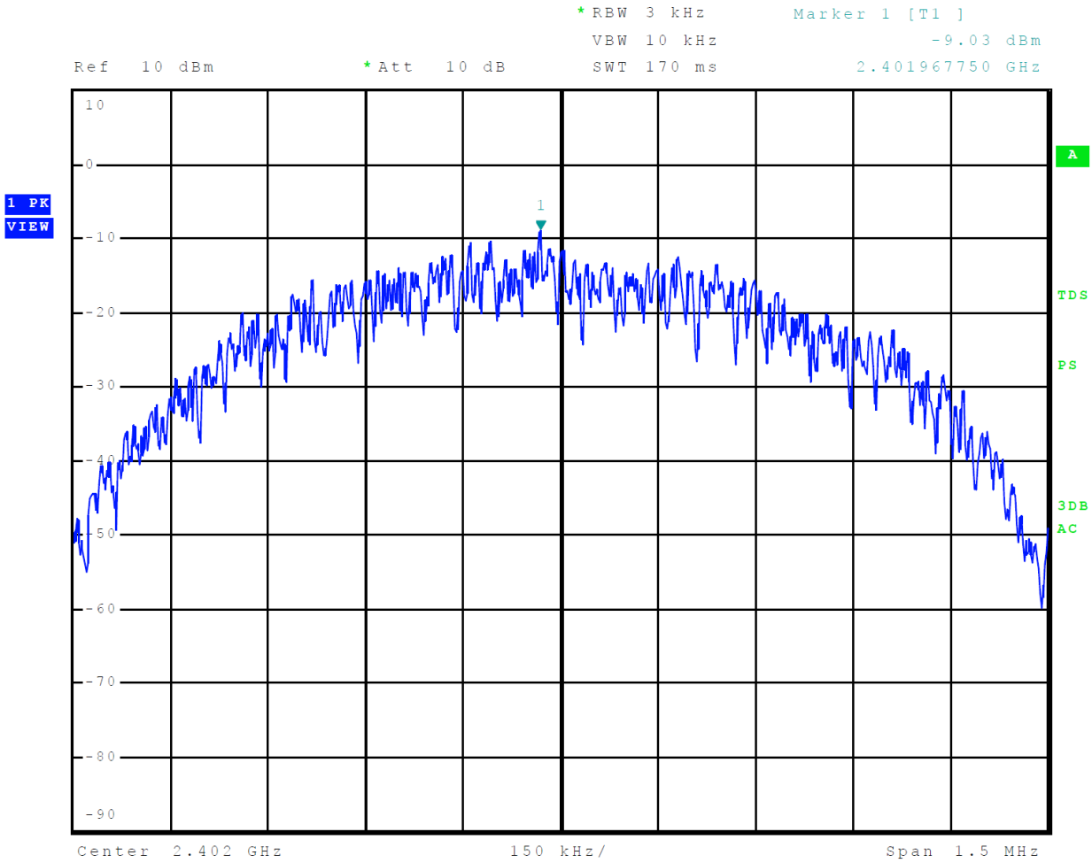
Figure 37 Plot of Transmitter Power Spectral Density Mode 5, BT BLE (GMSK)
