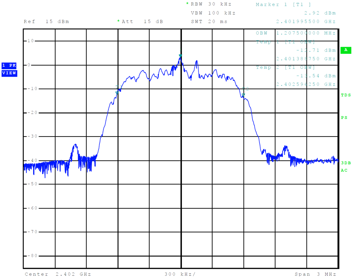
Figure 24 Plot of Transmitter 99% Occupied Bandwidth Mode 3, BT 2EDR ( \pi/4 -DQPSK)
