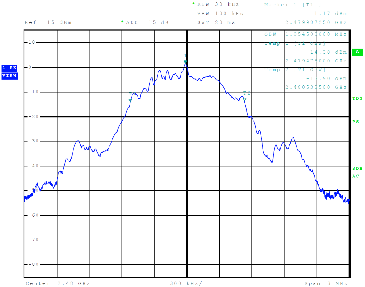
Figure 28 Plot of Transmitter 99% Occupied Bandwidth Mode 5, BT BLE (GMSK)
