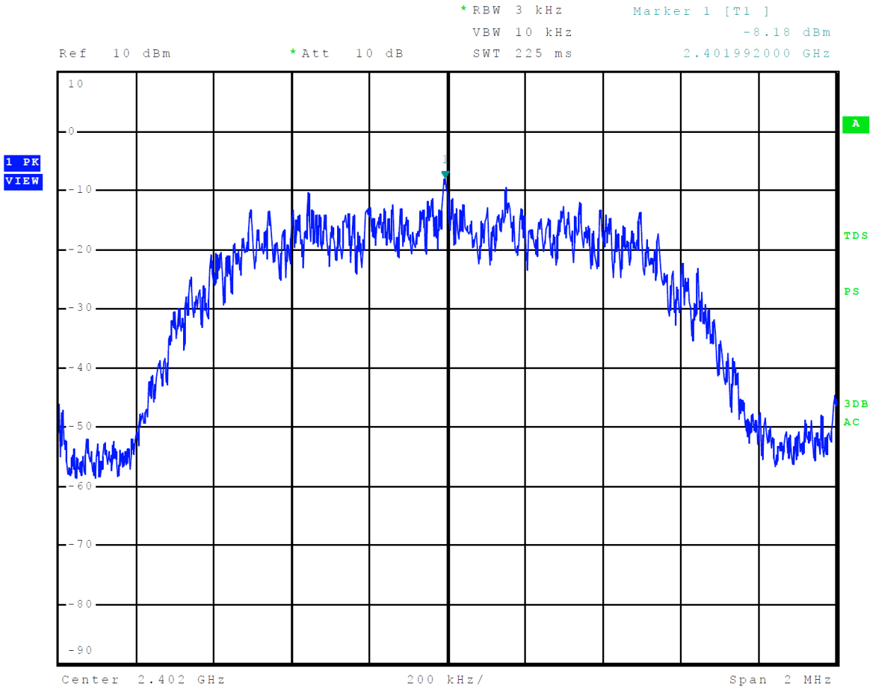
Figure 35 Plot of Transmitter Power Spectral Density Mode 3, BT 2EDR ( \pi/4 -DQPSK)
