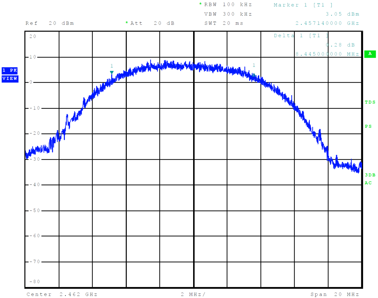
Figure 29 Plot of 6-dB Occupied Bandwidth Mode 6, 802.11b (DSSS/CCK)
