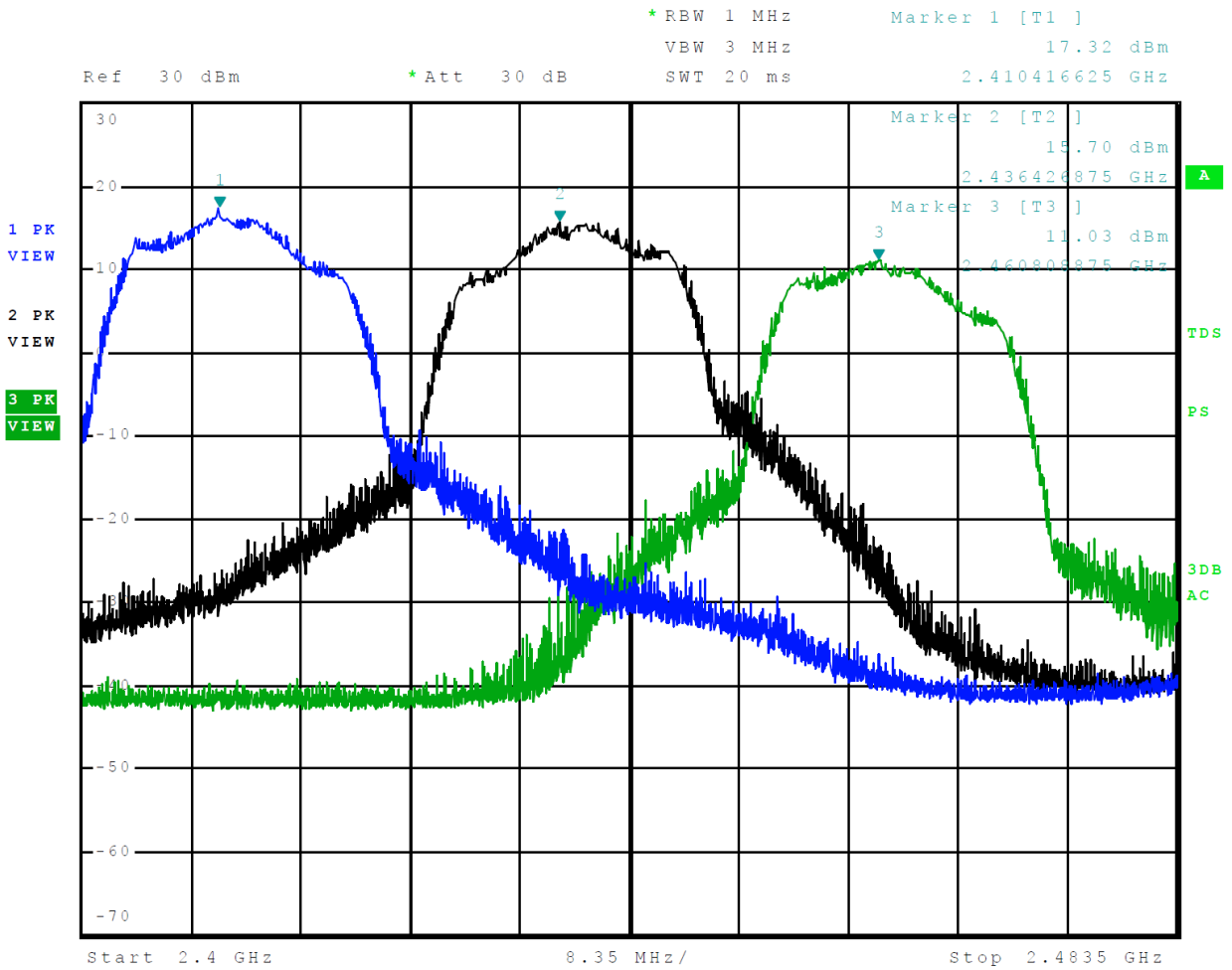
Figure 10 Plot of Transmitter Operation in 2412-2462 MHz Mode 8, 802.11n (MSC)
