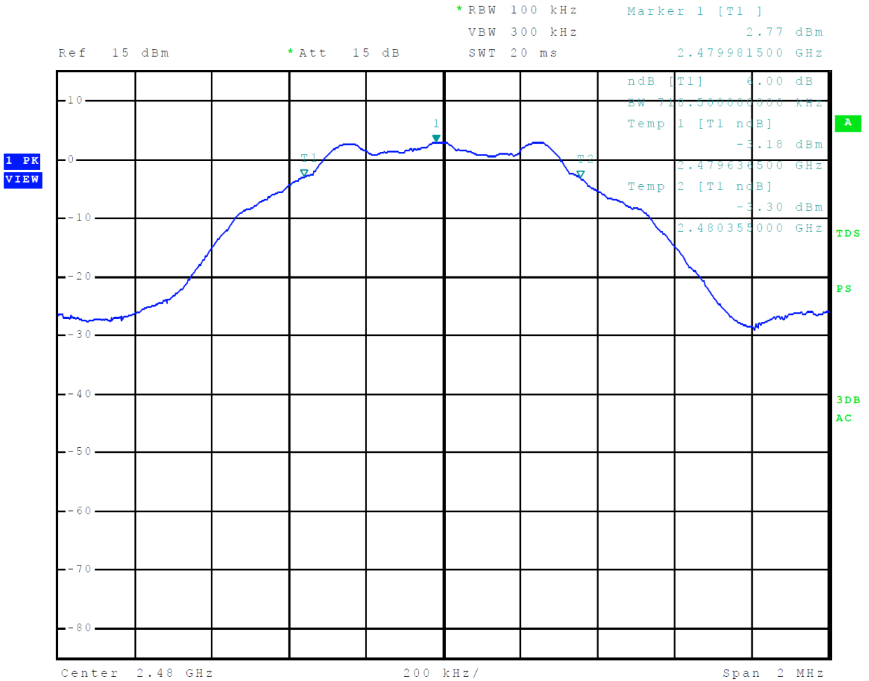
Figure 27 Plot of 6-dB Occupied Bandwidth Mode 5, BT BLE (GMSK)
