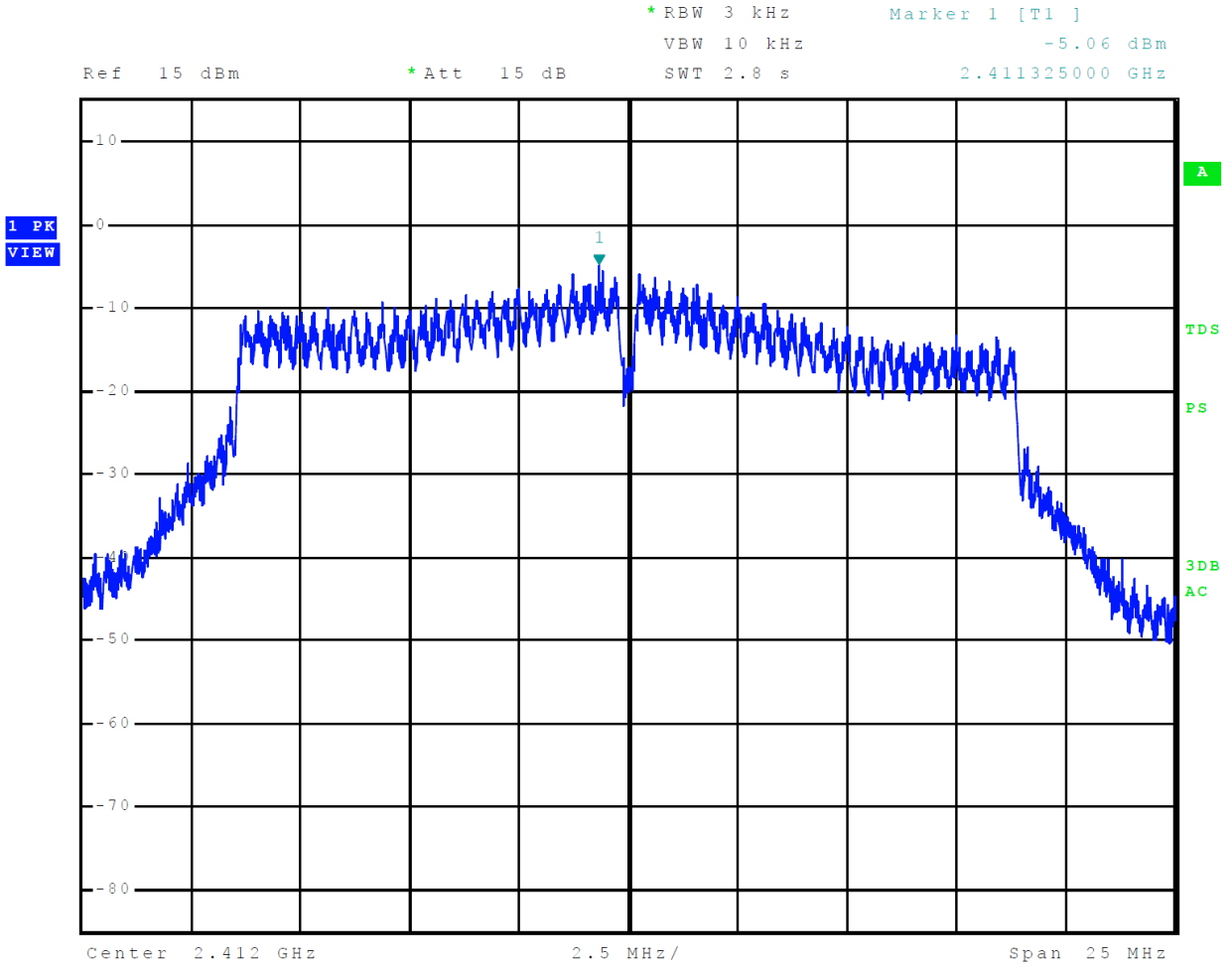
Figure 40 Plot of Transmitter Power Spectral Density Mode 8, 802.11n (MSC)
