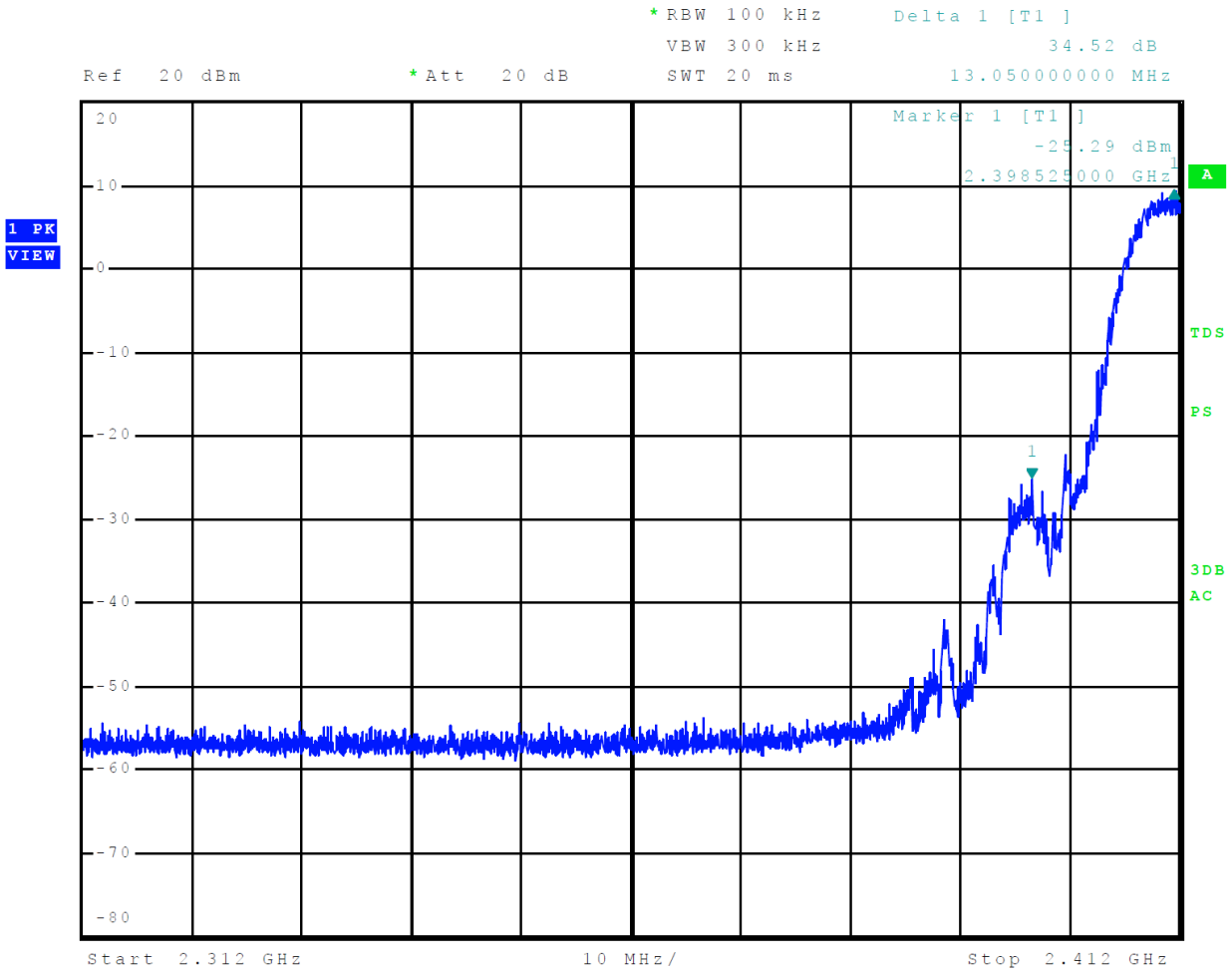
Figure 14 Plot of Transmitter Emissions Low Band Edge Mode 6, 802.11b (DSSS/CCK)
