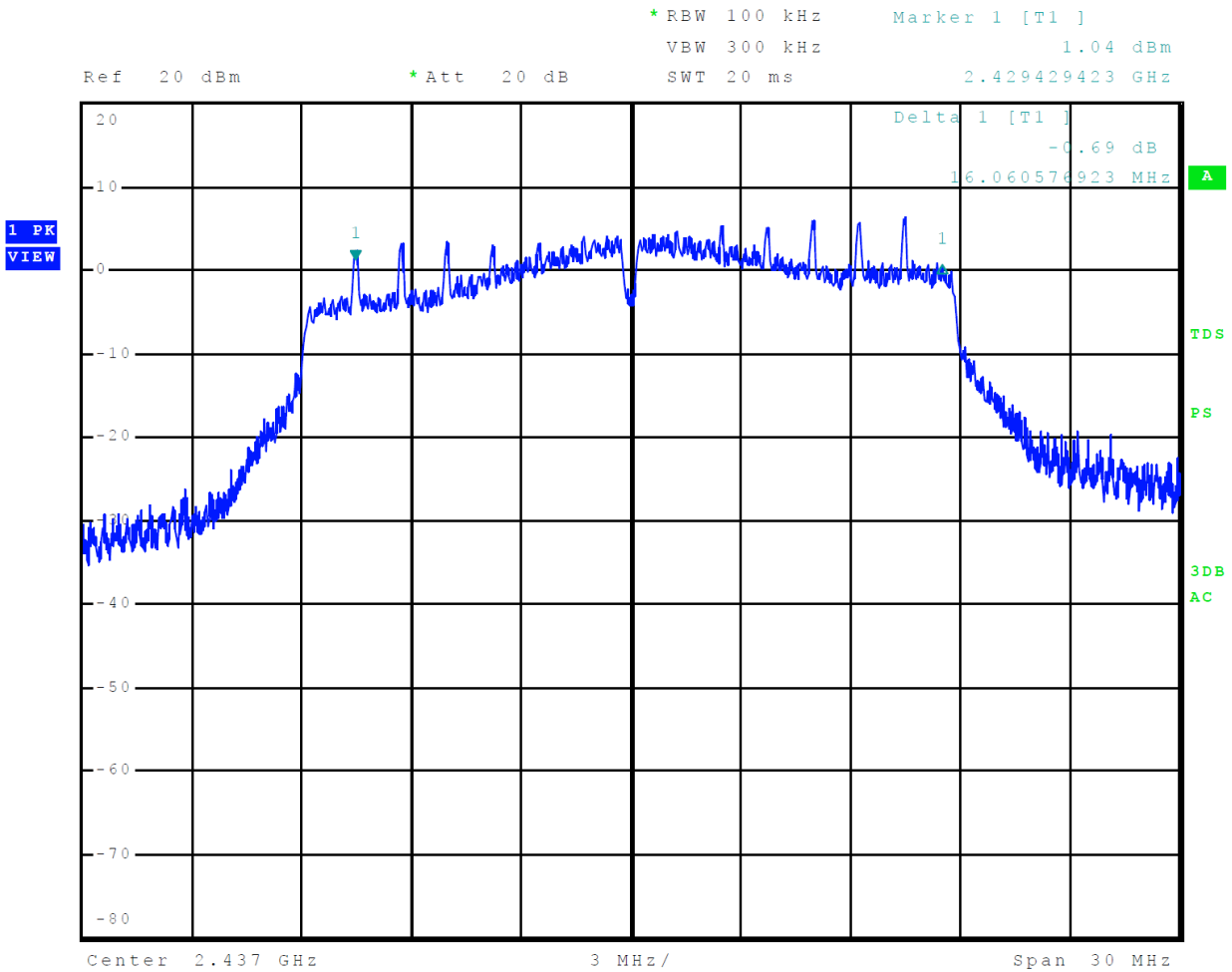
Figure 33 Plot of 6-dB Occupied Bandwidth Mode 8, 802.11n (MSC)
