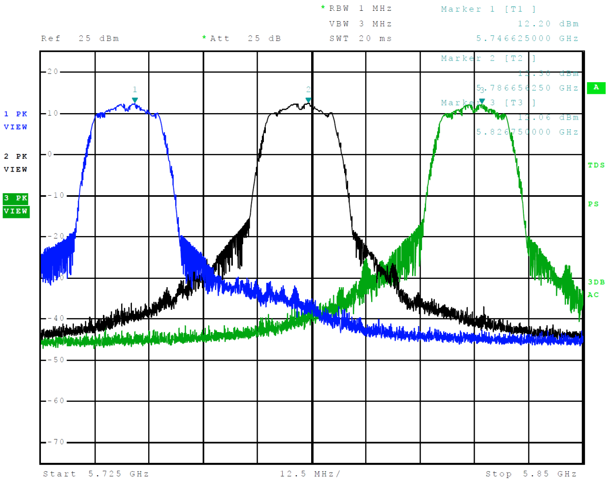
Figure 20 Plot of Transmitter Emissions Across 5725-5850 MHz Mode 12, U-NII-3 (802.11a)
