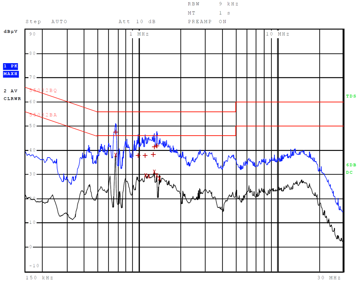
Figure 2 AC Line Conducted emissions of EUT Configuration #2 line 2 (EUT – AC Adapter)
