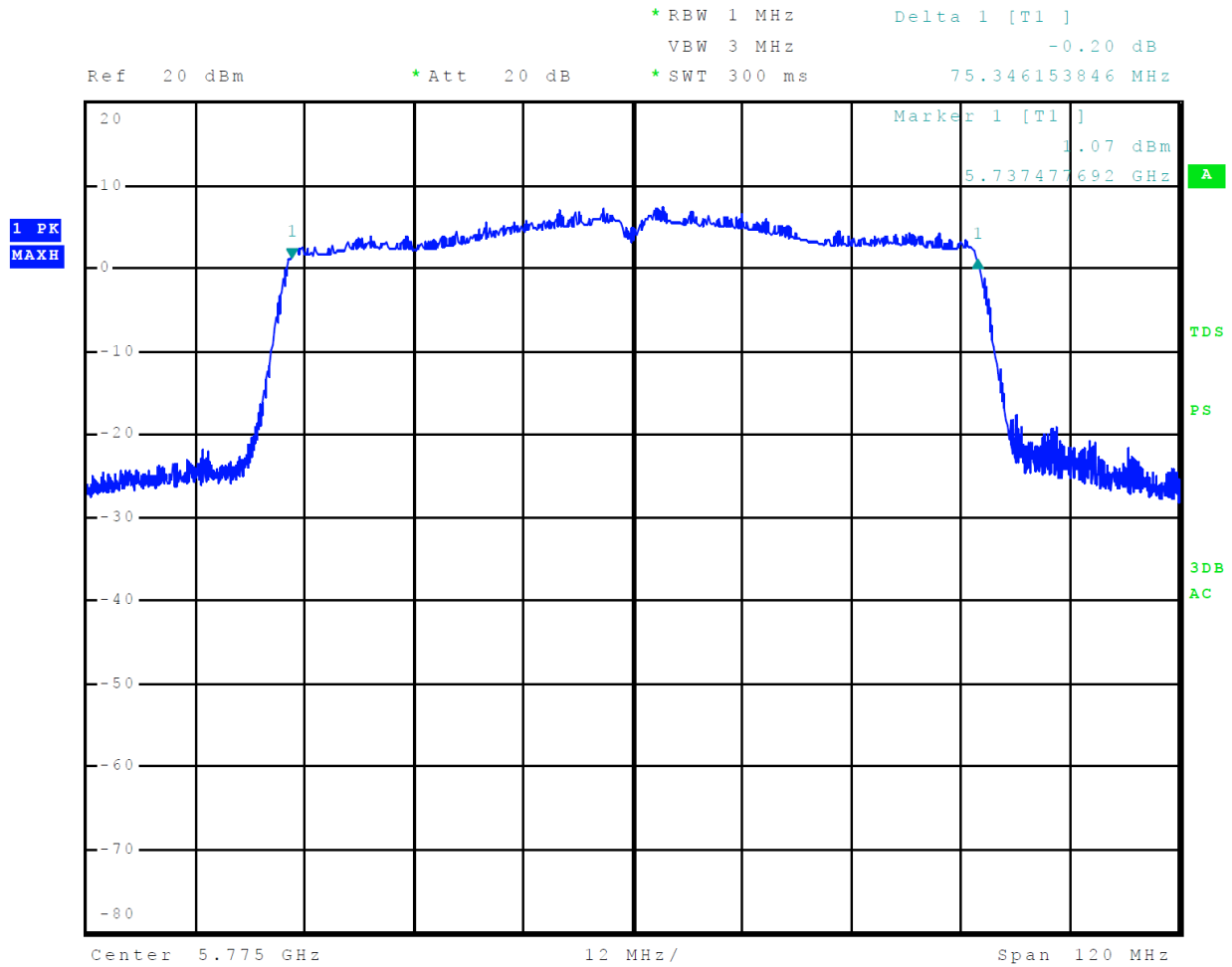
Figure 47 Plot of 6-dB Occupied Bandwidth 5725-5850 MHz Mode 12, U-NII-3 (802.11a)
