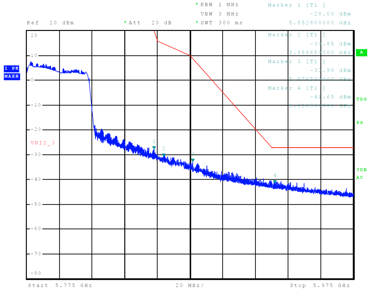
Figure 45 Plot of Upper Band Edge Across 5725-5850 MHz Mode 12, U-NII-3 (802.11a)
