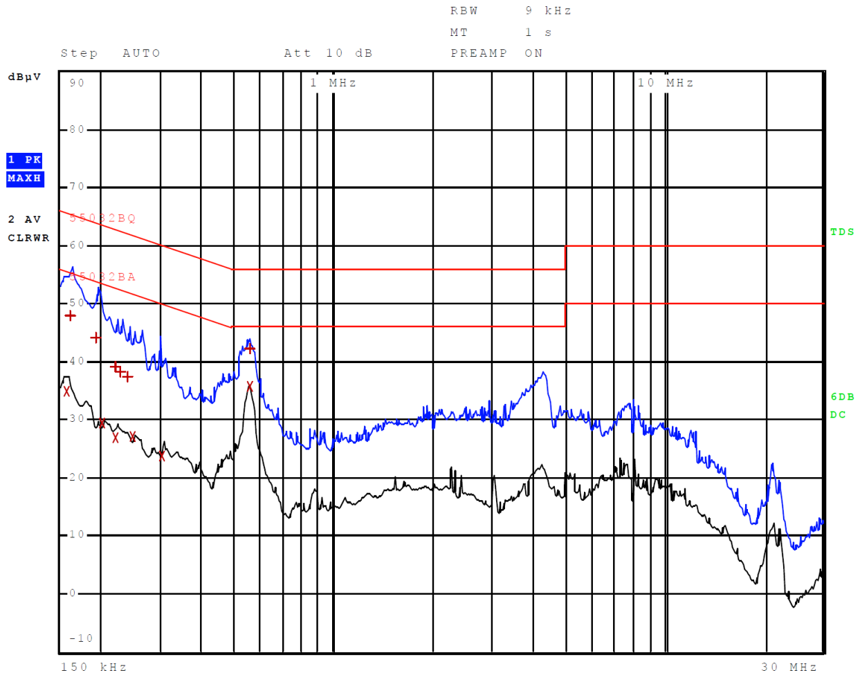
Figure 4 AC Line Conducted emissions of EUT Configuration #3 line 2 (EUT – CPU)
