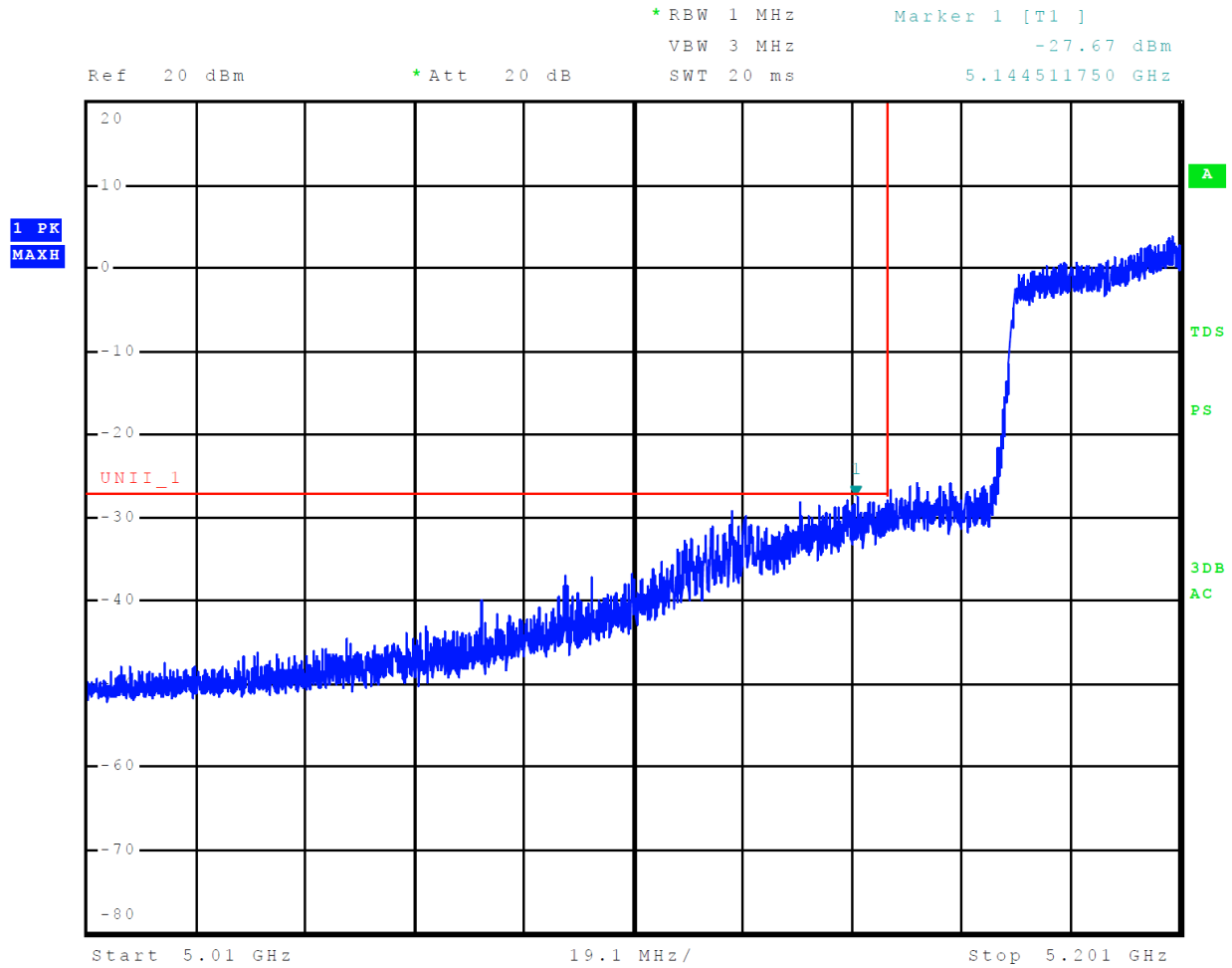
Figure 39 Plot of Lower Band Edge Across 5150-5250 MHz Mode 9, U-NII-1 (802.11a)
