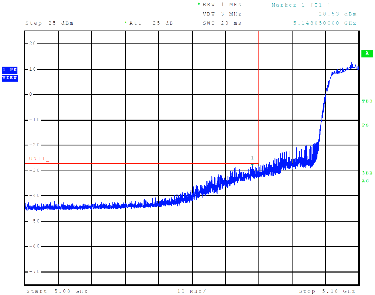
Figure 9 Plot of Lower Band Edge Across 5150-5250 MHz Mode 10, U-NII-1 (802.11n)
