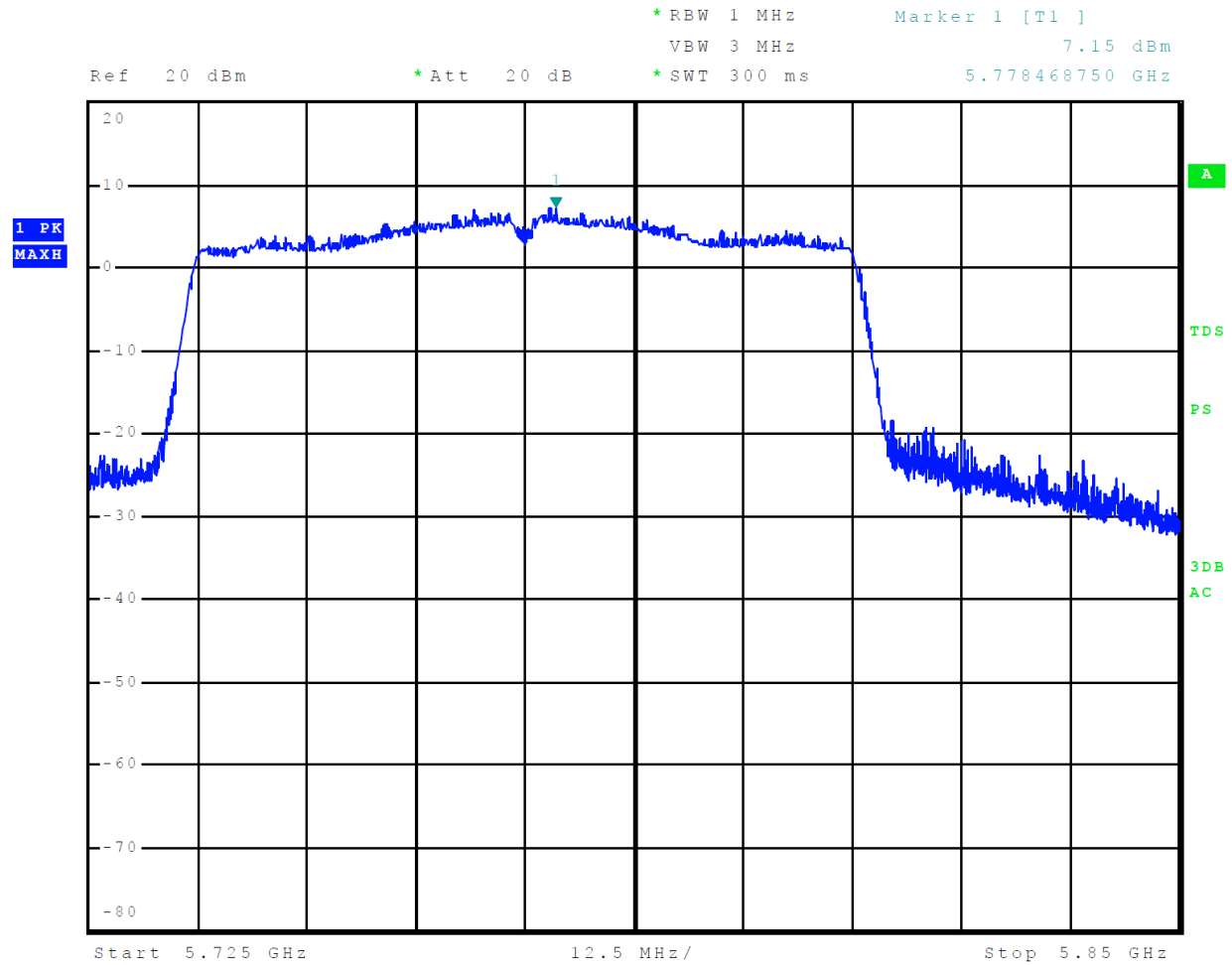
Figure 43 Plot of Transmitter Emissions Across 5725-5850 MHz Mode 12, U-NII-3 (802.11a)
