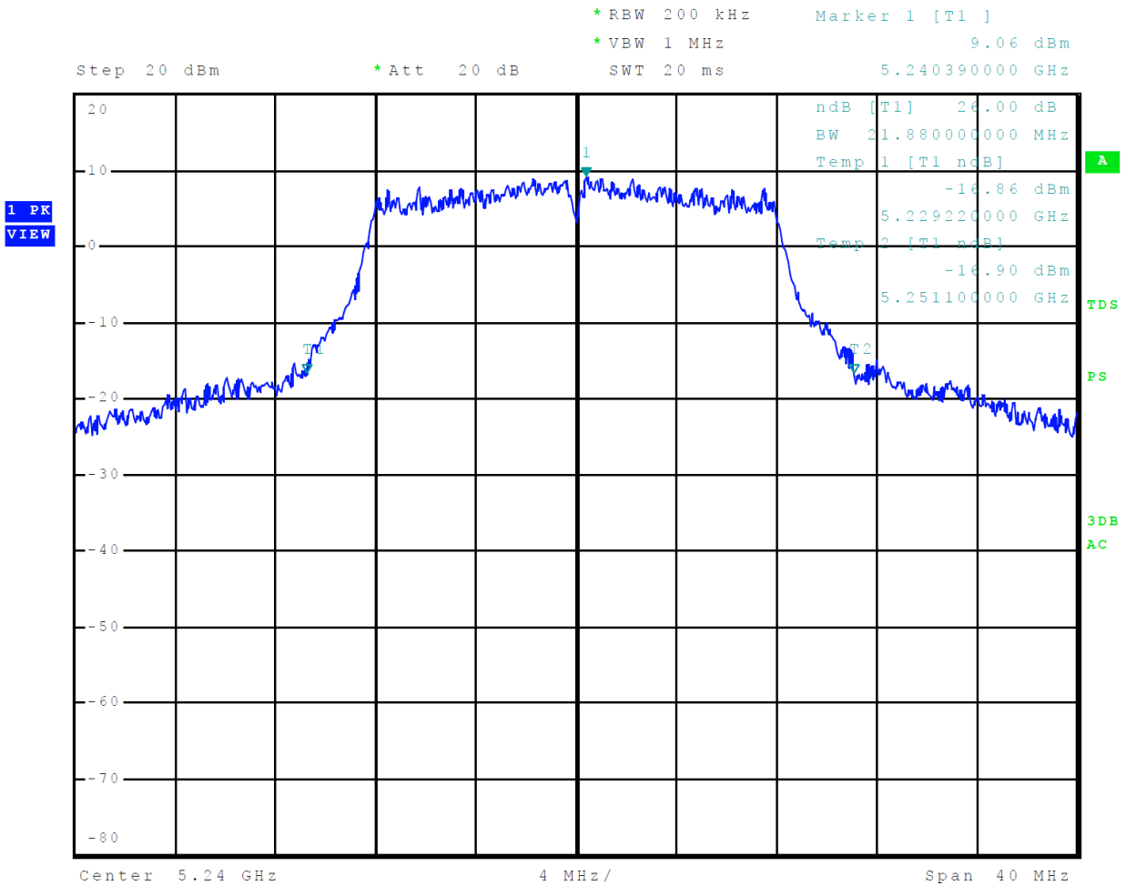
Figure 14 Plot of 26-dB Occupied Bandwidth 5150-5250 MHz Mode 9, U-NII-1 (802.11a)
