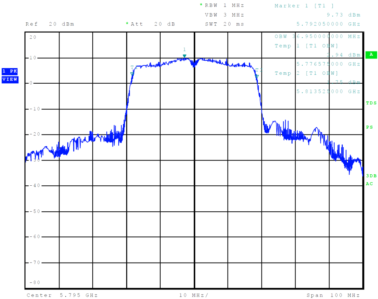
Figure 31 Plot of 99% Occupied Bandwidth 5725-5850 MHz Mode 14, U-NII-3 (802.11n40)
