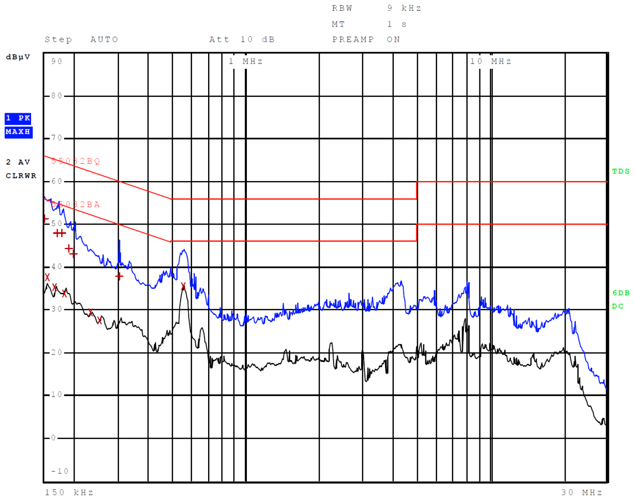
Figure 3 AC Line Conducted emissions of EUT Configuration #3 line 1 (EUT – CPU)
