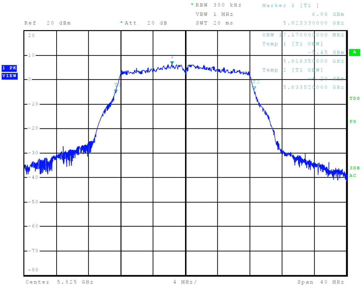
Figure 29 Plot of 99% Occupied Bandwidth 5725-5850 MHz Mode 12, U-NII-3 (802.11a)
