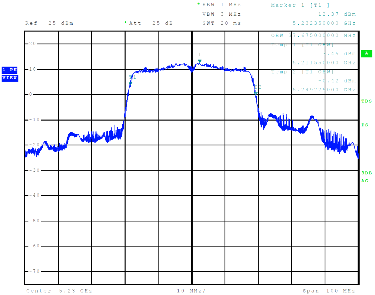
Figure 19 Plot of 99% Occupied Bandwidth 5150-5250 MHz Mode 11, U-NII-1 (802.11n40)
