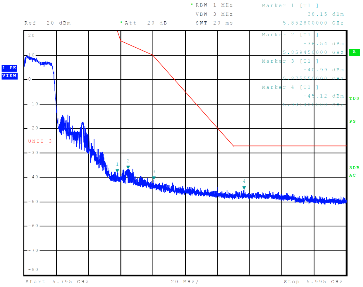
Figure 28 Plot of Upper Band Edge Across 5725-5850 MHz Mode 14, U-NII-3 (802.11n40)
