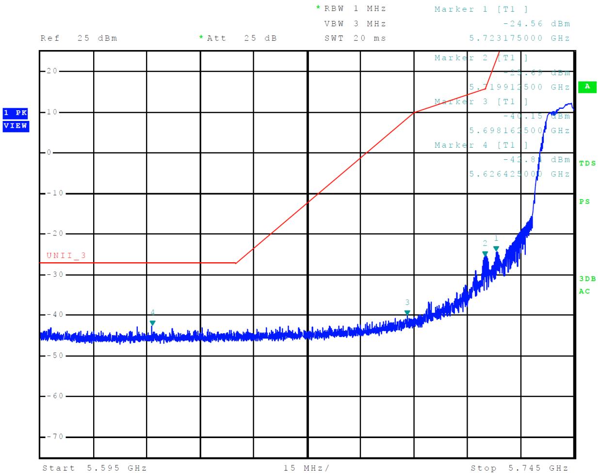
Figure 23 Plot of Lower Band Edge Across 5725-5850 MHz Mode 12, U-NII-3 (802.11a)
