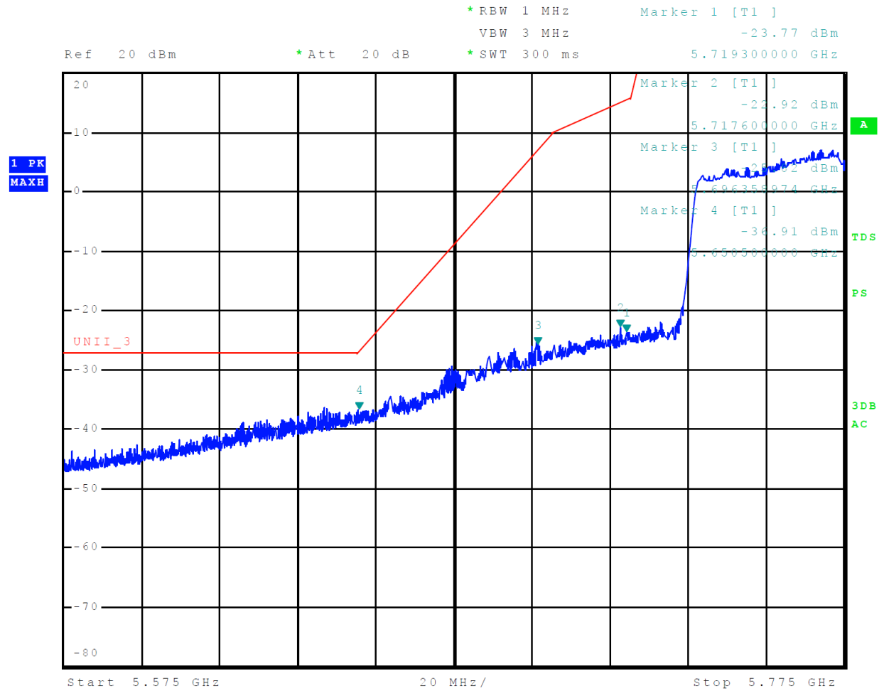
Figure 44 Plot of Lower Band Edge Across 5725-5850 MHz Mode 12, U-NII-3 (802.11a)
