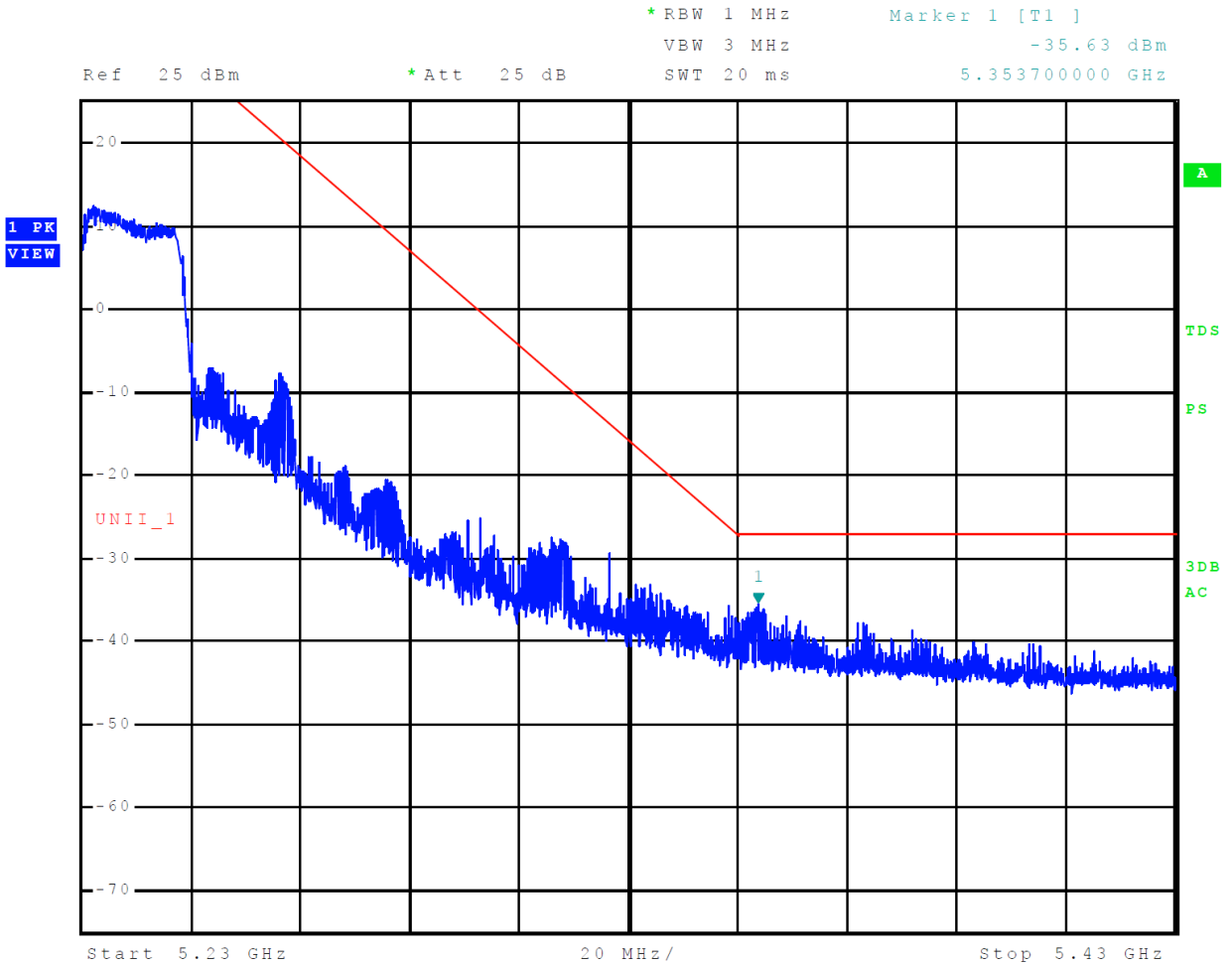
Figure 13 Plot of Upper Band Edge Across 5150-5250 MHz Mode 11, U-NII-1 (802.11n40)
