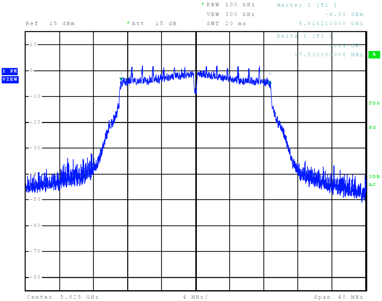
Figure 33 Plot of 6-dB Occupied Bandwidth 5725-5850 MHz Mode 13, U-NII-3 (802.11n)
