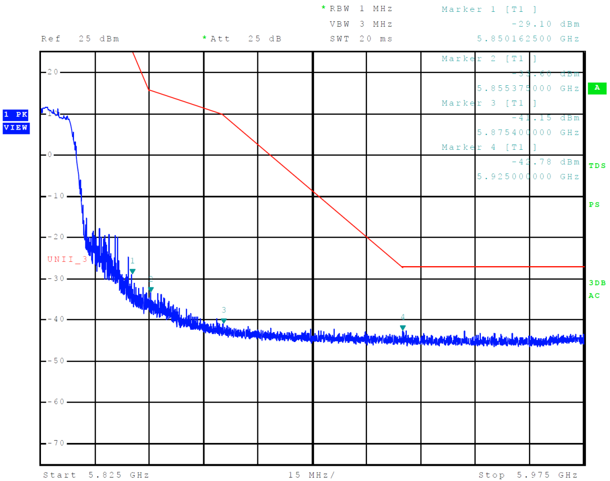
Figure 27 Plot of Upper Band Edge Across 5725-5850 MHz Mode 13, U-NII-3 (802.11n)
