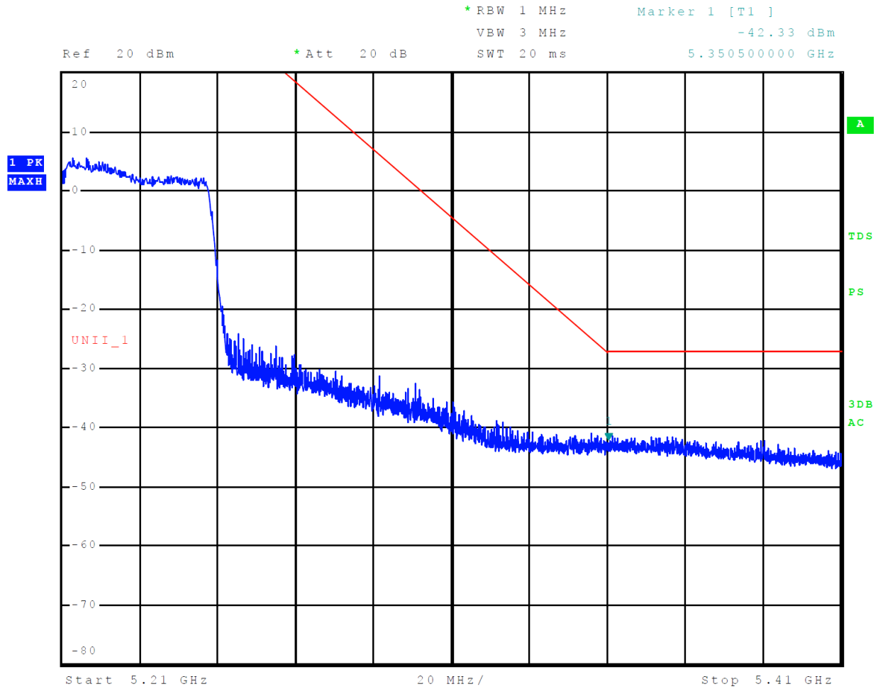
Figure 40 Plot of Upper Band Edge Across 5150-5250 MHz Mode 9, U-NII-1 (802.11a)
