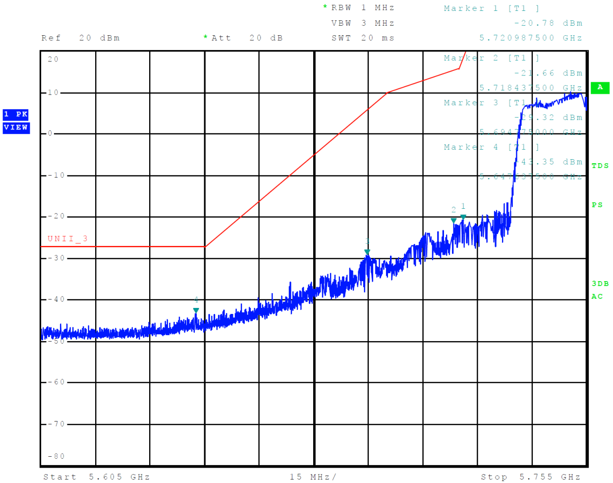
Figure 25 Plot of Lower Band Edge Across 5725-5850 MHz Mode 14, U-NII-3 (802.11n40)
