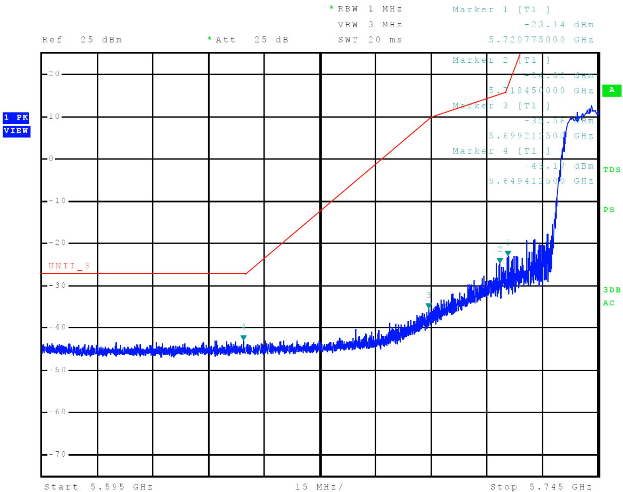
Figure 24 Plot of Lower Band Edge Across 5725-5850 MHz Mode 13, U-NII-3 (802.11n)
