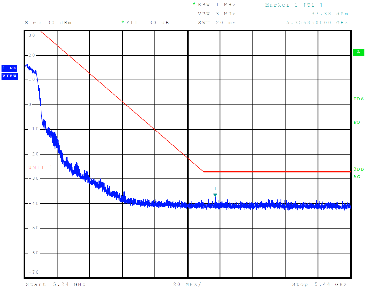
Figure11 Plot of Upper Band Edge Across 5150-5250 MHz Mode 9, U-NII-1 (802.11a)
