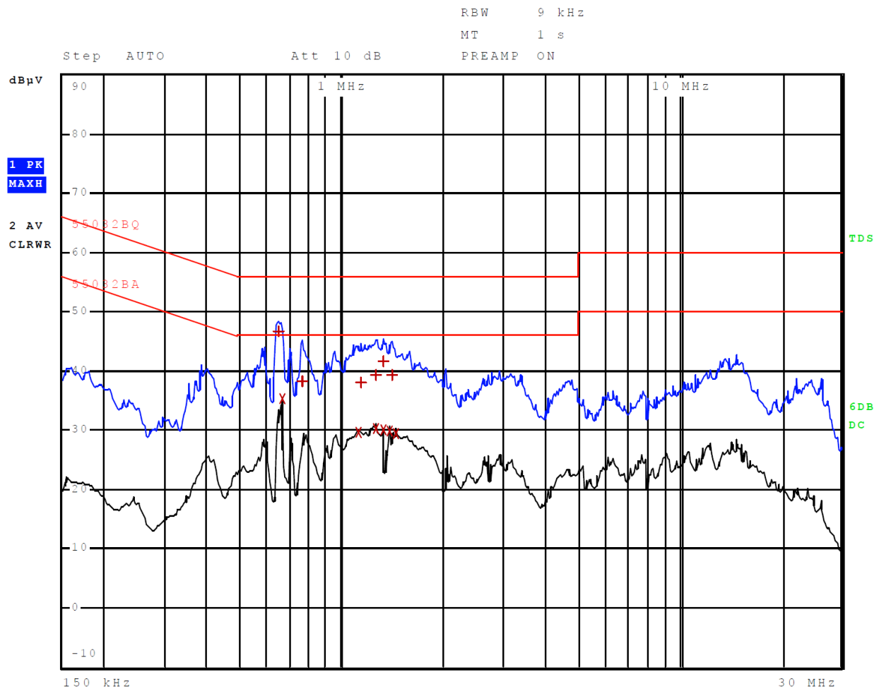
Figure 1 AC Line Conducted emissions of EUT Configuration #2 line 1 (EUT – AC Adapter)
