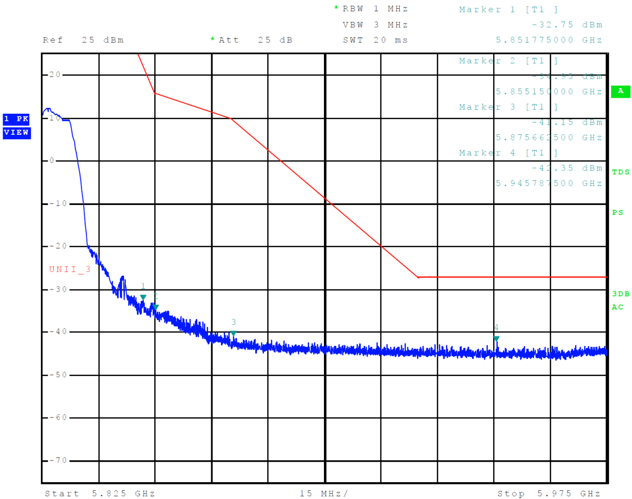
Figure 26 Plot of Upper Band Edge Across 5725-5850 MHz Mode 12, U-NII-3 (802.11a)
