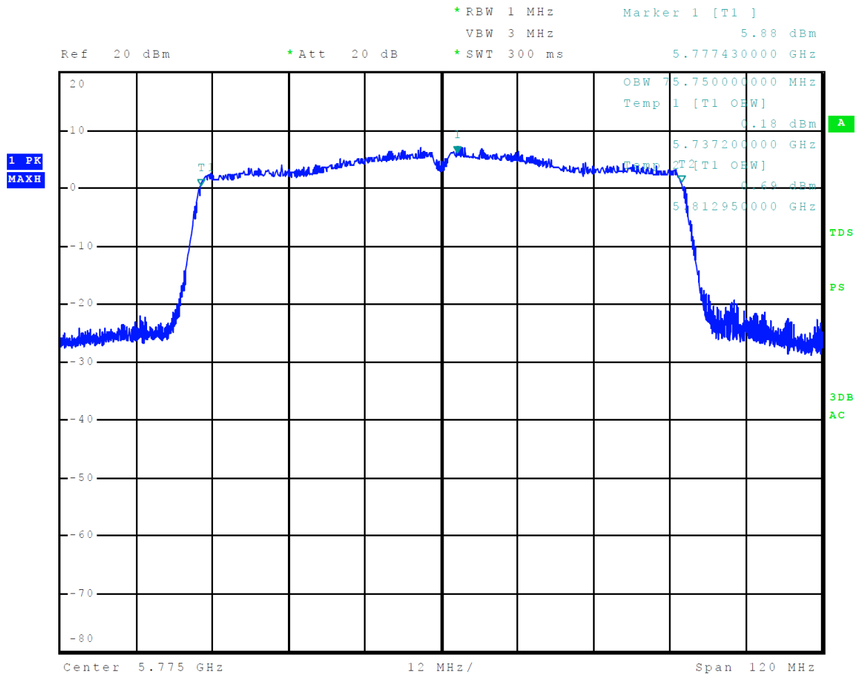
Figure 46 Plot of 99% Occupied Bandwidth 5725-5850 MHz Mode 12, U-NII-3 (802.11a)
