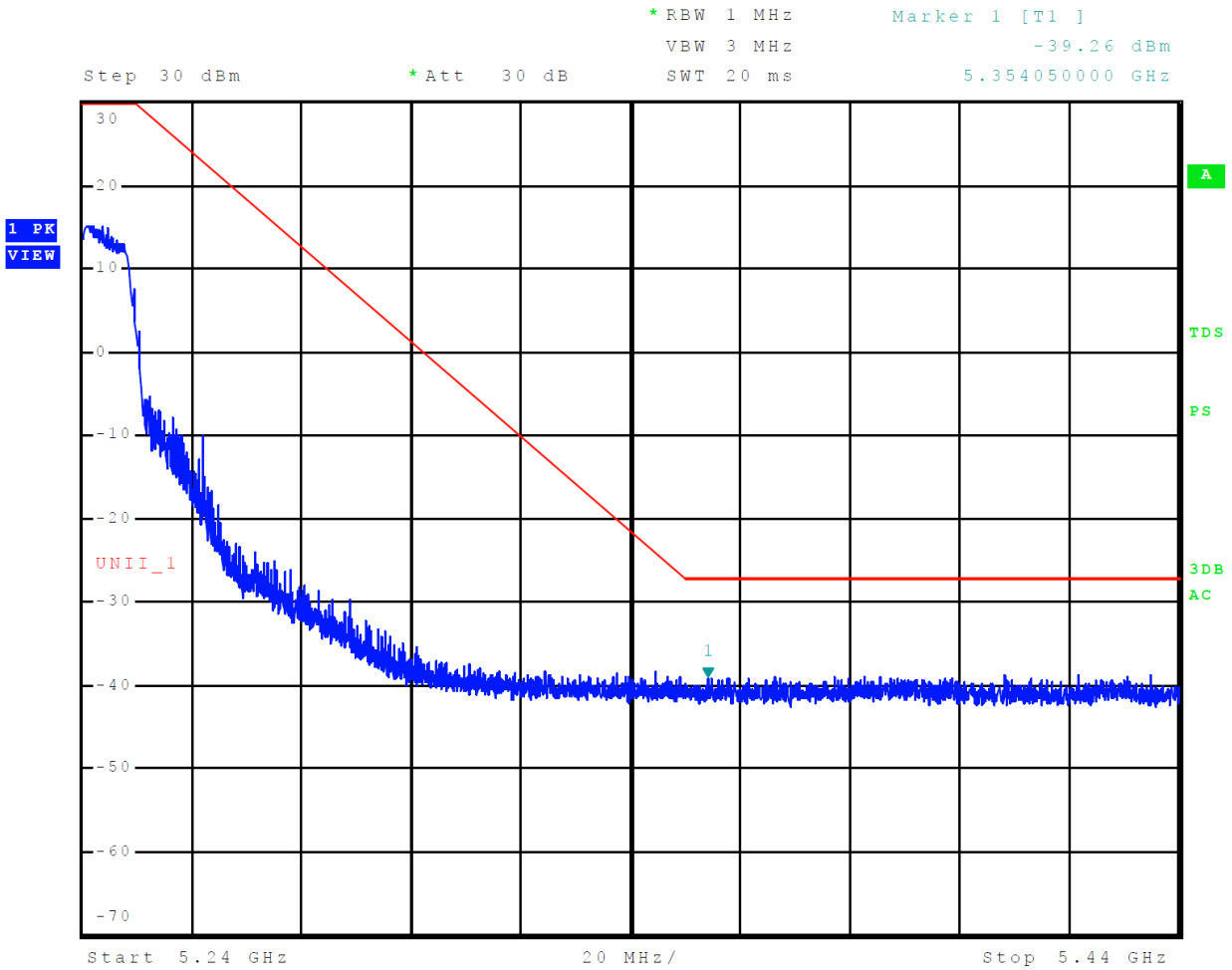
Figure 12 Plot of Upper Band Edge Across 5150-5250 MHz Mode 10, U-NII-1 (802.11n)
