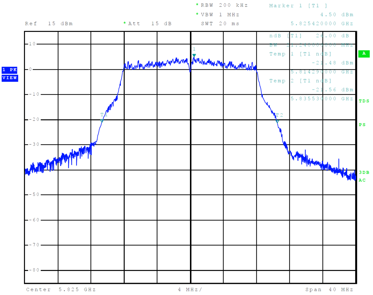
Figure 35 Plot of 26-dB Occupied Bandwidth 5725-5850 MHz Mode 12, U-NII-3 (802.11a)
