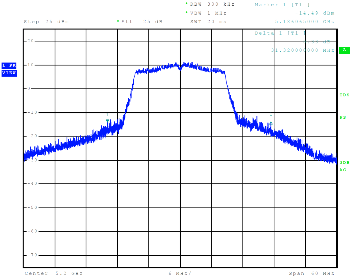
Figure 15 Plot of 26-dB Occupied Bandwidth 5150-5250 MHz Mode 10, U-NII-1 (802.11n)
