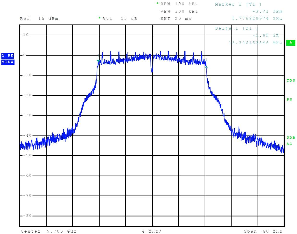
Figure 32 Plot of 6-dB Occupied Bandwidth 5725-5850 MHz Mode 12, U-NII-3 (802.11a)
