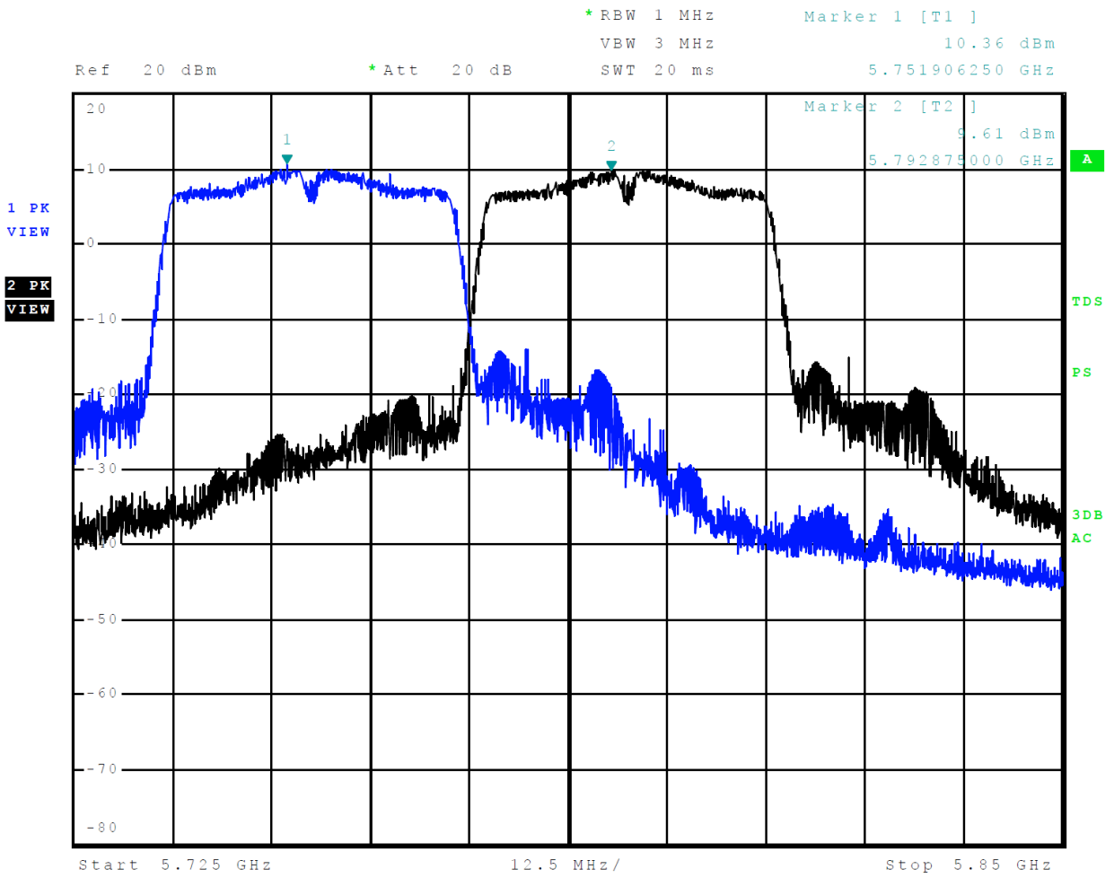
Figure 22 Plot of Transmitter Emissions Across 5725-5850 MHz Mode 14, U-NII-3 (802.11n40)
