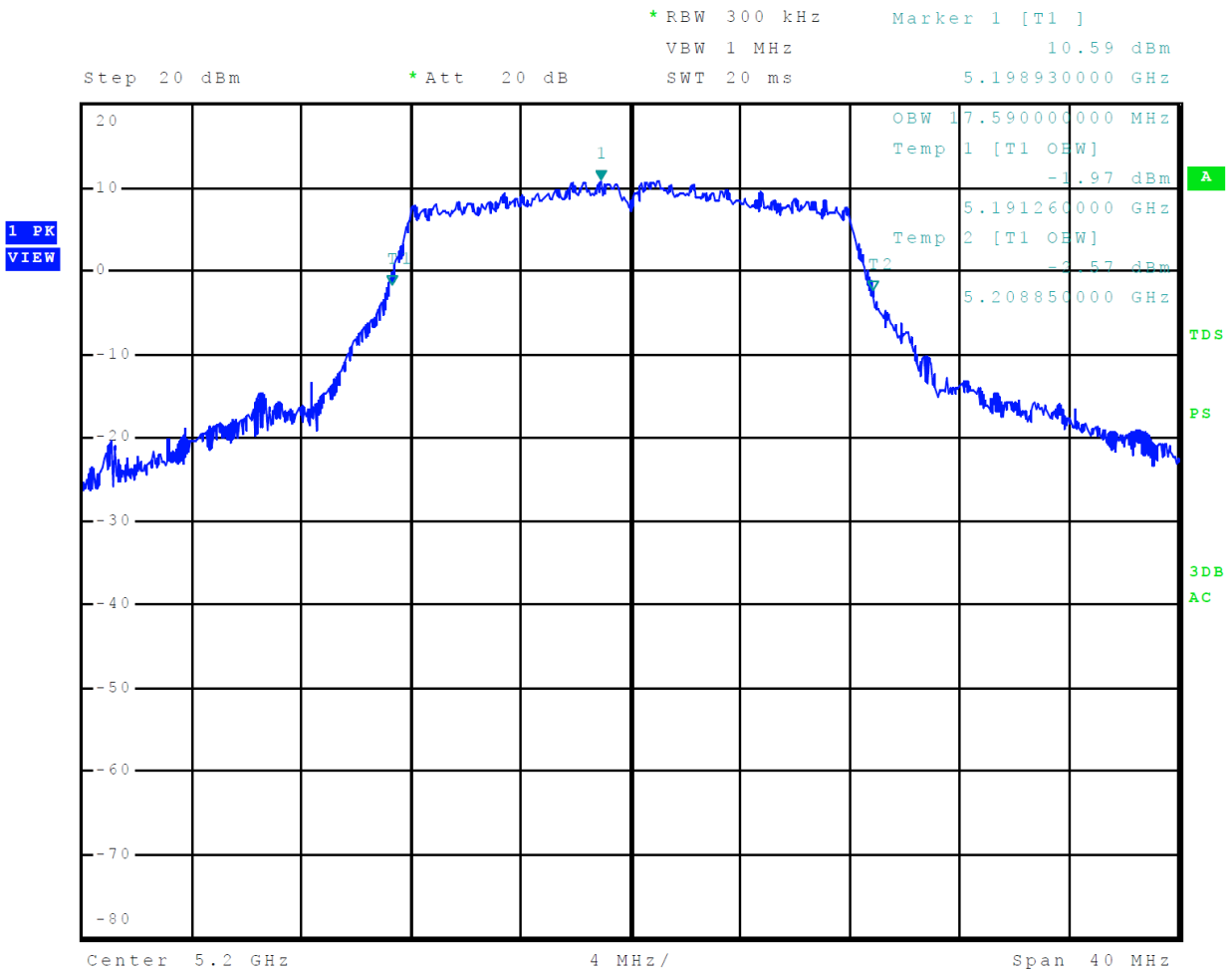
Figure 17 Plot of 99% Occupied Bandwidth 5150-5250 MHz Mode 9, U-NII-1 (802.11a)
