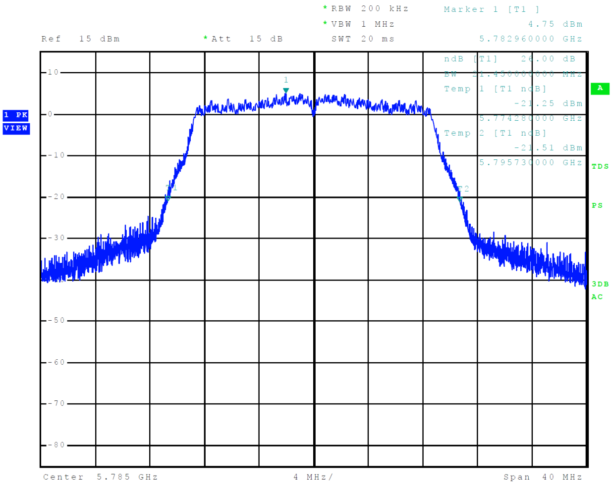
Figure 36 Plot of 26-dB Occupied Bandwidth 5725-5850 MHz Mode 13, U-NII-3 (802.11n)
