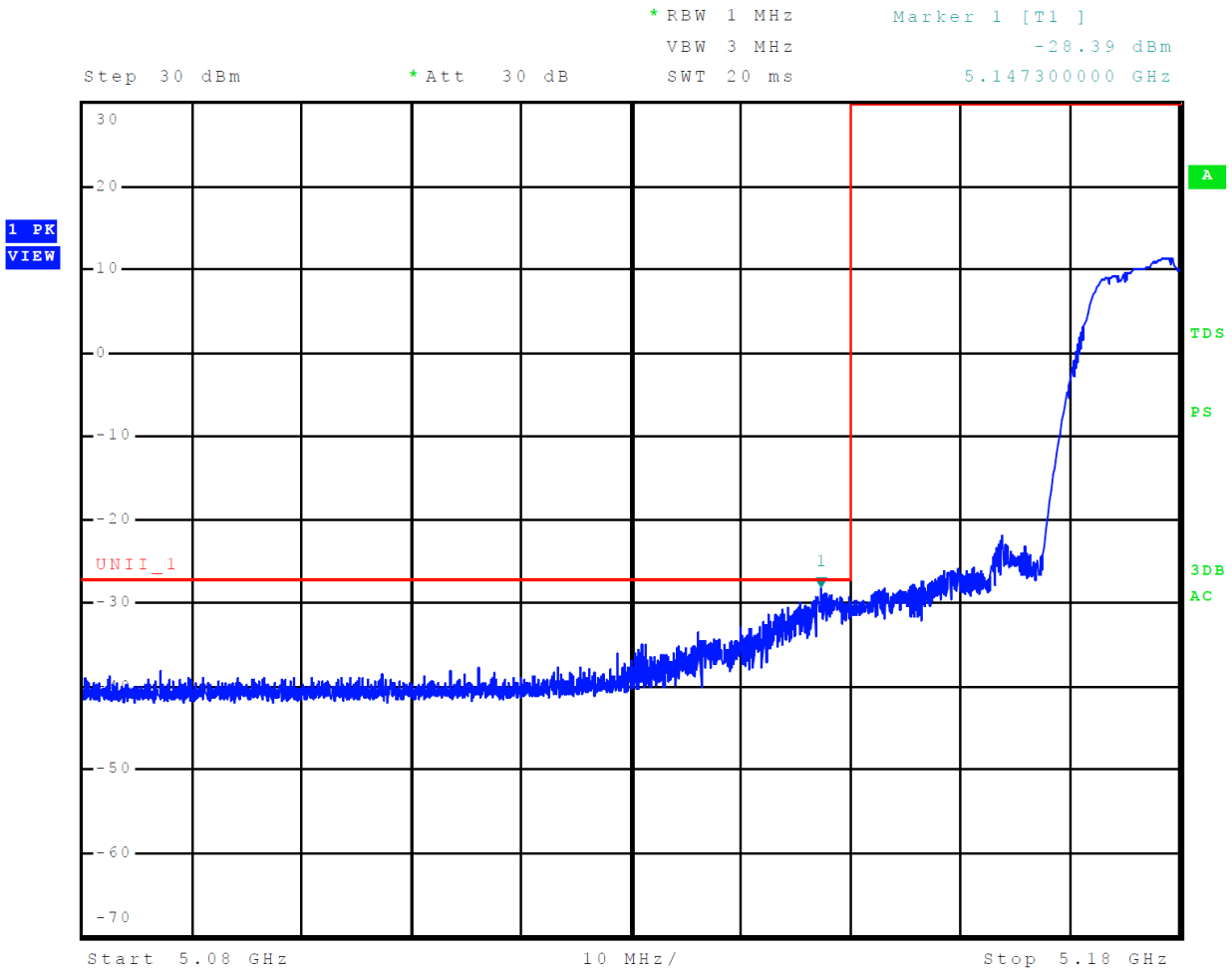
Figure 8 Plot of Lower Band Edge Across 5150-5250 MHz Mode 9, U-NII-1 (802.11a)
