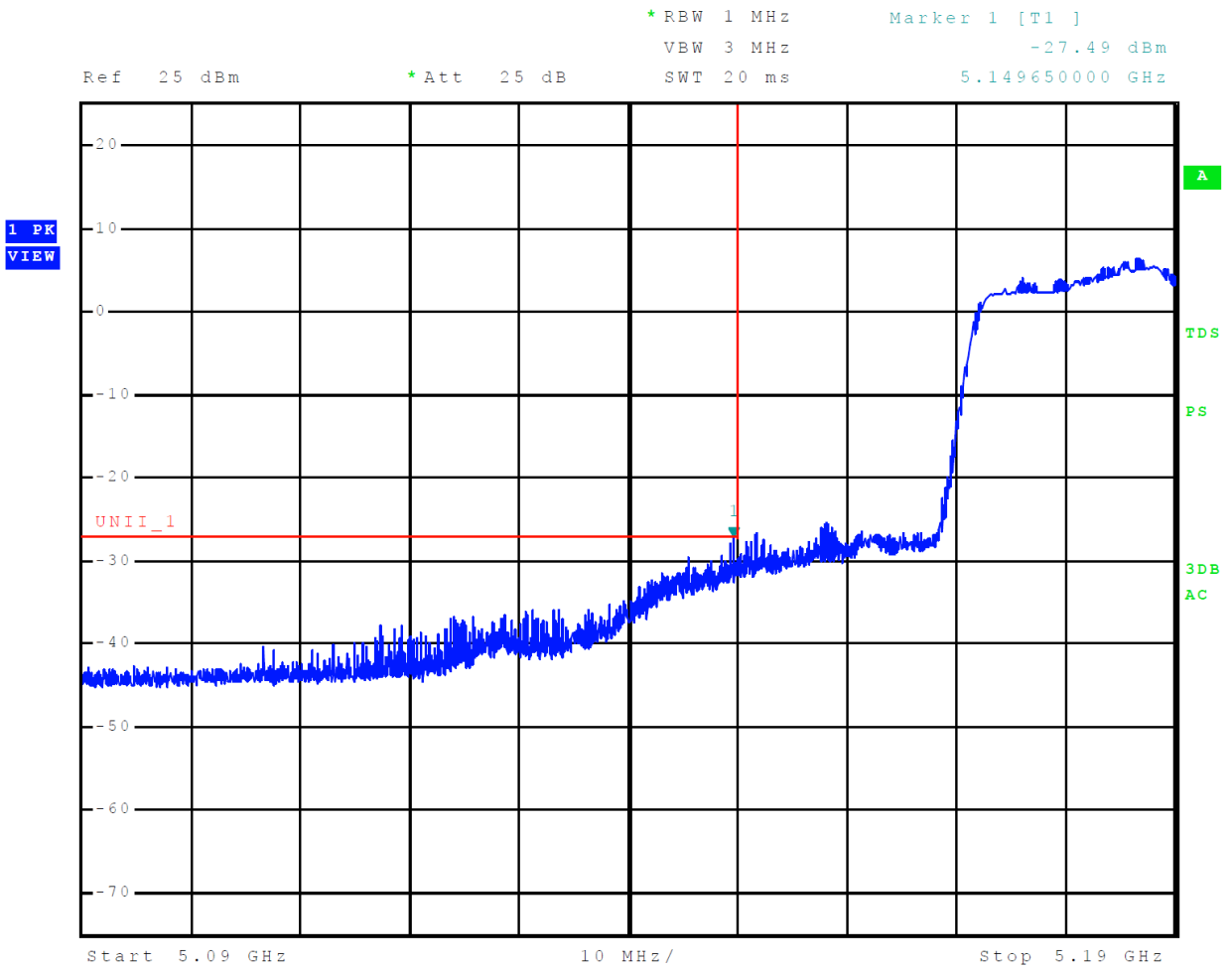
Figure 10 Plot of Lower Band Edge Across 5150-5250 MHz Mode 11, U-NII-1 (802.11n40)
