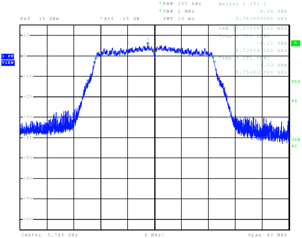
Figure 30 Plot of 99% Occupied Bandwidth 5725-5850 MHz Mode 13, U-NII-3 (802.11n)
