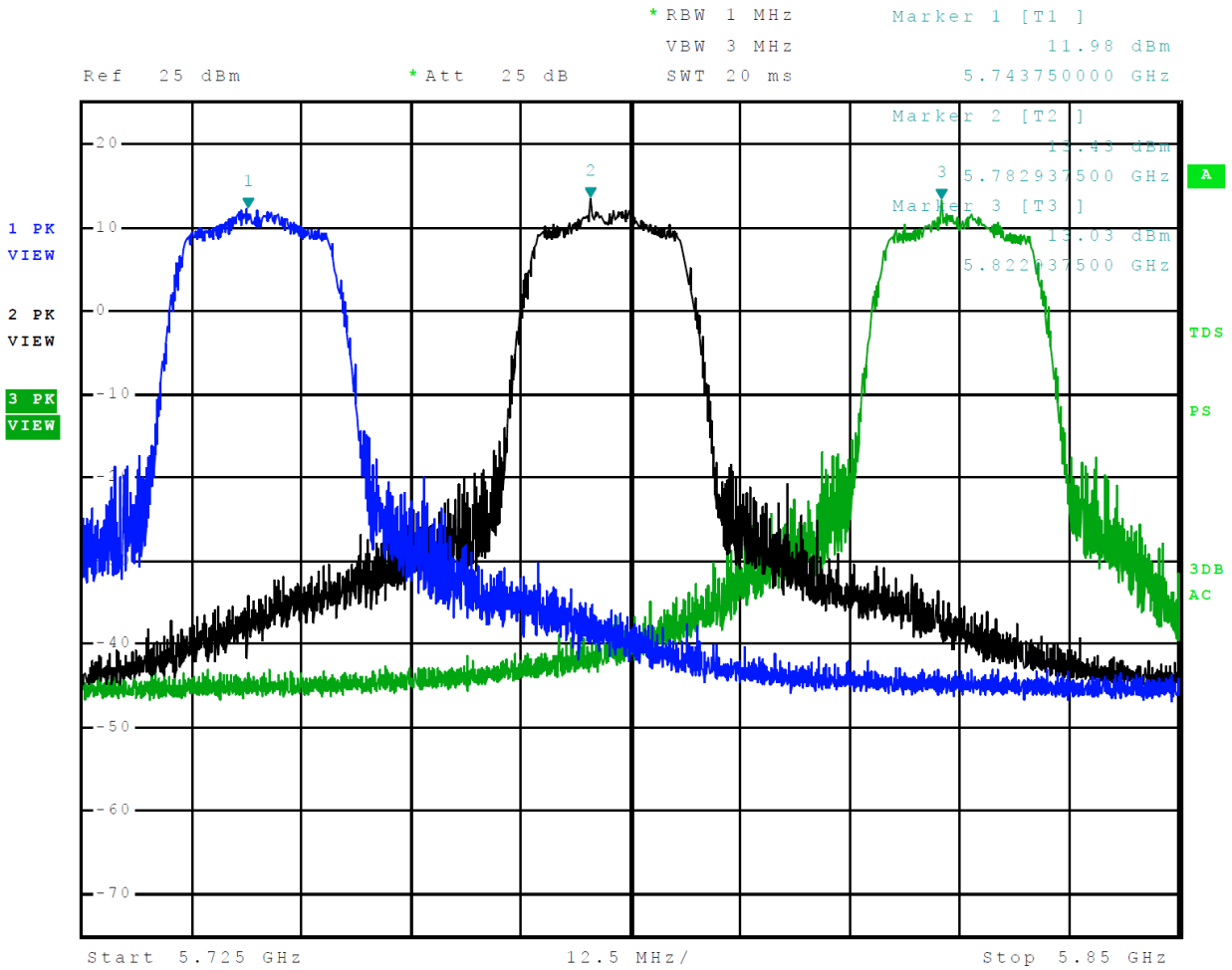
Figure 21 Plot of Transmitter Emissions Across 5725-5850 MHz Mode 13, U-NII-3 (802.11n)
