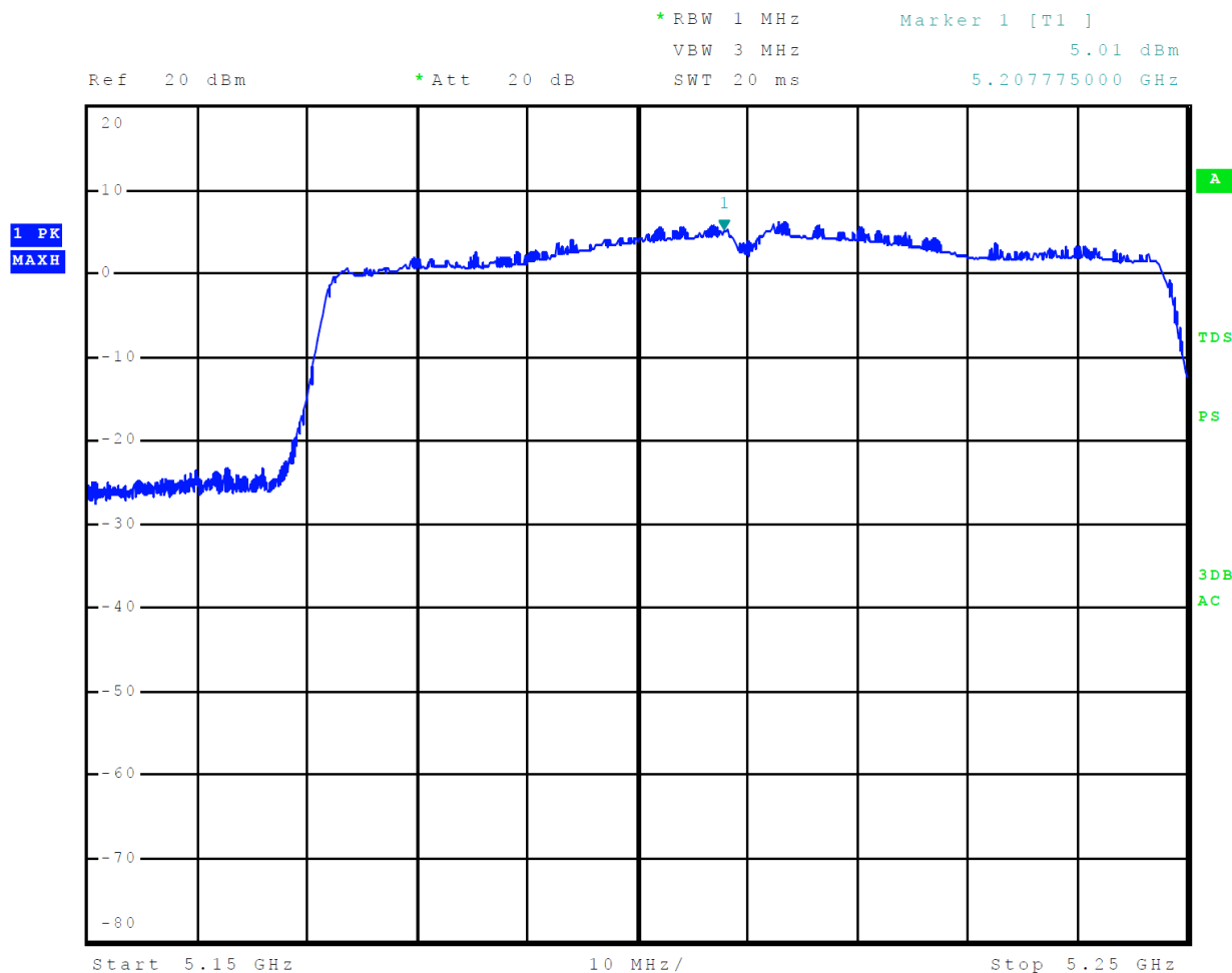
Figure 38 Plot of Transmitter Emissions Across 5150-5250 MHz Mode 15, U-NII-1 (802.11ac80)
