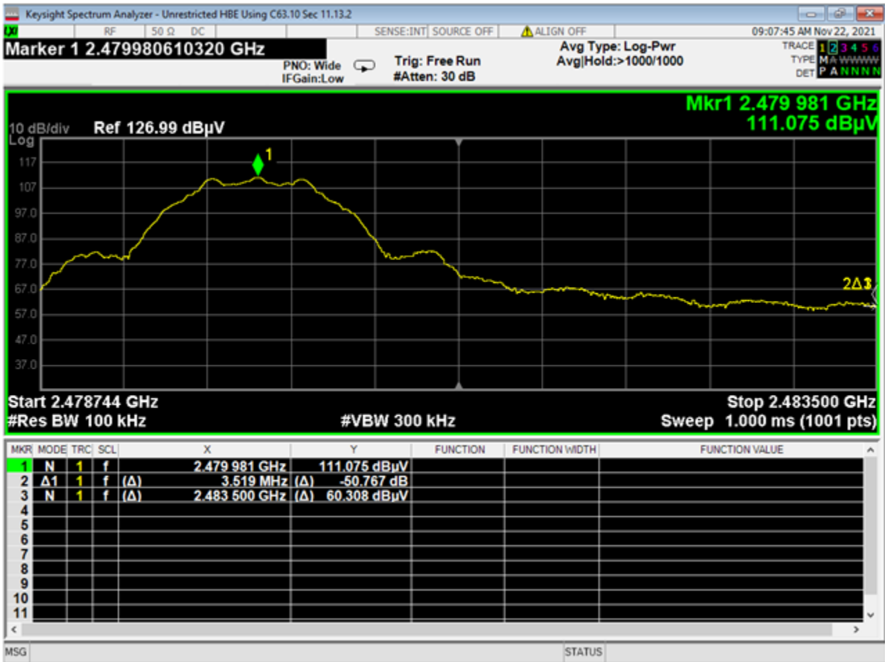
11 HBE Unrestricted Bandedge
