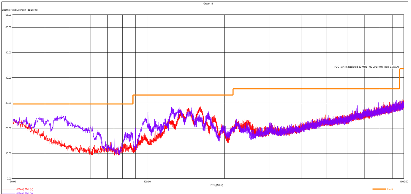
Figure 5 - Radiated Emissions Plot, BLE, Low Channel
