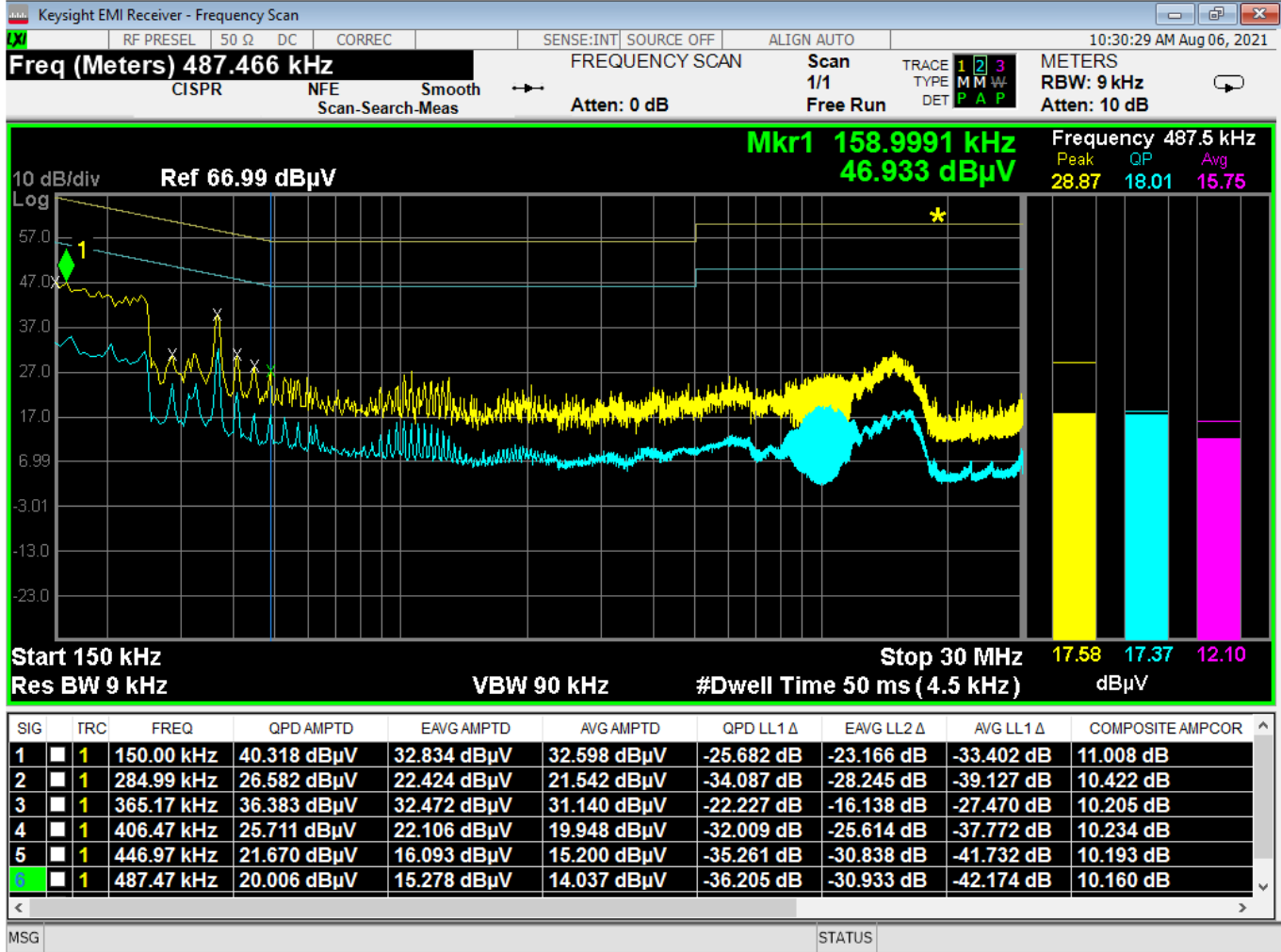
Figure 13 - Conducted Emissions Plot, Line, IDLE
