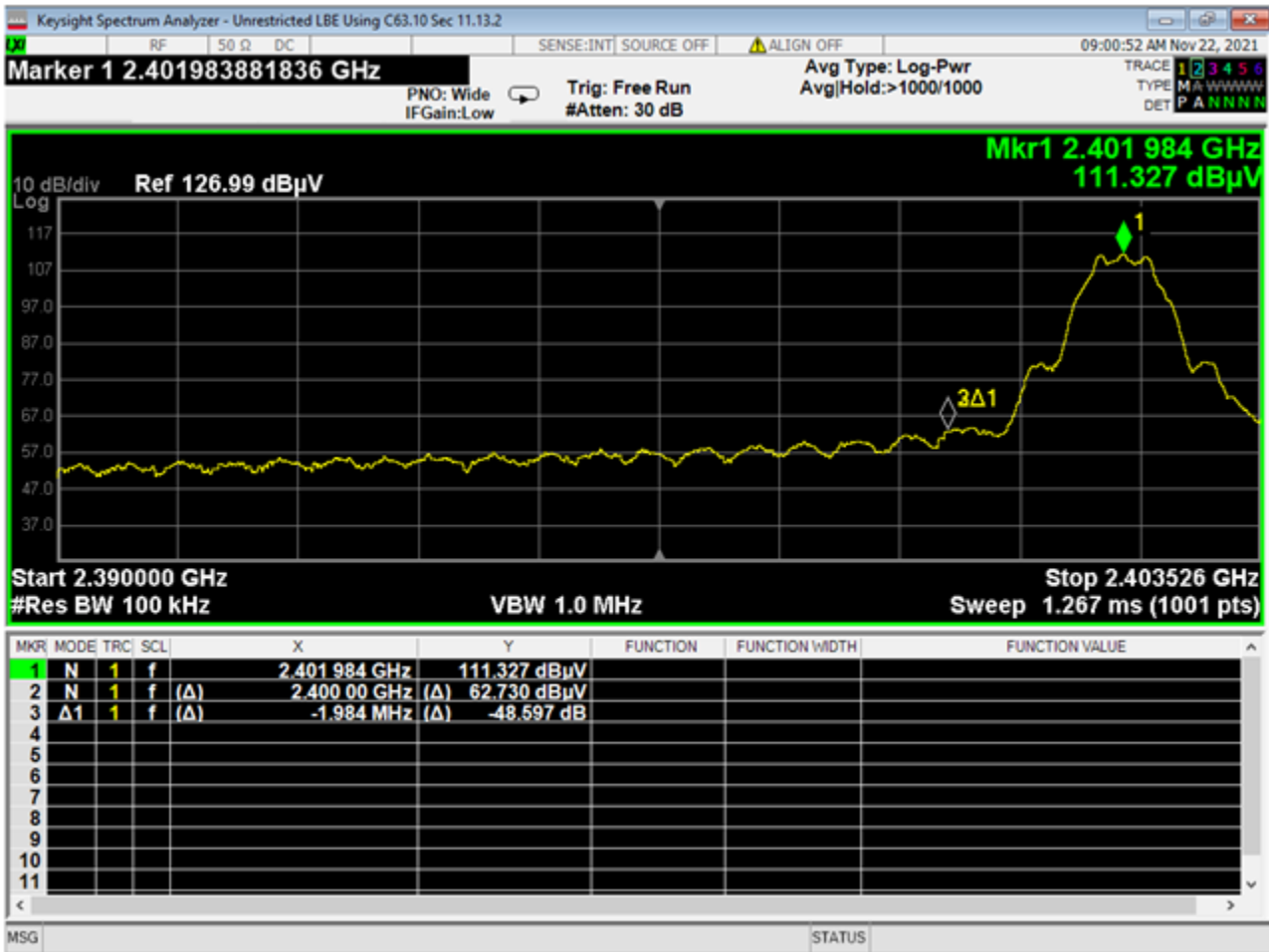
13 LBE Unrestricted Bandedge
