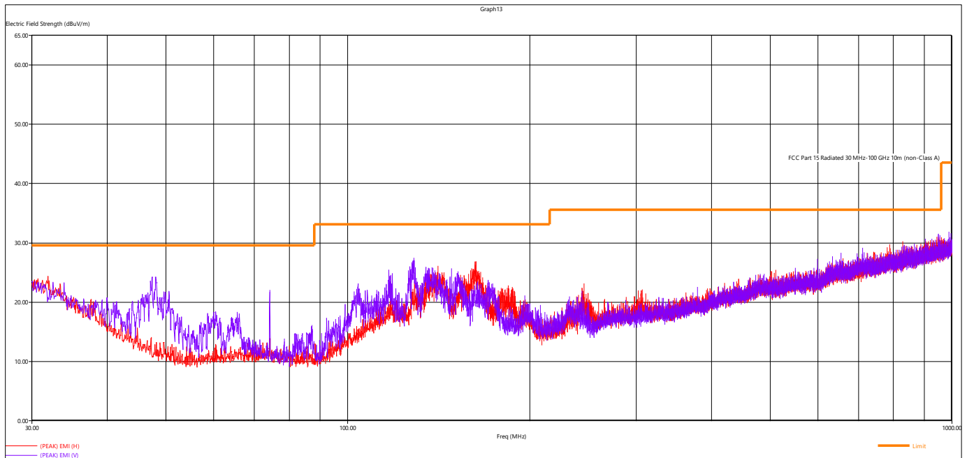
Figure 7 - Radiated Emissions Plot, BLE, High Channel
