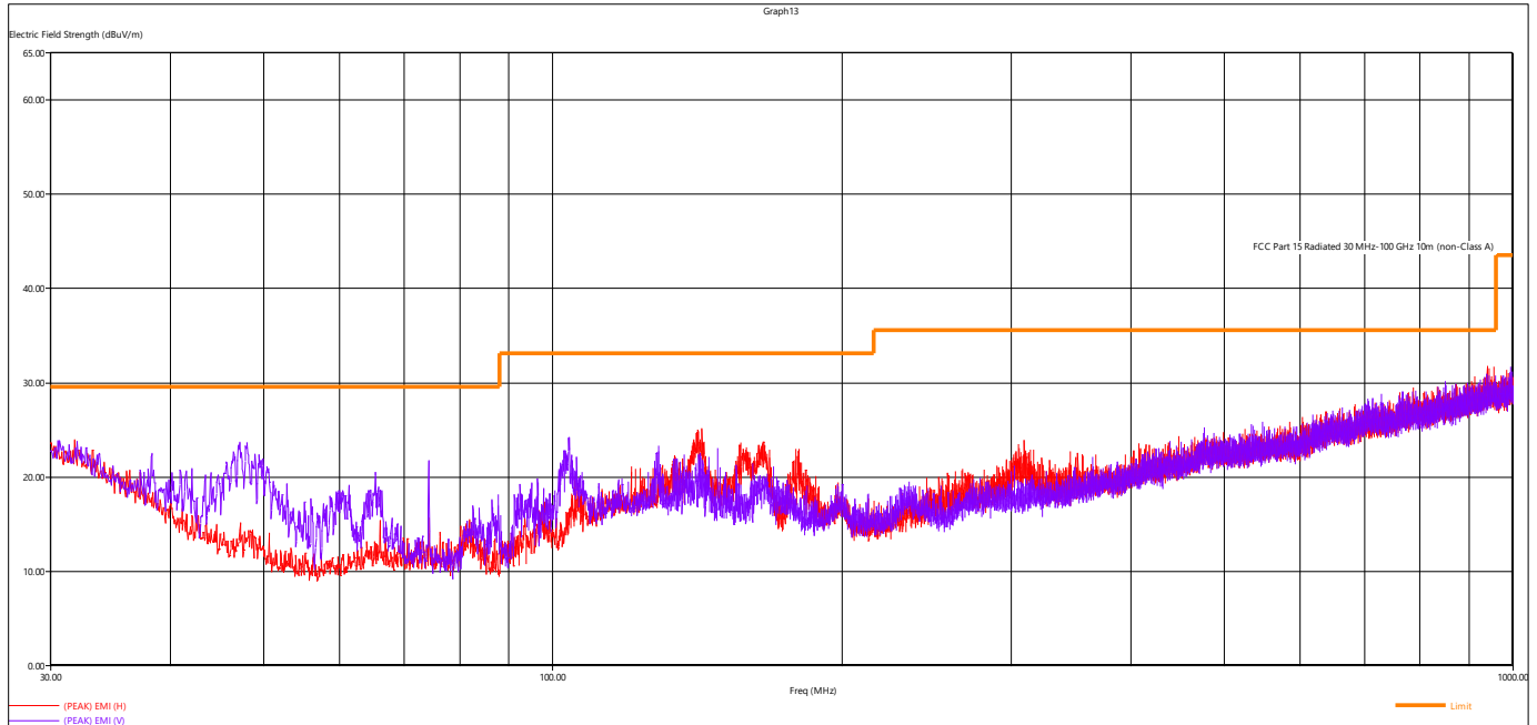
Figure 6 - Radiated Emissions Plot, BLE, Mid Channel
