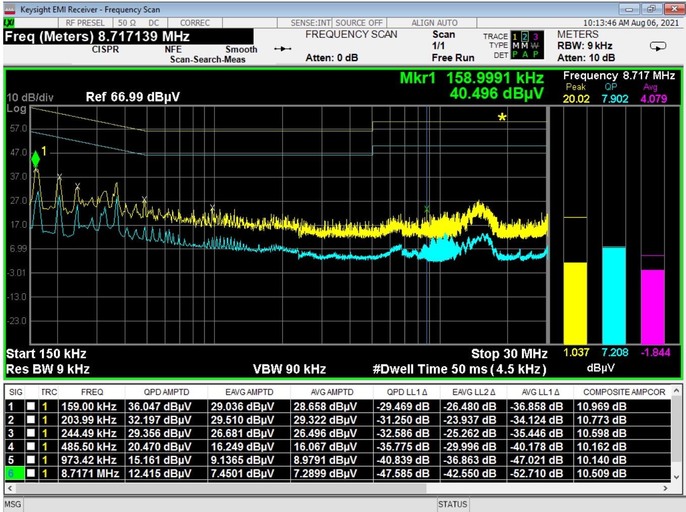
Figure 14 - Conducted Emissions Plot, Neutral, IDLE
