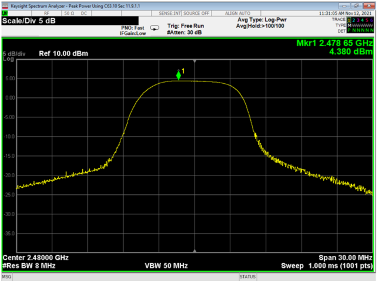
03 Peak Power High
