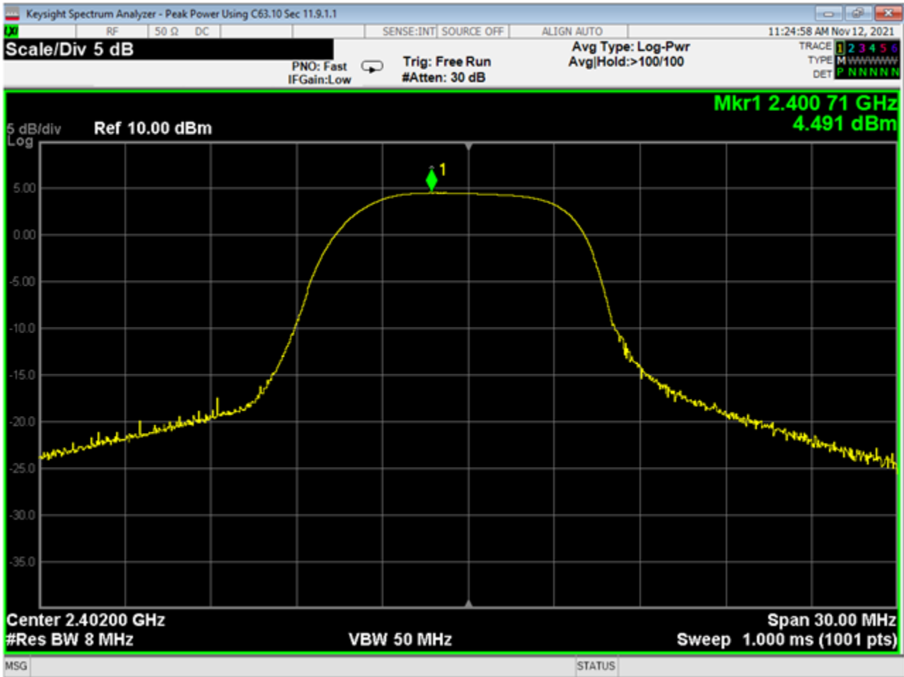
01 Peak Power Low
