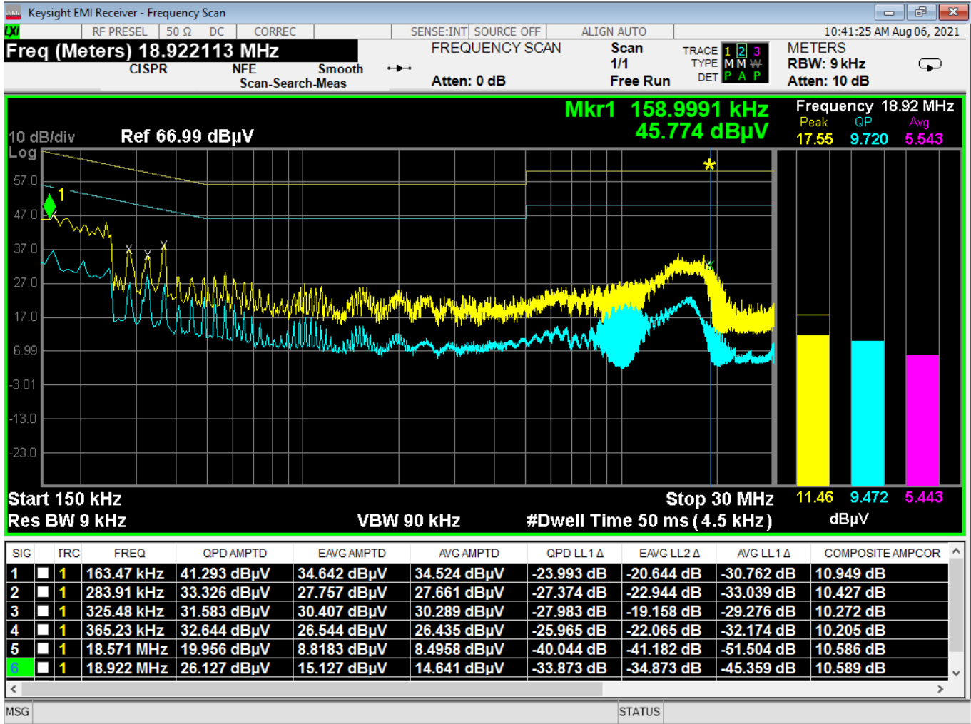
Figure 11 - Conducted Emissions Plot, Line, TX
