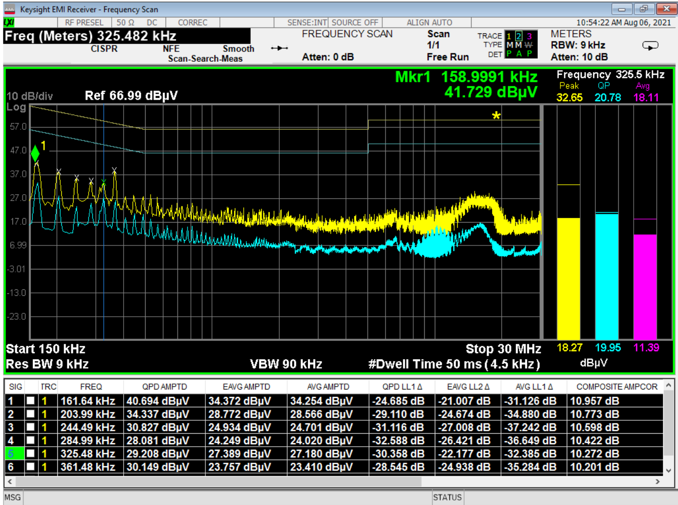
Figure 12 - Conducted Emissions Plot, Neutral, TX
