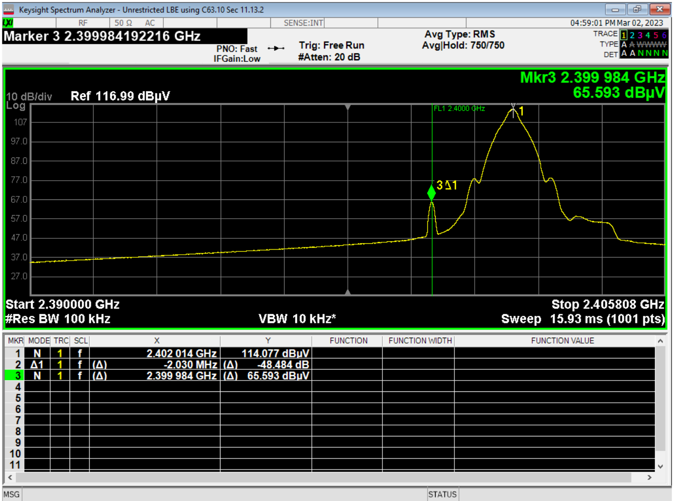
07 Lower Bandedge, Unrestricted, BTBR
