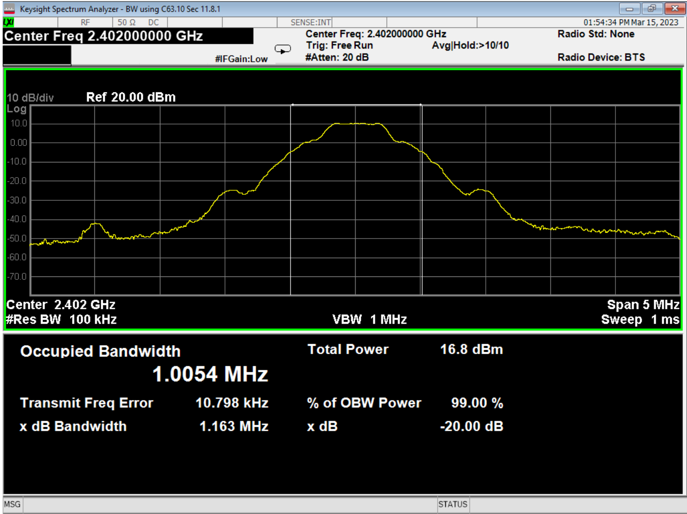
04 OBW-20dB, Low Channel, BTBR
