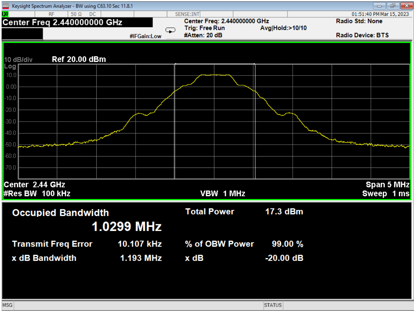
05 OBW-20dB, Mid Channel, BTBR
