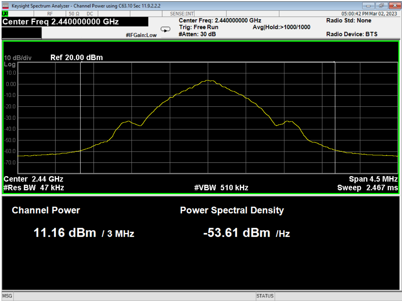
02 Average Power, Mid Channel, BTBR
