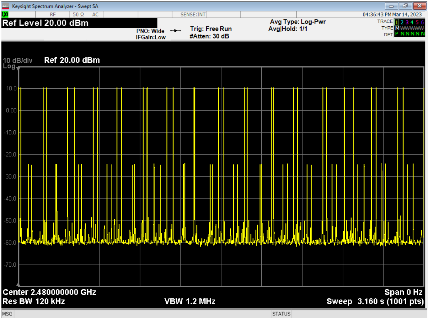
11 Dwell Time, 3.16S (reported for better resolution)
