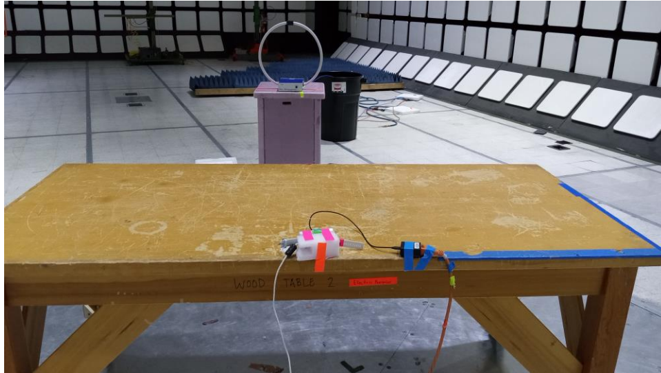
150kHz – 30 MHz Test Setup
