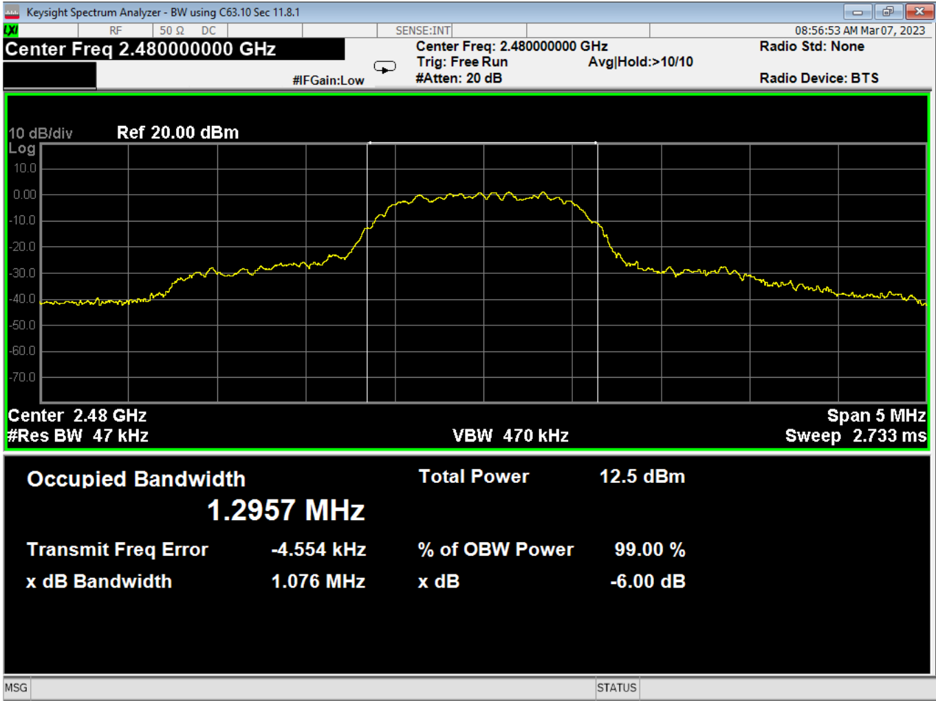
16 Occupied Bandwidth, High Channel, 2EDR
