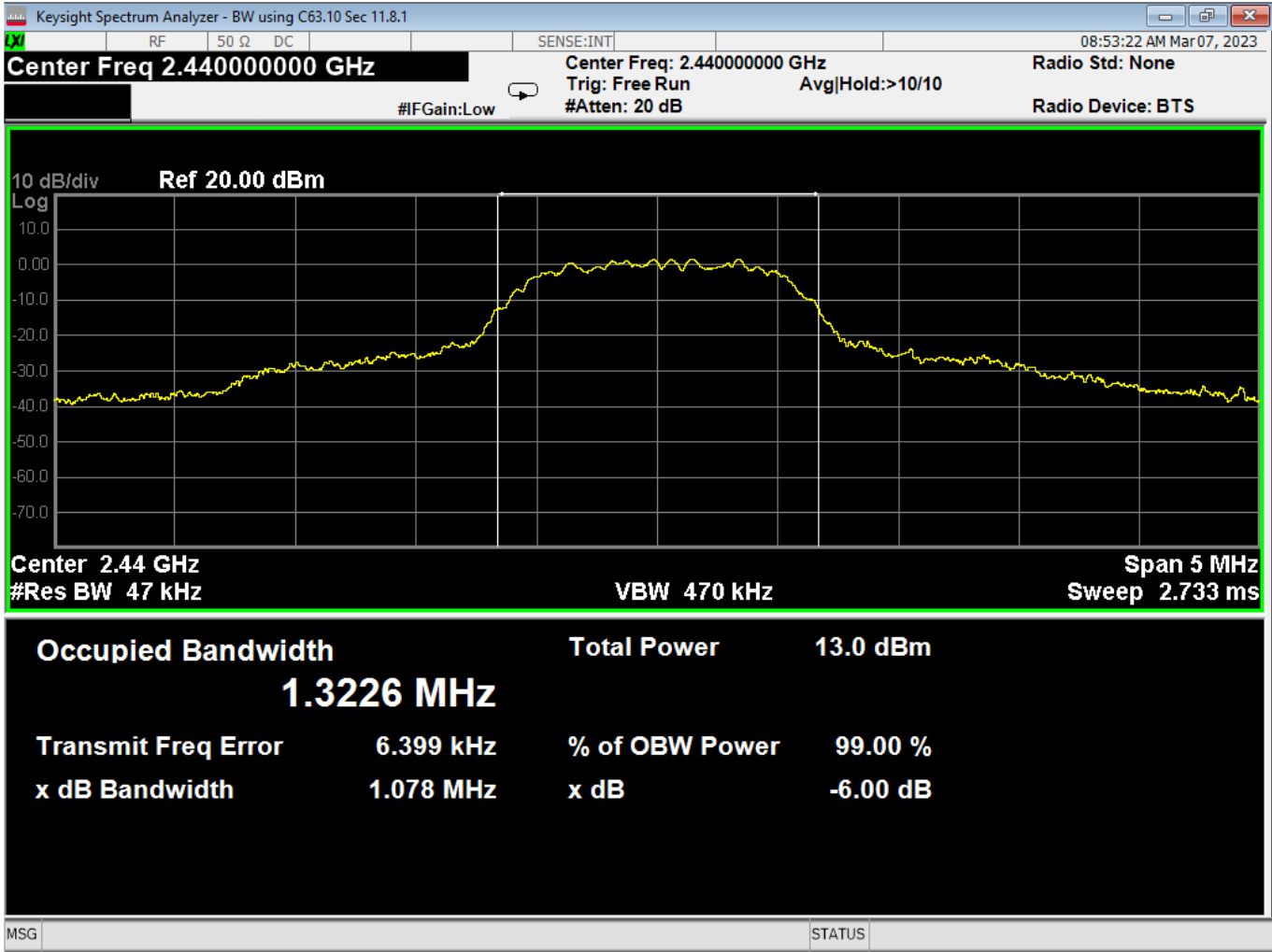
15 Occupied Bandwidth, Mid Channel, 2EDR
