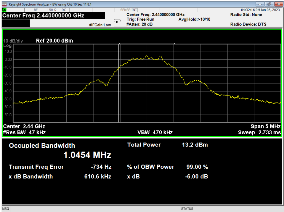
15 Occupied Bandwidth, Mid Channel, GMSK 1MB
