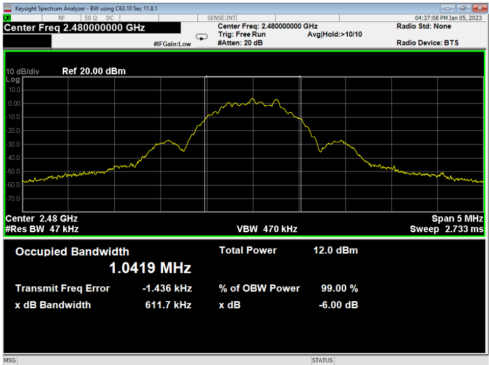
16 Occupied Bandwidth, High Channel, GMSK 1MB
