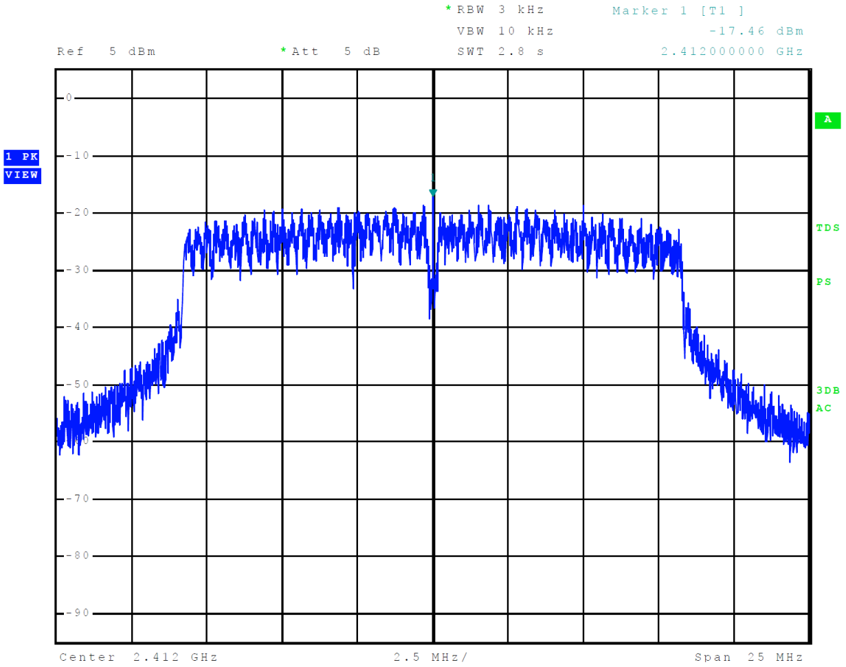
Figure 24 Plot of Transmitter Power Spectral Density Mode 7 802.11g (OFDM)
