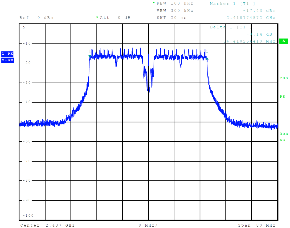
Figure 21 Plot of 6-dB Occupied Bandwidth Mode 9 802.11n40 (MSC)
