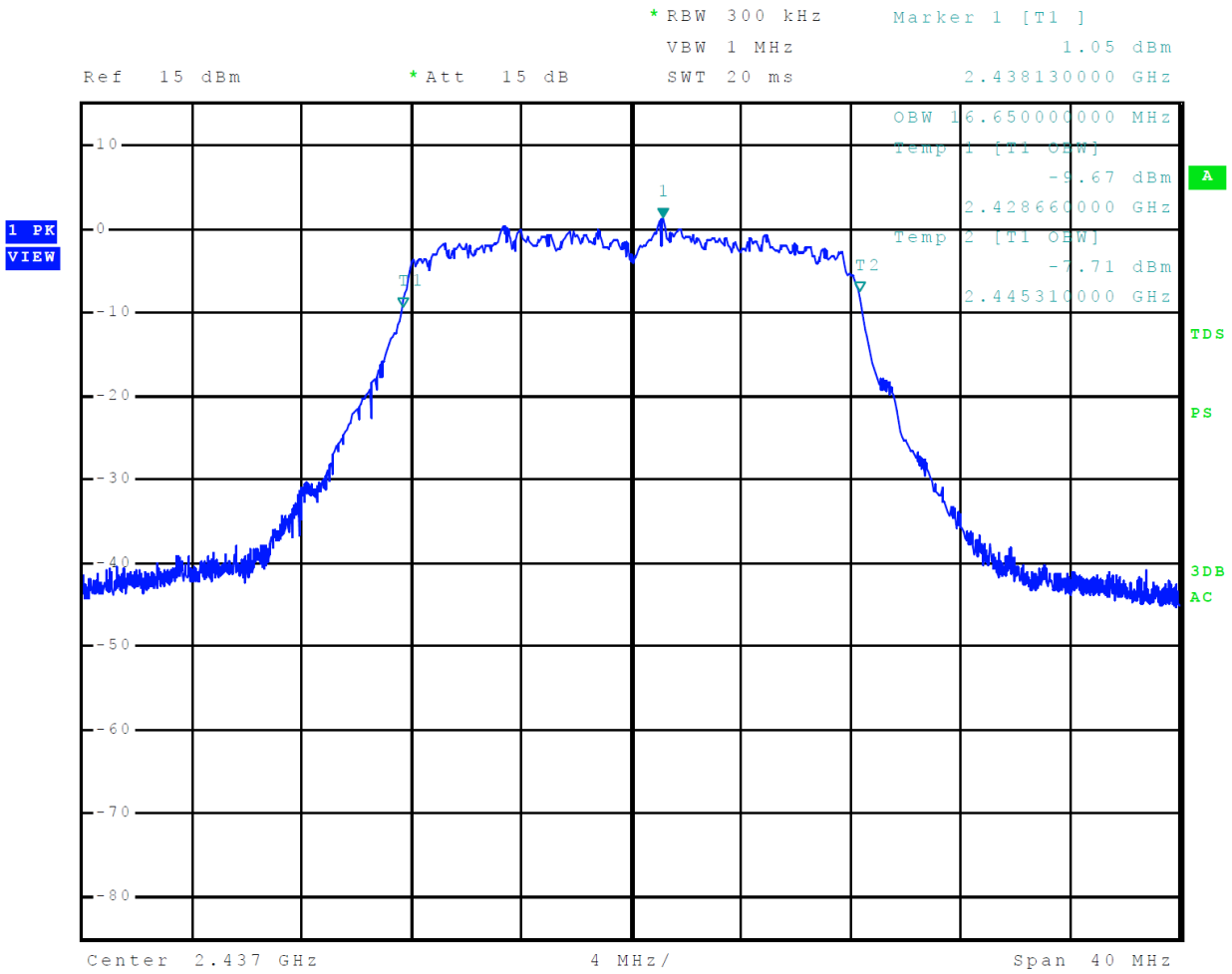
Figure 18 Plot of 99% Occupied Bandwidth Mode 7 802.11g (OFDM)
