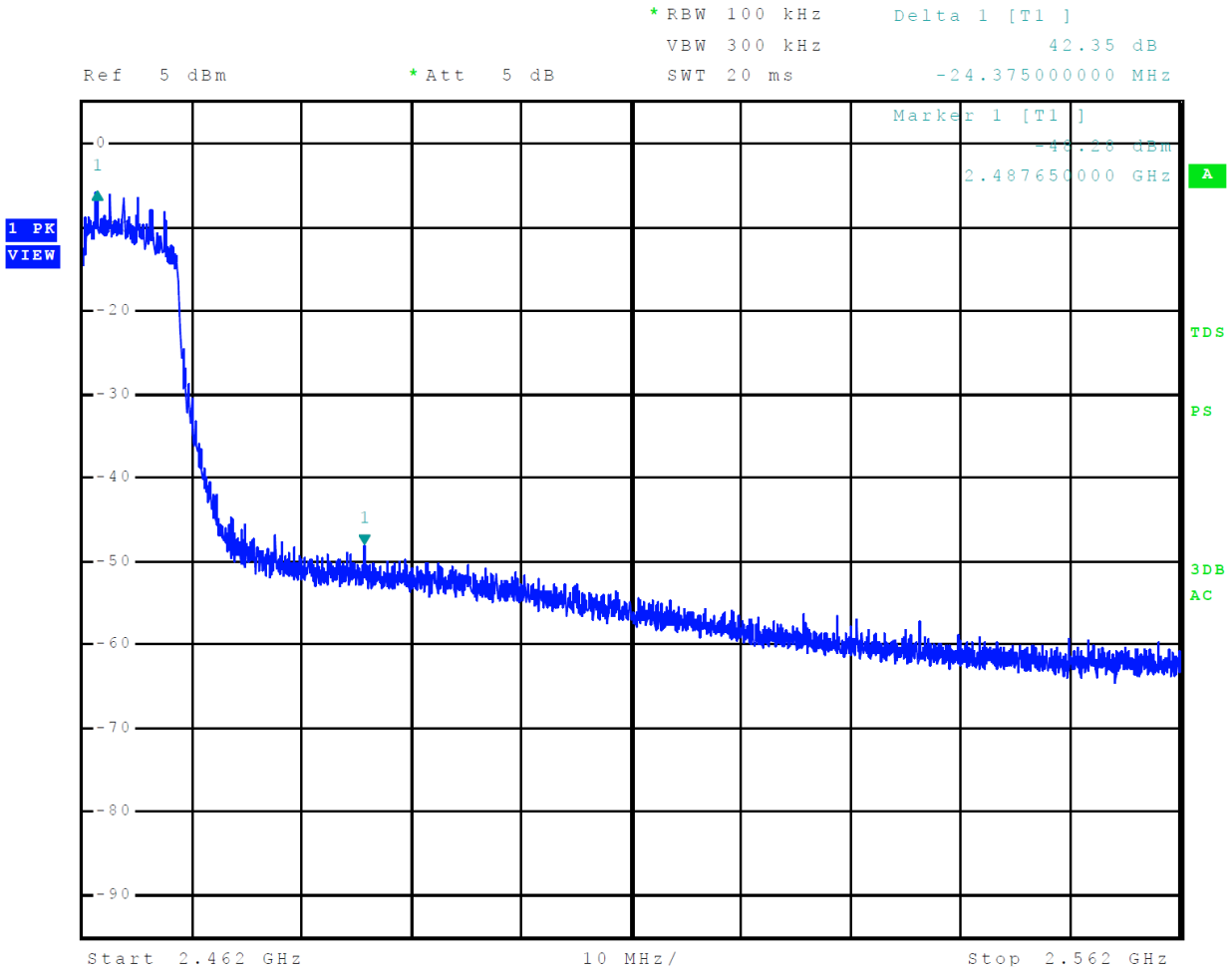
Figure 13 Plot of Transmitter Emissions High Band Edge Mode 8 802.11n (MSC)
