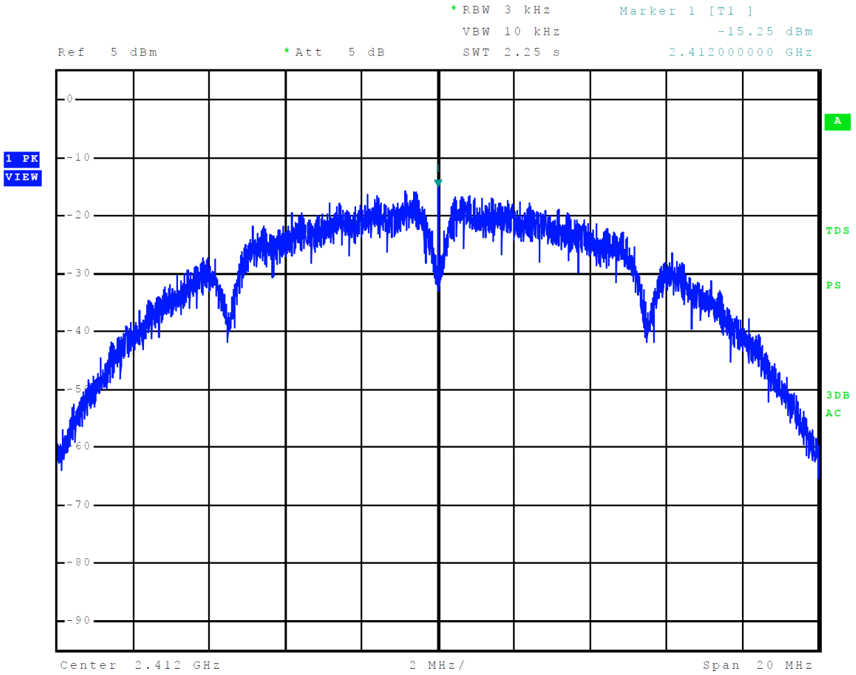
Figure 23 Plot of Transmitter Power Spectral Density Mode 6 802.11b (DSSS/CCK)
