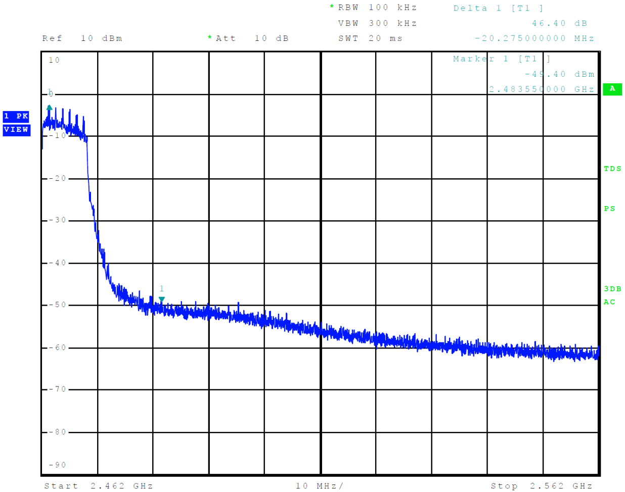
Figure 12 Plot of Transmitter Emissions High Band Edge Mode 7 802.11g (OFDM)
