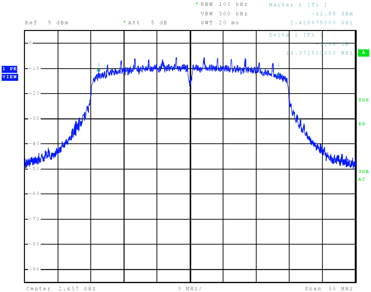
Figure 19 Plot of 6-dB Occupied Bandwidth Mode 8 802.11n (MSC)
