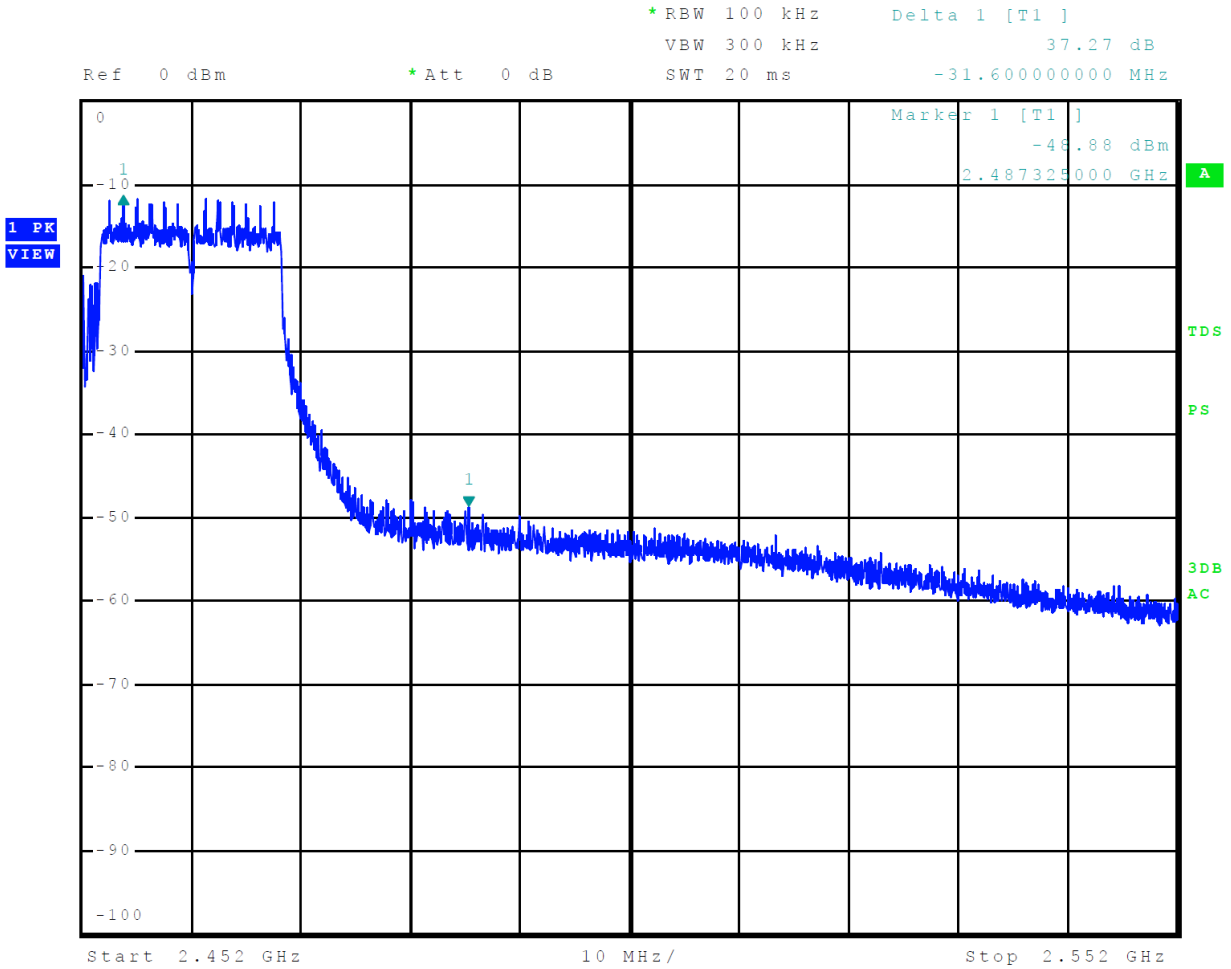
Figure 14 Plot of Transmitter Emissions High Band Edge Mode 9 802.11n40 (MSC)
