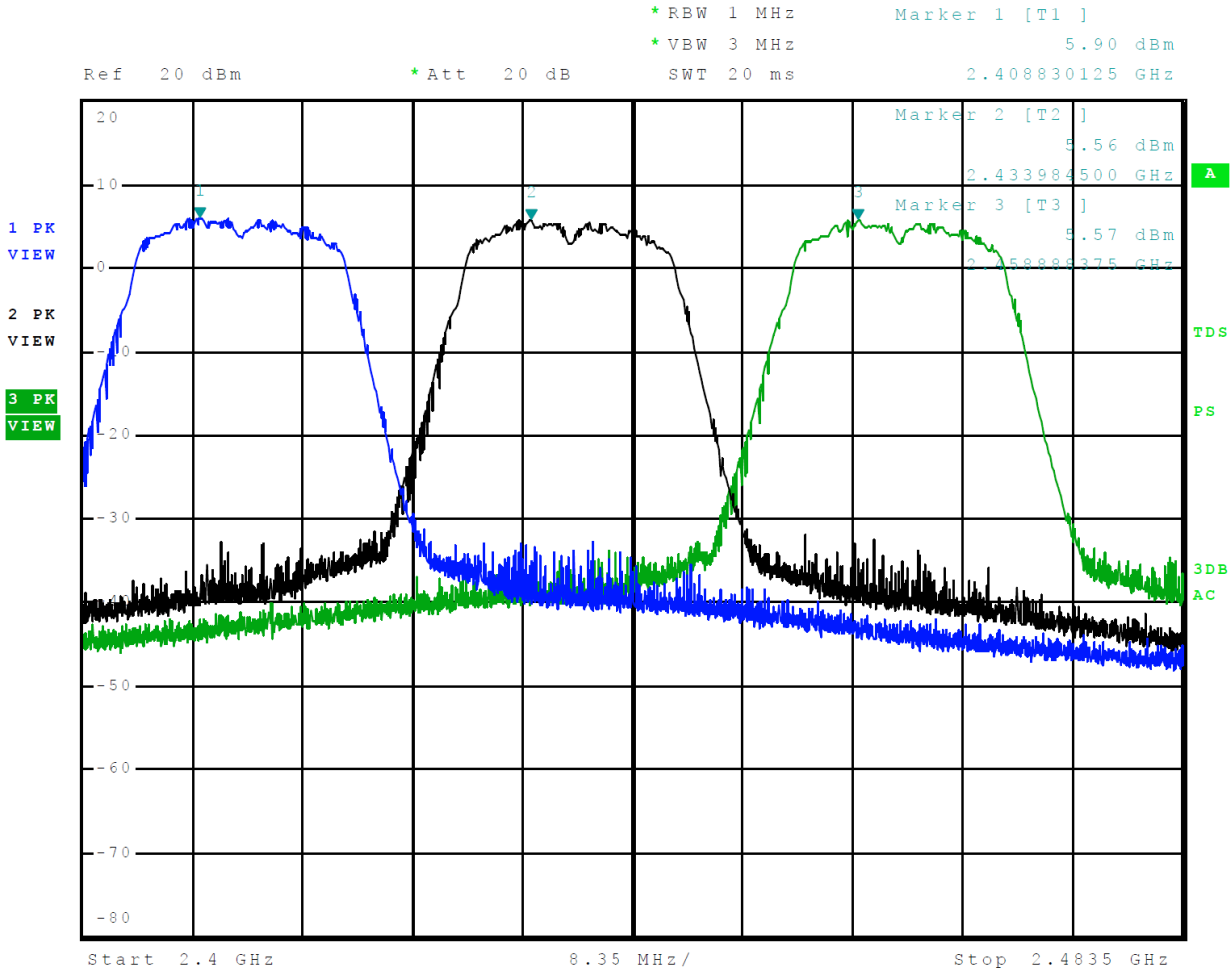
Figure 4 Plot of Transmitter Operation in 2412-2462 MHz Mode 7 802.11g (OFDM)
