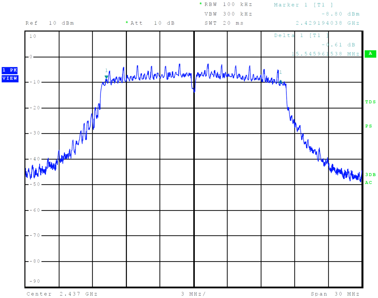
Figure 17 Plot of 6-dB Occupied Bandwidth Mode 7 802.11g (OFDM)
