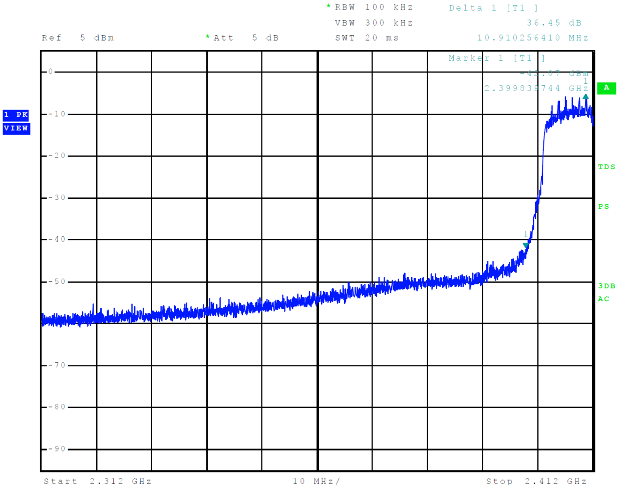
Figure 9 Plot of Transmitter Emissions Low Band Edge Mode 8 802.11n (MSC)
