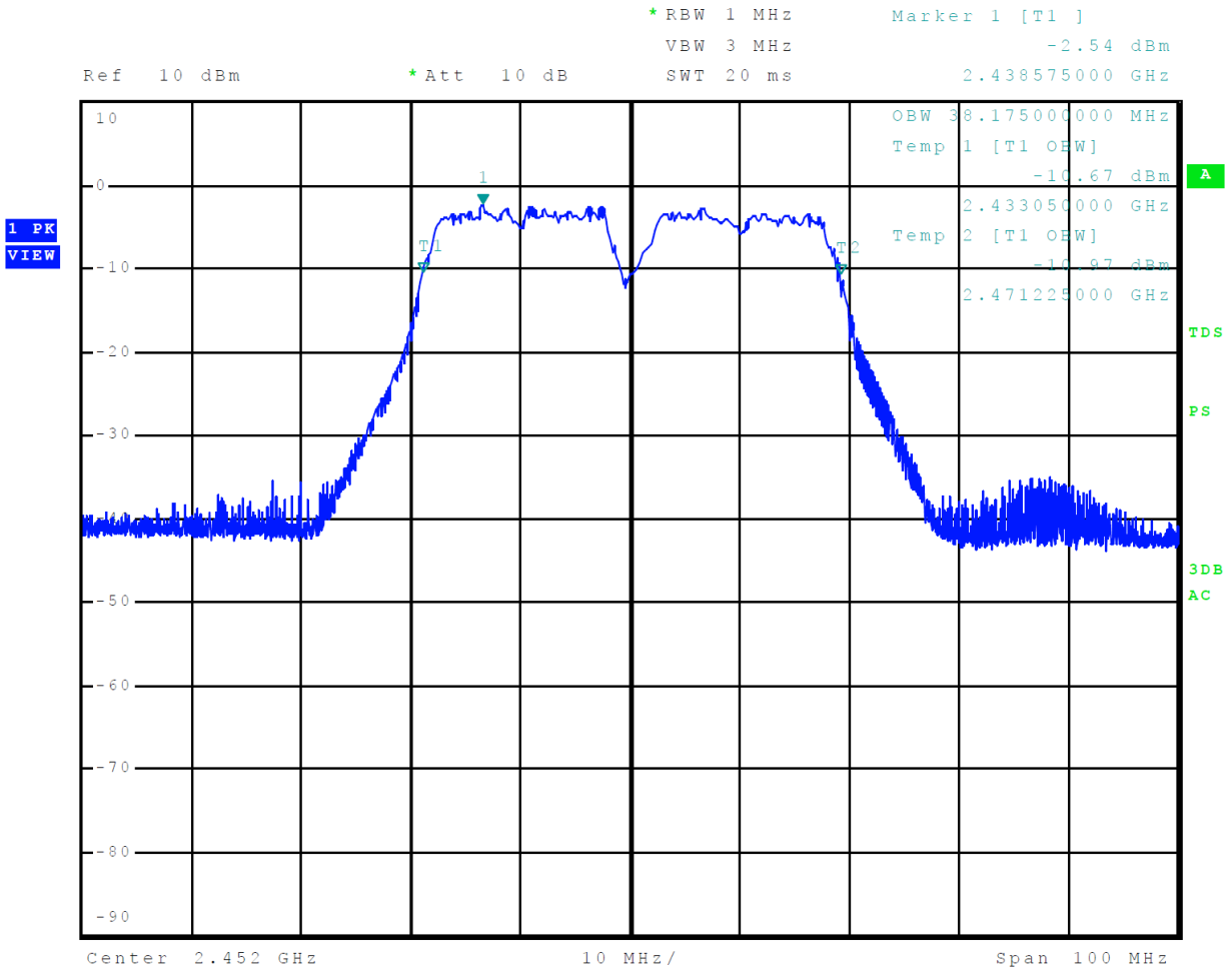
Figure 22 Plot of 99% Occupied Bandwidth Mode 9 802.11n40 (MSC)
