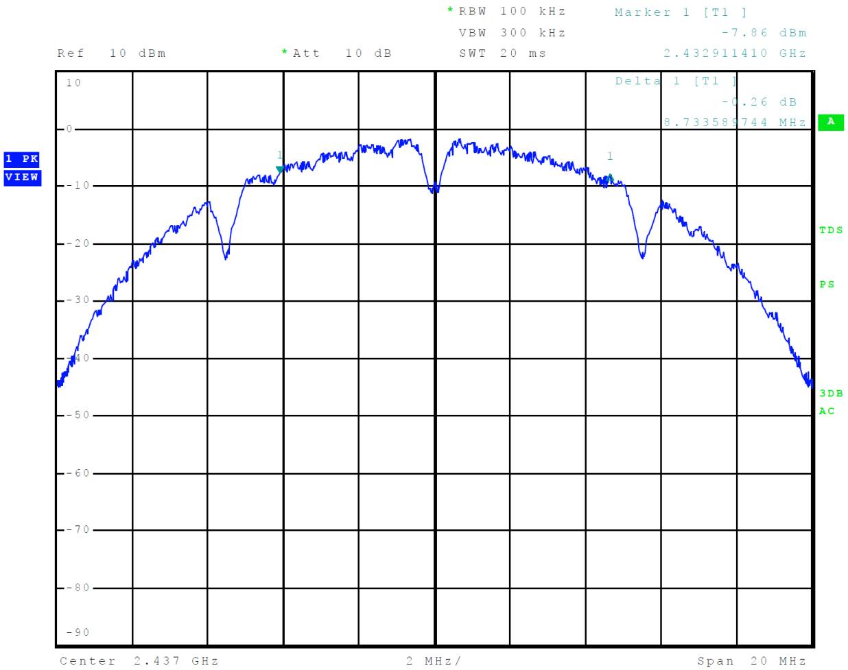
Figure 15 Plot of 6-dB Occupied Bandwidth Mode 6 802.11b (DSSS/CCK)
