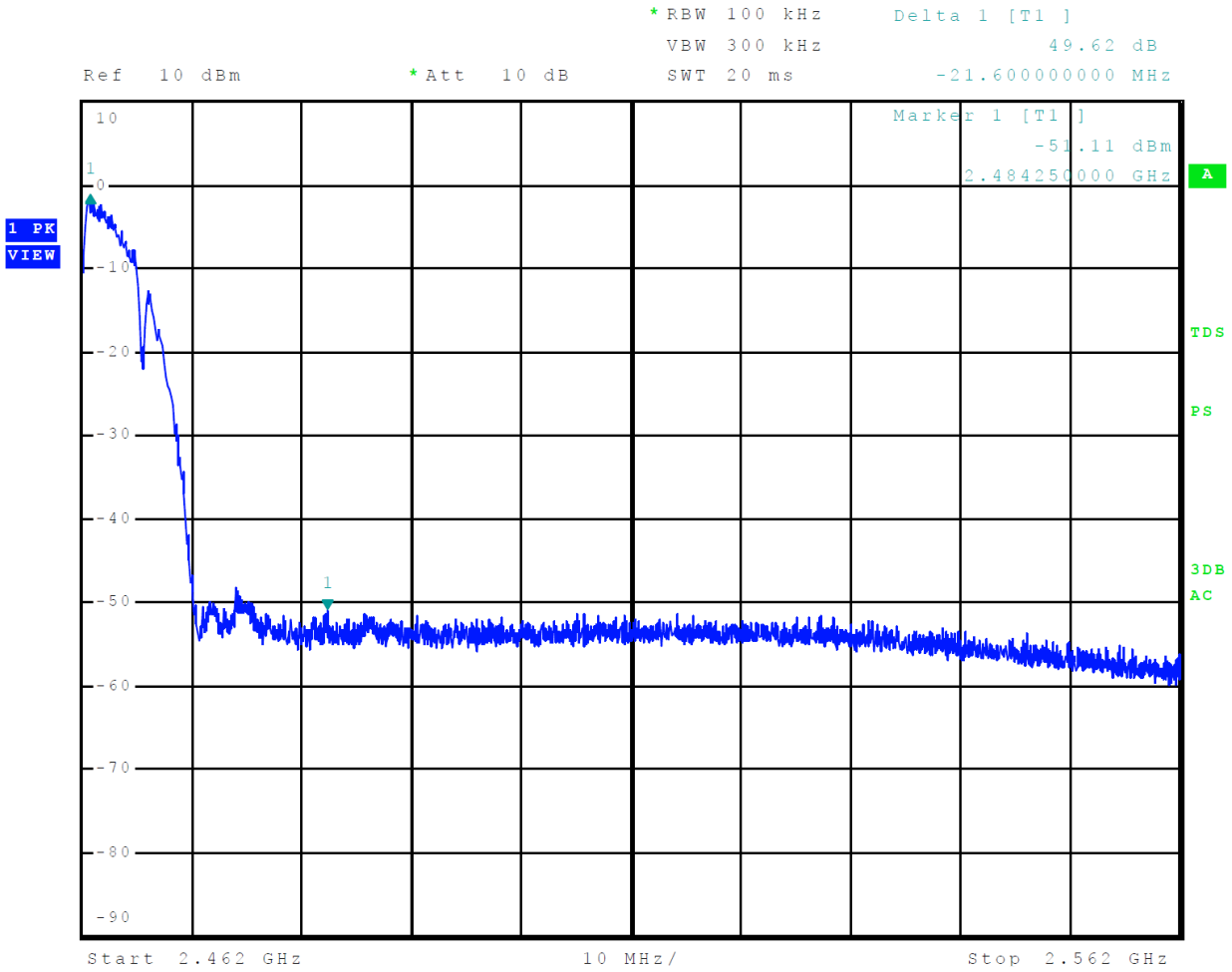
Figure 11 Plot of Transmitter Emissions High Band Edge Mode 6 802.11b (DSSS/CCK)
