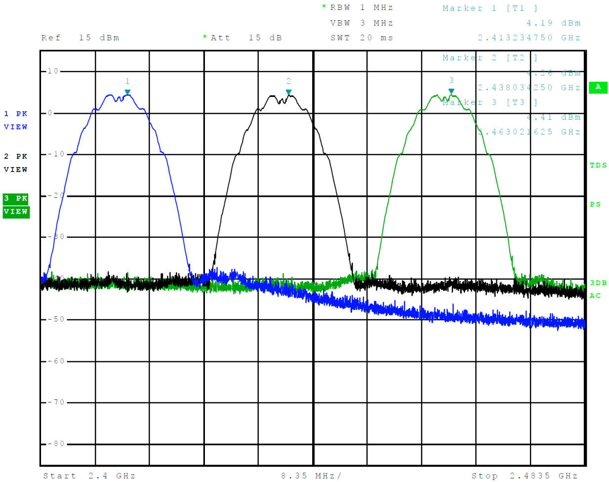
Figure 3 Plot of Transmitter Operation in 2412-2462 MHz Mode 6 802.11b (DSSS/CCK)
