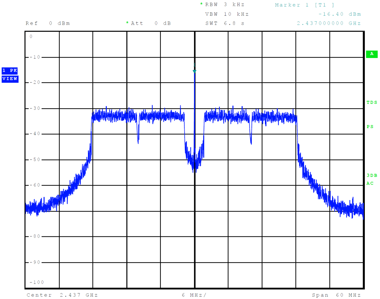
Figure 26 Plot of Transmitter Power Spectral Density Mode 9 802.11n40 (MSC)
