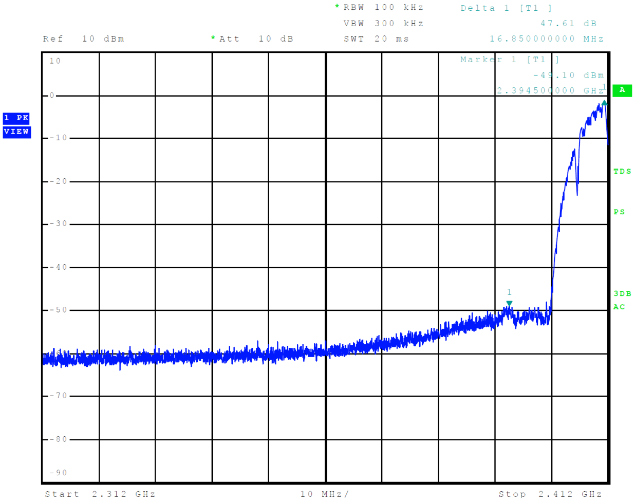
Figure 7 Plot of Transmitter Emissions Low Band Edge Mode 6 802.11b (DSSS/CCK)
