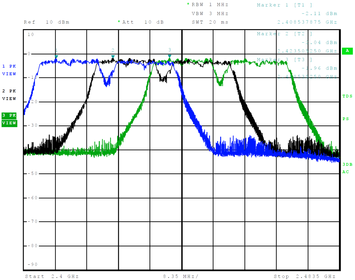
Figure 6 Plot of Transmitter Operation in 2422-2452 MHz Mode 9 802.11n40 (MSC)
