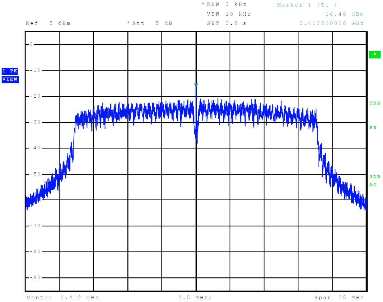
Figure 25 Plot of Transmitter Power Spectral Density Mode 8 802.11n (MSC)
