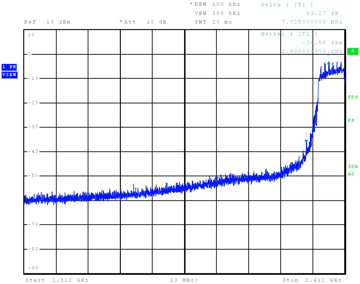
Figure 8 Plot of Transmitter Emissions Low Band Edge Mode 7 802.11g (OFDM)
