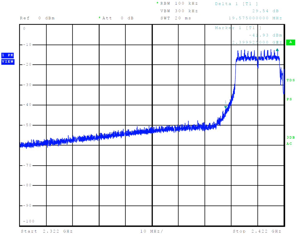
Figure 10 Plot of Transmitter Emissions Low Band Edge Mode 9 802.11n40 (MSC)
