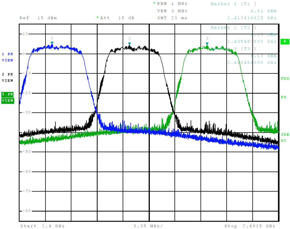
Figure 5 Plot of Transmitter Operation in 2412-2462 MHz Mode 8 802.11n (MSC)
