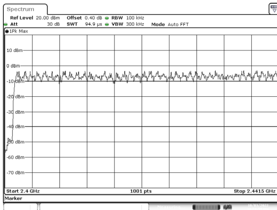
2402 MHz
