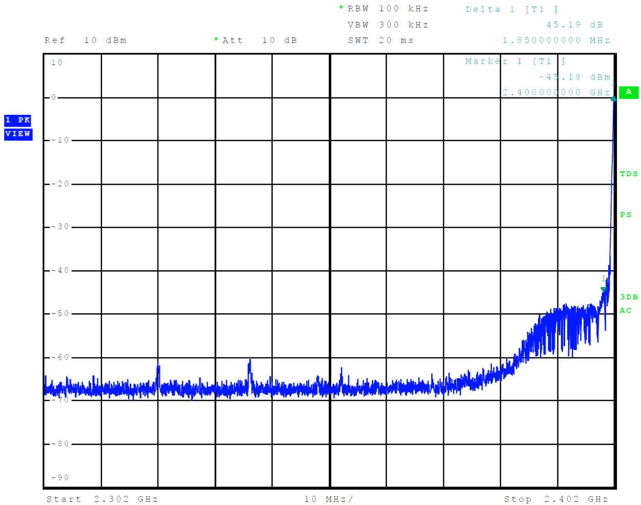
Figure 2 Plot of Transmitter Emissions Low Band Edge Mode 1 BT BR (GFSK)
