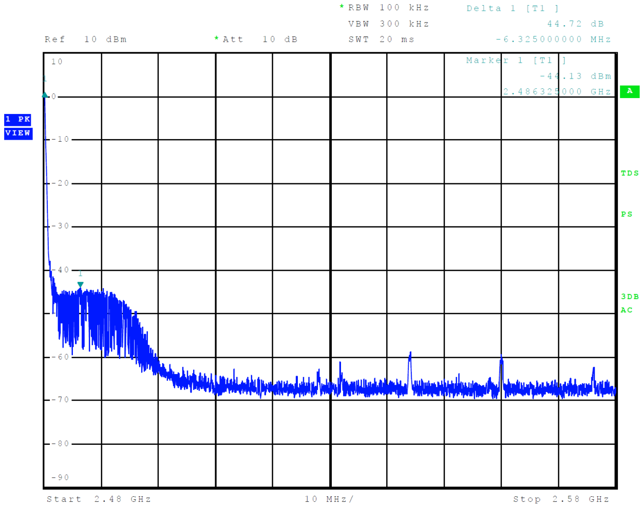
Figure 3 Plot of Transmitter Emissions High Band Edge Mode 1 BT BR (GFSK)
