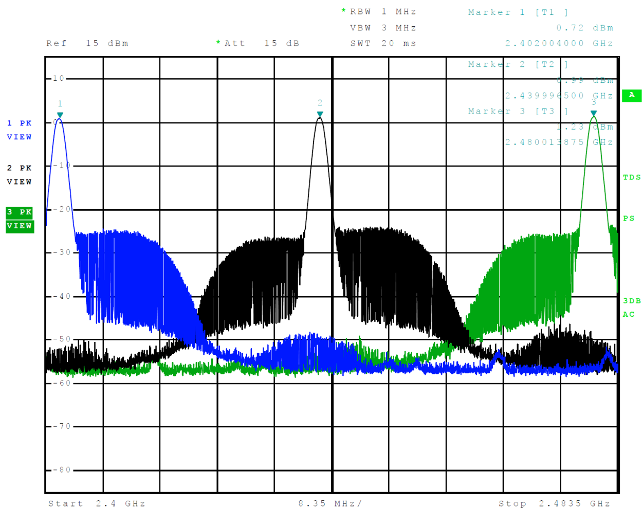
Figure 1 Plot of Transmitter Emissions in 2402-2480 MHz Mode 1 BT BR (GFSK)
