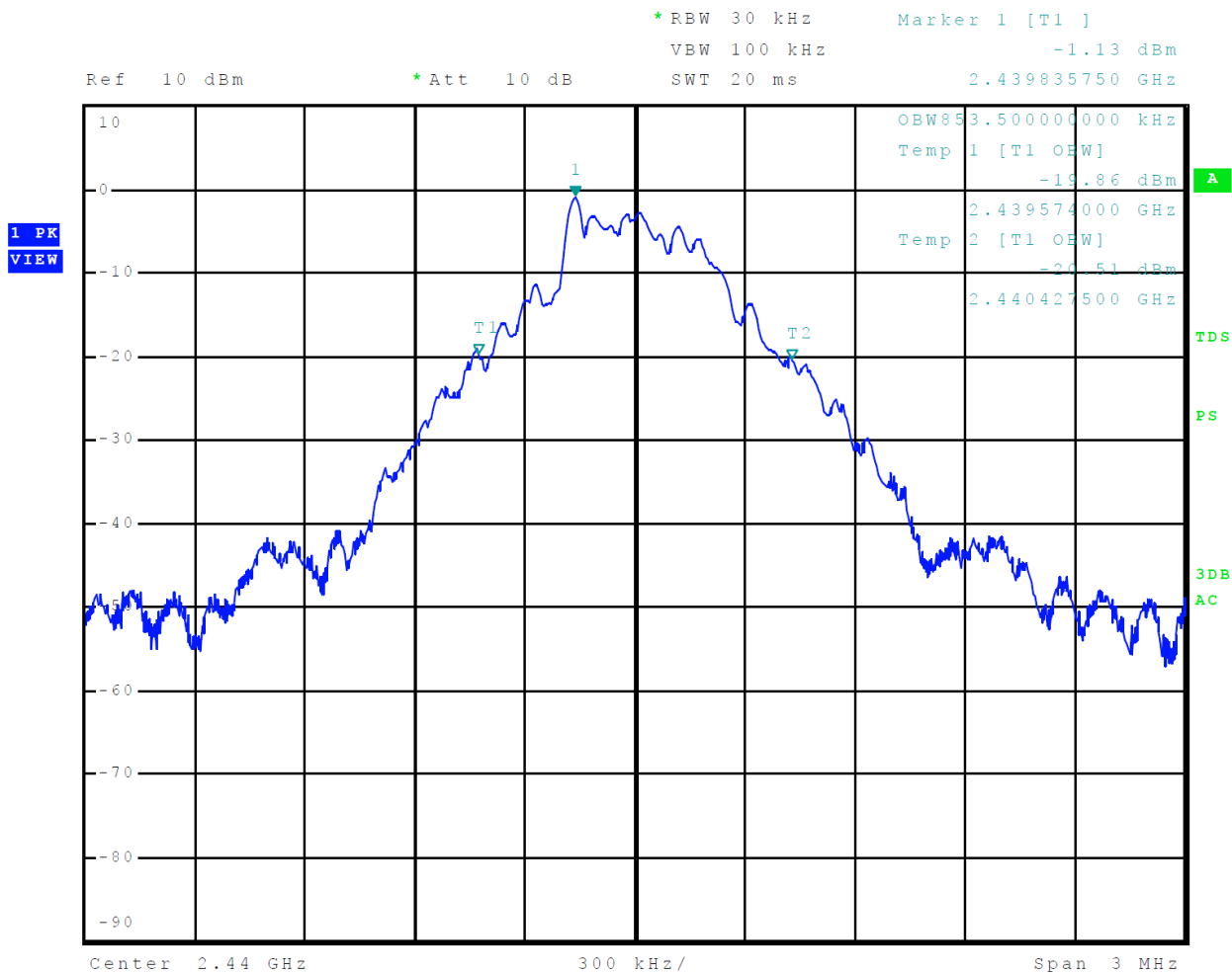
Figure 4 Plot of Transmitter 99% Occupied Bandwidth Mode 1 BT BR (GFSK)
