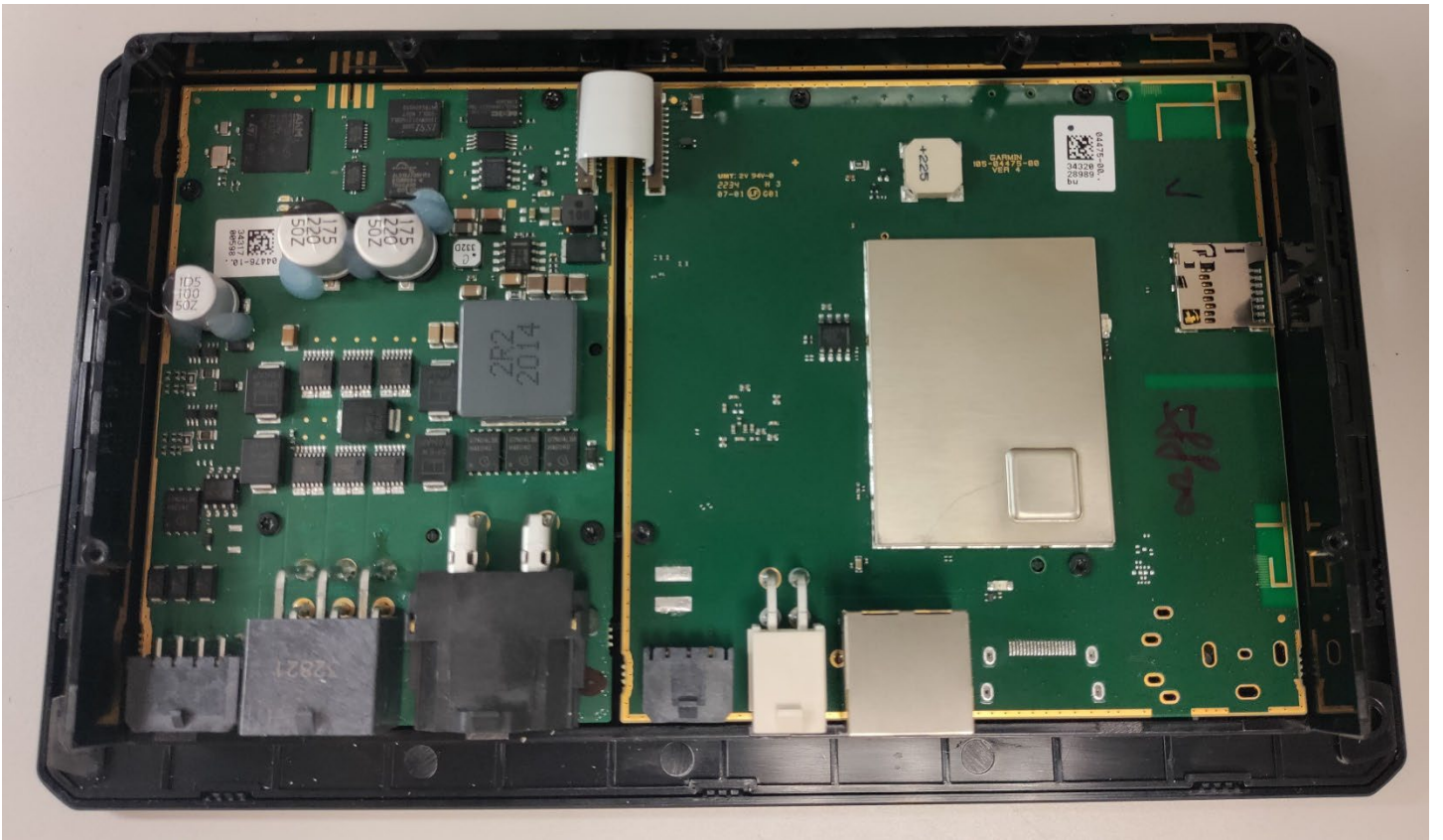
A04475 7" Internal photo showing PCB locations
