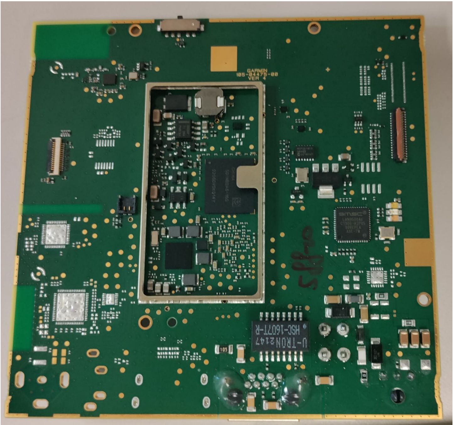
A04475 7" Digital Board – bottom side without cover
