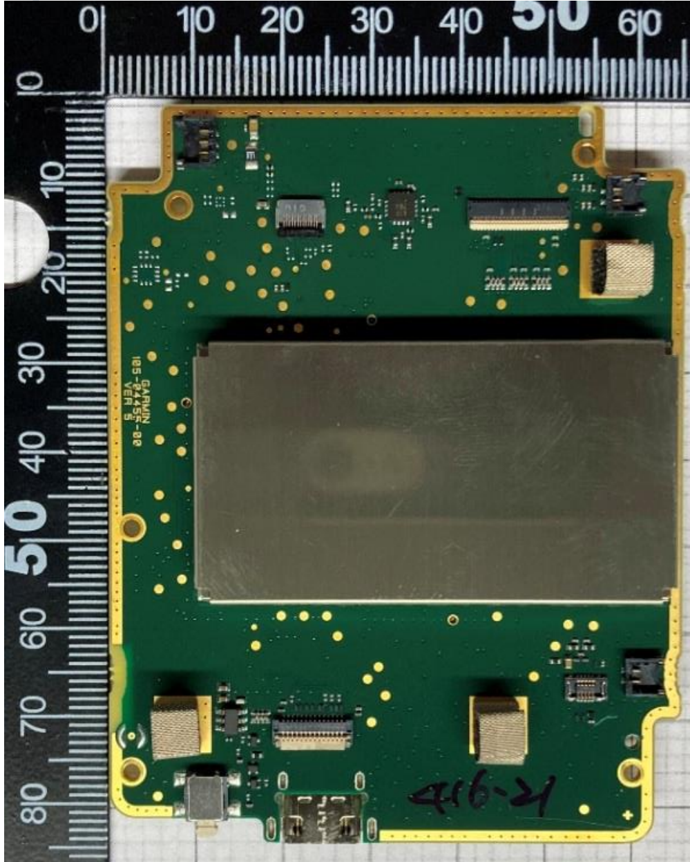
Top with Shield
