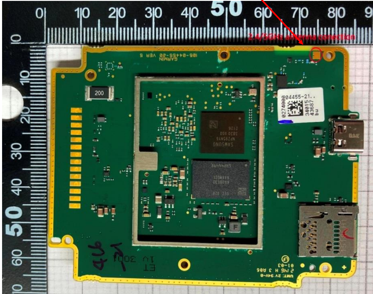
Bottom Shield removed and Antenna Connection point
