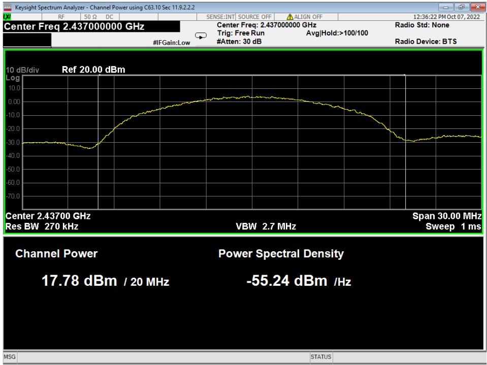
Figure 17 – Conducted Average Power Measurement, 802.11b 11MB
