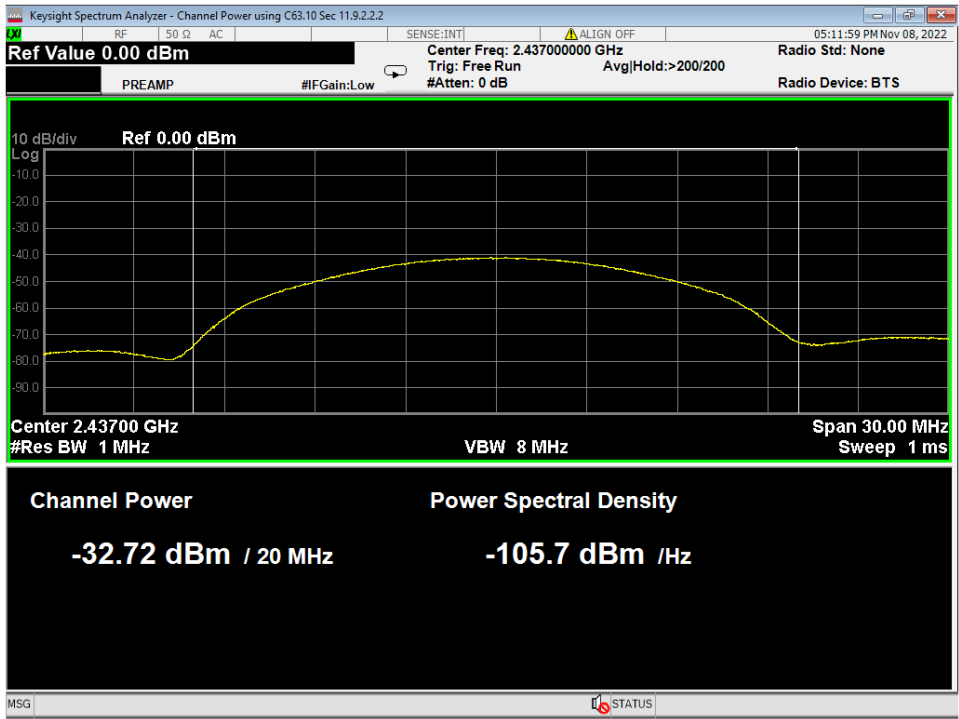
Figure 18 – Radiated Average Power Measurement, 802.11b 11MB
