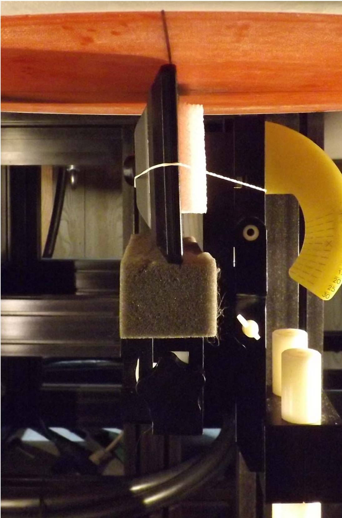
Figure C.7 – Setup Photo, Top Edge - Far
