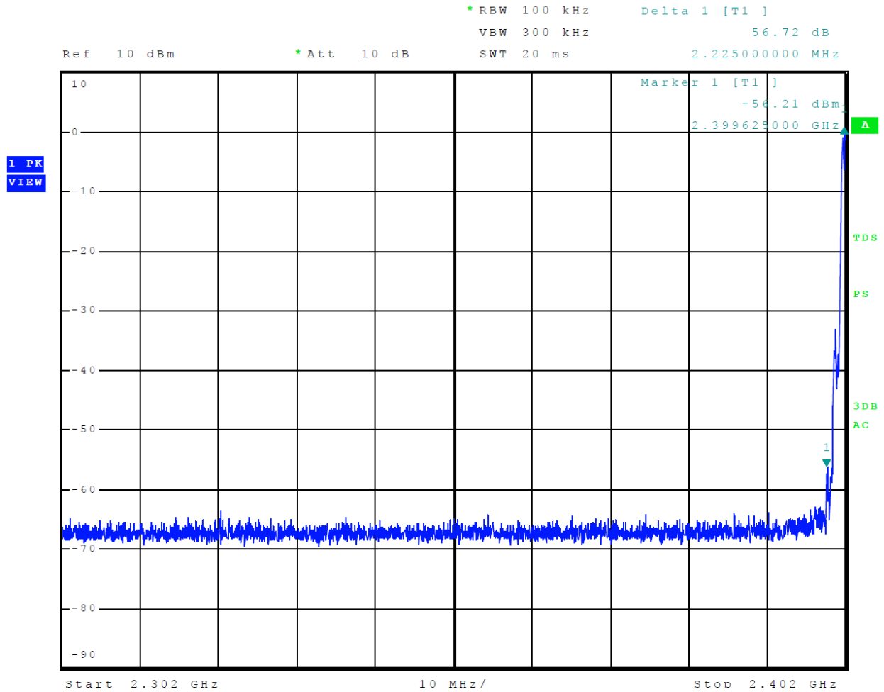
Figure 12 Plot of Transmitter Emissions Low Band Edge Mode 2 BT 2EDR
