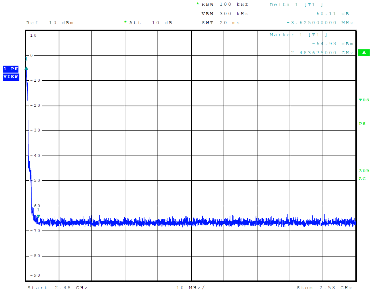
Figure 19 Plot of Transmitter Emissions High Band Edge Mode 2 BT 2EDR
