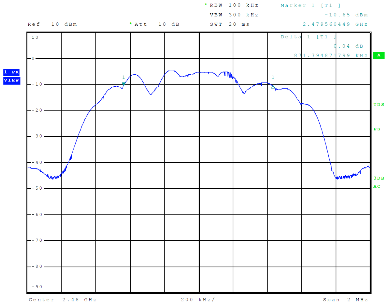
Figure 41 Plot of Transmitter Power Spectral Density Mode 3 BT 3EDR
