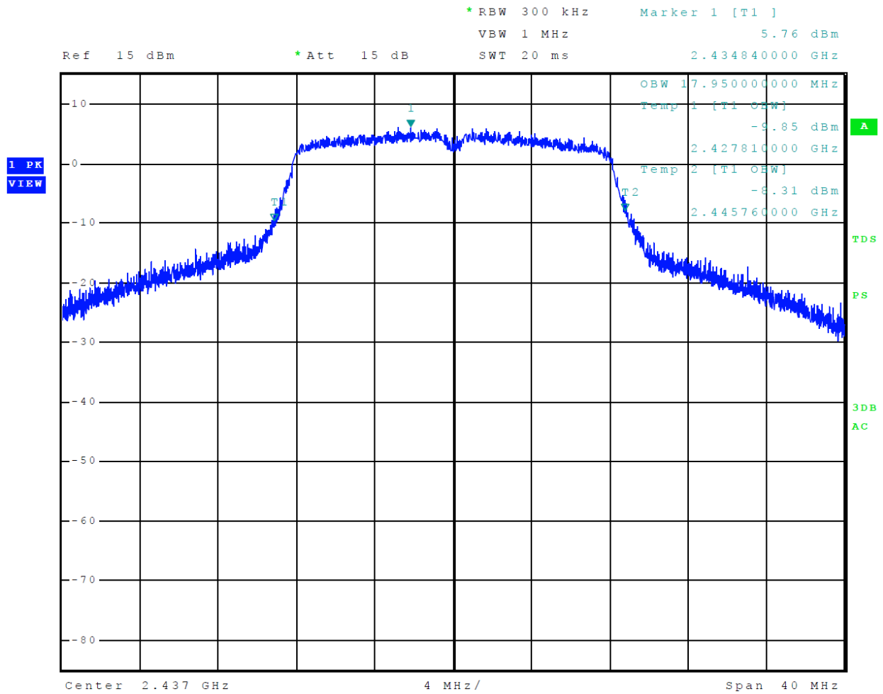
Figure 35 Plot of 99% Occupied Bandwidth Mode 6 802.11g
