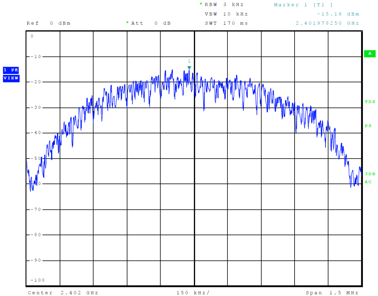
Figure 42 Plot of Transmitter Power Spectral Density Mode 4 BT BLE
