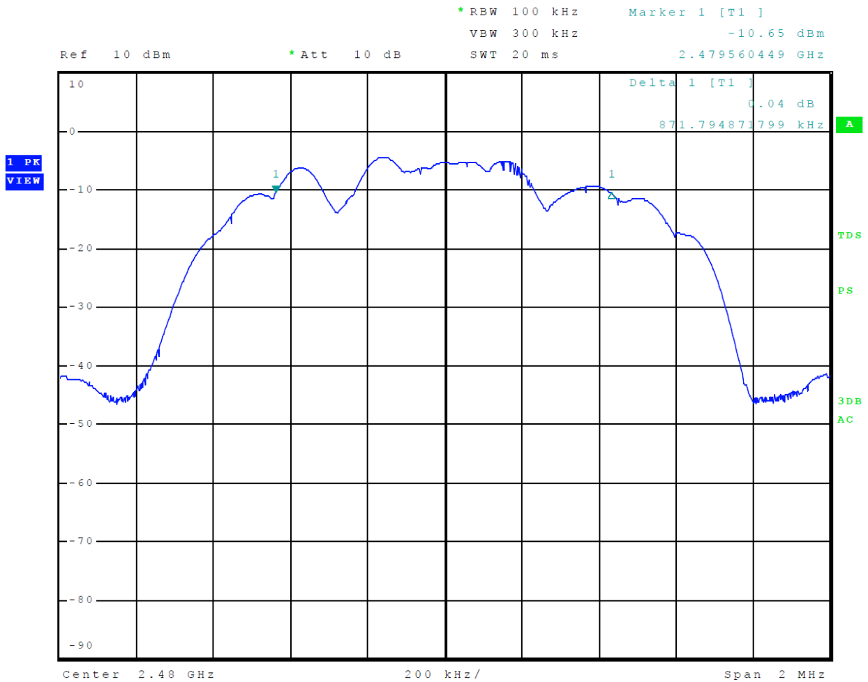
Figure 28 Plot of 6-dB Occupied Bandwidth Mode 3 BT 3EDR
