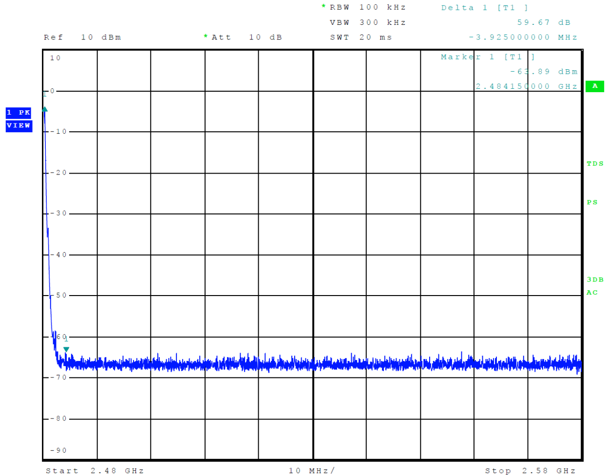
Figure 21 Plot of Transmitter Emissions High Band Edge Mode 4 BT BLE
