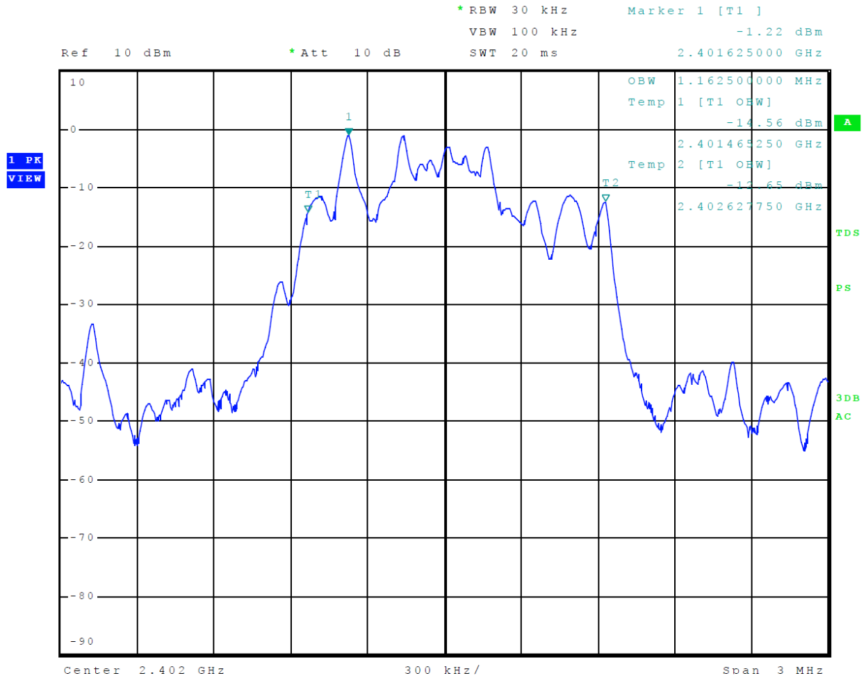
Figure 27 Plot of 99% Occupied Bandwidth Mode 2 BT 2EDR
