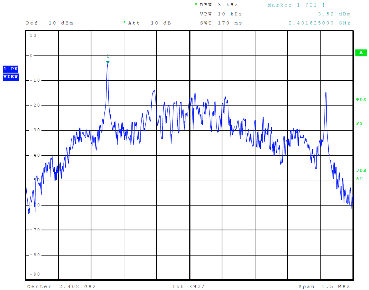
Figure 40 Plot of Transmitter Power Spectral Density Mode 2 BT 2EDR
