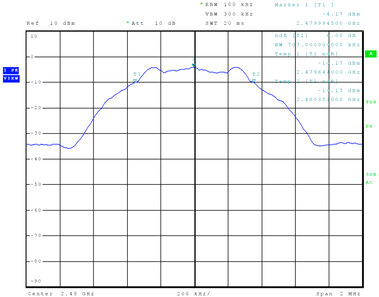
Figure 30 Plot of 6-dB Occupied Bandwidth Mode 4 BT BLE
