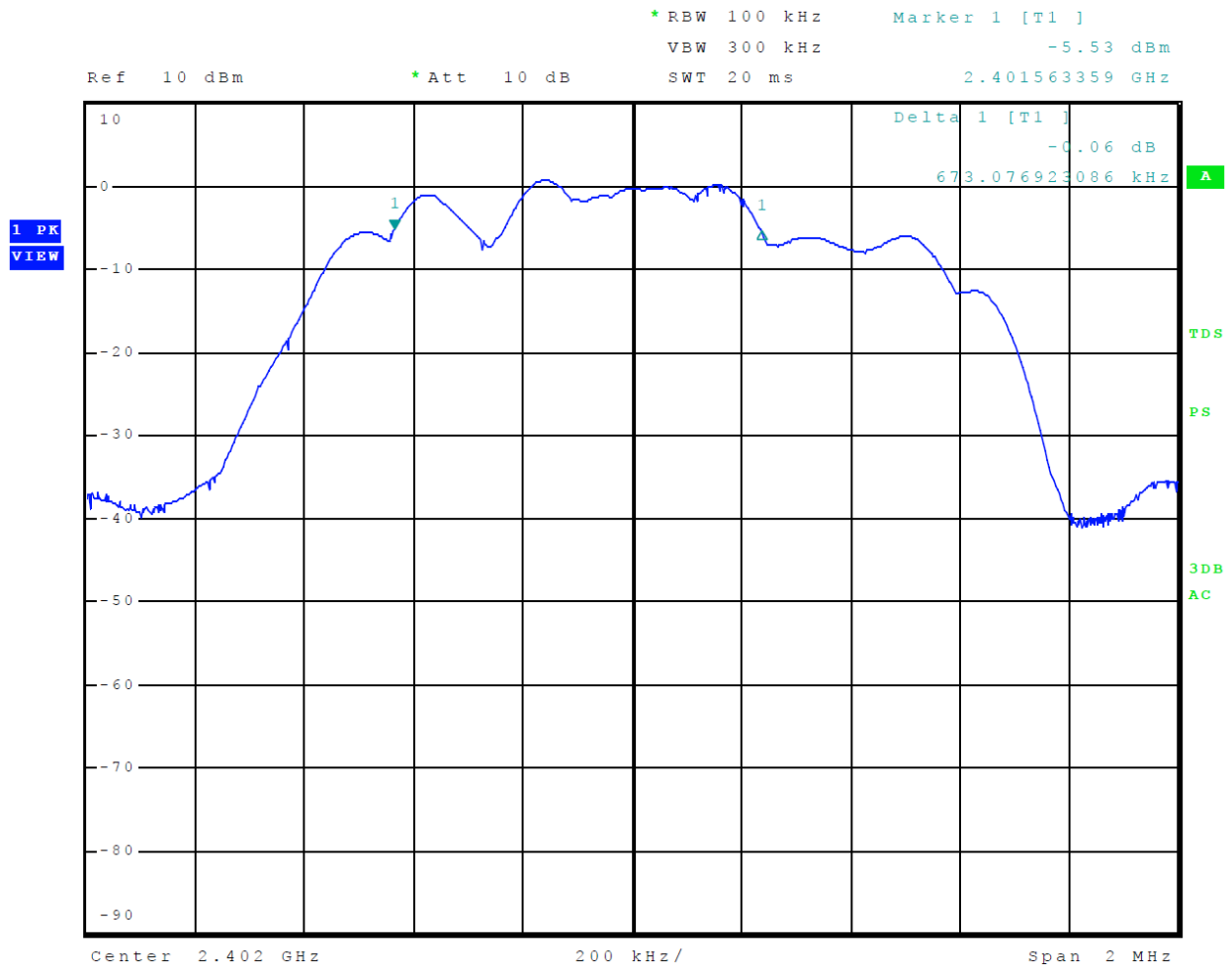
Figure 26 Plot of 6-dB Occupied Bandwidth Mode 2 BT 2EDR
