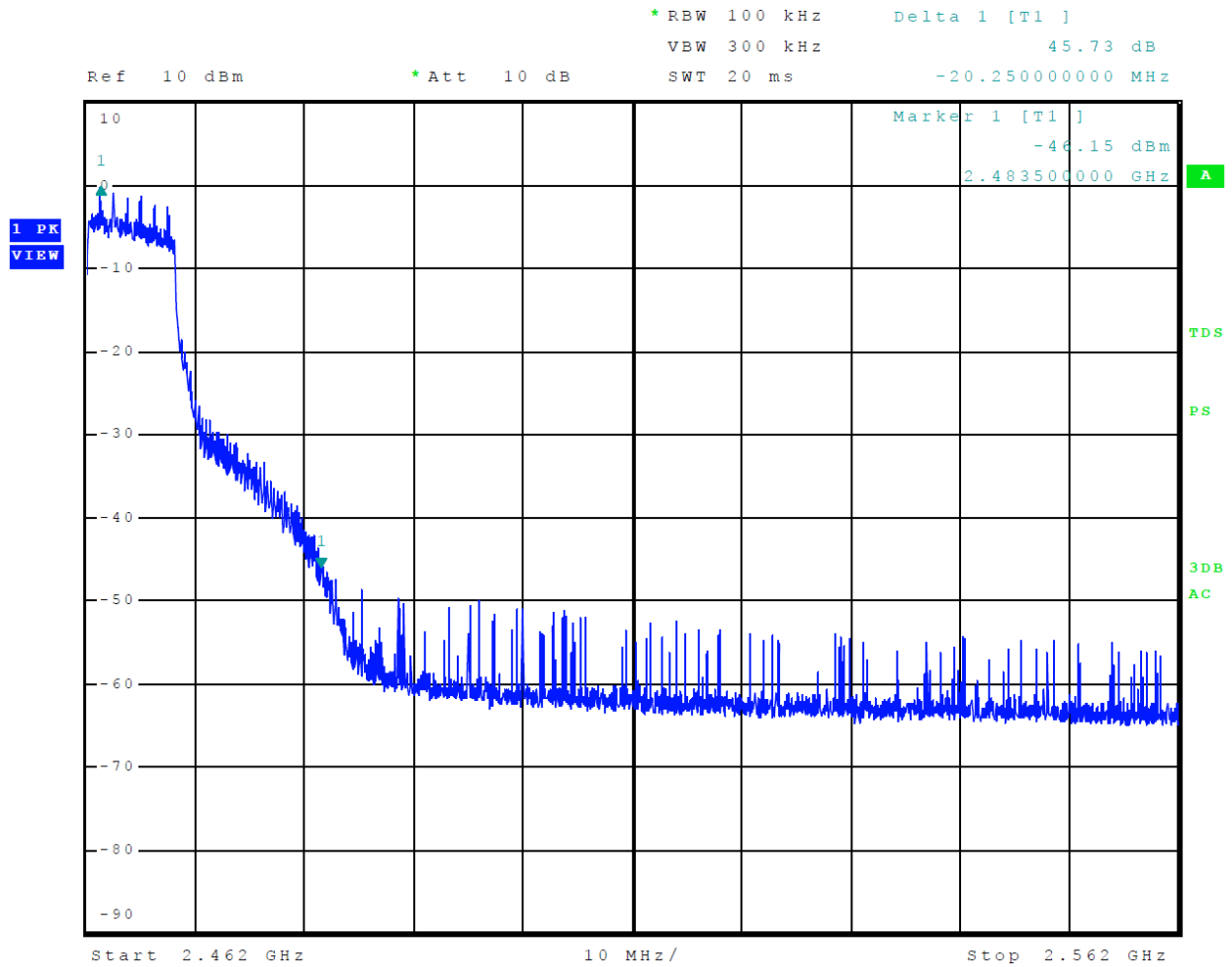
Figure 23 Plot of Transmitter Emissions High Band Edge Mode 6 802.11g
