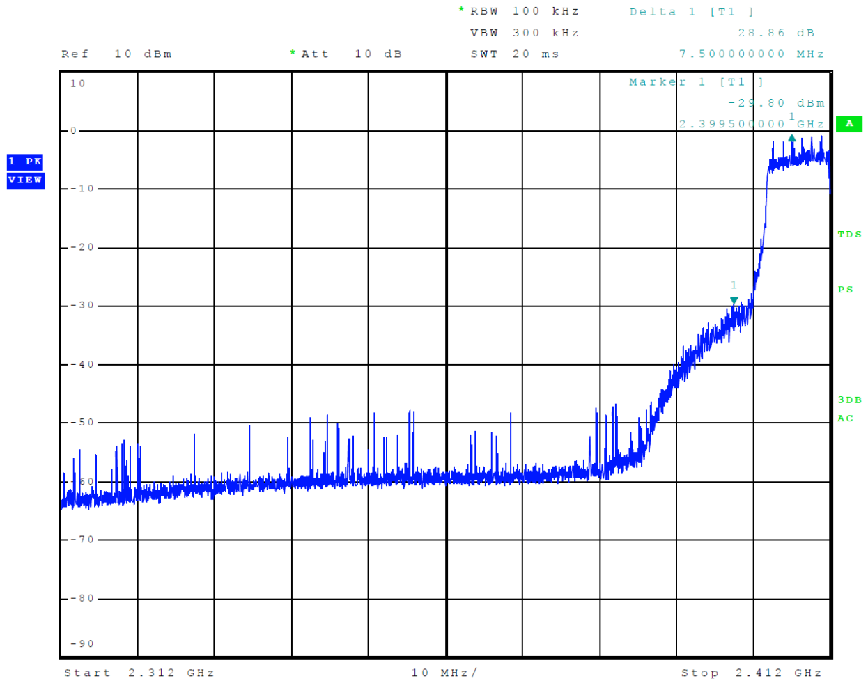
Figure 16 Plot of Transmitter Emissions Low Band Edge Mode 6 802.11g
