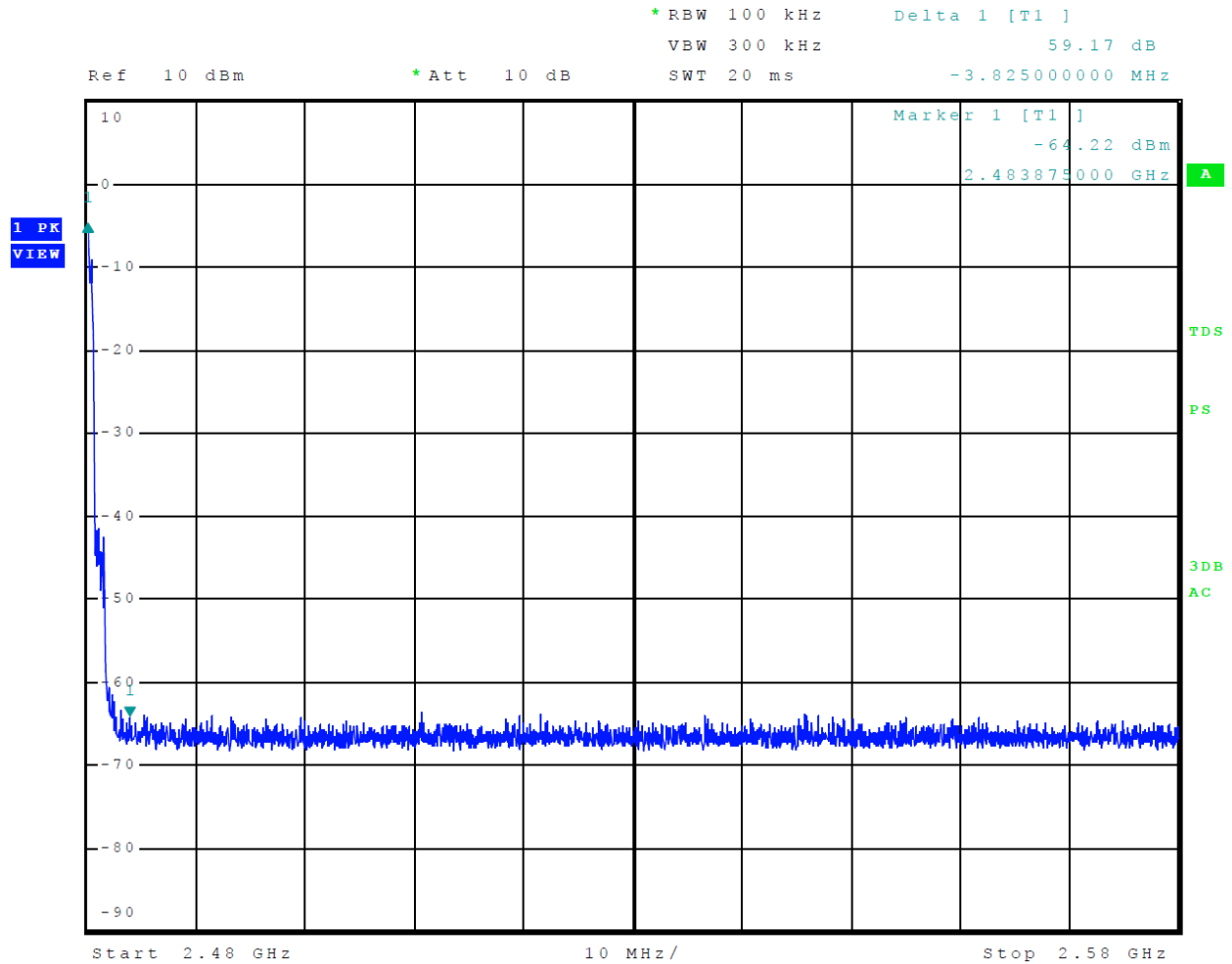
Figure 20 Plot of Transmitter Emissions High Band Edge Mode 3 BR 3EDR
