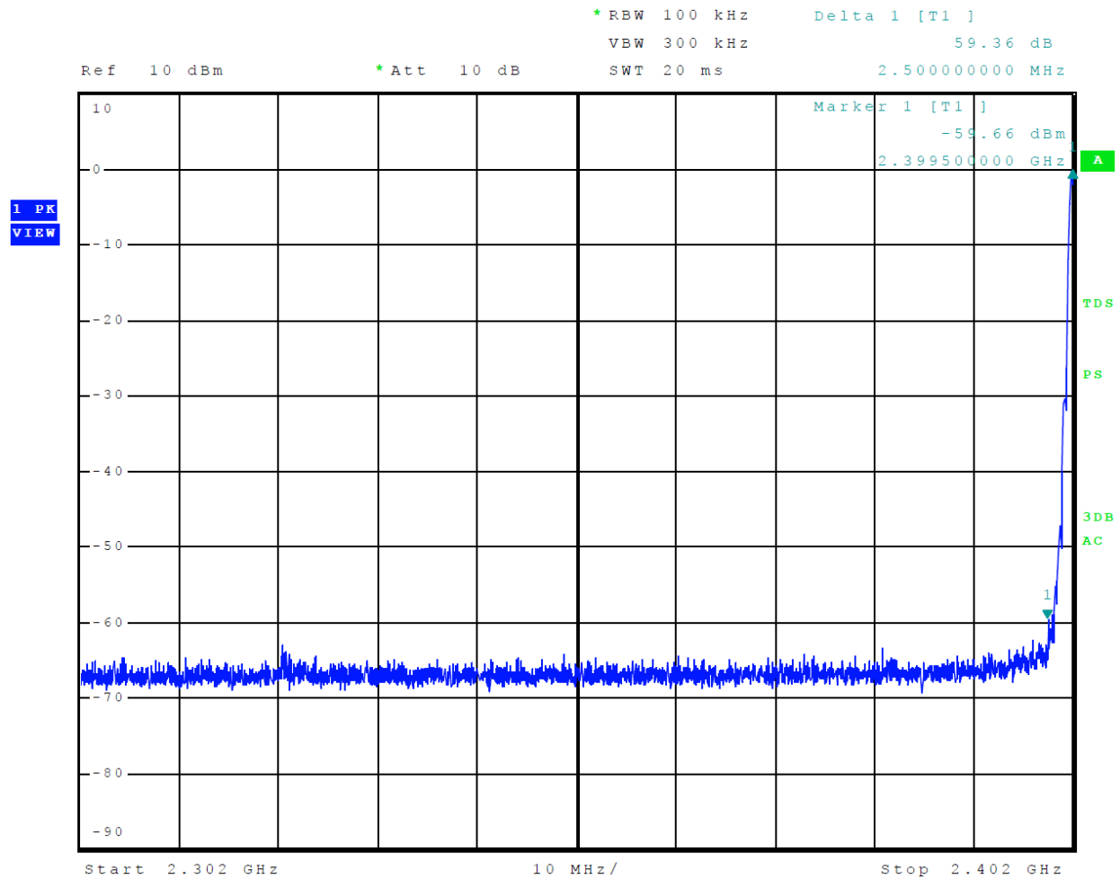
Figure 14 Plot of Transmitter Emissions Low Band Edge Mode 4 BT BLE
