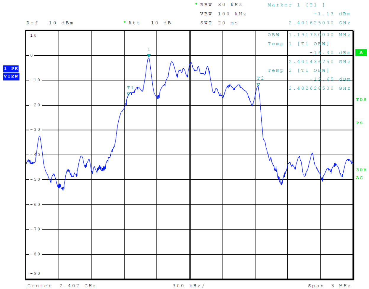
Figure 29 Plot of 99% Occupied Bandwidth Mode 3 BT 3EDR
