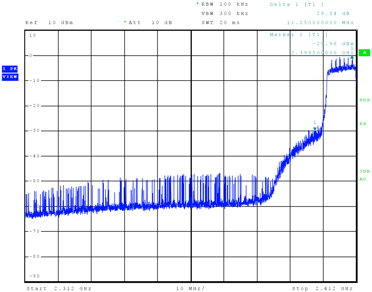
Figure 17 Plot of Transmitter Emissions Low Band Edge Mode 7 802.11n
