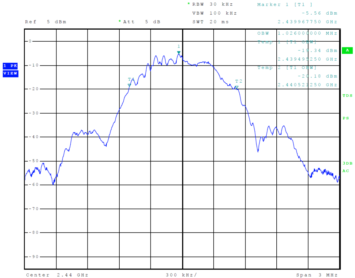
Figure 31 Plot of 99% Occupied Bandwidth Mode 4 BT BLE
