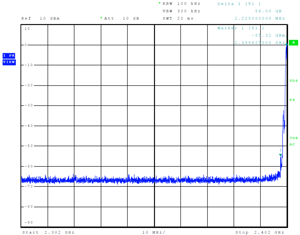
Figure 13 Plot of Transmitter Emissions Low Band Edge Mode 3 BT 3EDR
