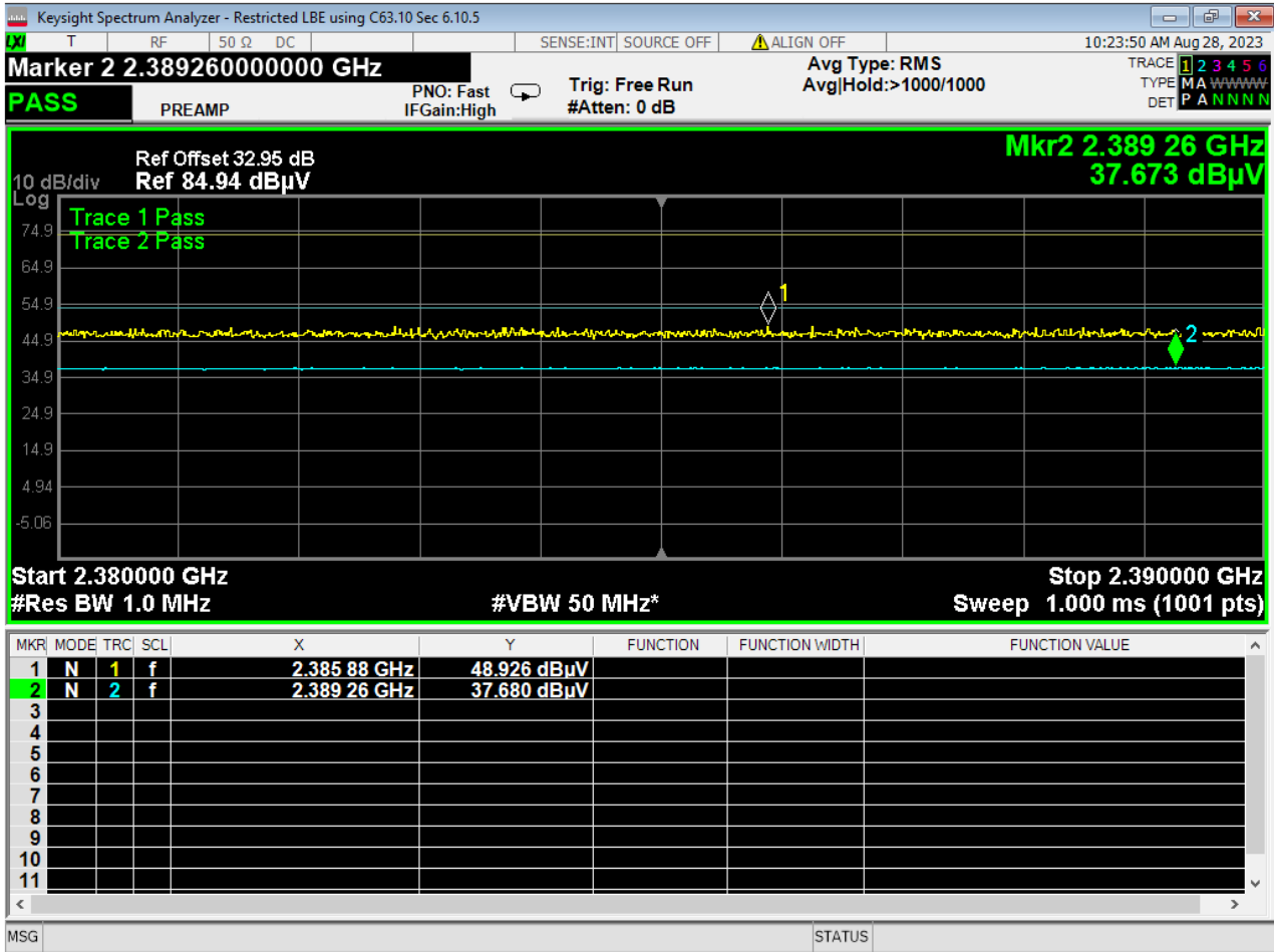
25 Lower Bandedge, Restricted, GMSK 1MB
