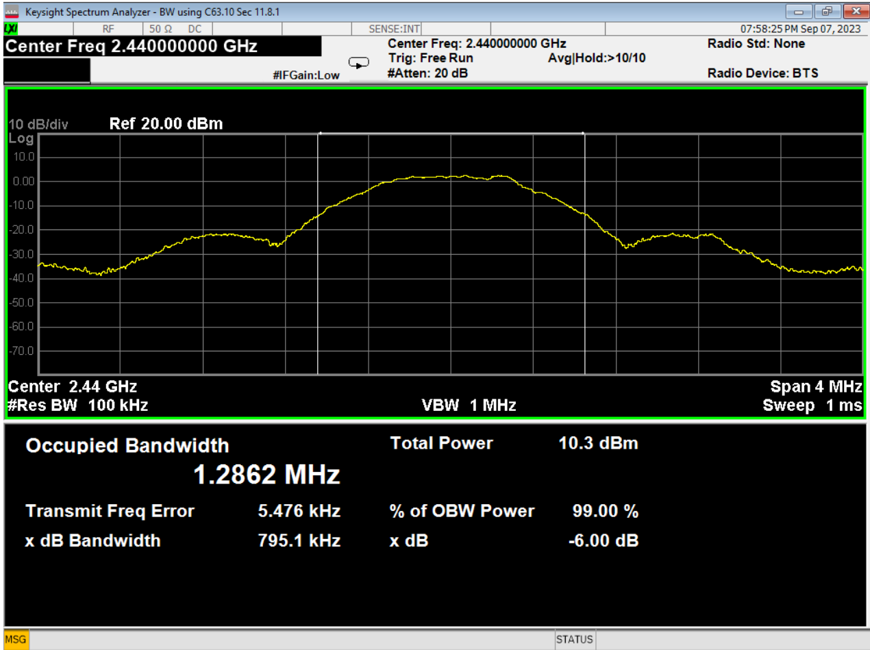
18 6dB Bandwidth, Mid Channel, GMSK 1MB
