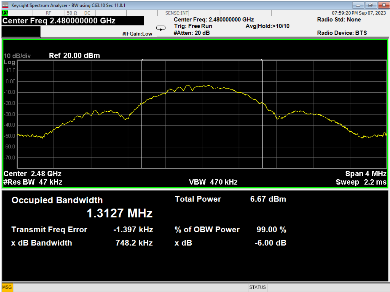
45 Occupied Bandwidth, High Channel, GMSK 1MB
