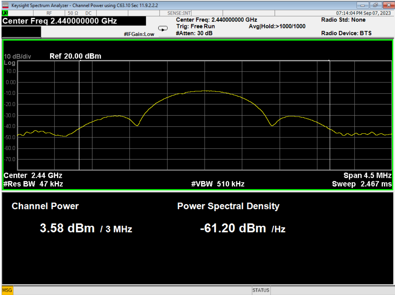
15 Average Power, Mid Channel, GMSK 1MB
