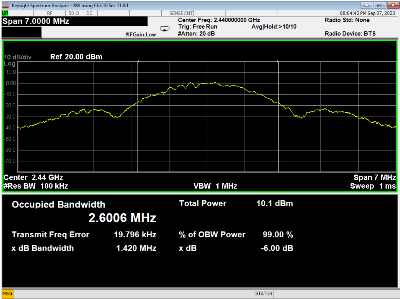
31 6dB Bandwidth, Mid Channel, GMSK 2MB
