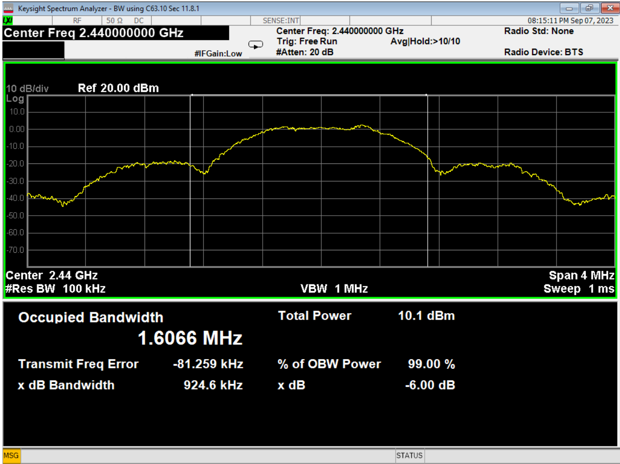
05 6dB Bandwidth, Mid Channel, GFSK
