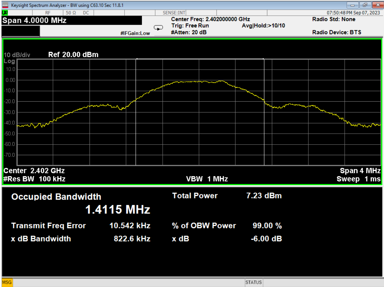
17 6dB Bandwidth, Low Channel, GMSK 1MB
