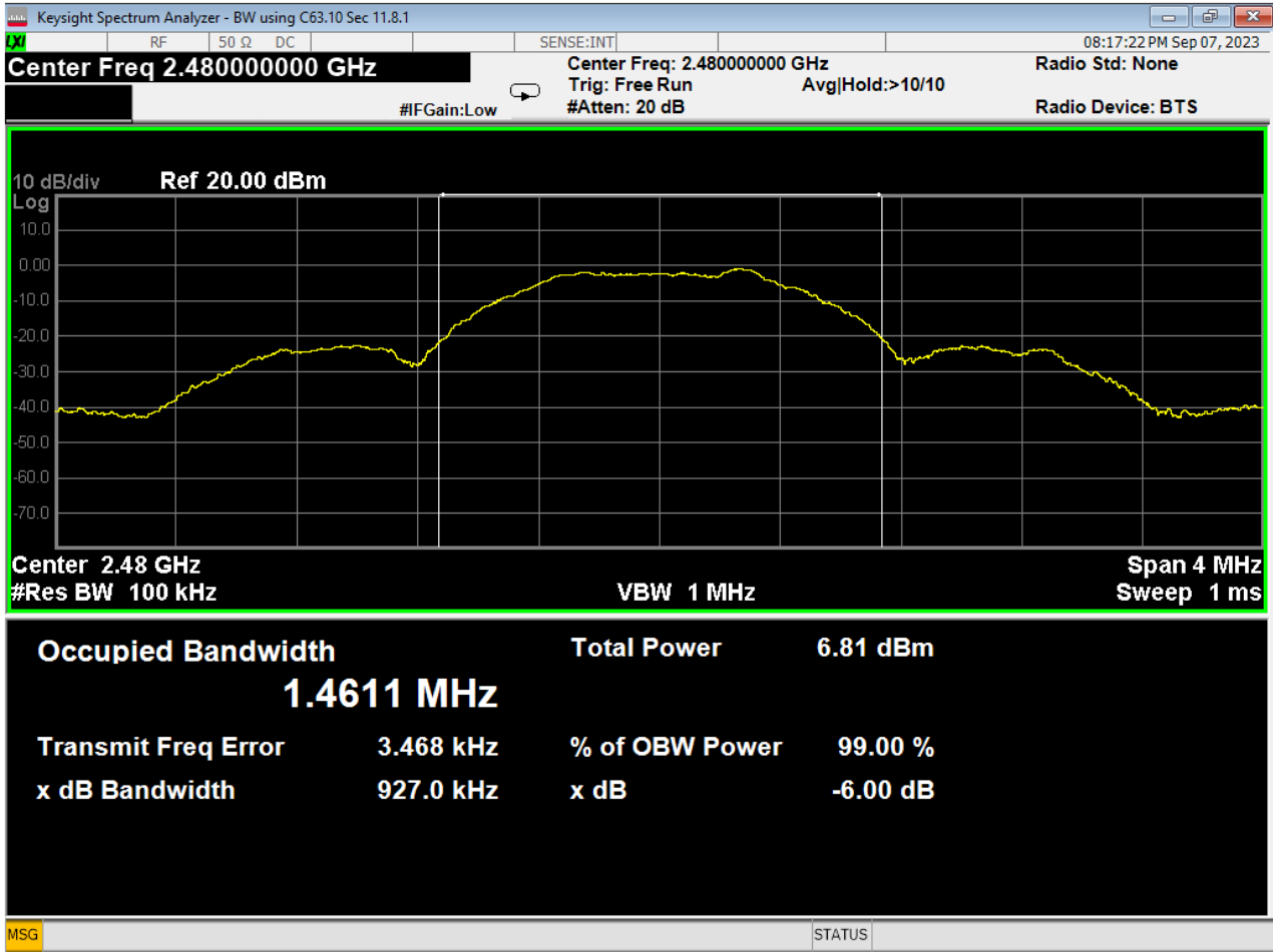
06 6dB Bandwidth, High Channel, GFSK
