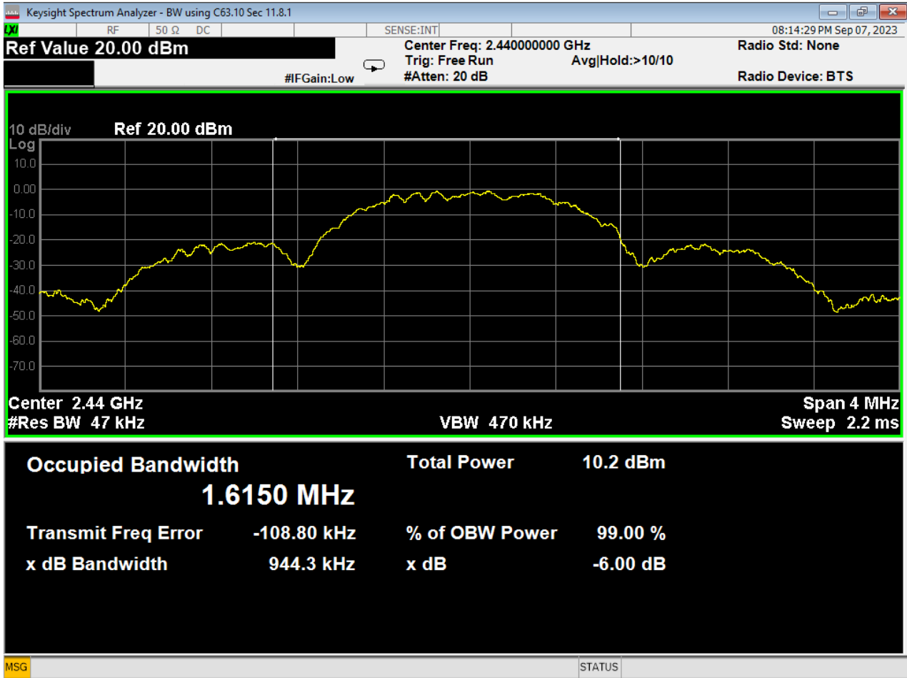
41 Occupied Bandwidth, Mid Channel, GFSK
