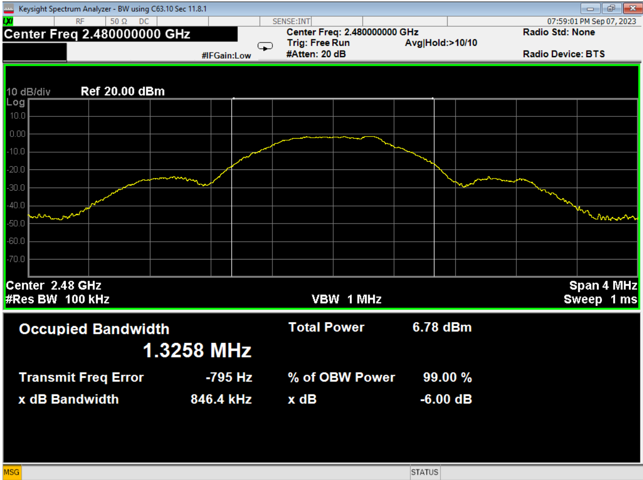
19 6dB Bandwidth, High Channel, GMSK 1MB
