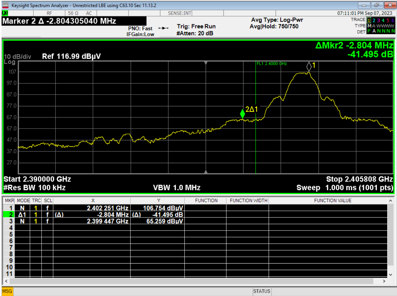
23 Lower Bandedge, Unrestricted, GMSK 1MB
