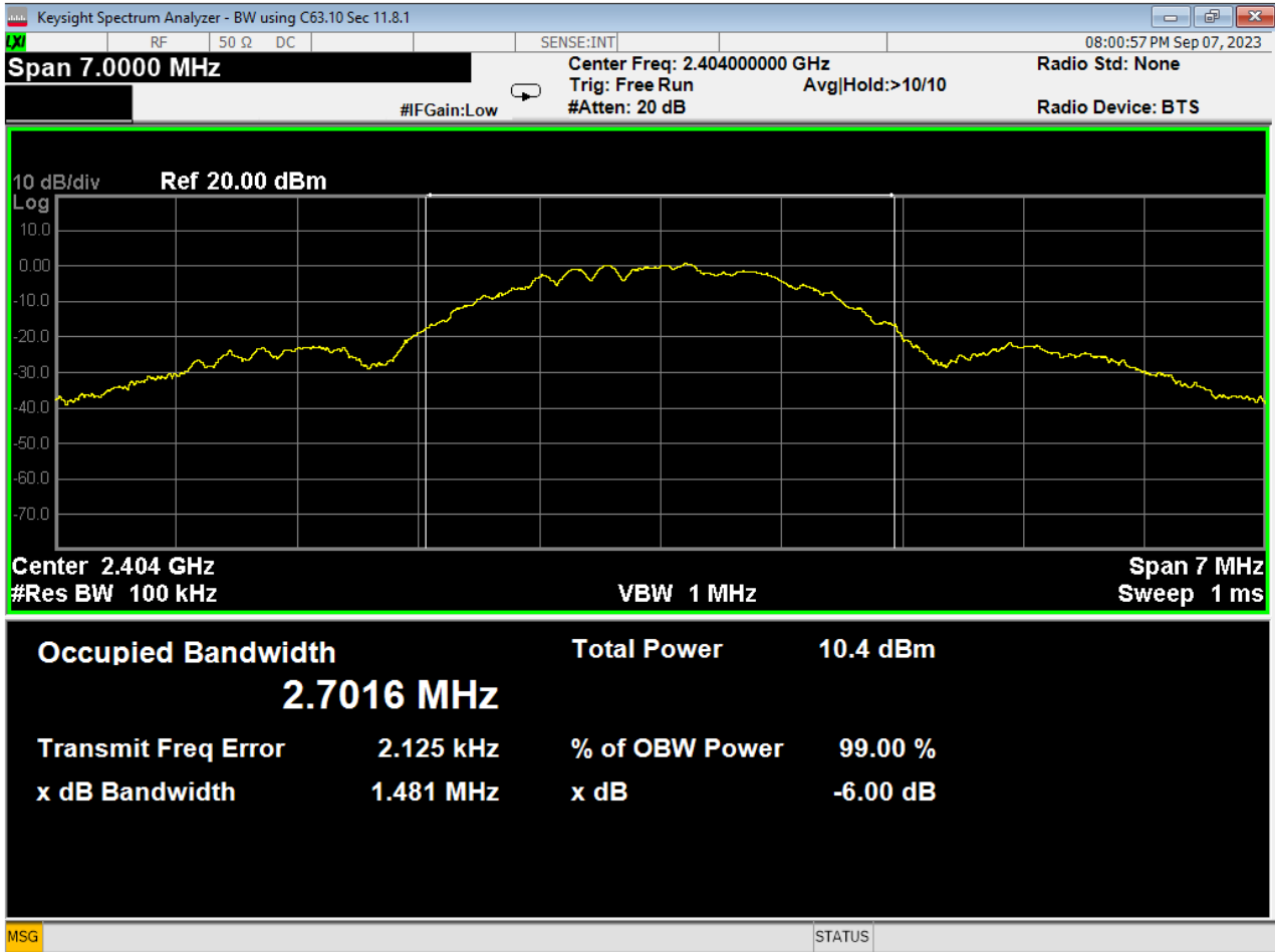
30 6dB Bandwidth, Low Channel, GMSK 2MB
