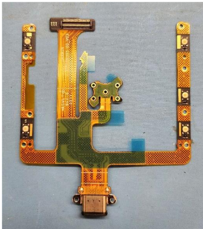
FPC Back
