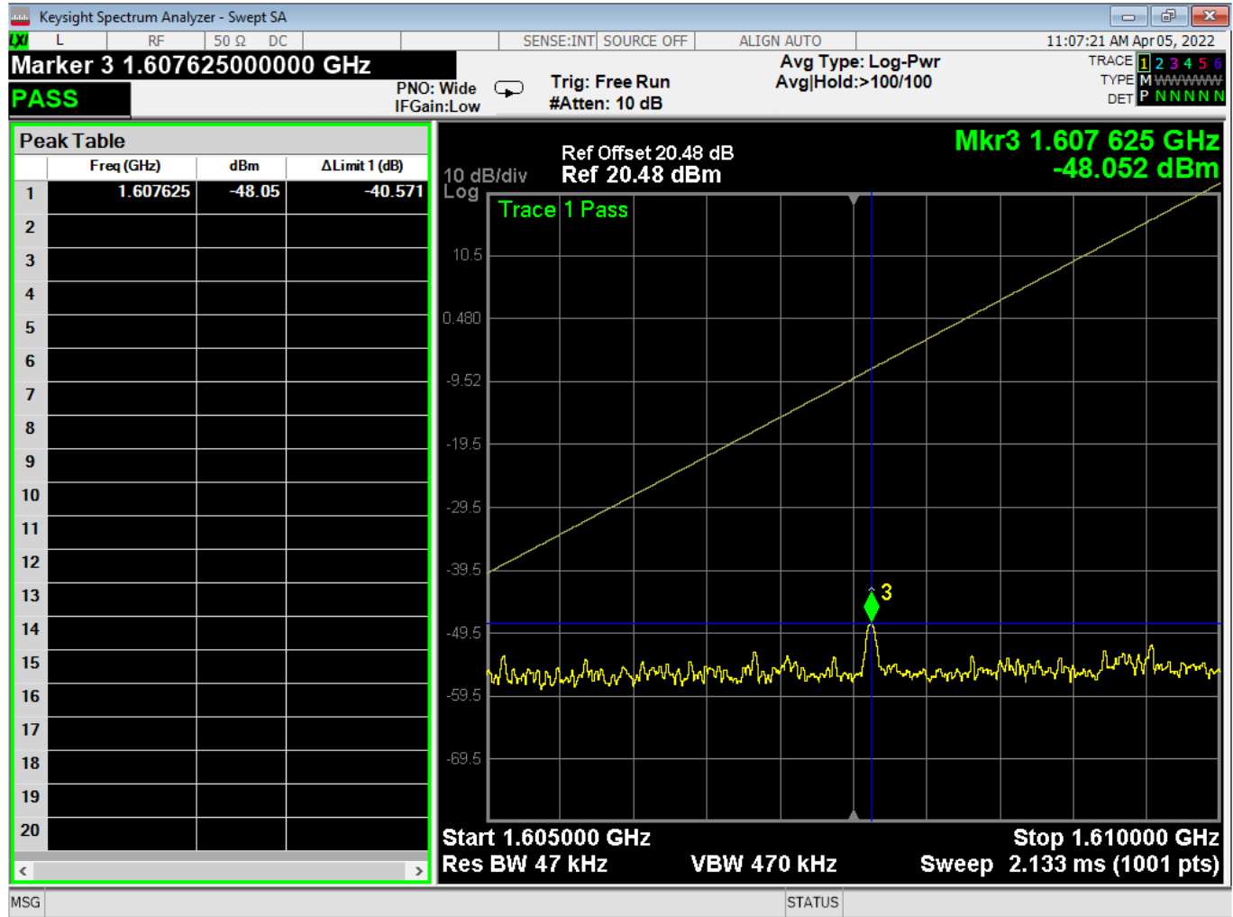
Figure 11 – Part 25.216(g), Transmitting at 1616.020752 MHz, Conducted Measurement *Limits have been converted from dBW to dBm. \text{dBW} = \text{dBm} + 30 Margin shown in the plot does not include antenna gain.
