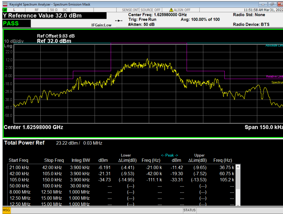
Figure 7 – Part 25.202(f) Mask, Transmitting at 1625.979126 MHz
