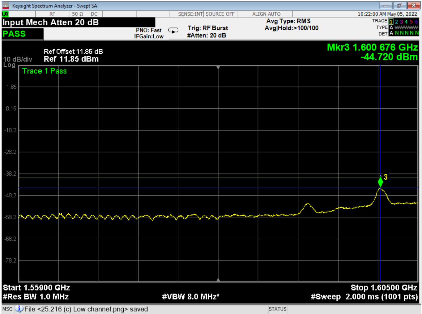
Figure 10 – Part 25.216(c), Transmitting at 1625.979126 MHz, Conducted Measurement *Limits have been converted from dBW to dBm. dBW = dBm + 30
