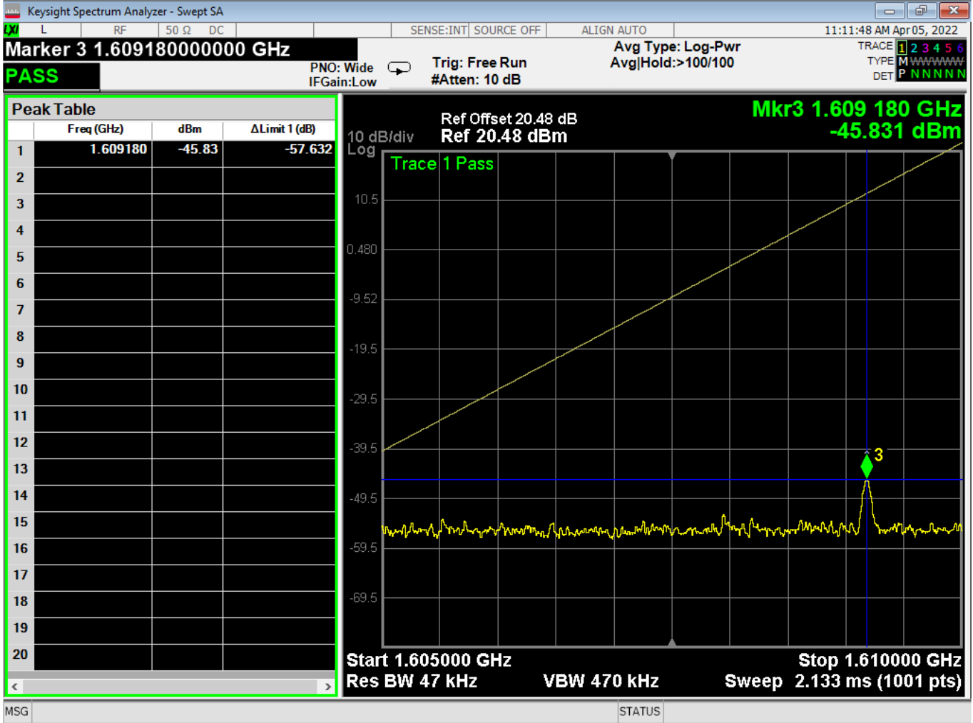
Figure 13 – Part 25.216(g), Transmitting at 1625.979126 MHz, Conducted Measurement *Limits have been converted from dBW to dBm. dBW = dBm + 30
