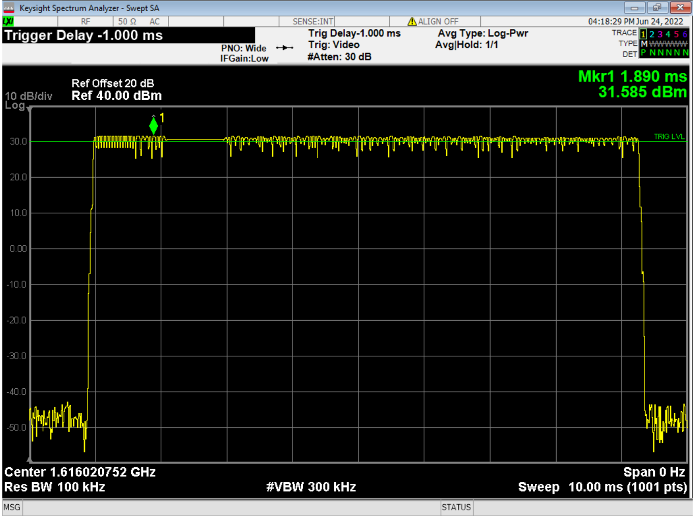
Figure 20 – Supporting Plots for modulation characteristic, Low Channel
