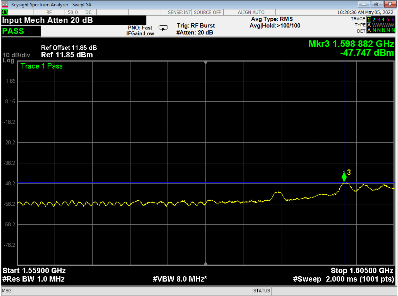
Figure 8 – Part 25.216(c), Transmitting at 1616.020752 MHz, Conducted Measurement *Limits have been converted from dBW to dBm. dBW = dBm + 30
