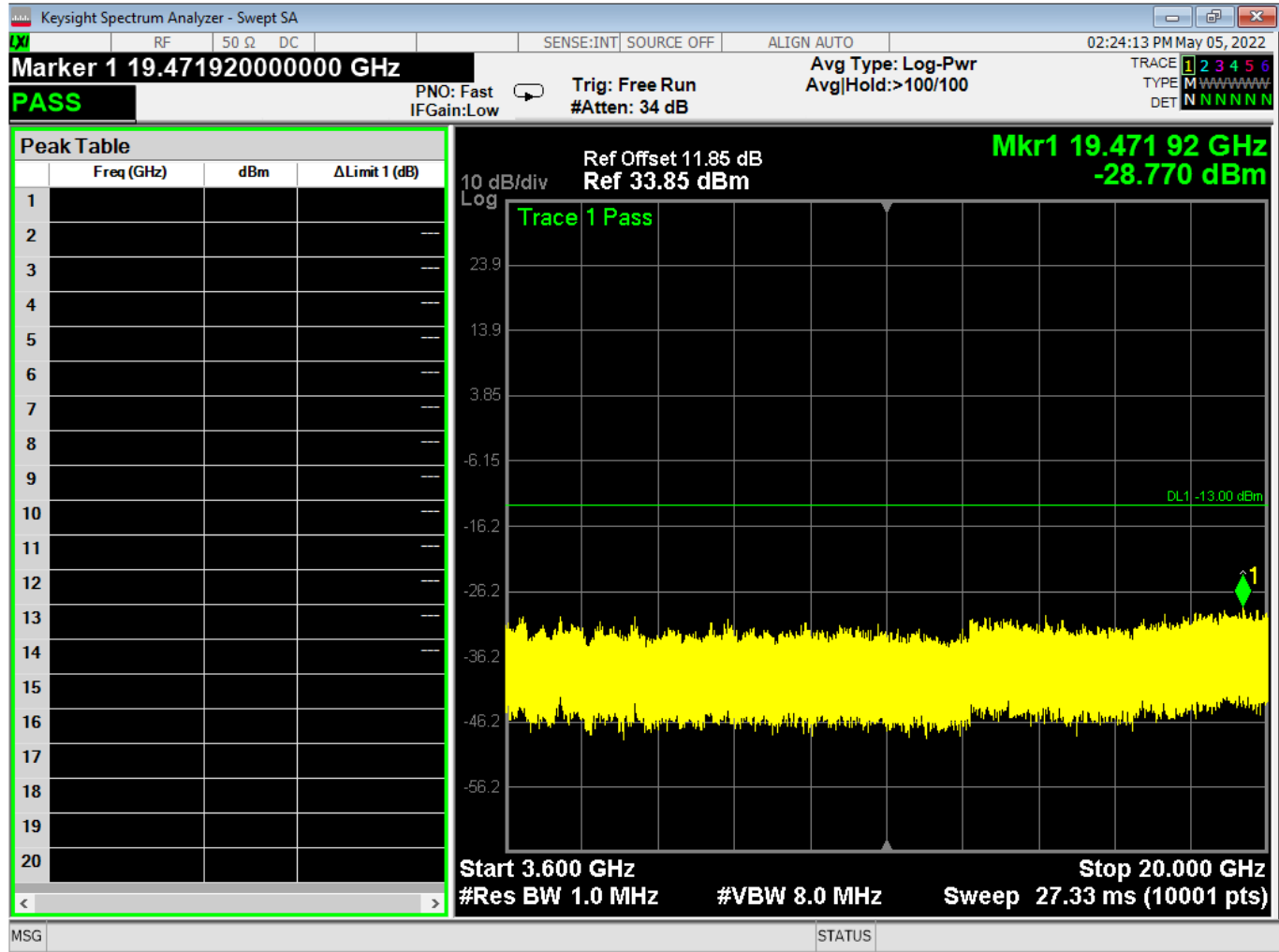
Figure 16 – Conducted Spurious Plot, 3.6G – 20G
