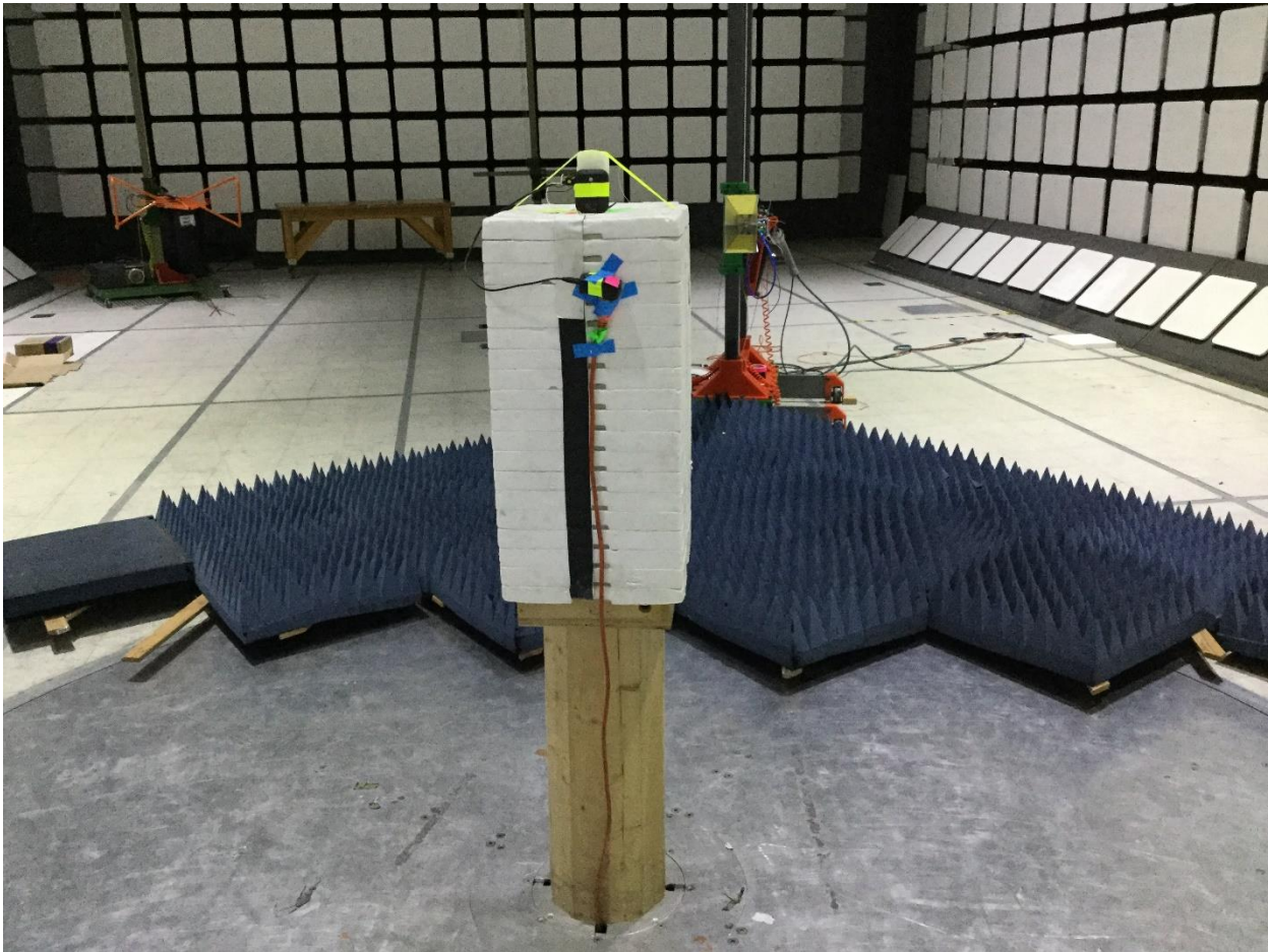
1 – 26 GHz Test Setup
