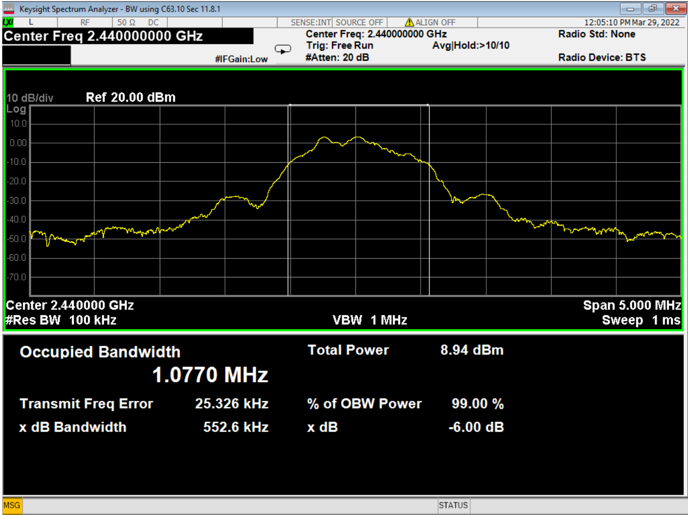
5 Bandwidth, Mid Channel, GMSK
