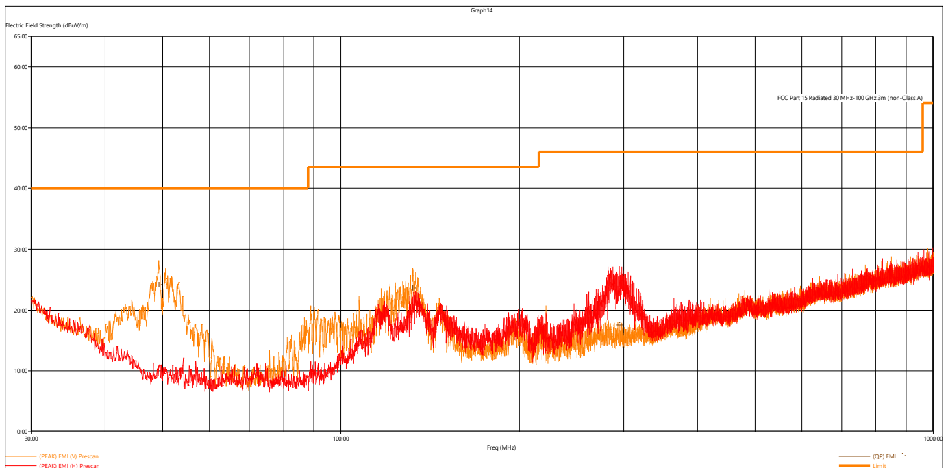
Figure 5 - Radiated Emissions Plot, GMSK
