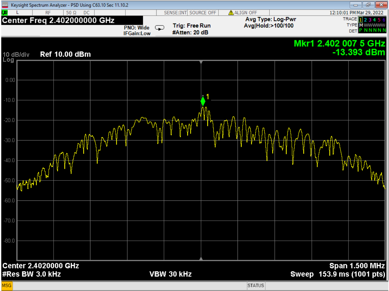
7 PSD, Low Channel, GMSK
