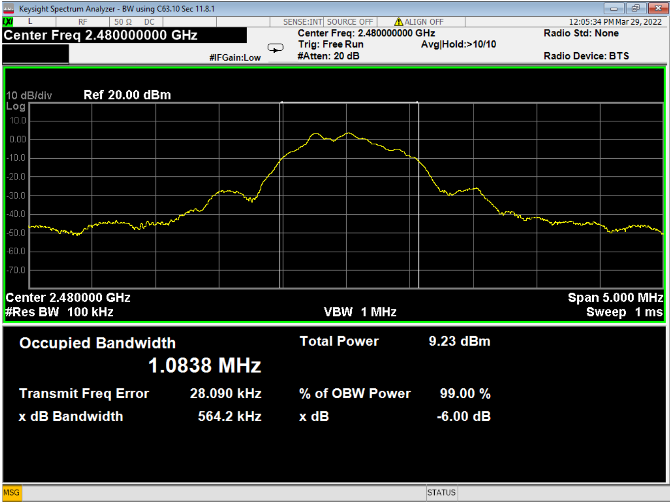
6 Bandwidth, High Channel, GMSK
