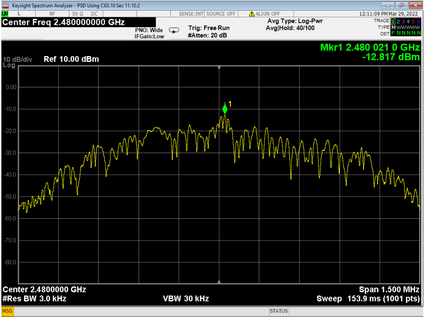
9 PSD, High Channel, GMSK
