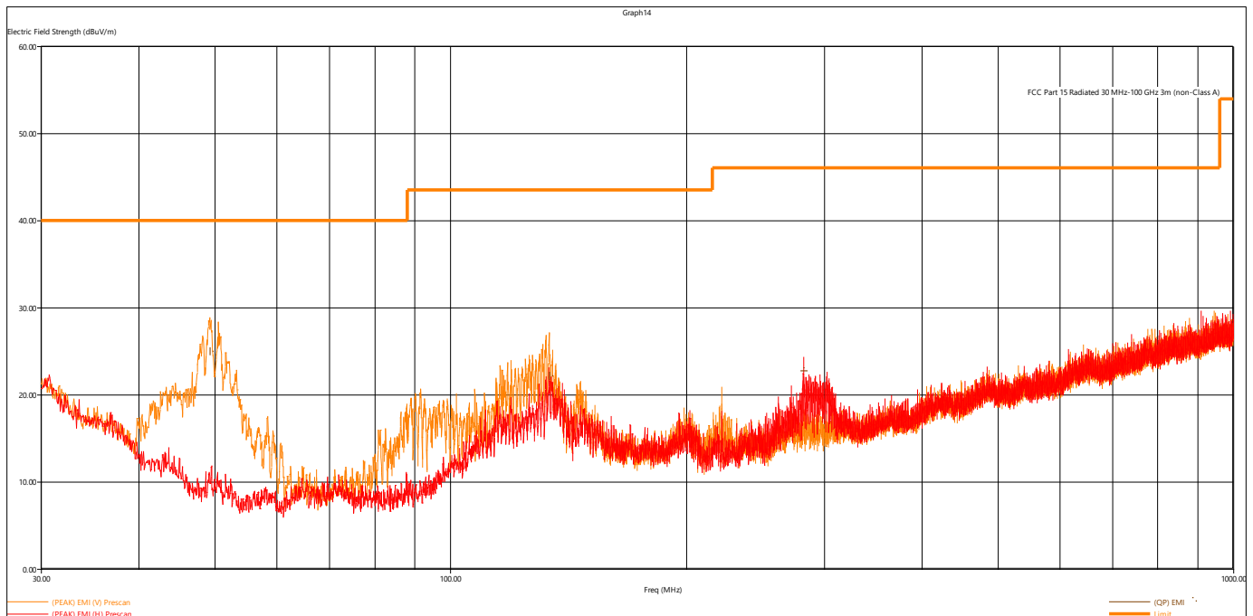
Figure 5 - Radiated Emissions Plot, Low Channel, GFSK
