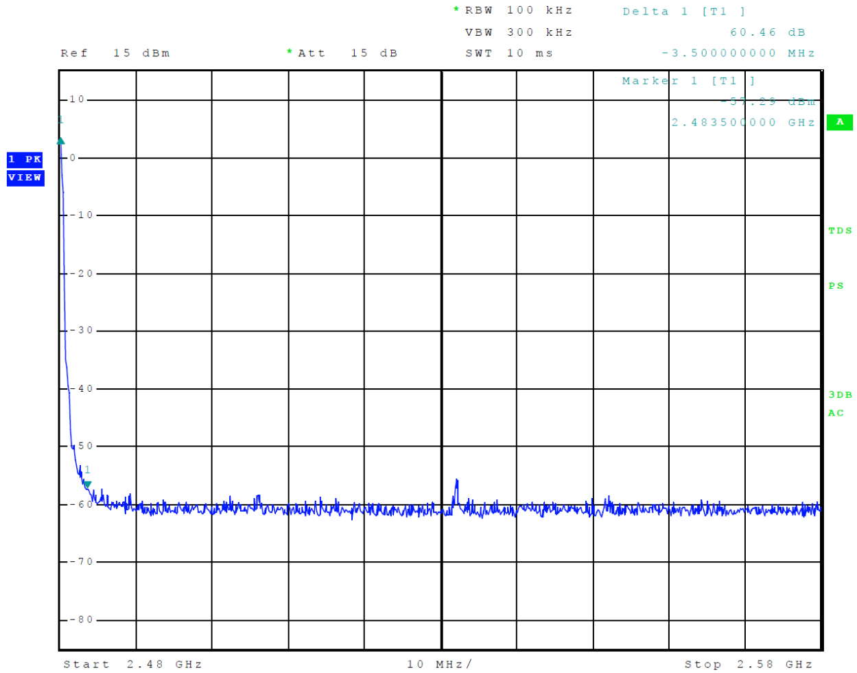
Figure 10 Plot of Transmitter Emissions High Band Edge Mode 3 BT 2EDR
