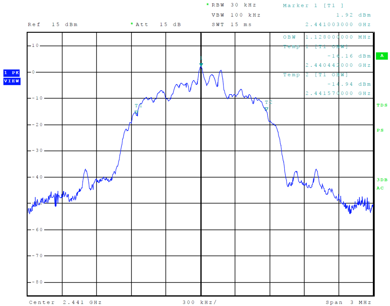
Figure 13 Plot of 99% Occupied Bandwidth Mode 2 BT 2EDR
