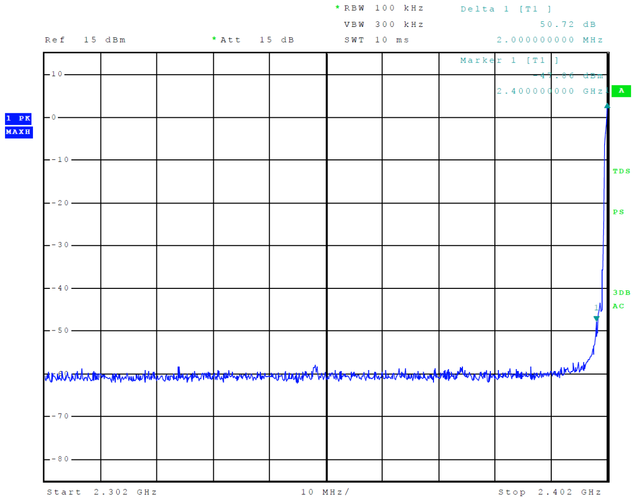
Figure 7 Plot of Transmitter Emissions Low Band Edge Mode 3 BT 3EDR
