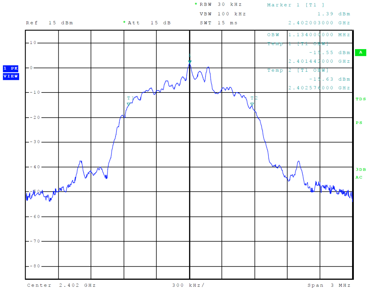
Figure 15 Plot of 99% Occupied Bandwidth Mode 3 BT 3EDR
