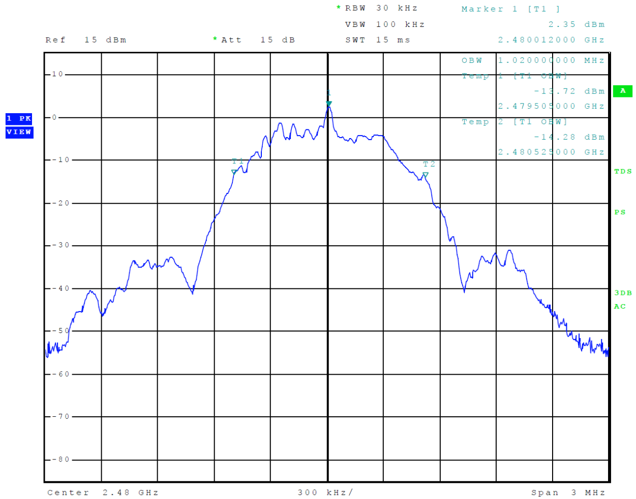
Figure 17 Plot of 99% Occupied Bandwidth Mode 4 BT BLE
