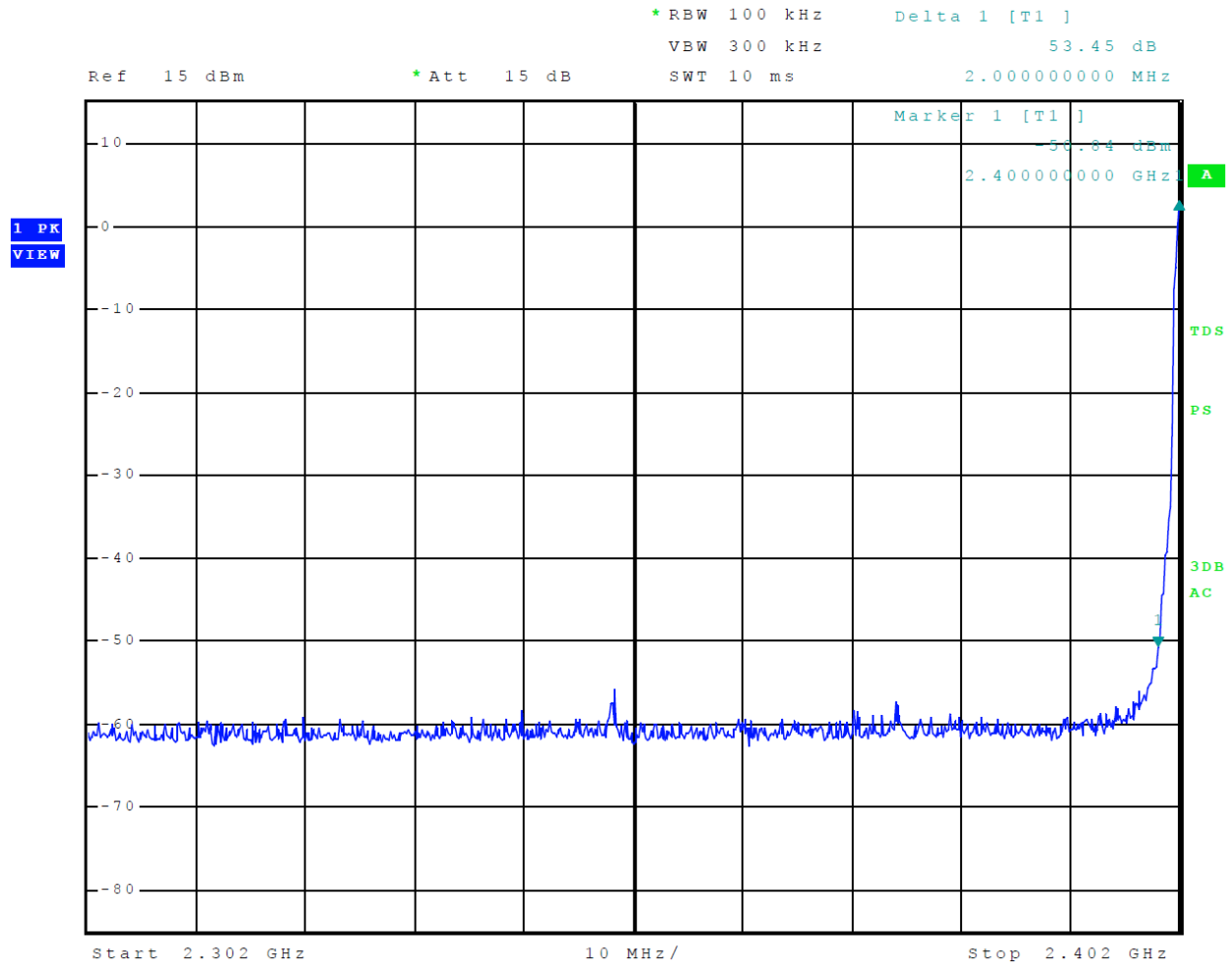
Figure 6 Plot of Transmitter Emissions Low Band Edge Mode 2 BT 2EDR
