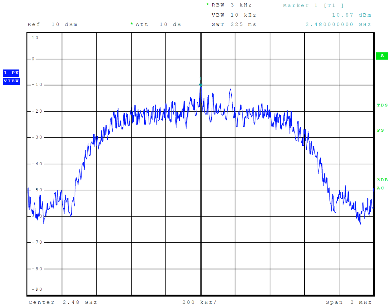
Figure 19 Plot of Transmitter Power Spectral Density Mode 3 BT 3EDR
