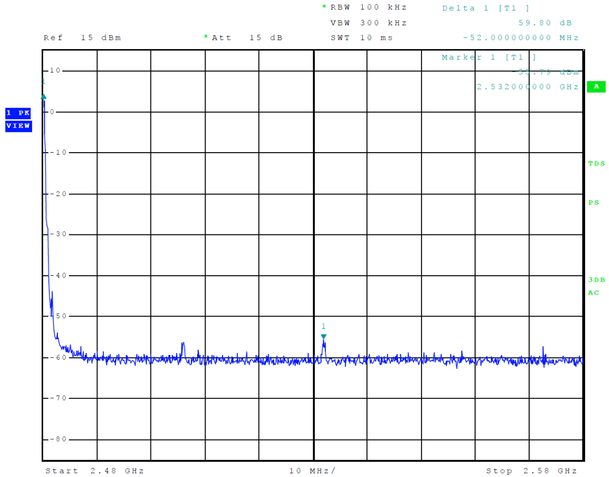
Figure 11 Plot of Transmitter Emissions High Band Edge Mode 4 BT BLE
