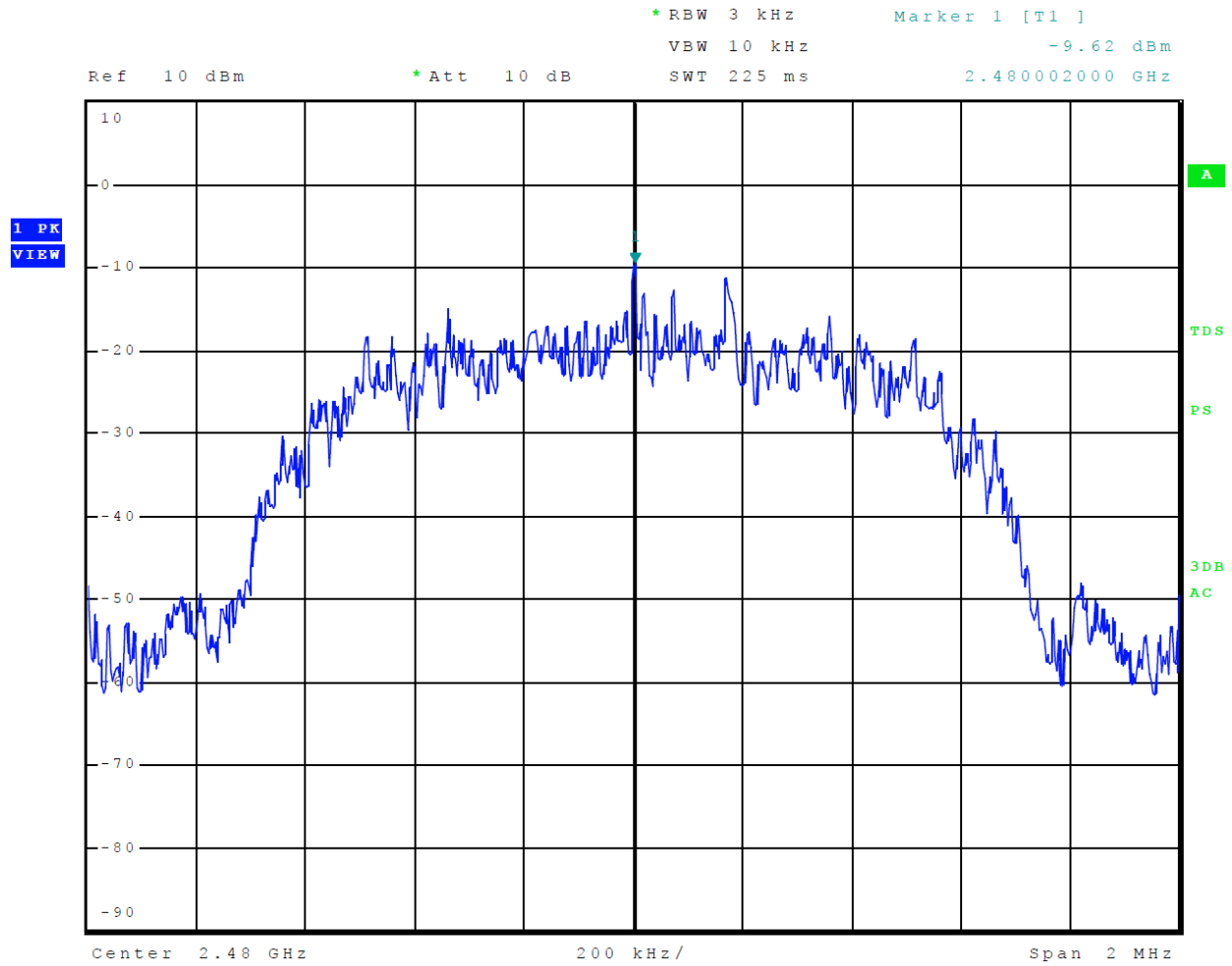
Figure 18 Plot of Transmitter Power Spectral Density Mode 2 BT 2EDR
