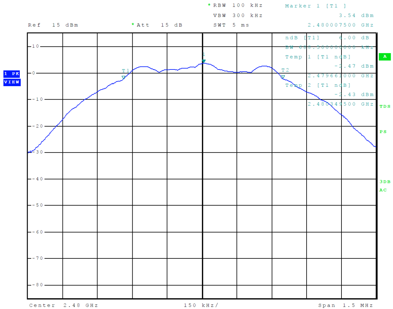
Figure 16 Plot of 6-dB Occupied Bandwidth Mode 4 BT BLE
