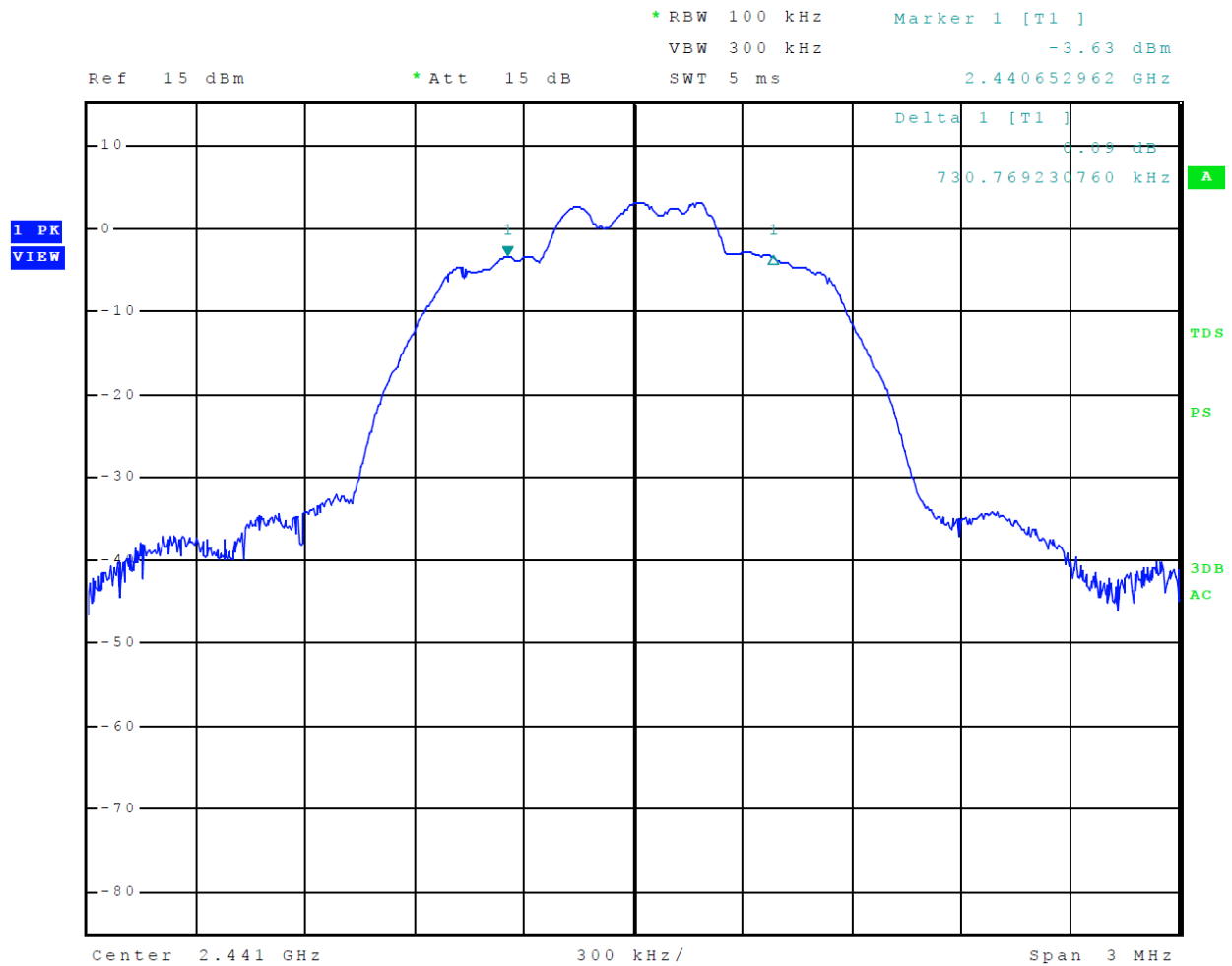
Figure 12 Plot of 6-dB Occupied Bandwidth Mode 2 BT 2EDR
