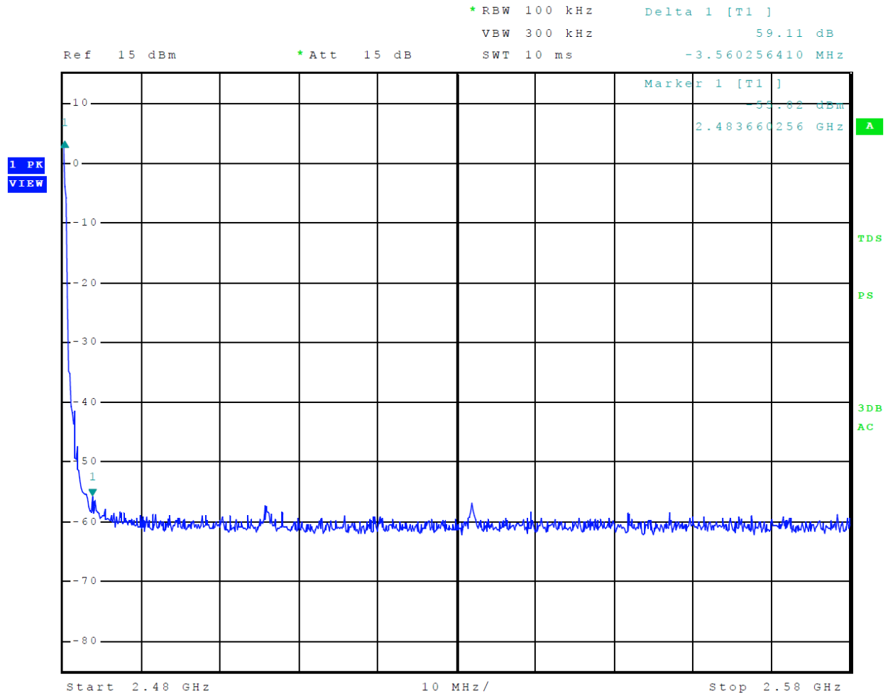
Figure 9 Plot of Transmitter Emissions High Band Edge Mode 2 BT 2EDR
