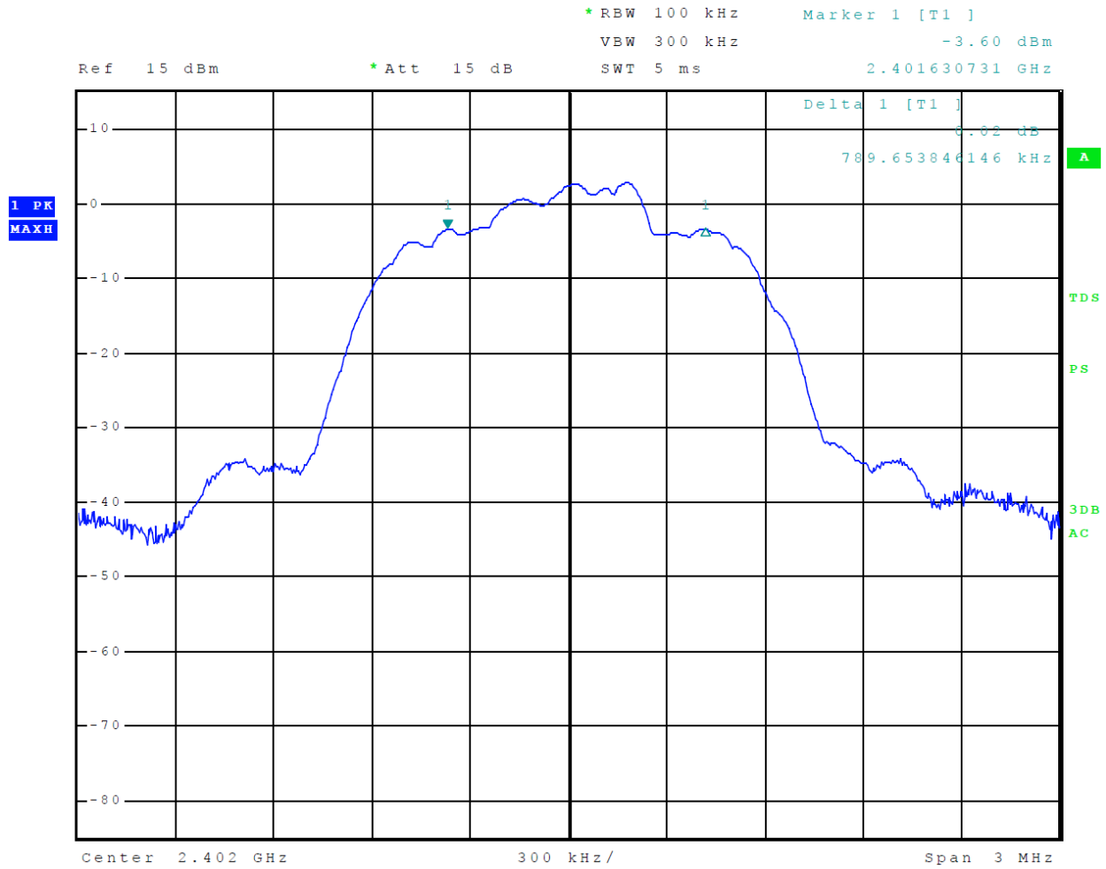
Figure 14 Plot of 6-dB Occupied Bandwidth Mode 3 BT 3EDR
