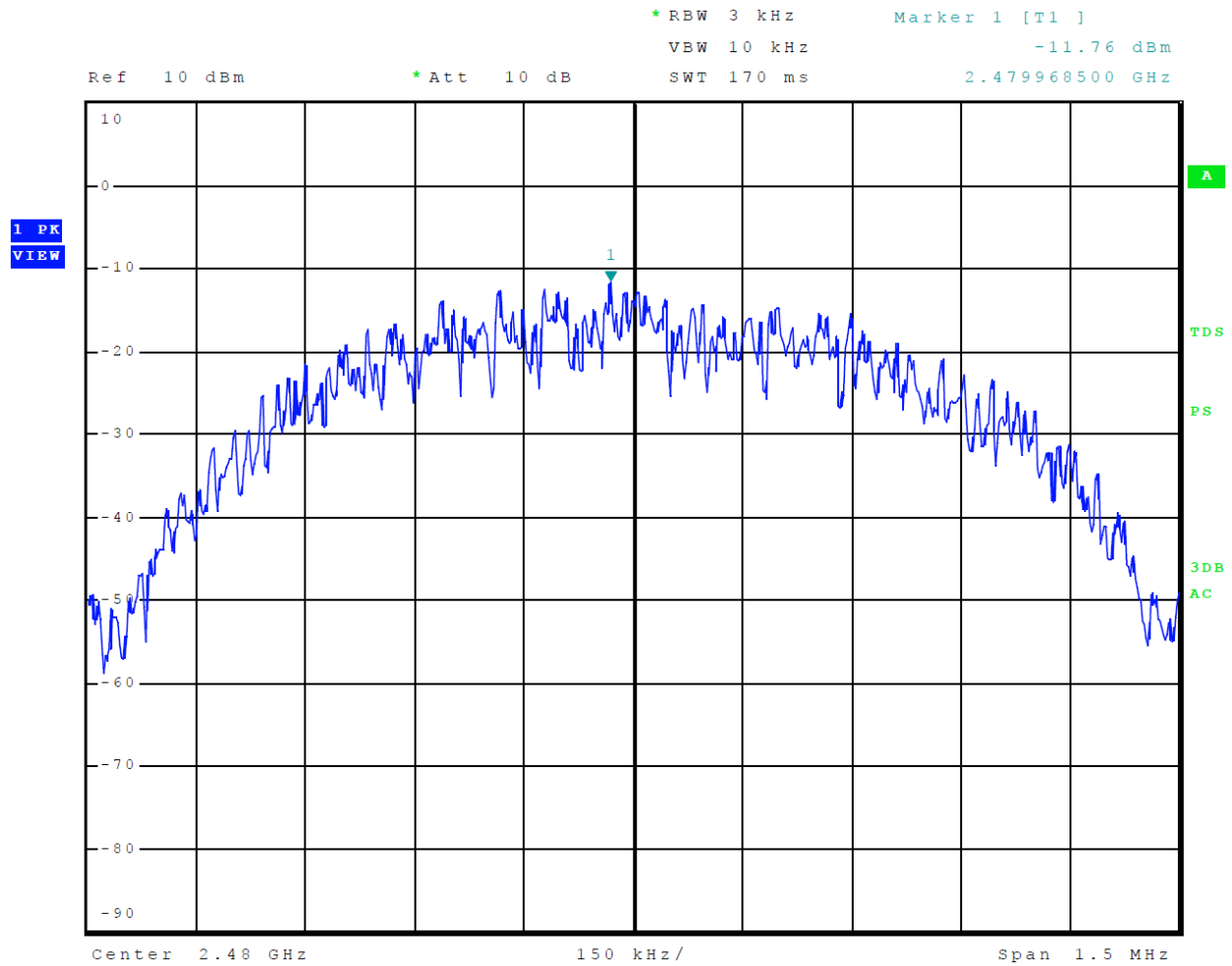
Figure 20 Plot of Transmitter Power Spectral Density Mode 4 BT BLE
