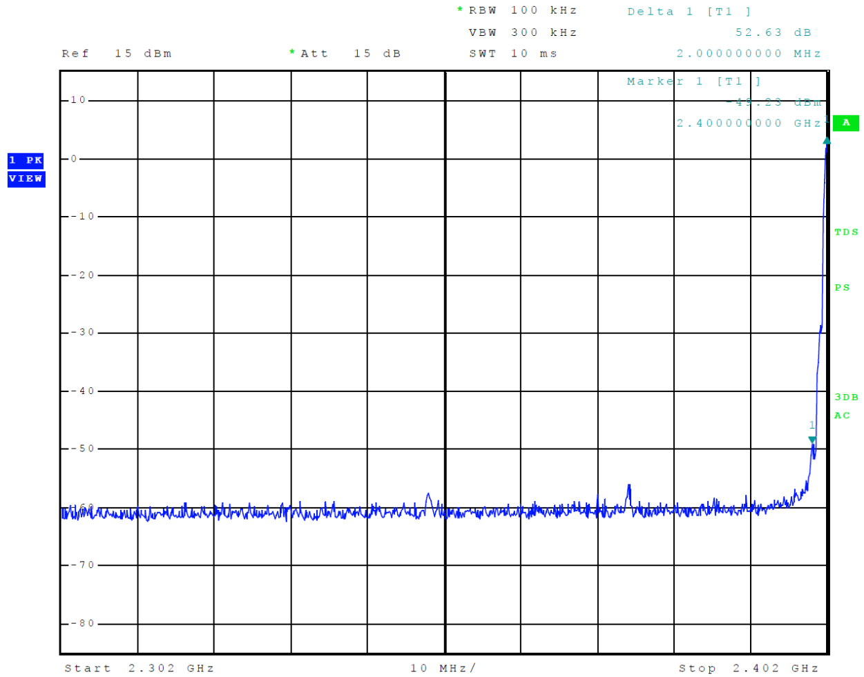
Figure 8 Plot of Transmitter Emissions Low Band Edge Mode 4 BT BLE
