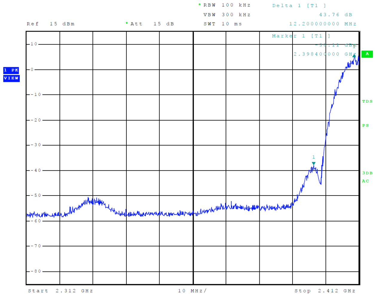
Figure 3 Plot of Transmitter Emissions Low Band Edge Mode 1 802.11b
