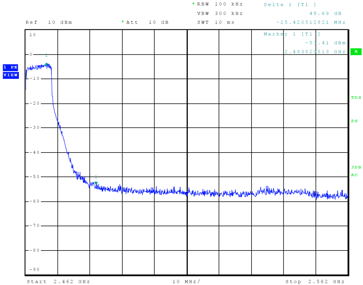
Figure 6 Plot of Transmitter Emissions High Band Edge Mode 2 802.11g
