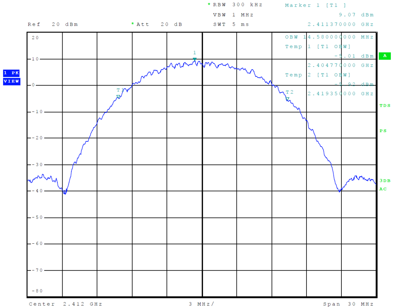
Figure 8 Plot of 99% Occupied Bandwidth Mode 1 802.11b
