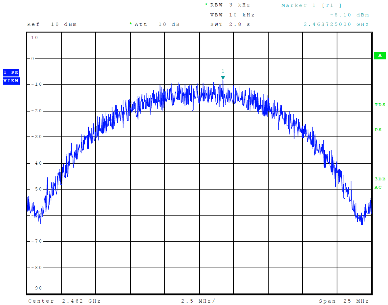
Figure 11 Plot of Transmitter Power Spectral Density Mode 1 802.11b
