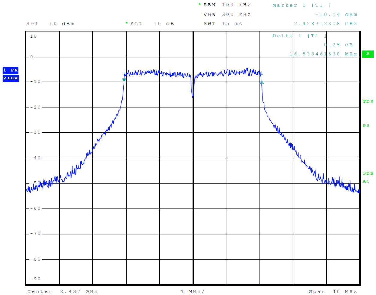
Figure 9 Plot of 6-dB Occupied Bandwidth Mode 2 802.11g
