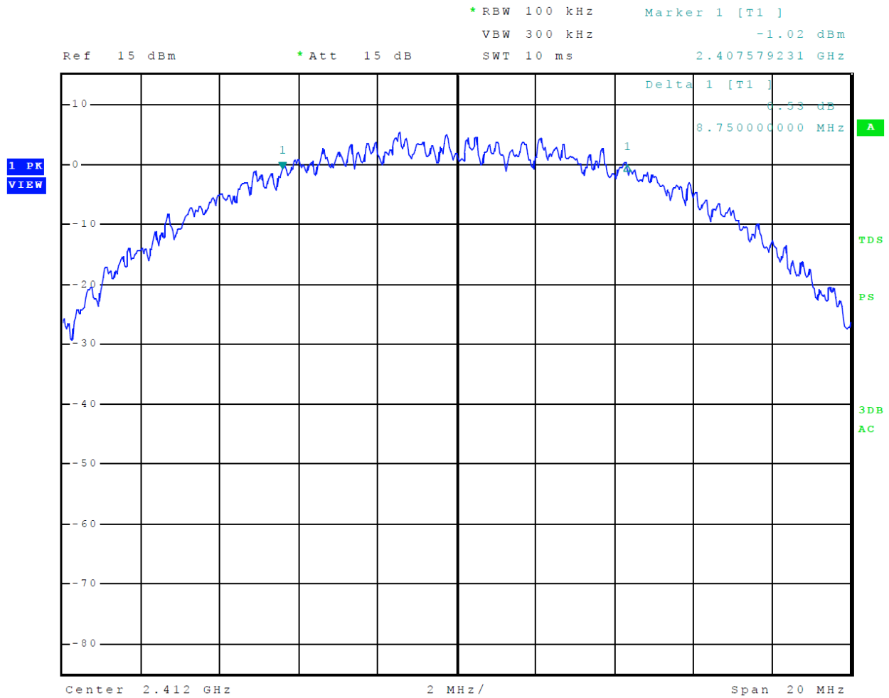
Figure 7 Plot of 6-dB Occupied Bandwidth Mode 1 802.11b
