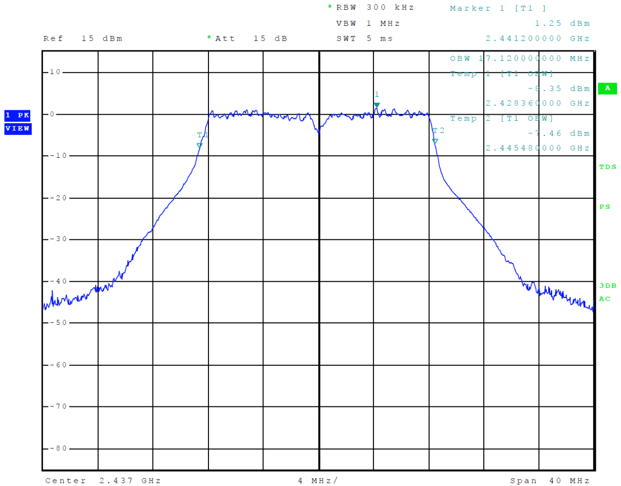
Figure 9 Plot of 99% Occupied Bandwidth Mode 2 802.11g
