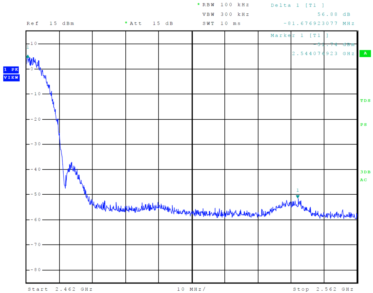
Figure 5 Plot of Transmitter Emissions High Band Edge Mode 1 802.11b
