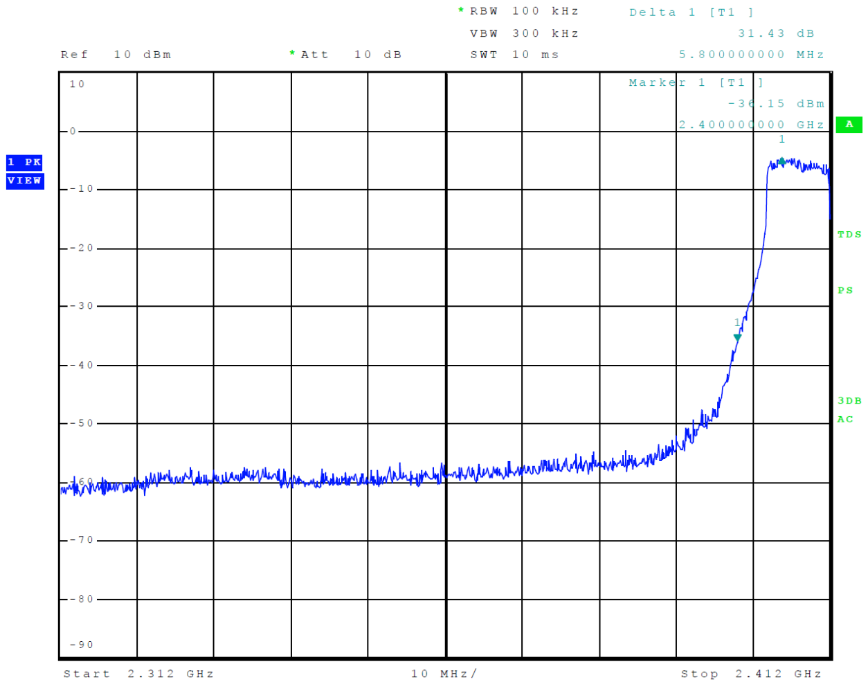
Figure 4 Plot of Transmitter Emissions Low Band Edge Mode 2 802.11g
