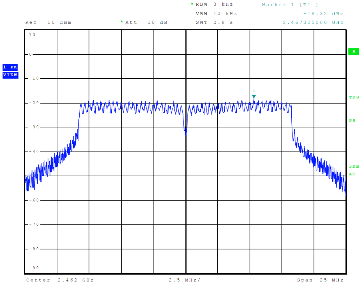
Figure 12 Plot of Transmitter Power Spectral Density Mode 2 802.11g
