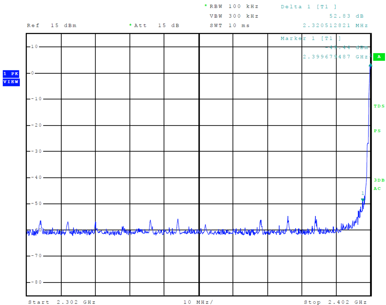
Figure 12 Plot of Transmitter Emissions Low Band Edge Mode 2 BLE (GMSK)
