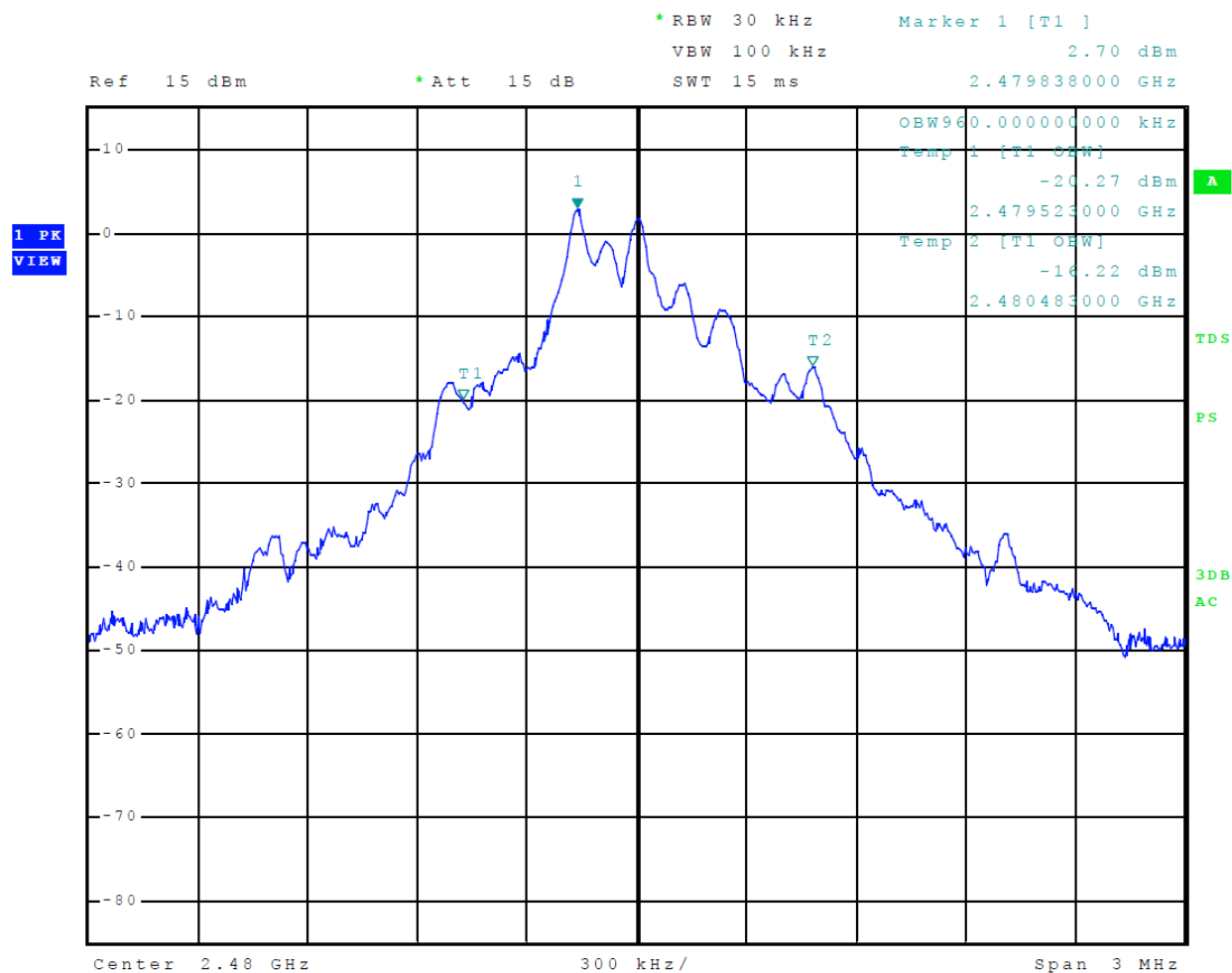
Figure 10 Plot of Transmitter Emissions 99% Occupied Bandwidth Mode 1 ANT (GFSK)
