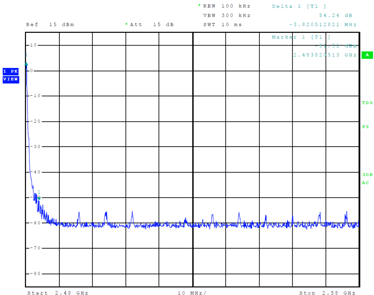
Figure 13 Plot of Transmitter Emissions High Band Edge Mode 2 BLE (GMSK)
