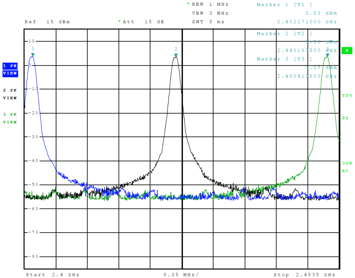
Figure 11 Plot of Transmitter Emissions Operation in 2402-2480 MHz Mode 2 BLE (GMSK)
