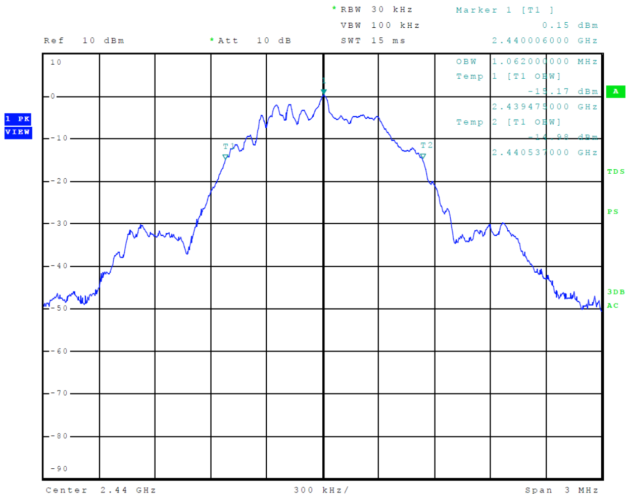
Figure 14 Plot of Transmitter Emissions 99% Occupied Bandwidth Mode 2 BLE (GMSK)
