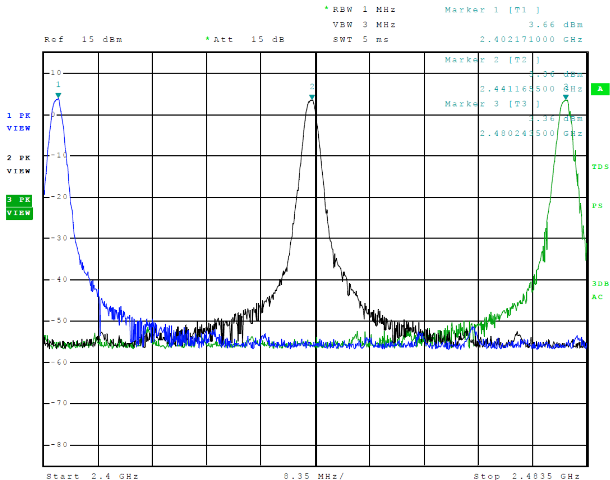
Figure 7 Plot of Transmitter Emissions Operation in 2402-2480 MHz Mode 1 ANT (GFSK)
