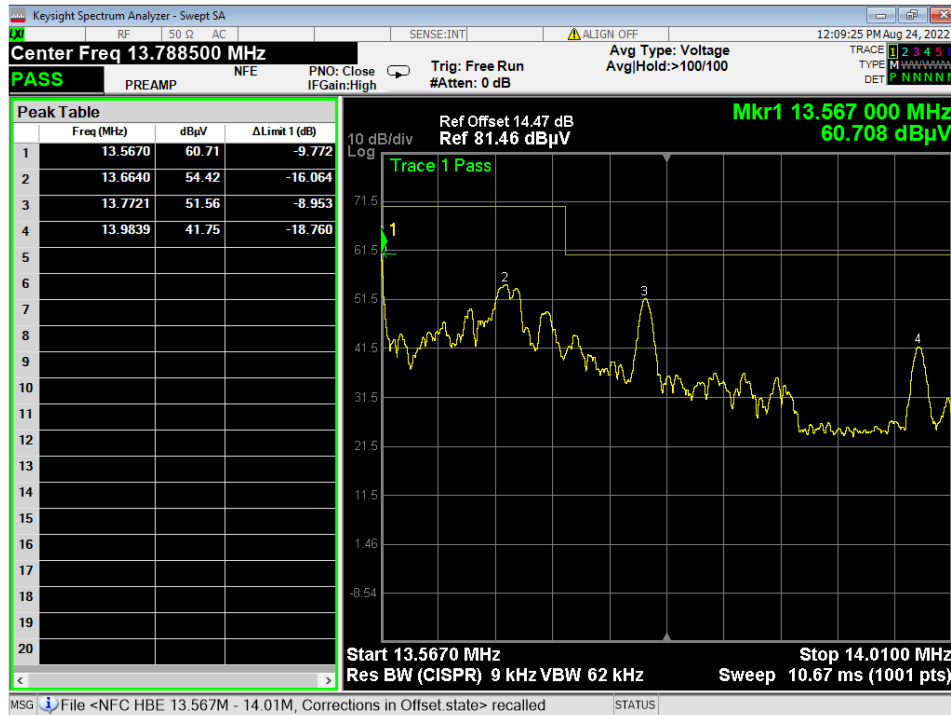
Figure 6 – Upper Bandedge
