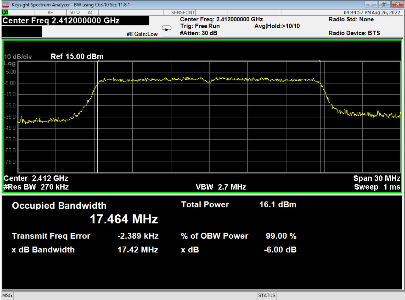
94 6dB Bandwidth, Low, Wifi N, High Data Rate
