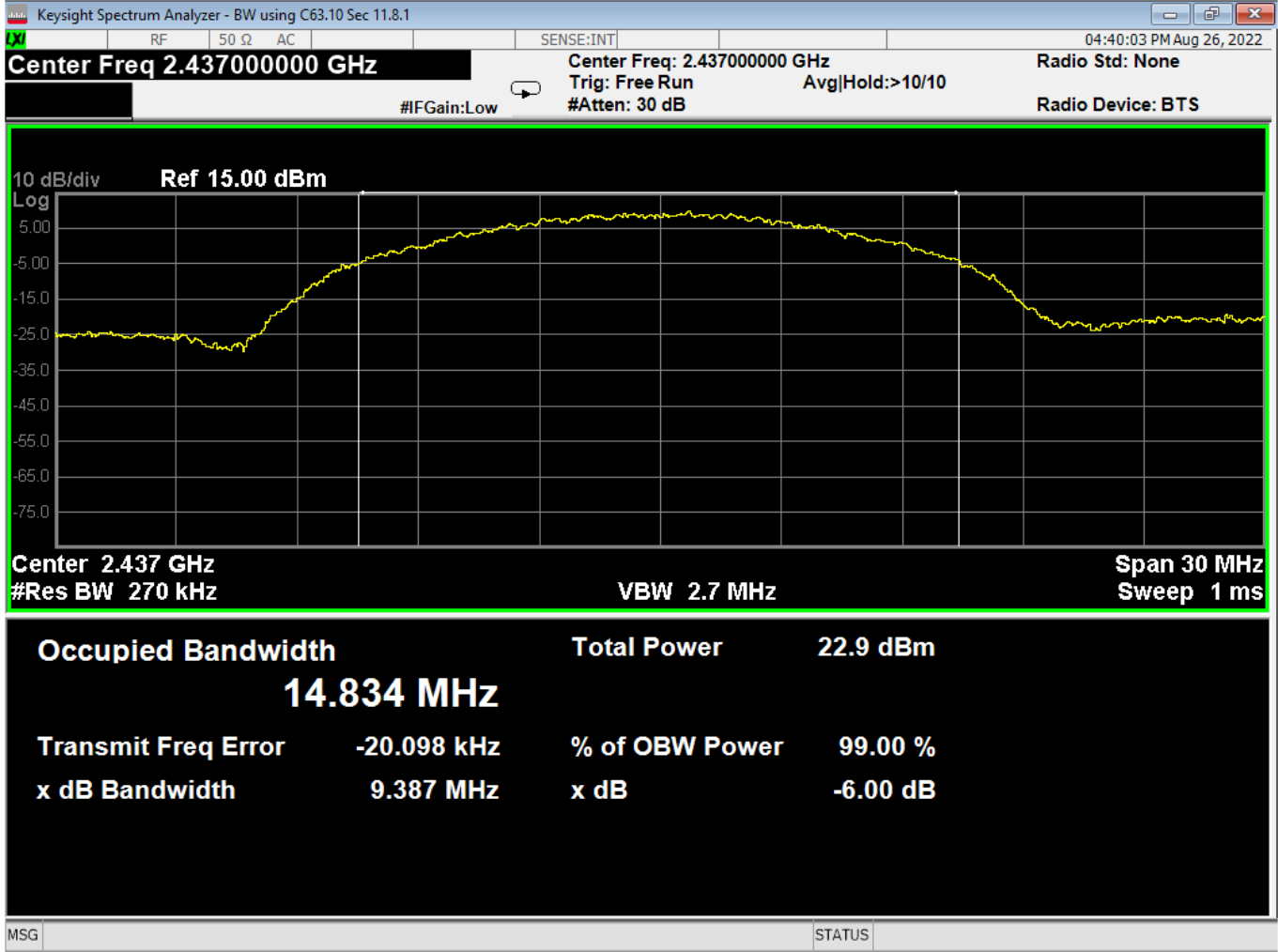
89 6dB Bandwidth, Mid, Wifi B, High Data Rate
