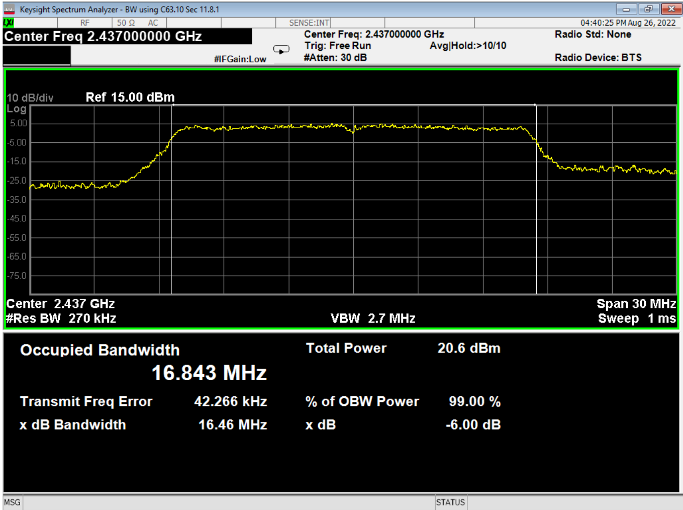
83 6dB Bandwidth, Mid, Wifi G, Low Data Rate
