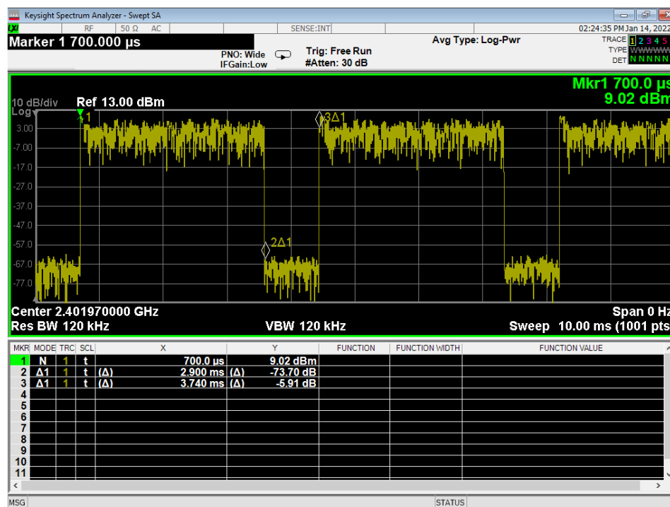
Figure 3 –Duty Cycle, 2EDR
