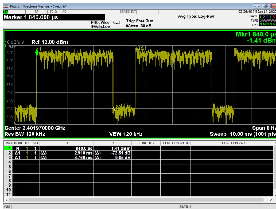
Figure 4 –Duty Cycle, 3EDR
