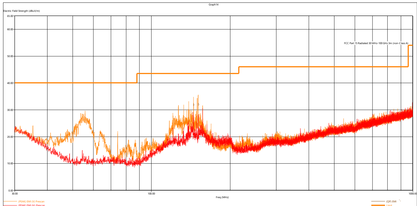
Figure 7 - Radiated Emissions Plot, BT EDR 2MB
