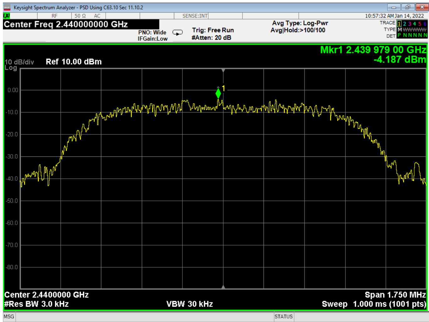
21 PSD, Mid Channel, 3EDR
