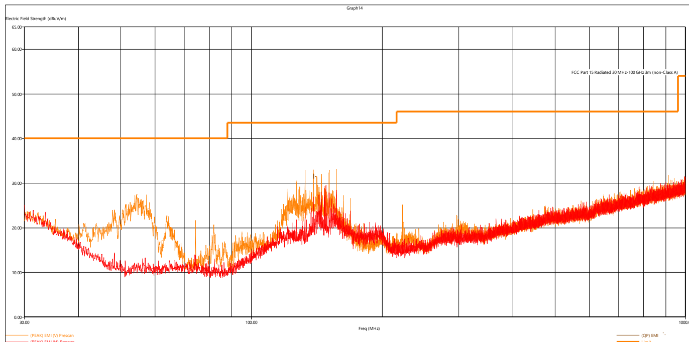
Figure 8 - Radiated Emissions Plot, BT EDR 3MB
