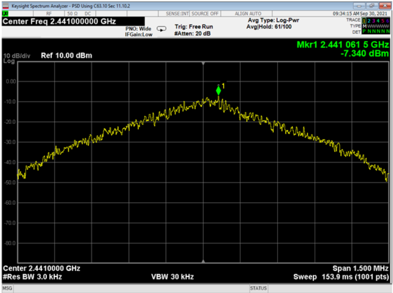
21 Power Spectral Density, Mid Frequency, GFSK
