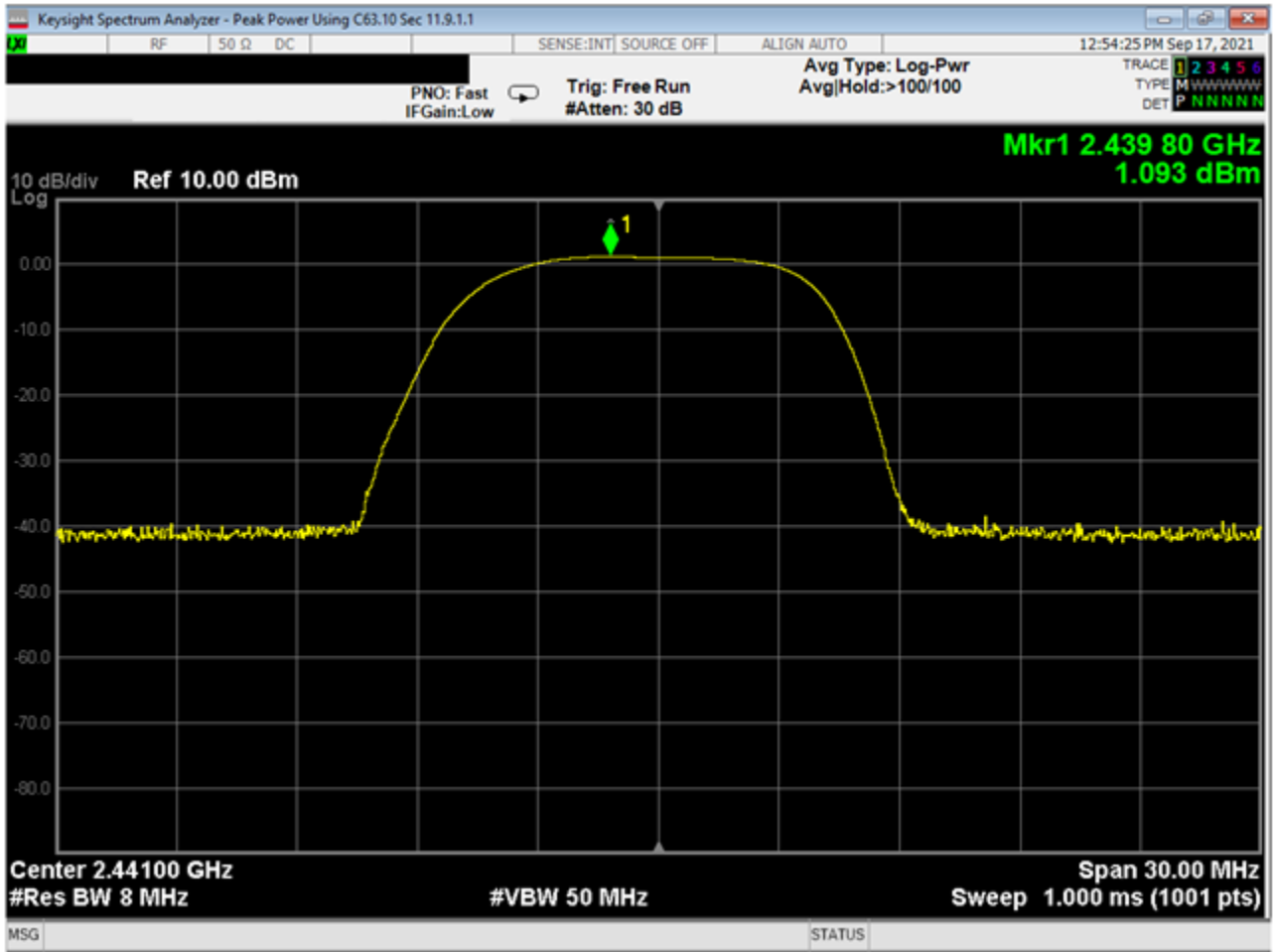
15 Peak Power, Mid Frequency, GFSK
