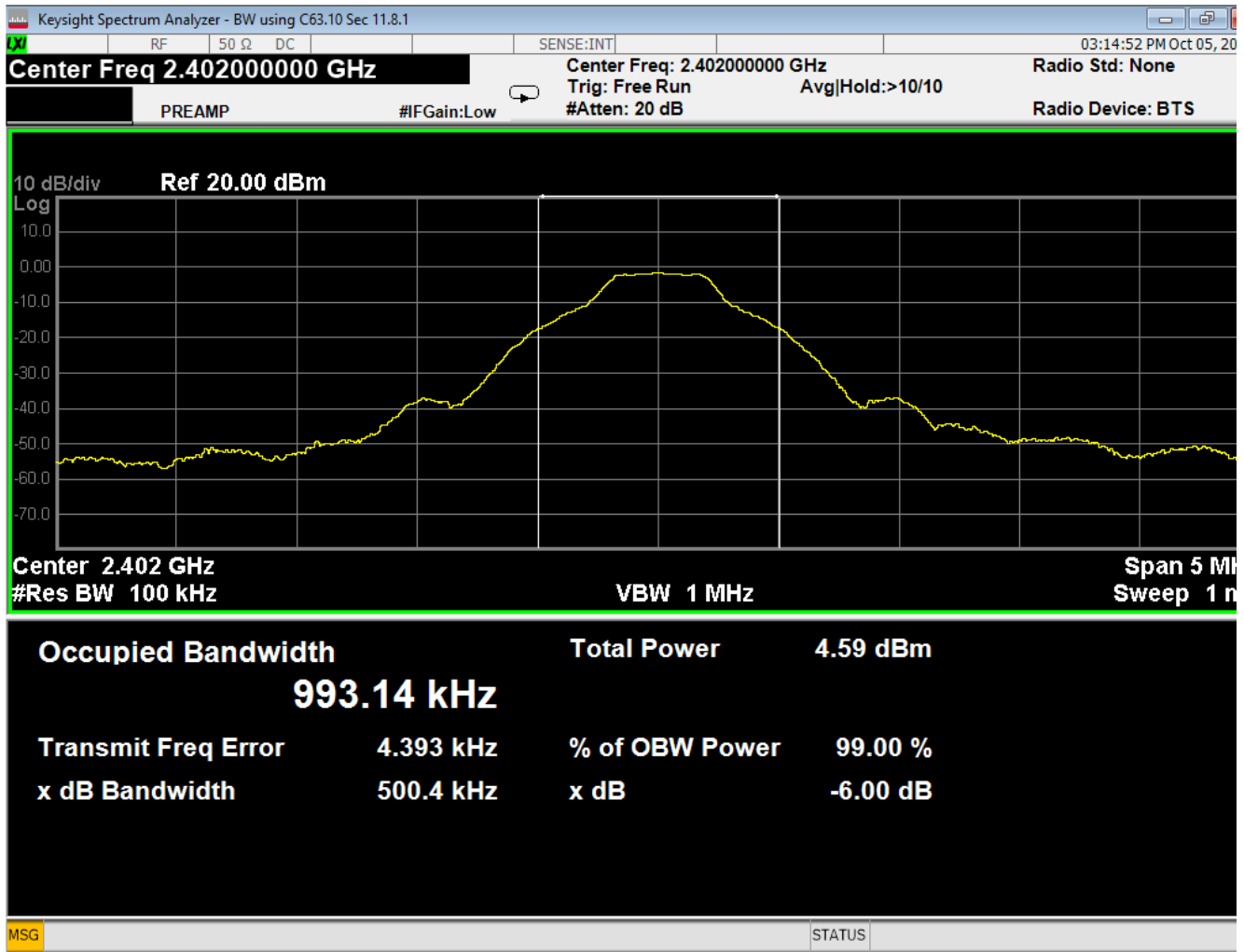
17 Bandwidth, Low Frequency, GFSK
