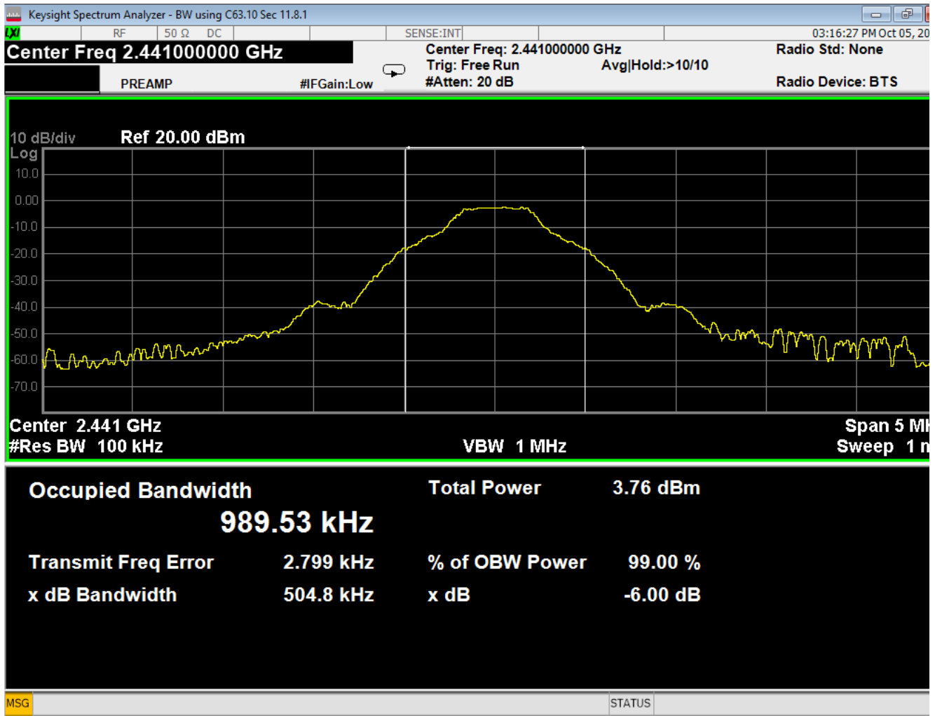
18 Bandwidth, Mid Frequency, GFSK
