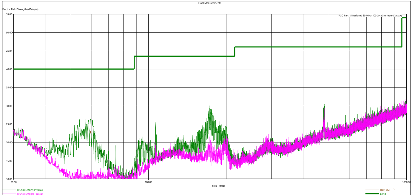
Figure 8 - Radiated Emissions Plot, Low Channel, GFSK
