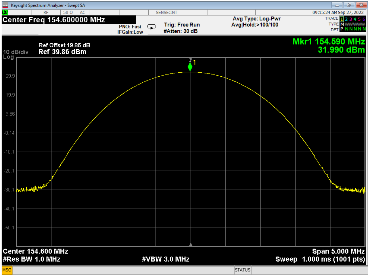
Figure 6 –Output Power, 154.600 MHz
