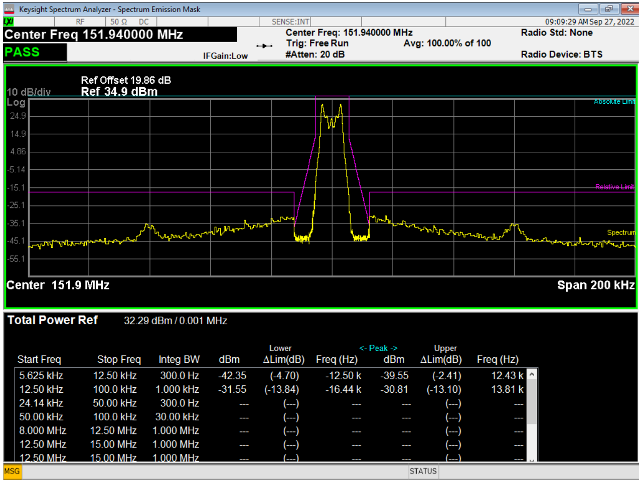
Figure 12 - Emissions Mask, 151.940 MHz
