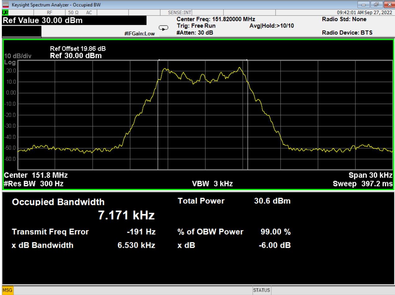
Figure 8 - Bandwidth, 151.820 MHz
