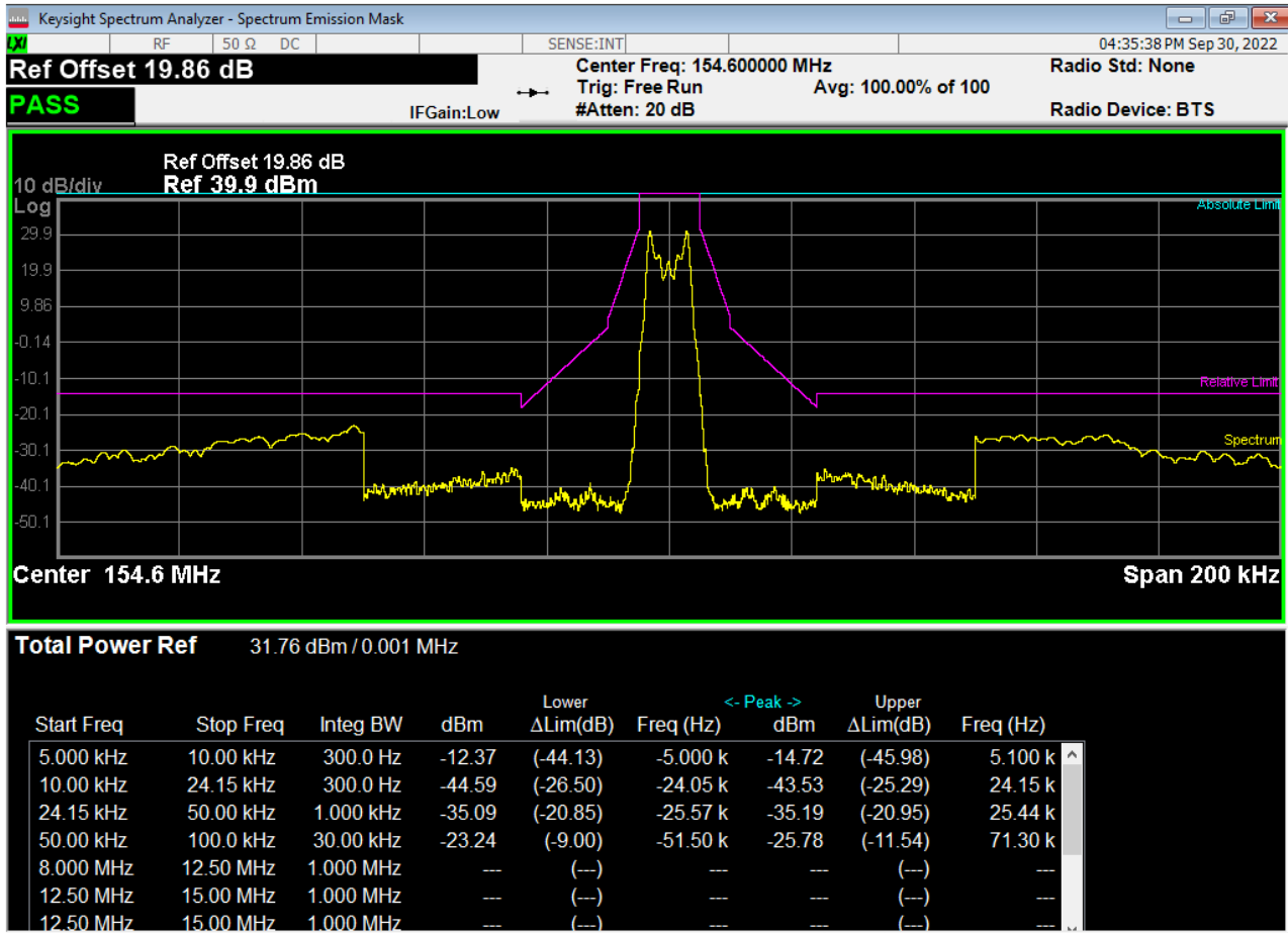
Figure 13 - Emissions Mask, 154.600 MHz
