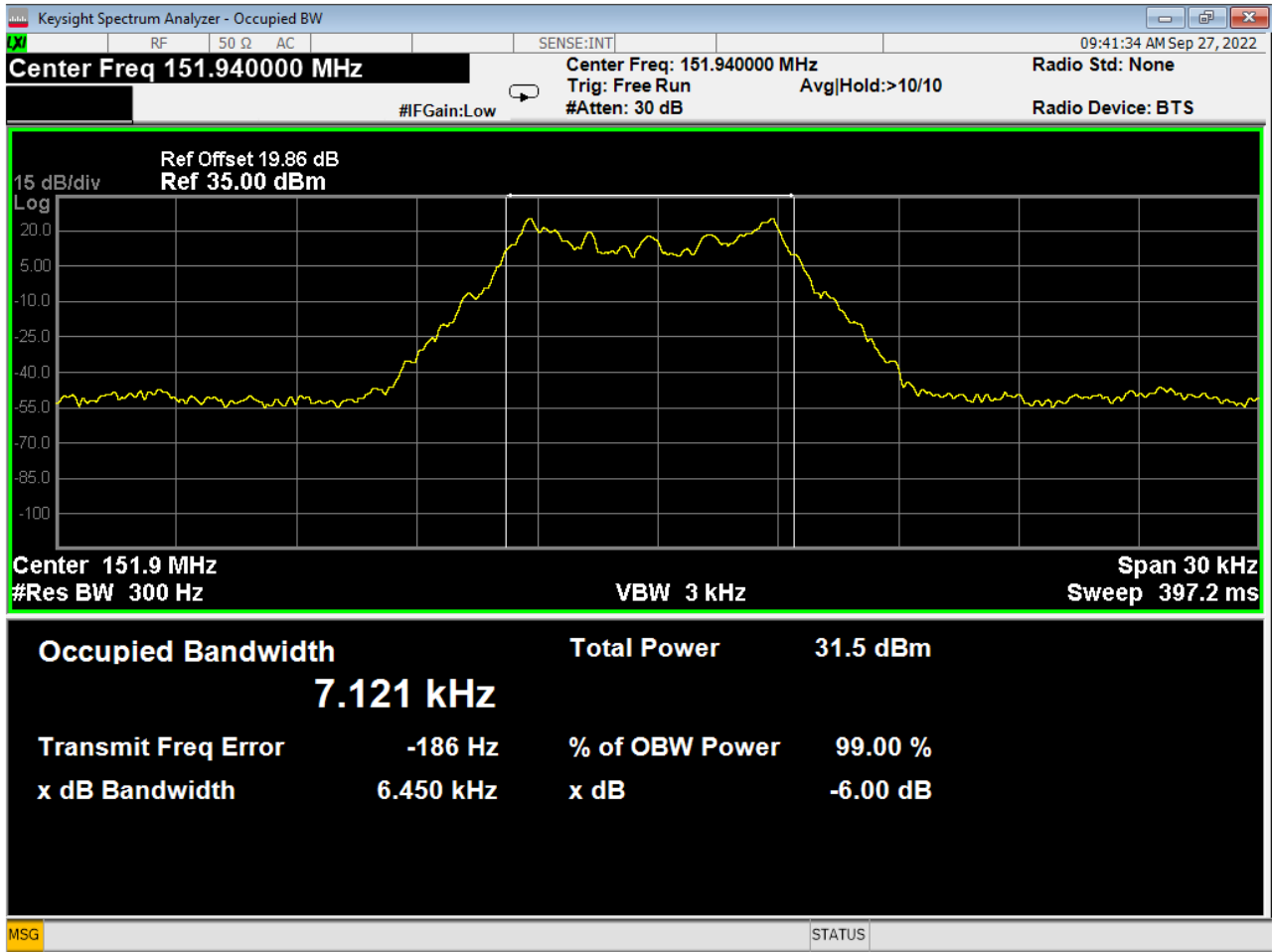
Figure 9 - Bandwidth, 151.940 MHz
