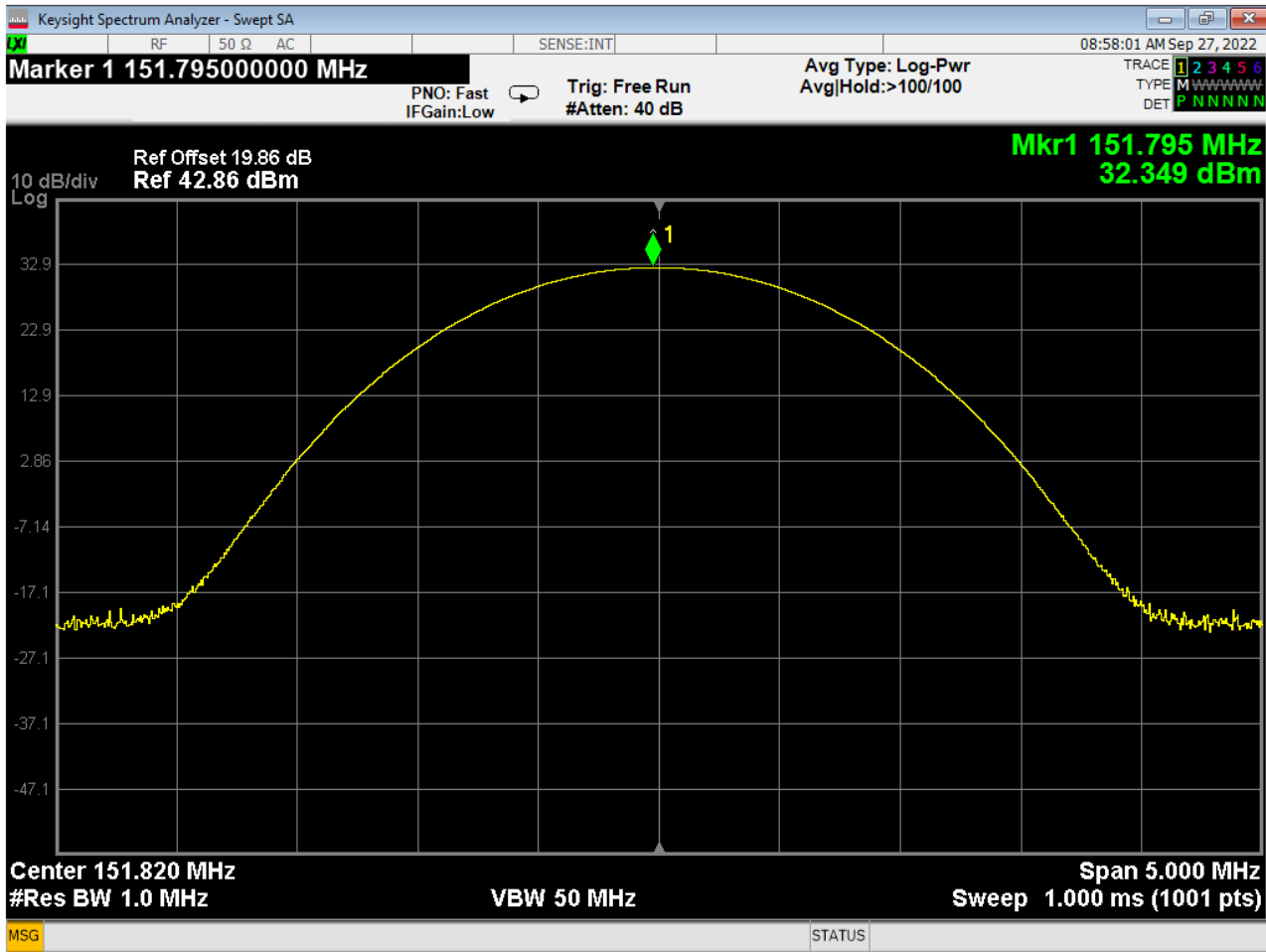
Figure 4 –Output Power, 151.820 MHz
