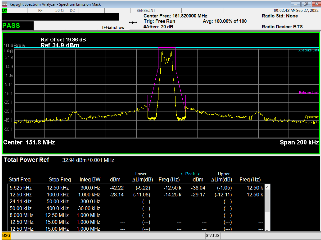
Figure 11 - Emissions Mask, 151.820 MHz
