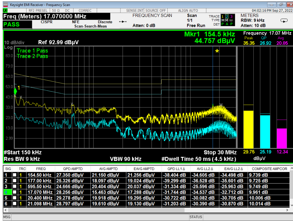
Figure 16 - Conducted Emissions Plot, Neutral
