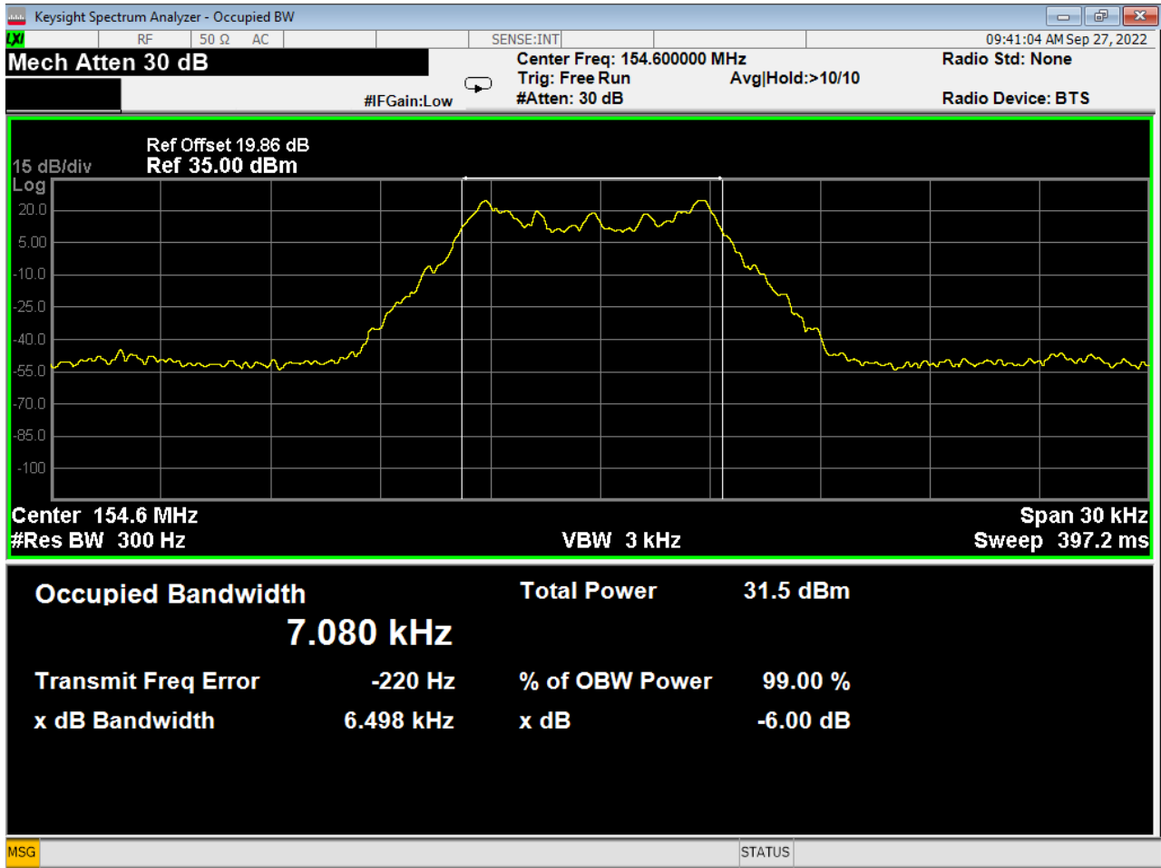
Figure 10 - Bandwidth, 154.600 MHz
