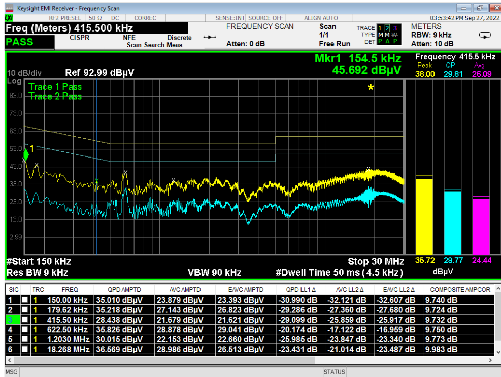
Figure 15 - Conducted Emissions Plot, Line
