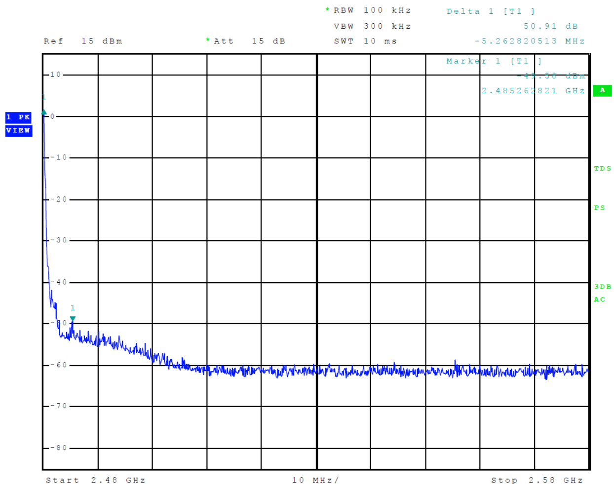
Figure 11 Plot of Transmitter Emissions High Band Edge Mode 2 BT BR (GFSK)
