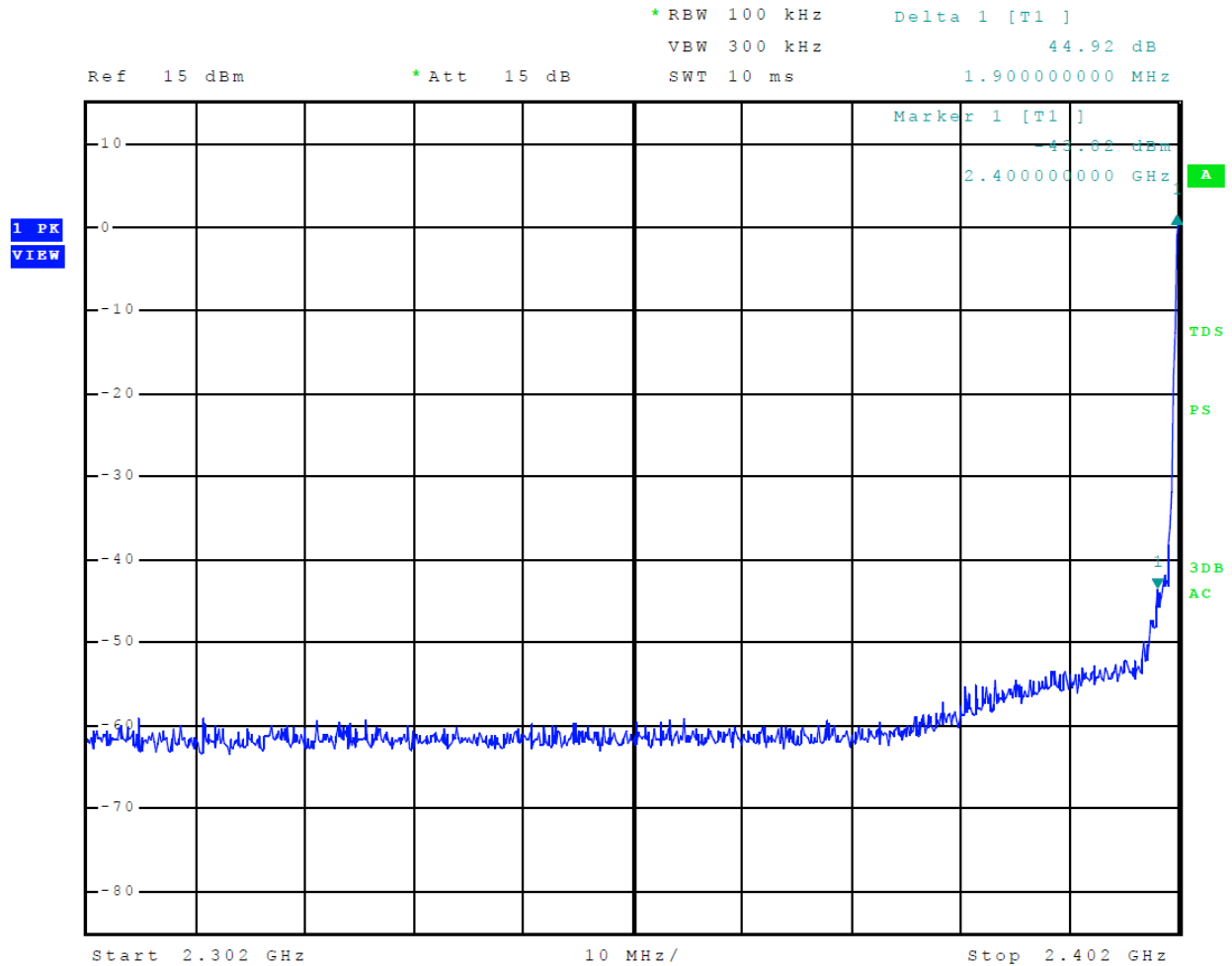
Figure 10 Plot of Transmitter Emissions Low Band Edge Mode 2 BT BR (GFSK)
