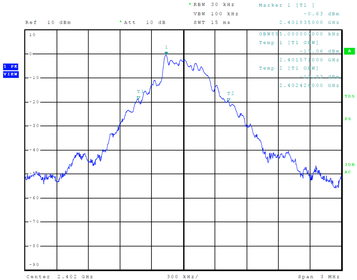
Figure 12 Plot of Transmitter Emissions 99% Occupied Bandwidth Mode 2 BT BR (GFSK)
